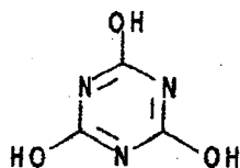
Cyanuric Acid
