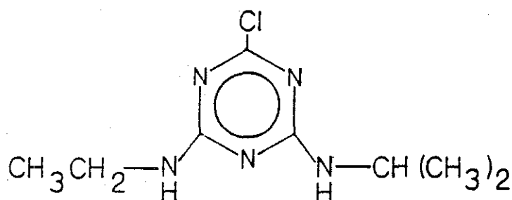
Atrazine G-30027 2-Chloro-4-ethylamino- 6-isopropylamino-s- triazine
