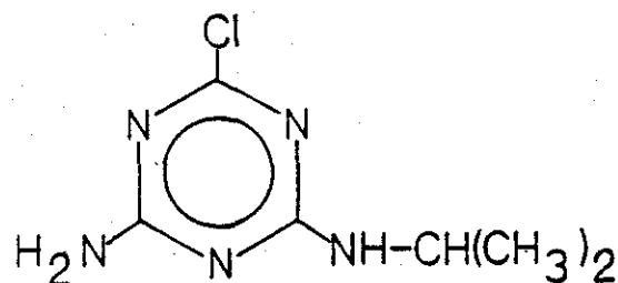
G-30033 2-Amino-4-chloro-6- isopropylamino-s- triazine
