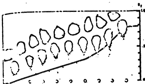
Fig. 3—Effect of soil pH (line) on the mobility of dicamba (upper spots) and fenac (lower spots) in a modified Hagerstown silt plate.
