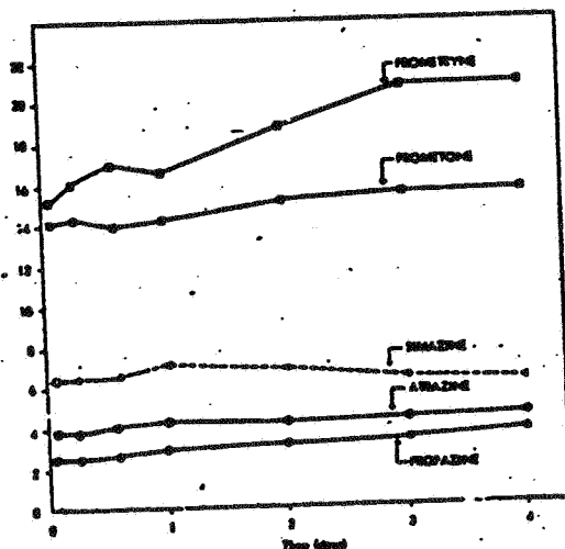
Figure 1. Effect of time on the distribution coefficient ( K_d ) of five s-triazines between Marshall silty clay loam and the aqueous phase of the suspension.
