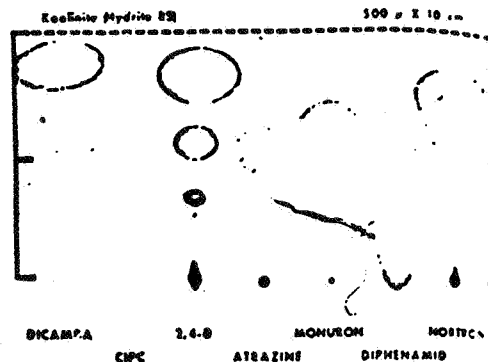
Fig. 8.—Movement of herbicides in a kaolinite TLC plate.
