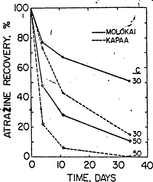
Figure 2. Atrazine recovery by methanol extraction of the Molokai and Kapaa soils treated with 10 ppmw ^{14}\text{C} -atrazine and incubated at 30 and 50°C (Corrections were made for the presence of triazine degradation products in the methanol extract).
