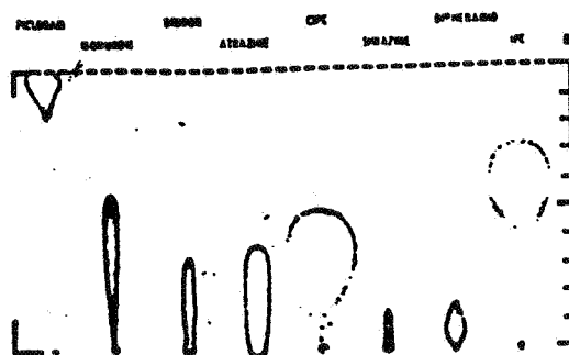
Fig. 4—Effect of organic matter oxidation on mobilities of eight herbicides in a Hagerstown silt plate.
