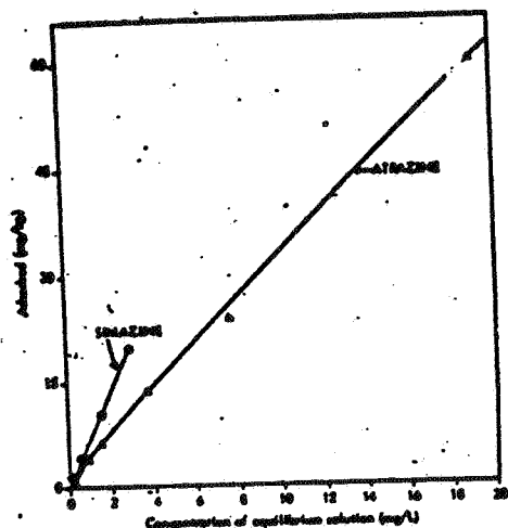
Figure 1. Isotherms for the adsorption of simazine and atrazine by Marshall silty clay loam.
