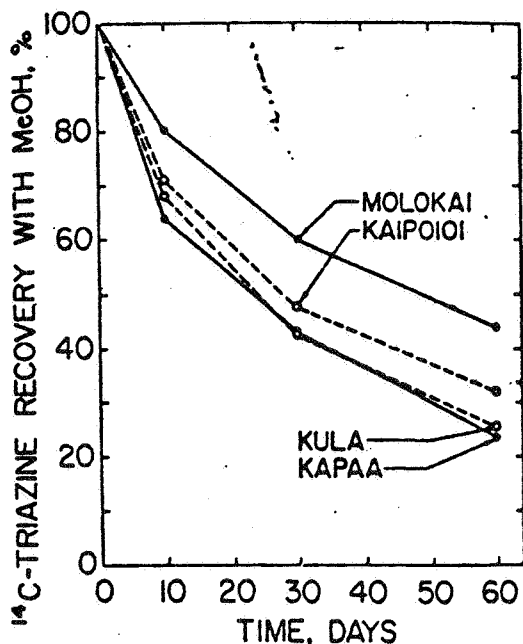
Figure 1. ^{14}\text{C} -triazine recovery by methanol extractions of four Hawaiian soils treated with 10 ppmw ^{14}\text{C} -atrazine (No correction was made for the presence of ^{14}\text{C} degradation products).
