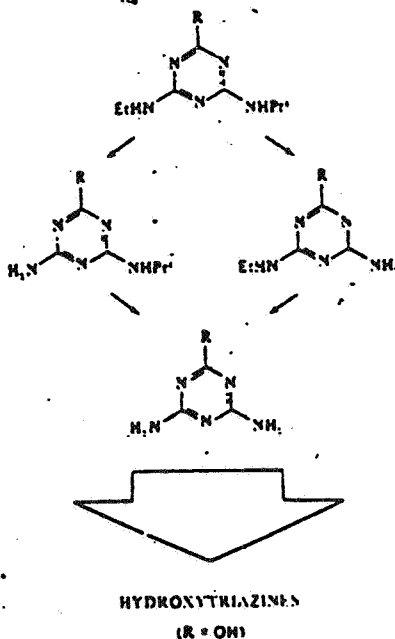
Figure 1. Pathway of photolytic degradation of atrazine (R = CN) and atraton (R = OMe) in aqueous solution containing 1% of acetone.
