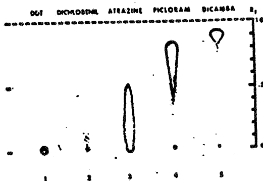
Fig. 1.—Movement of five pesticides in Hagerstown silt soil TLC plates, 500 \mu by 10 cm. Number below each pesticide refers to the mobility class (22; see also Table 1).
