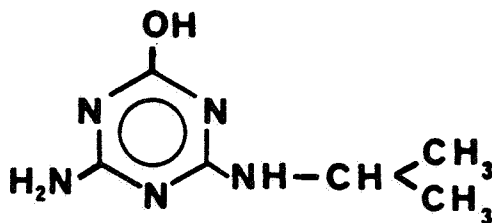
2-Amino-4-hydroxy-6-isopropylamino- s-triazine
