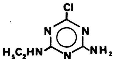
2-Amino-4-chloro-6-ethylamino-s-triazine
