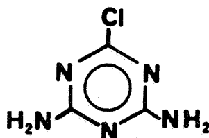
2,4-diamino-6-chloro-triazine
