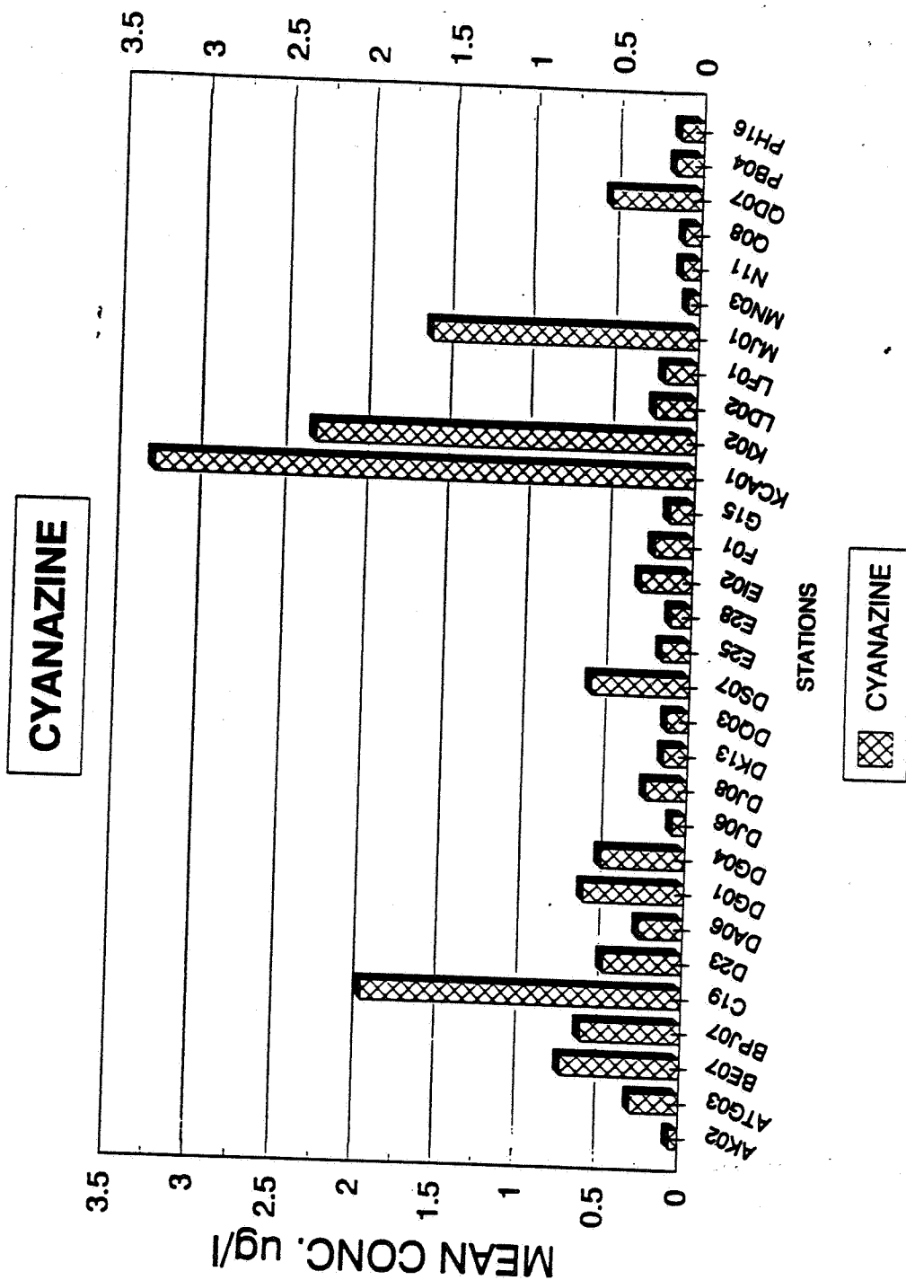
Figure 11. Mean concentrations from October 1985 to October 1988 for cyanazine for each Pesticide Subnetwork Station
