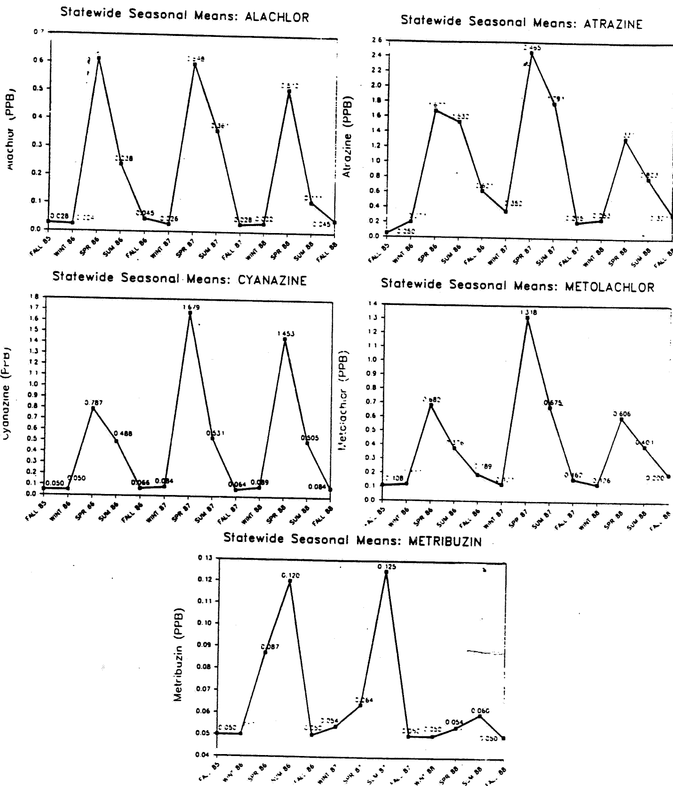
8.6 Figure 3 Statewide Seasonal Means
