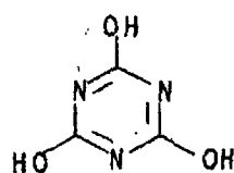
Cyanuric acid
