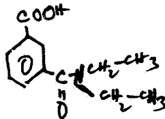
Metabolite A
