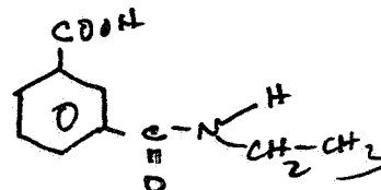
Metabolite B
