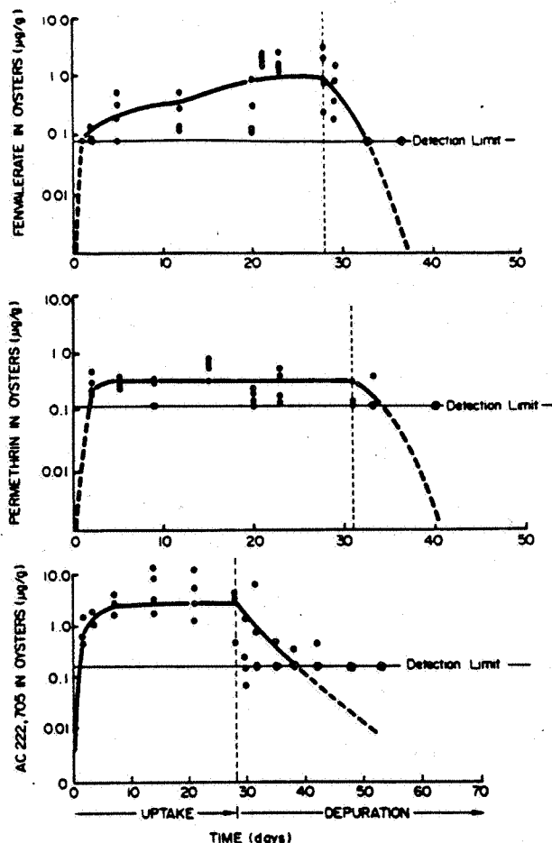
Figure 2. Uptake and depuration of AC 222,705, fenvalerate, and permethrin by eastern oysters ( Crassostrea virginica ) in flowing seawater tests.
