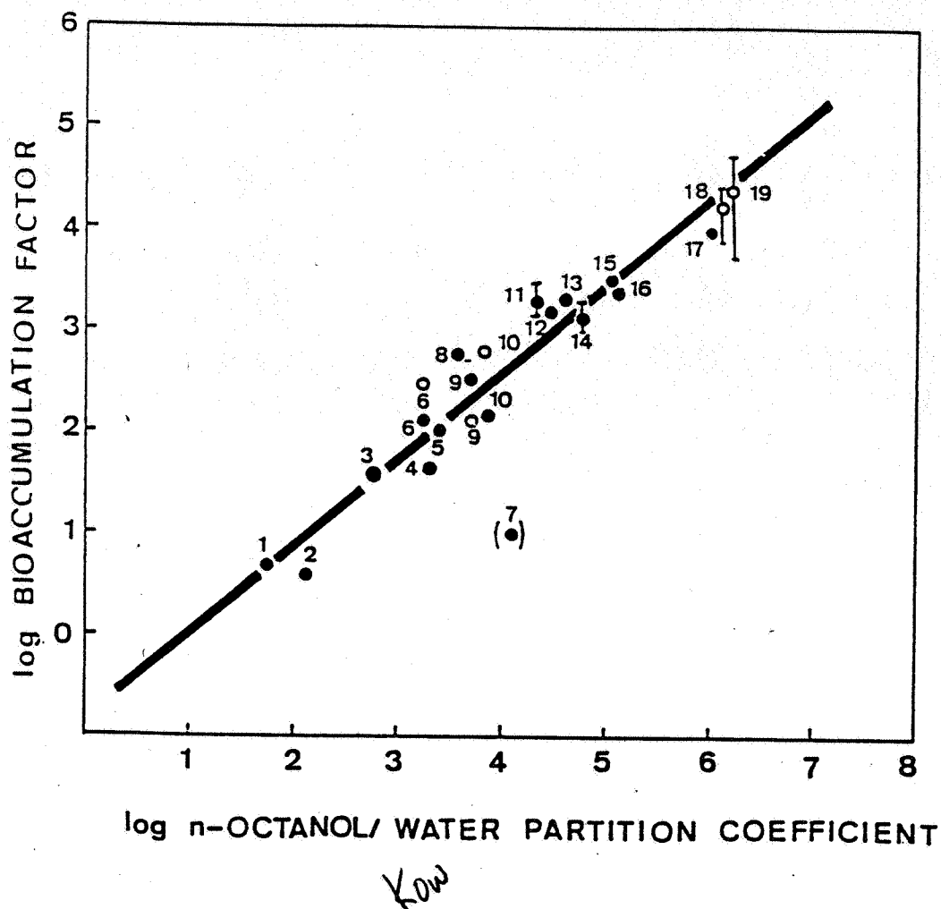
Fig. 2. Correlation of log bioaccumulation factor in the mussel Mytilus edulis with log n-octanol/water partition coefficient for organic chemicals. (Solid circles (•) designate laboratory experiments; open circles (o) indicate data from environmental analysis).
