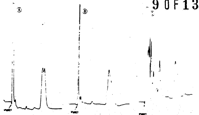
Figure 3. Gas chromatograms of extracts from studies with AC 222,705. (A) AC 222,705 standard response. (B) Tissue extract from the oyster bioconcentration study. (C) Sediment extract from the persistence study.
