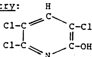
3,5,6-trichloro-2-pyridinol [TCP]
