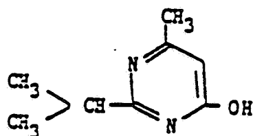
OXYPYRIMIDINE (G-27550)
