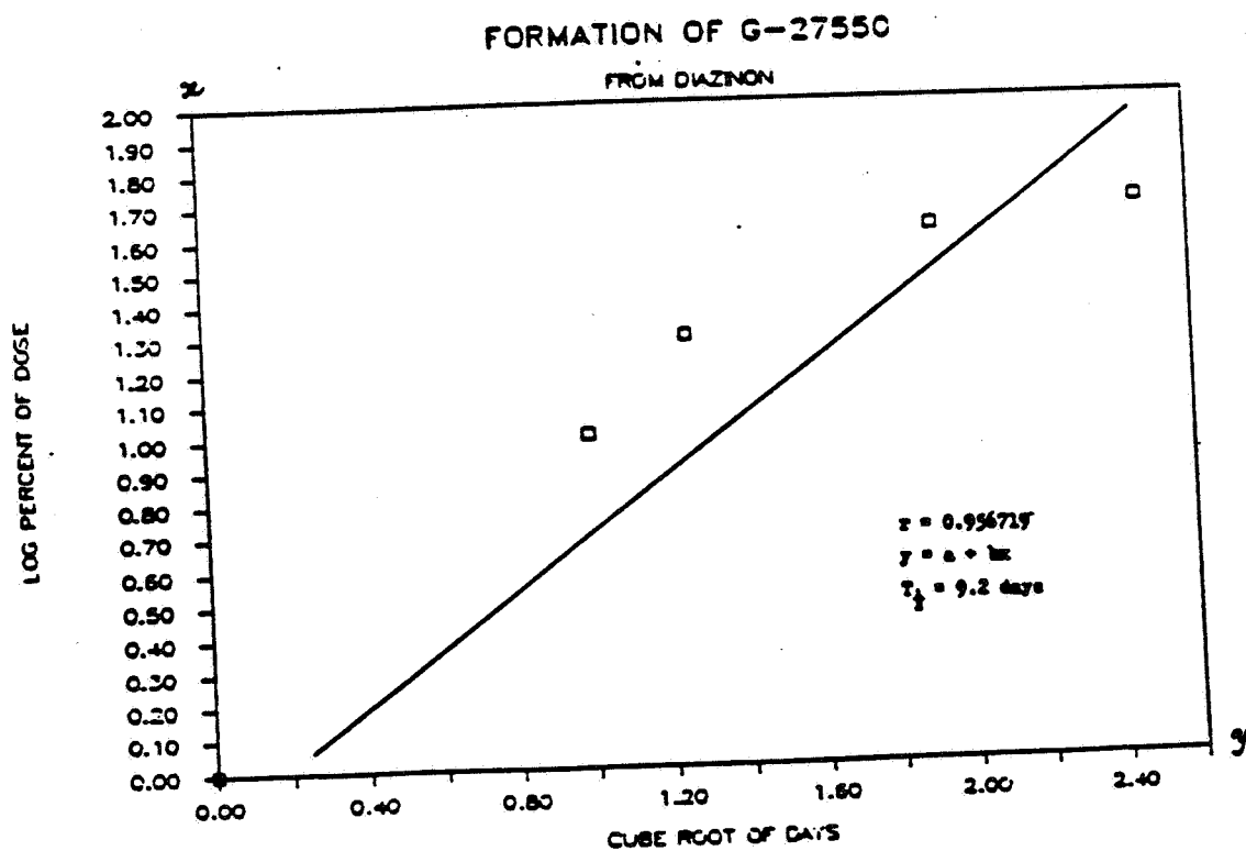
Figure 13. Kinetics of Formation of G-27550 from Diazinon Under Anaerobic Aquatic Soil Conditions
