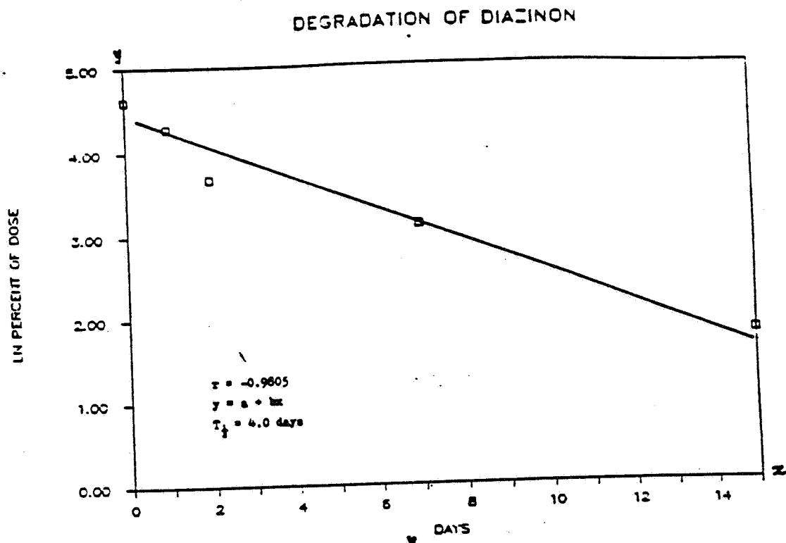
Figure 12. Kinetics of Degradation of Diazinon Under Anaerobic Aquatic Soil Conditions
