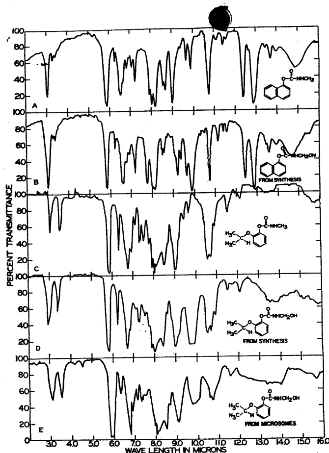
Figure 2. Infrared spectra for Sevin and Bayer 39007 (A and C), their N -hydroxymethyl analogs from synthesis (B and D), and one metabolite of Bayer 39007 from microsomes (E)
