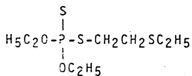
Ethylthiometon
