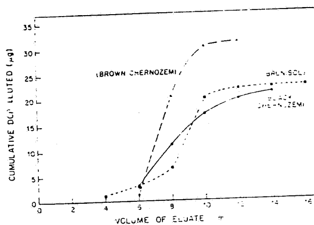
Figure 4. Elution curves of DCP from soil columns, 15 cm high and 0.7 cm in diameter. Application at 1.0 kg/ha. Flow rates averaged 0.5 mL/min.
