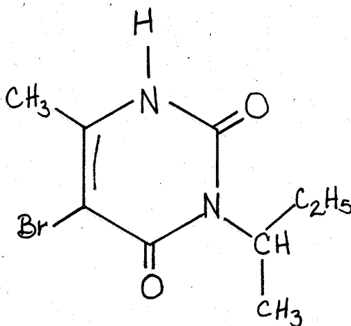
BROMACIL
