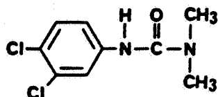
3-(3,4-DICHLOROPHENYL)-1,1-DIMETHYL- UREA
