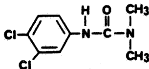
3-(3,4-DICHLOROPHENYL)-1,1-DIMETHYL- UREA
