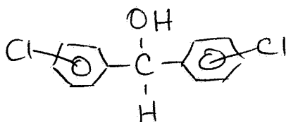
DCBH dichlorobenzhydrol
