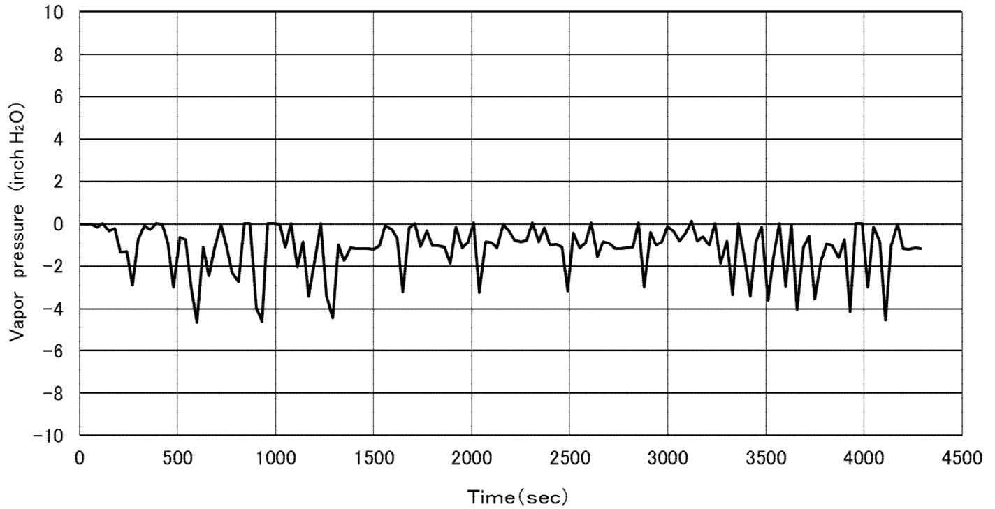
(b) Measured vapor space pressure profile
