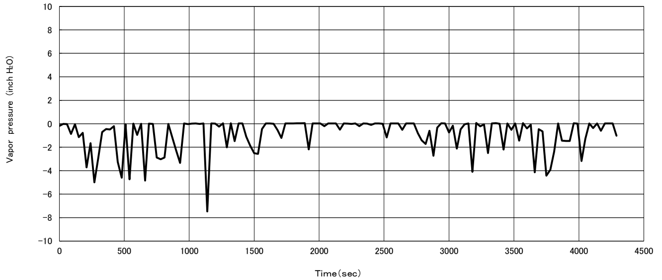
(b) Measured vapor space pressure profile
