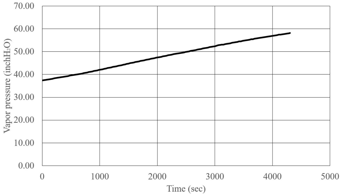
(b) Measured vapor space pressure profile
