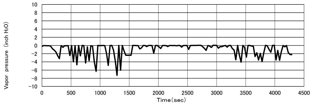
(b) Measured vapor space pressure profile
