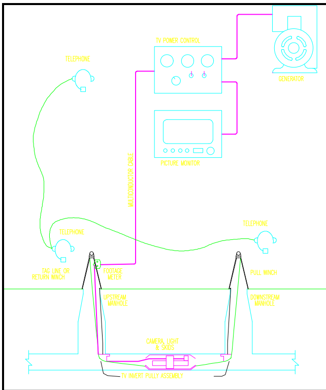
FIGURE 1 SETUP OF CCTV EQUIPMENT
