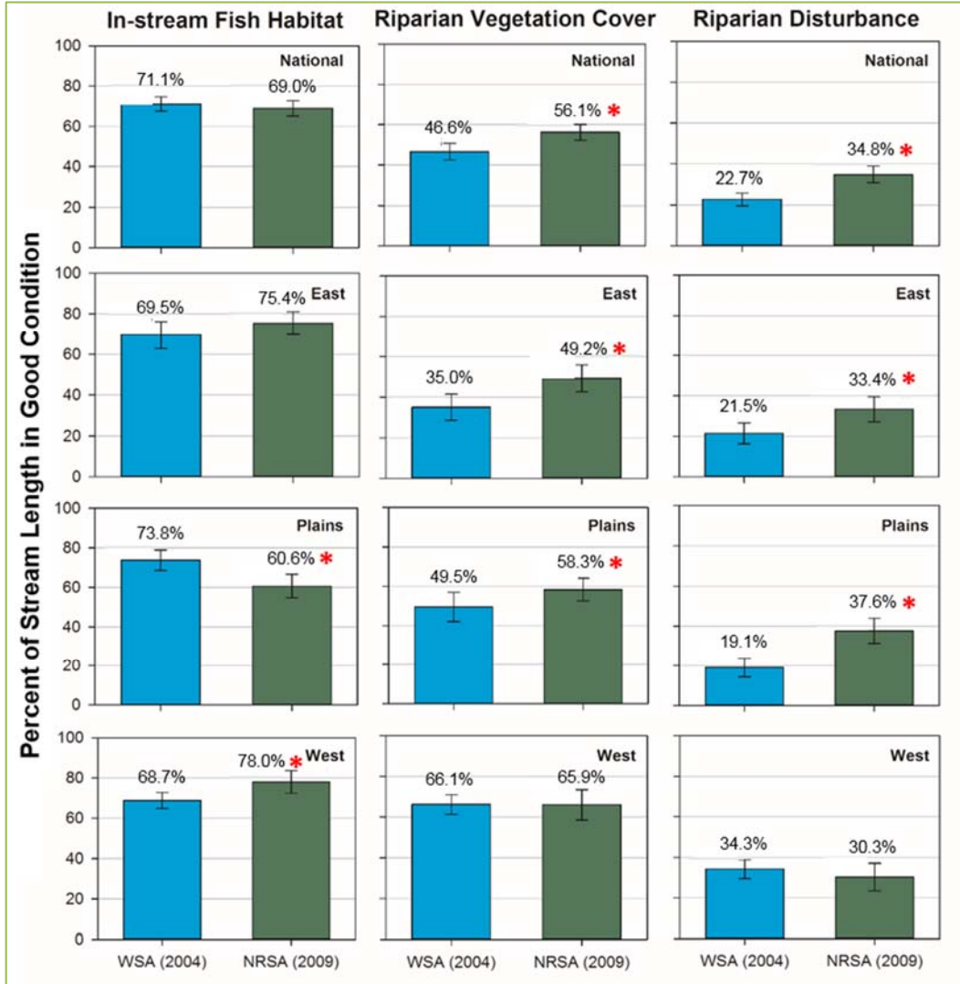
Figure 29. Change in stream fish habitat, riparian vegetation cover, and riparian disturbance between 2004 and 2008–2009 (EPA/NRSA). Percent of stream length in good condition; red stars indicate statistically significant change.
