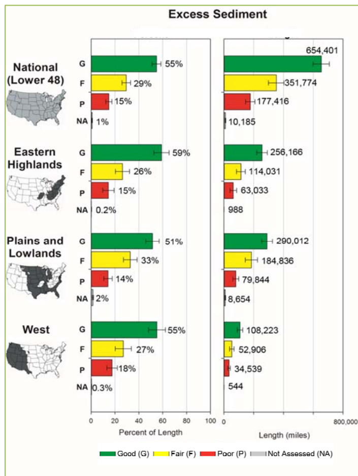
Figure 15. Excess streambed sediment in the nation's rivers and streams (EPA/NRSA).
