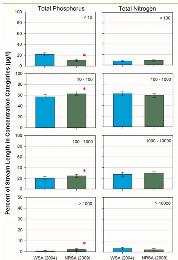
Figure 28. Total phosphorus and nitrogen concentrations in the nation's streams (EPA/NRSA). Percent of stream length in concentration categories for nutrients. Red stars indicate statistically significant change
