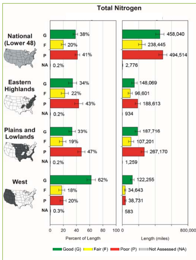
Figure 12. Total nitrogen concentrations in the nation's rivers and streams (EPA/NRSA). Percentages of river and stream length in good, fair or poor condition for nitrogen are compared to least-disturbed regional reference sites.
