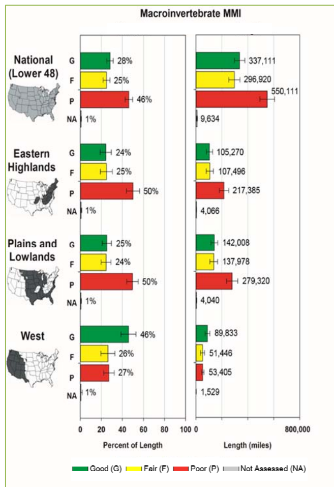
Figure 8. Biological condition of the nation's rivers and streams based on the macroinvertebrate MMI (EPA/NRSA.) This index combines metrics of benthic community structure and function into a single index for each region.
