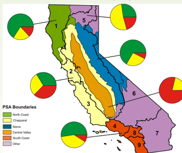
Figure 49. Biological condition of perennial streams in the six major ecoregions of California. Green = good biological condition, yellow = altered biological condition, and red = very altered biological condition.
