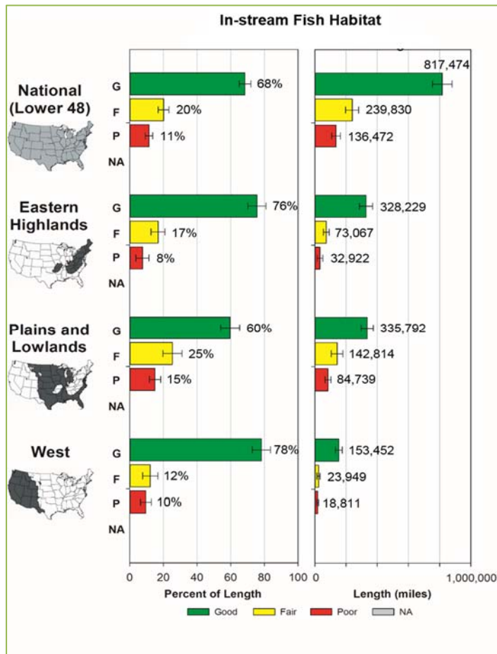
Figure 16. In-stream fish habitat in the nation's rivers and streams (EPA/NRSA).
