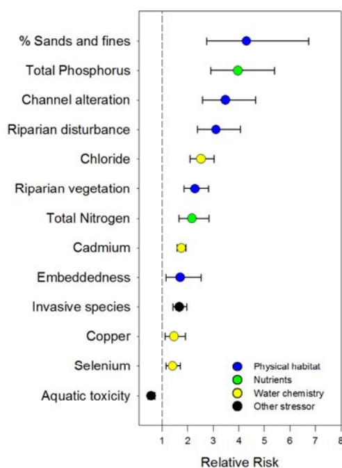
Figure 51. Relative risk of biological impairment associated with a series of habitat and chemistry variables in southern California streams.
