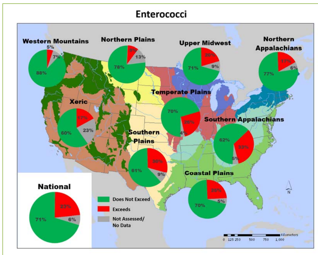
Figure 36. Enterococci human health threshold exceedance in rivers and streams across the nine ecoregions (EPA/NRSA). Margin of error for national results is approximately \pm 3\% ; for the ecoregions, the margin of error ranges between \pm 2 and \pm 11\% . Percentages may not add up to 100% due to rounding.
