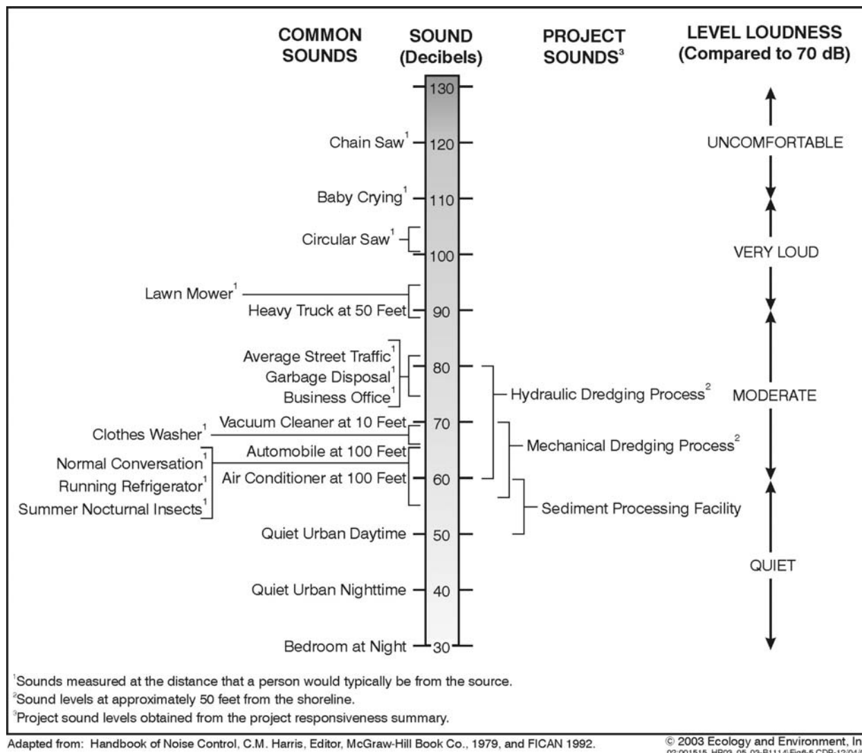
Figure 6-5 Comparison of Predicted Hudson River PCBs Superfund Site Noise Levels and Other Sources of Noise
