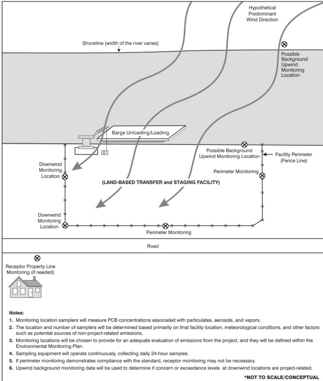
Figure 6-2 Conceptual Air Quality Monitoring Layout: Land-based
