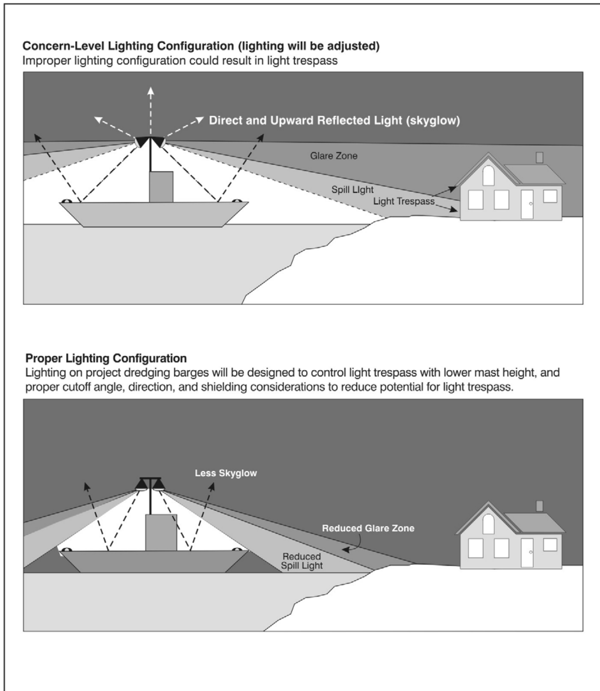
Figure 6-7 Conceptual Barge Lighting Configurations
