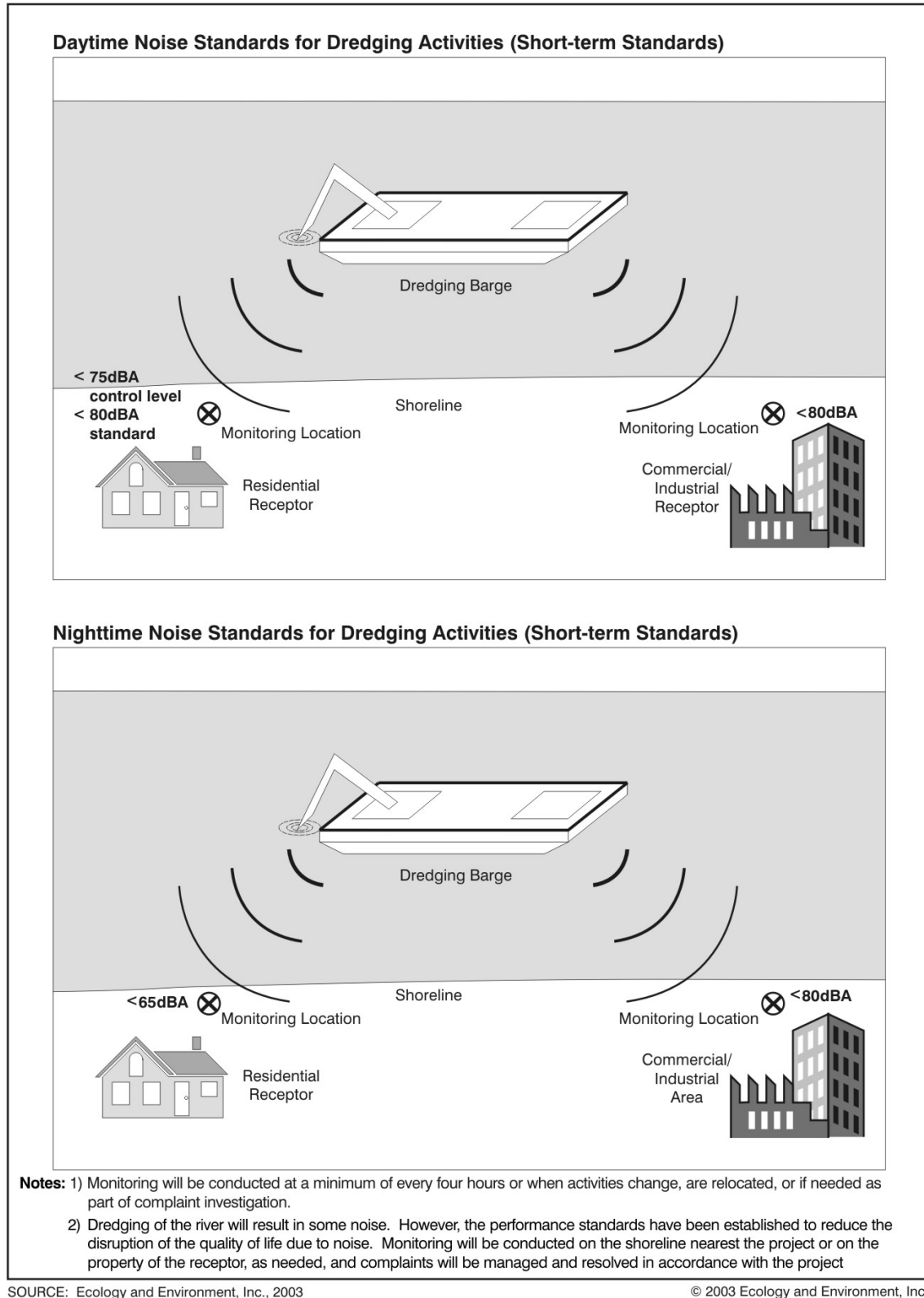
Figure 6-6 Conceptual Noise-Monitoring Layout
