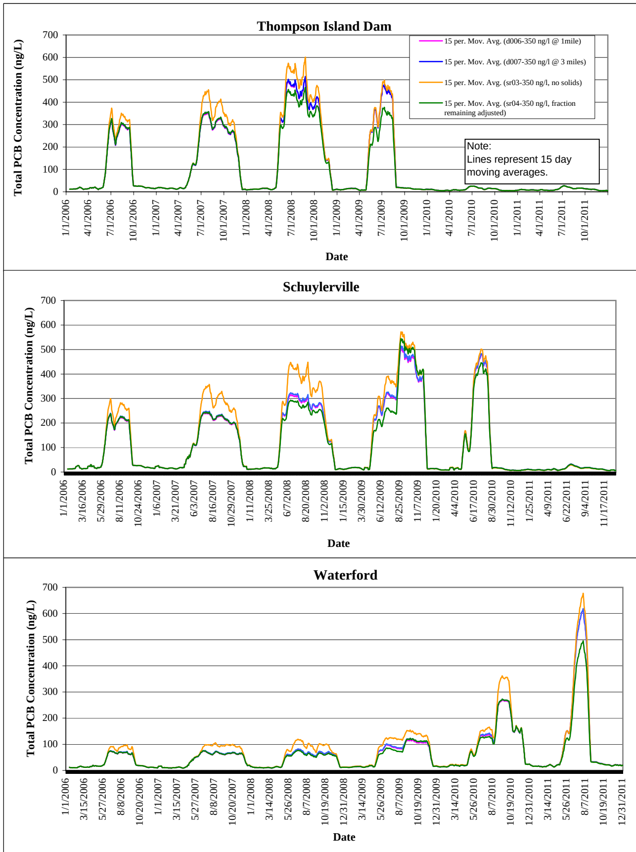
Figure 31 Whole Water Total PCB Concentration for Different 350 ng/L Input Formulations
