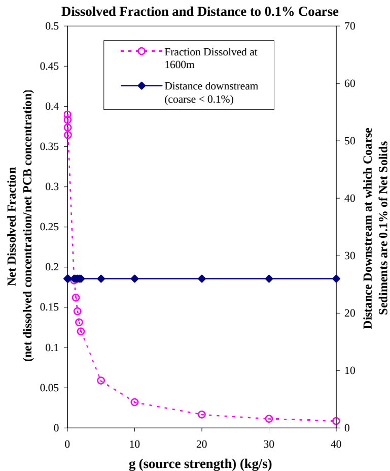
Figure 20 Net Dissolved PCB Fraction, Distance to Coarse < 0.1%, Net Total PCB Flux and Net TSS Flux at 1600 meters as Functions of Source Strength for the TSS-Chem
