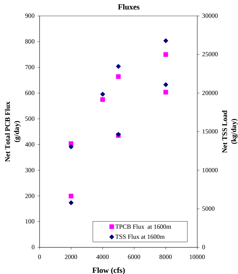
Figure 17 Net Dissolved PCB Fraction, Distance to Coarse < 0.1%, Net Total PCB Flux and Net TSS Flux at 1600 meters as Functions of Riverwide Volumetric Flow (Velocity-Depth Pairs) for the TSS-Chem
