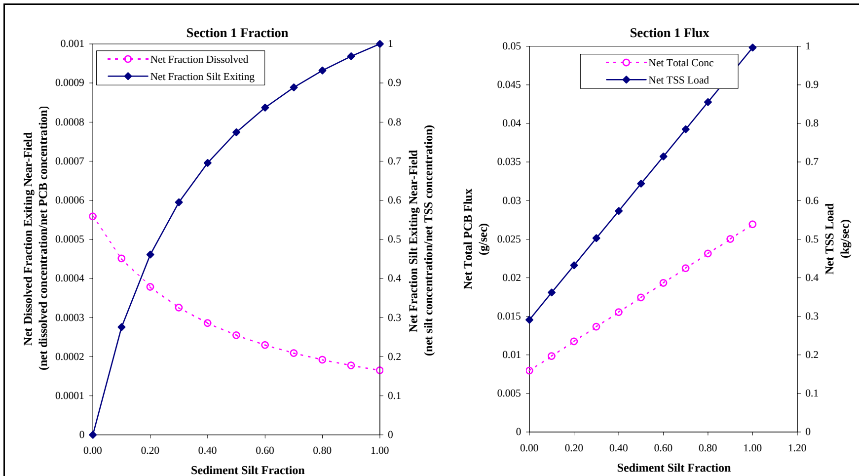
Figure 7 Net Dissolved PCB Fraction, Net Silt Fraction, Net Total PCB Flux and Net TSS Flux Exiting Near-Field as Functions of Sediment Silt Fraction for CSTR-Chem
