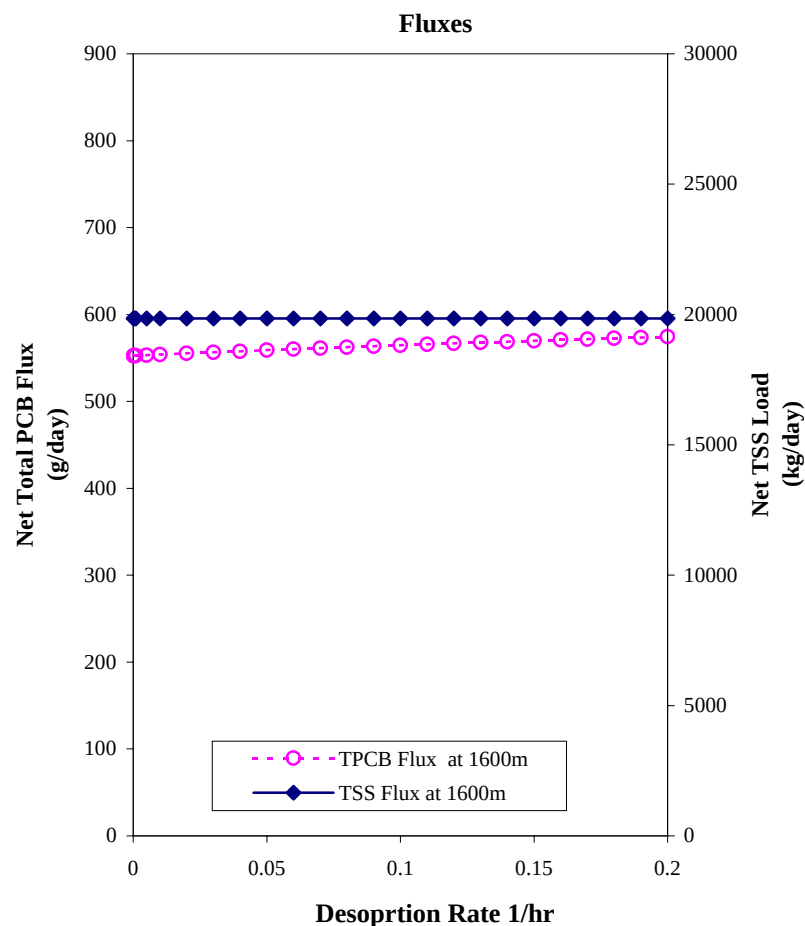
Figure 25 Net Dissolved PCB Fraction, Distance to Coarse < 0.1%, Net Total PCB Flux and Net TSS Flux at 1600 meters as Functions of Desorption Rate for the TSS-Chem
