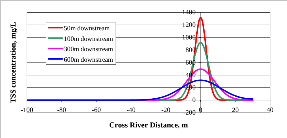
Figure 15 Estimated TSS Concentration Downstream of the Dredge Head in Section 1 (Flow is 4000 cfs and PCB concentration is 500 ng/L at the far field station)
