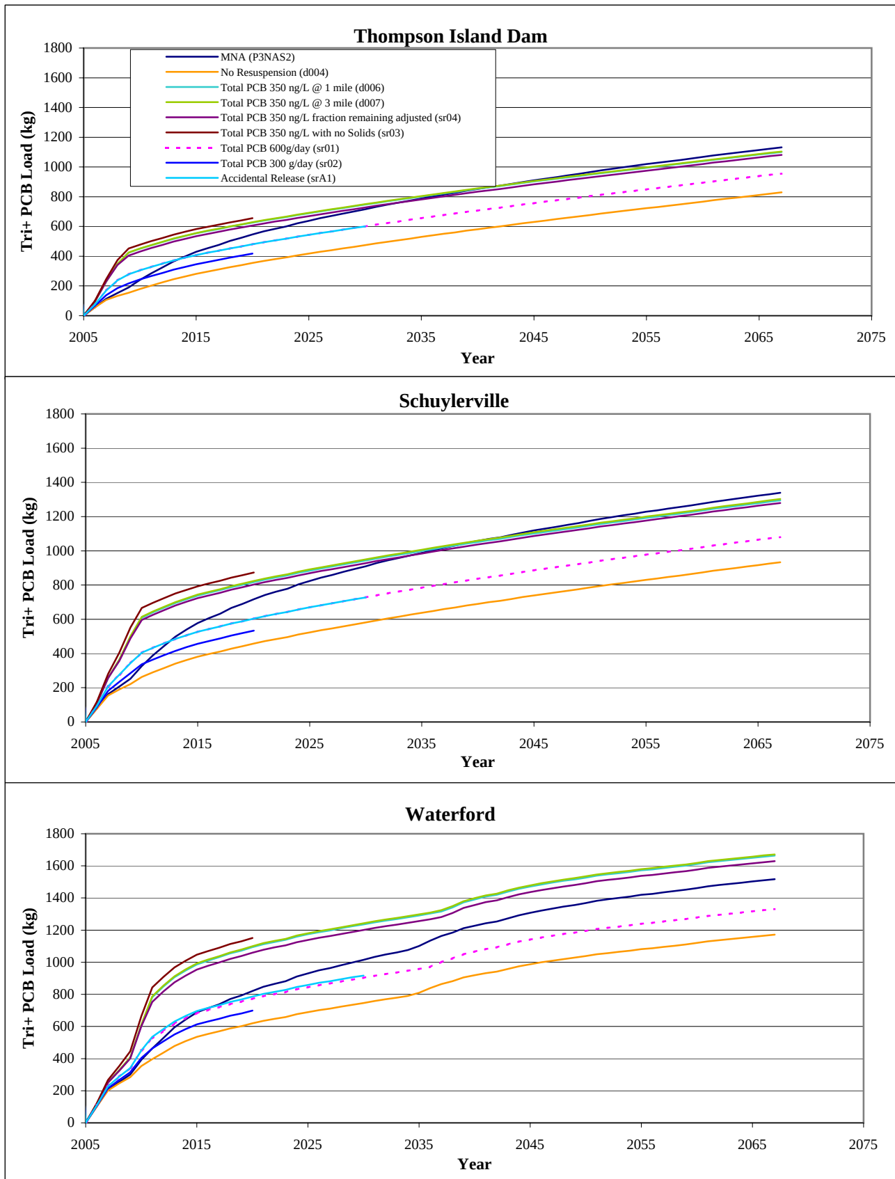
Figure 32 Tri+ PCB Cumulative Load for Different Dredging Scenarios
