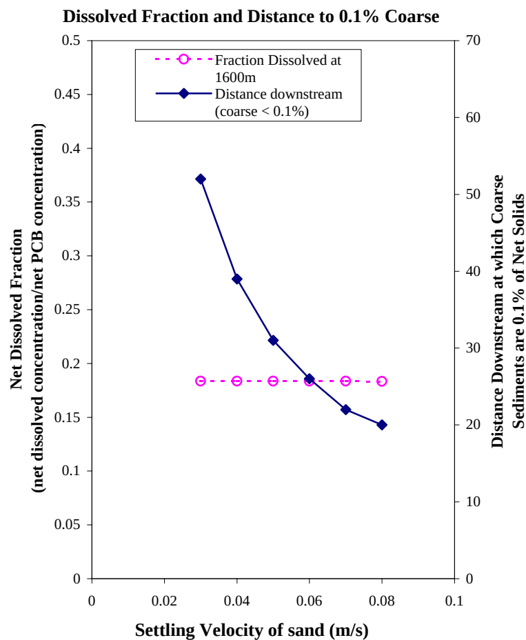
Figure 29 Net Dissolved PCB Fraction, Distance to Coarse < 0.1%, Net Total PCB Flux and Net TSS Flux at 1600 meters as Functions of Sand Settling Velocity for the TSS-Chem
