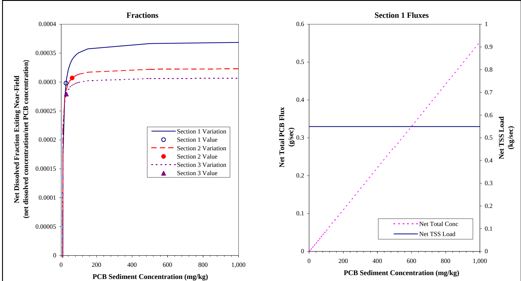
Figure 8 Net Dissolved PCB Fraction, Net Silt Fraction, Net Total PCB Flux and Net TSS Flux Exiting Near-Field as Functions of PCB Sediment Concentration for CSTR-Chem
