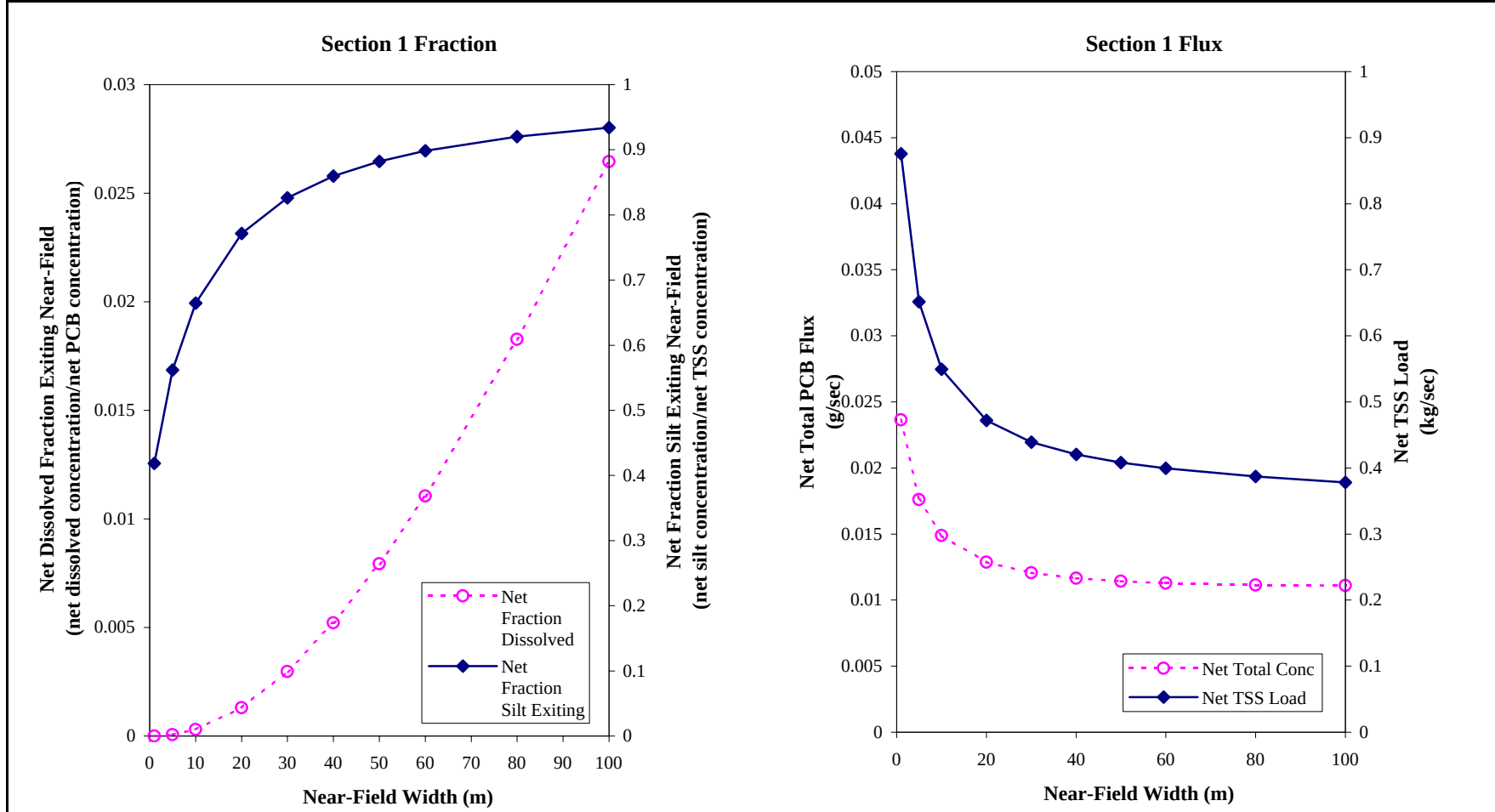
Figure 5 Net Dissolved PCB Fraction, Net Silt Fraction, Net Total PCB Flux and Net TSS Flux Exiting Near-Field as Functions of Near-Field Width for CSTR-Chem
