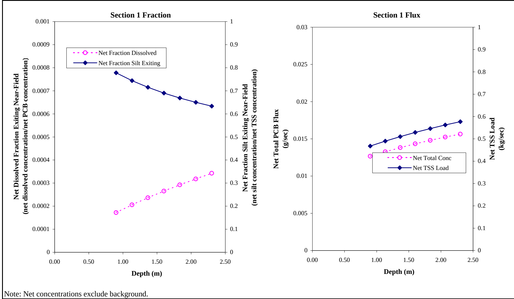
Figure 4 Net Dissolved PCB Fraction, Net Silt Fraction, Net Total PCB Flux and Net TSS Flux Exiting Near-Field as Functions of Depth for CSTR-Chem
