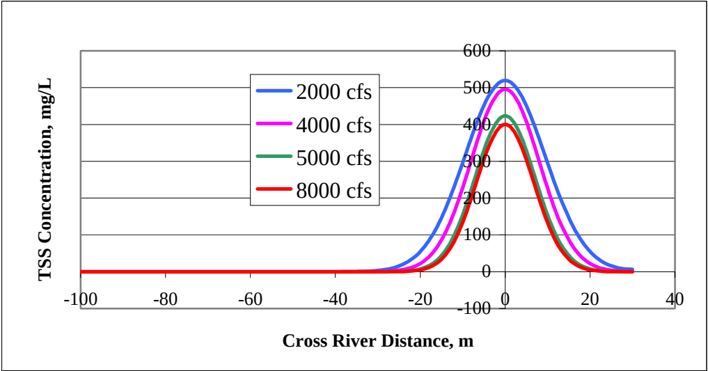
Figure 16 Estimated TSS Concentration at 300 m Downstream of the Dredge Head in Section 1 (PCB concentration at the far-field station is 500 ng/L)
