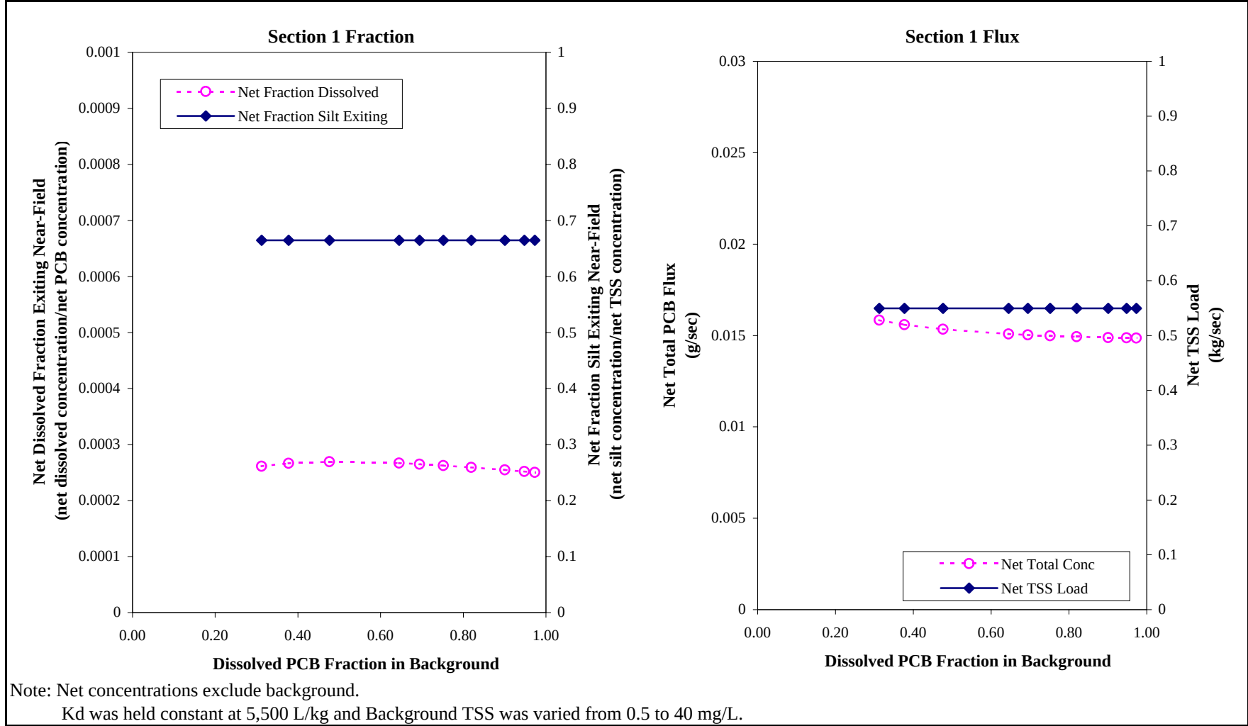
Figure 9 Net Dissolved PCB Fraction, Net Silt Fraction, Net Total PCB Flux and Net TSS Flux Exiting Near-Field as Functions of Dissolved PCB Fraction in the Background and TSS Background Concentrations for CSTR-Chem
