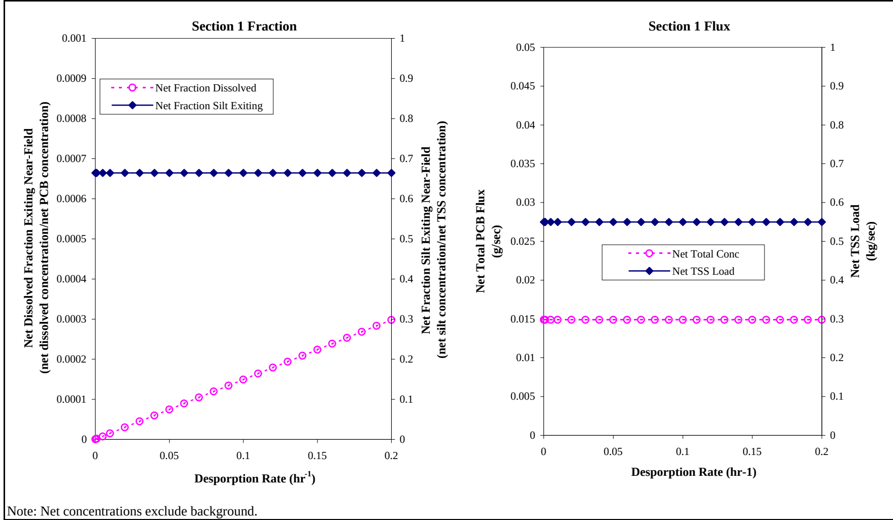
Figure 11 Net Dissolved PCB Fraction, Net Silt Fraction, Net Total PCB Flux and Net TSS Flux Exiting Near-Field as Functions of Desorption Rate for CSTR-Chem
