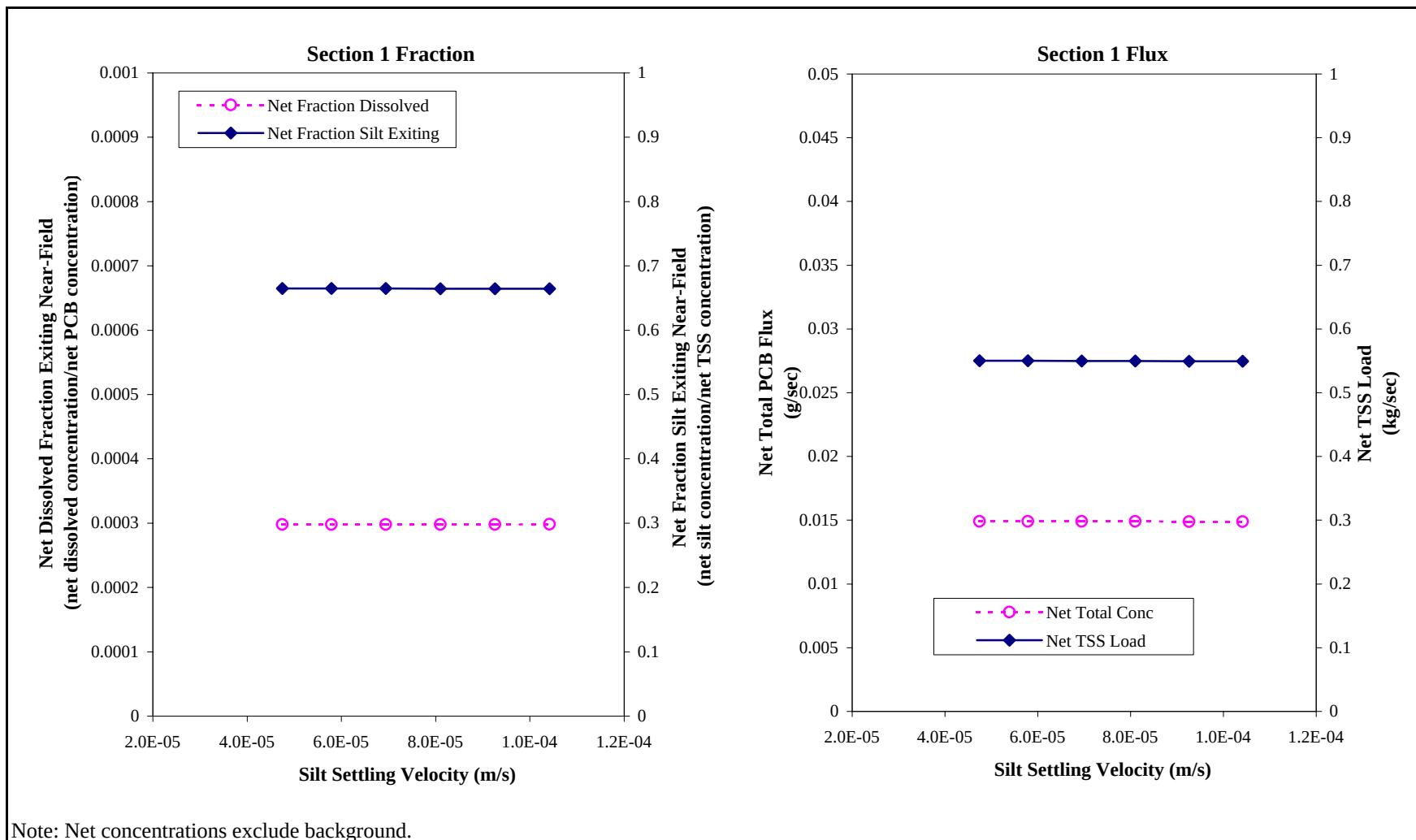
Figure 13 Net Dissolved PCB Fraction, Net Silt Fraction, Net Total PCB Flux and Net TSS Flux Exiting Near-Field as Functions of Silt Settling Velocity for CSTR-Chem
