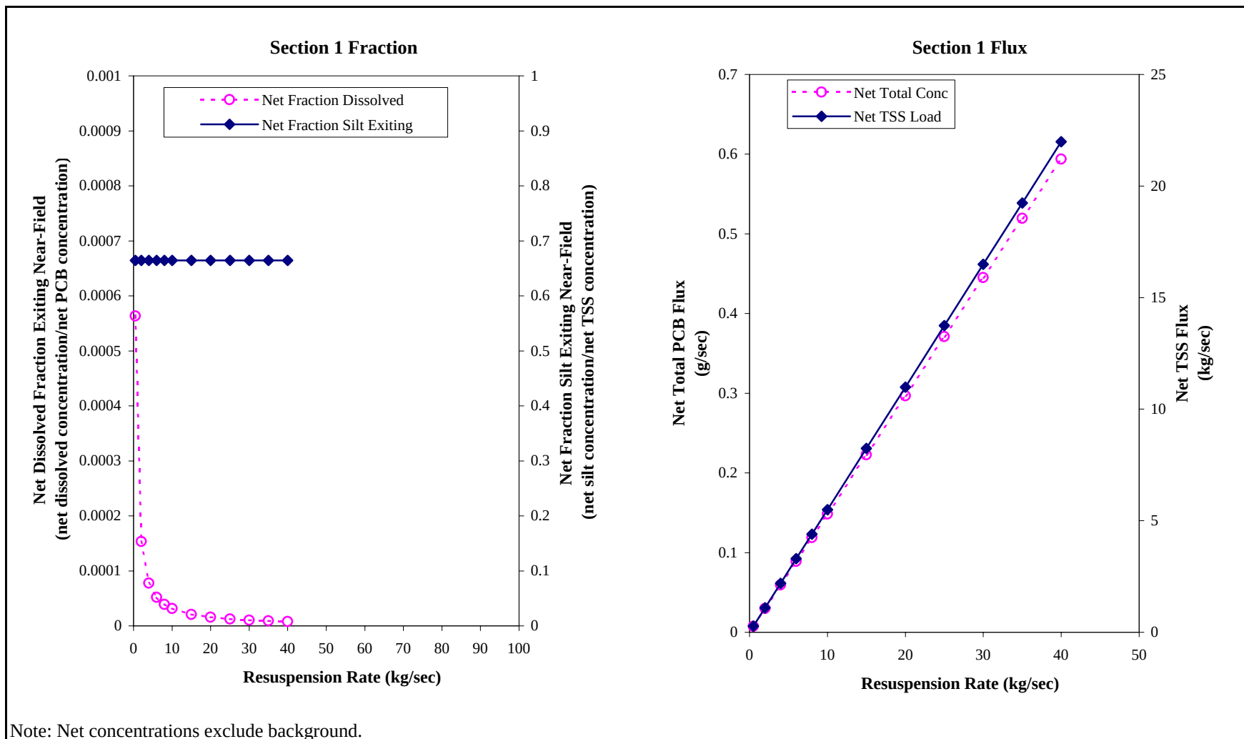
Figure 6 Net Dissolved PCB Fraction, Net Silt Fraction, Net Total PCB Flux and Net TSS Flux Exiting Near-Field as Functions of Resuspension Rate for CSTR-Chem
