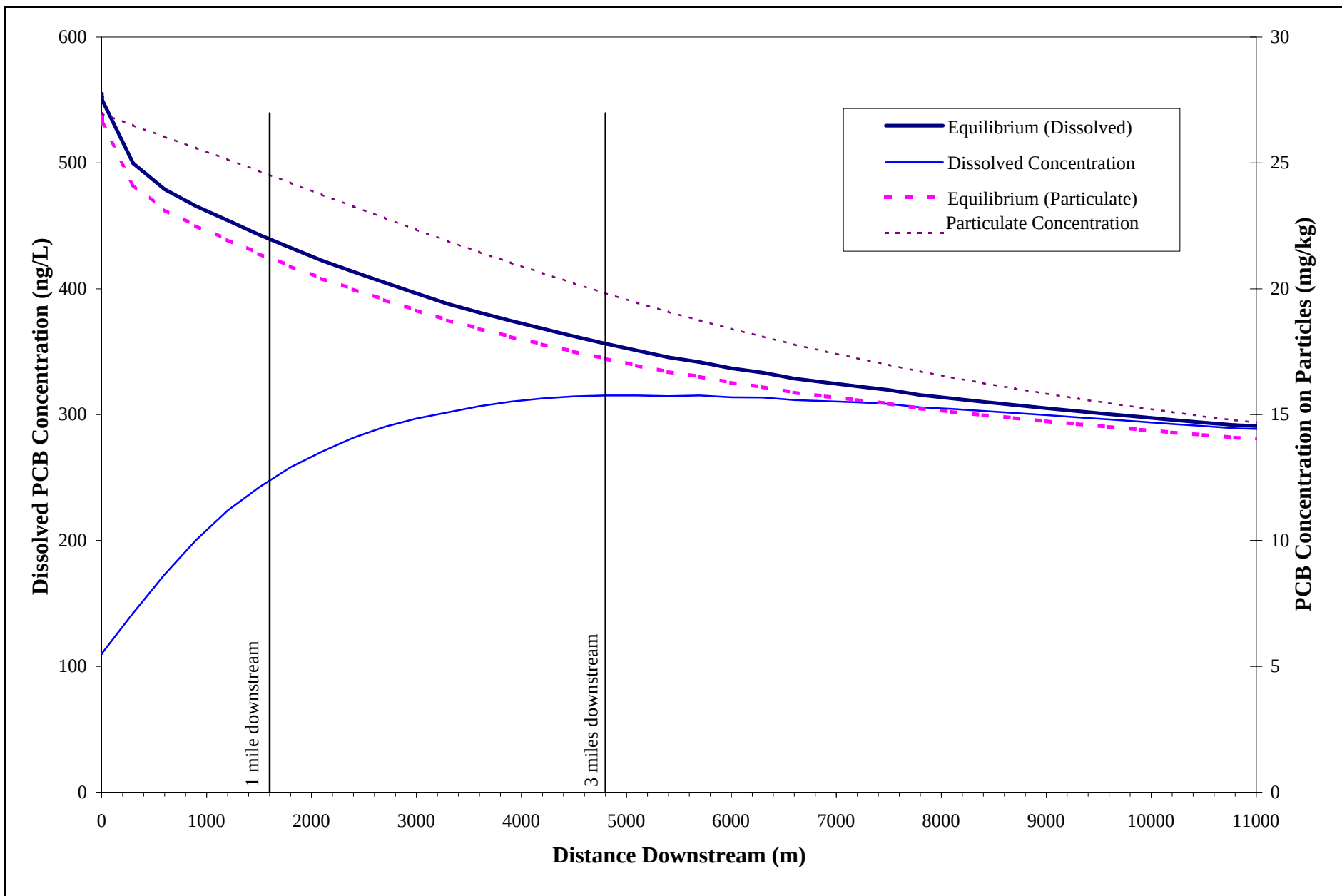
Figure 30 PCB Concentrations Downstream of Dredge for 350 ng/L scenario Section 1 at 1 mile and 3 miles
