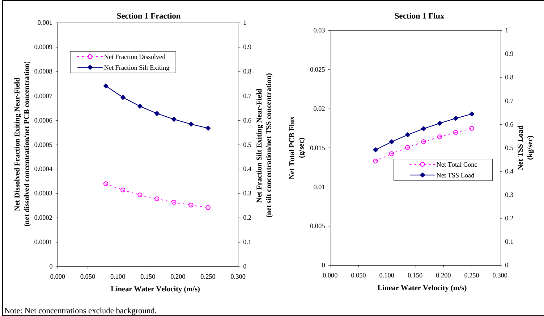
Figure 3 Net Dissolved PCB Fraction, Net Silt Fraction, Net Total PCB Flux and Net TSS Flux Exiting Near-Field as Functions of Velocity for CSTR-Chem
