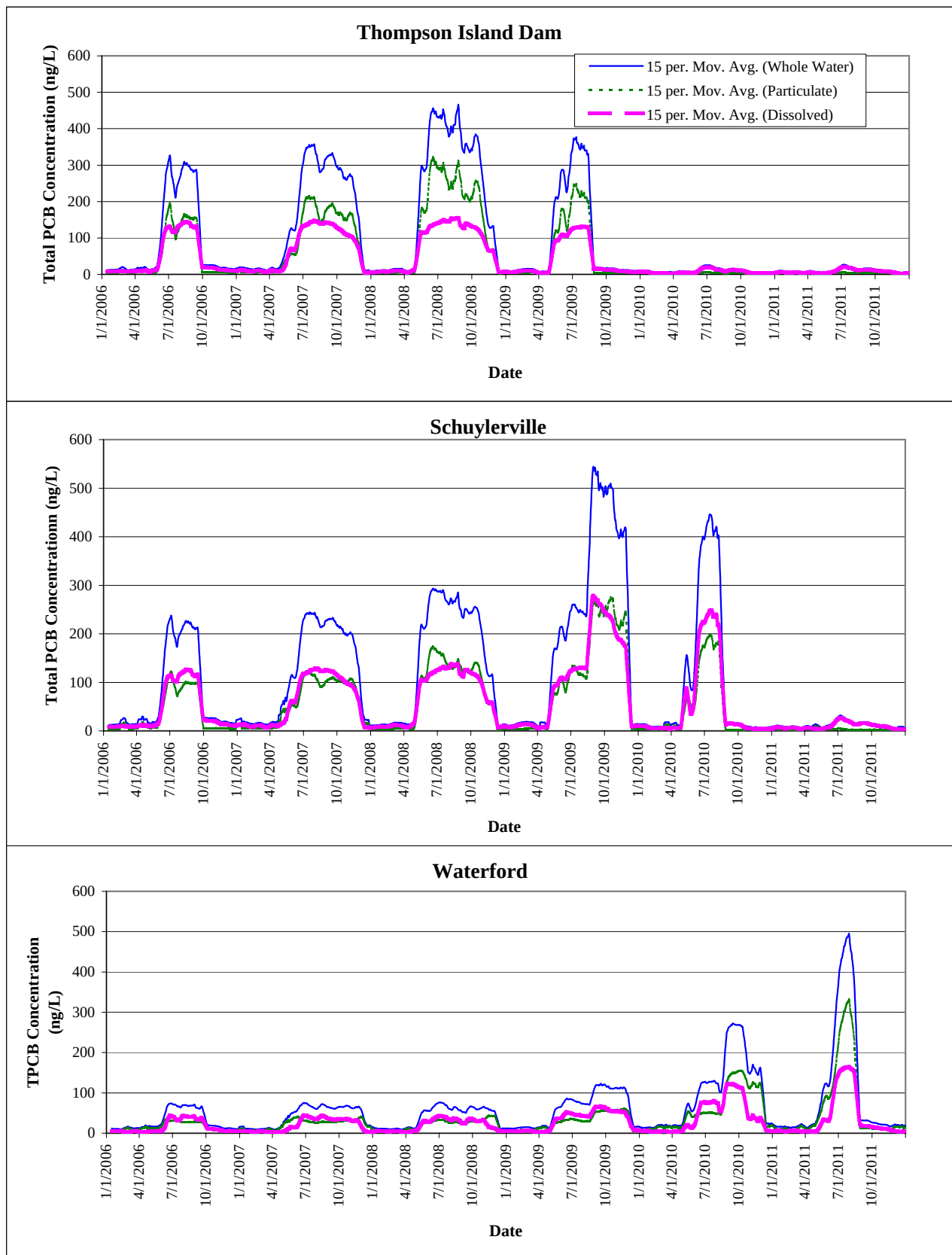
Figure 34 Whole Water, Particulate, and Dissolved Total PCB Concentrations for the 350 ng/L Dredging Scenario (sr04)
