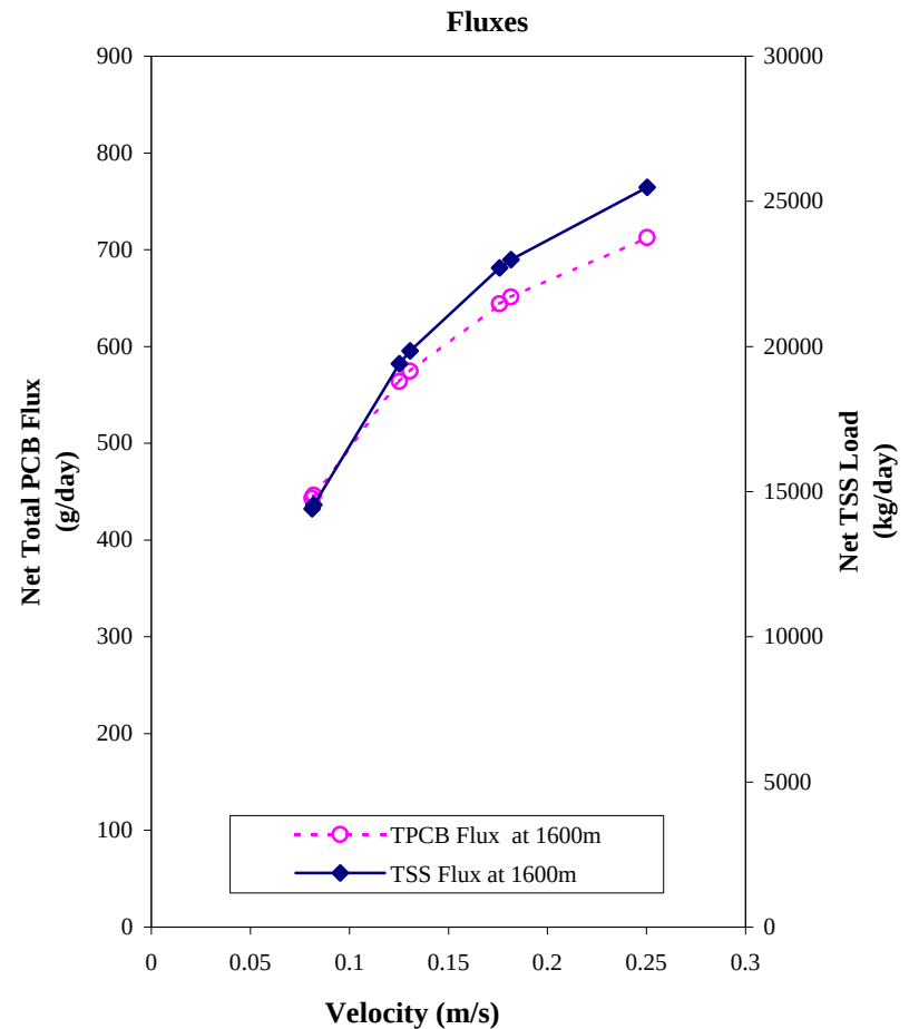
Figure 18 Net Dissolved PCB Fraction, Distance to Coarse < 0.1%, Net Total PCB Flux and Net TSS Flux at 1600 meters as Functions of Velocity for the TSS-Chem
