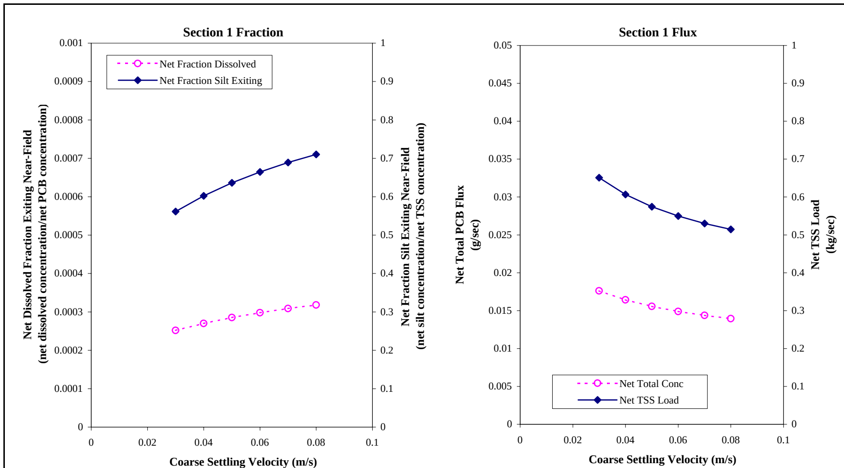
Figure 14 Net Dissolved PCB Fraction, Net Silt Fraction, Net Total PCB Flux and Net TSS Flux Exiting Near-Field as Functions of Coarse Settling Velocity for CSTR-Chem
