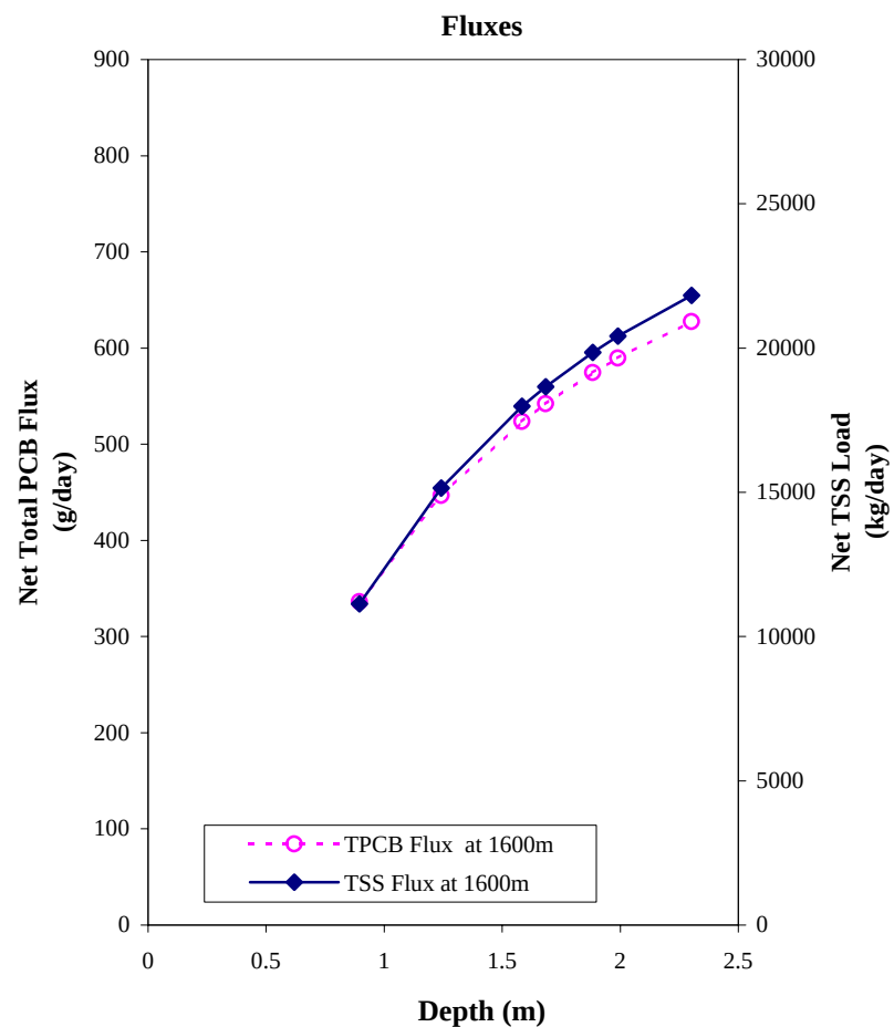
Figure 19 Net Dissolved PCB Fraction, Distance to Coarse < 0.1%, Net Total PCB Flux and Net TSS Flux at 1600 meters as Functions of Depth for the TSS-Chem
