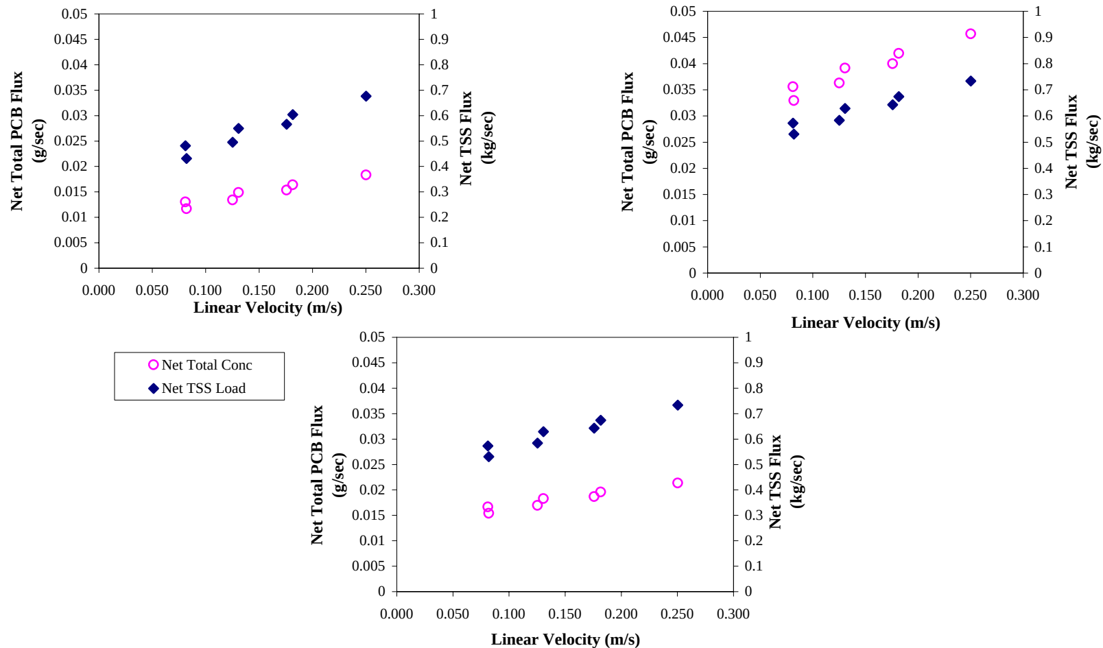
Figure 2 Sensitivity of Net Total PCB Flux and Net TSS Flux Exiting Near-Field with Variations in Linear Velocity and Depth for CSTR-Chem
