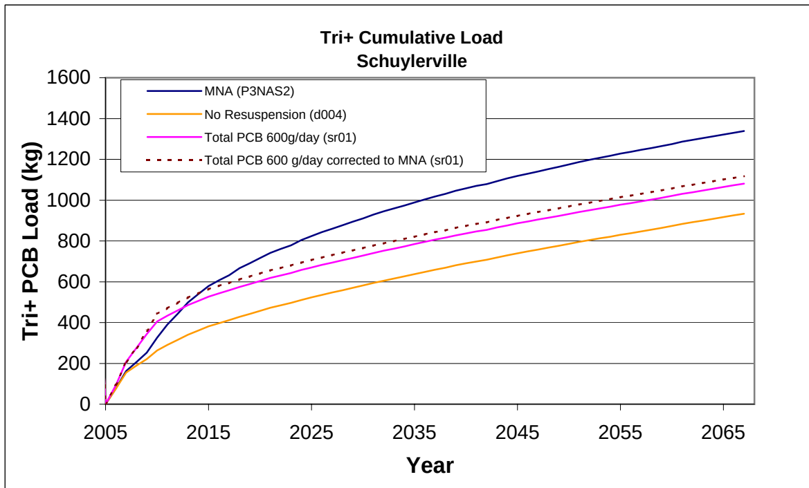
Figure 36 (Cont'd). Tri+ PCB and Total PCB Cumulative Load for 600 g/day (sr01) Scenario
