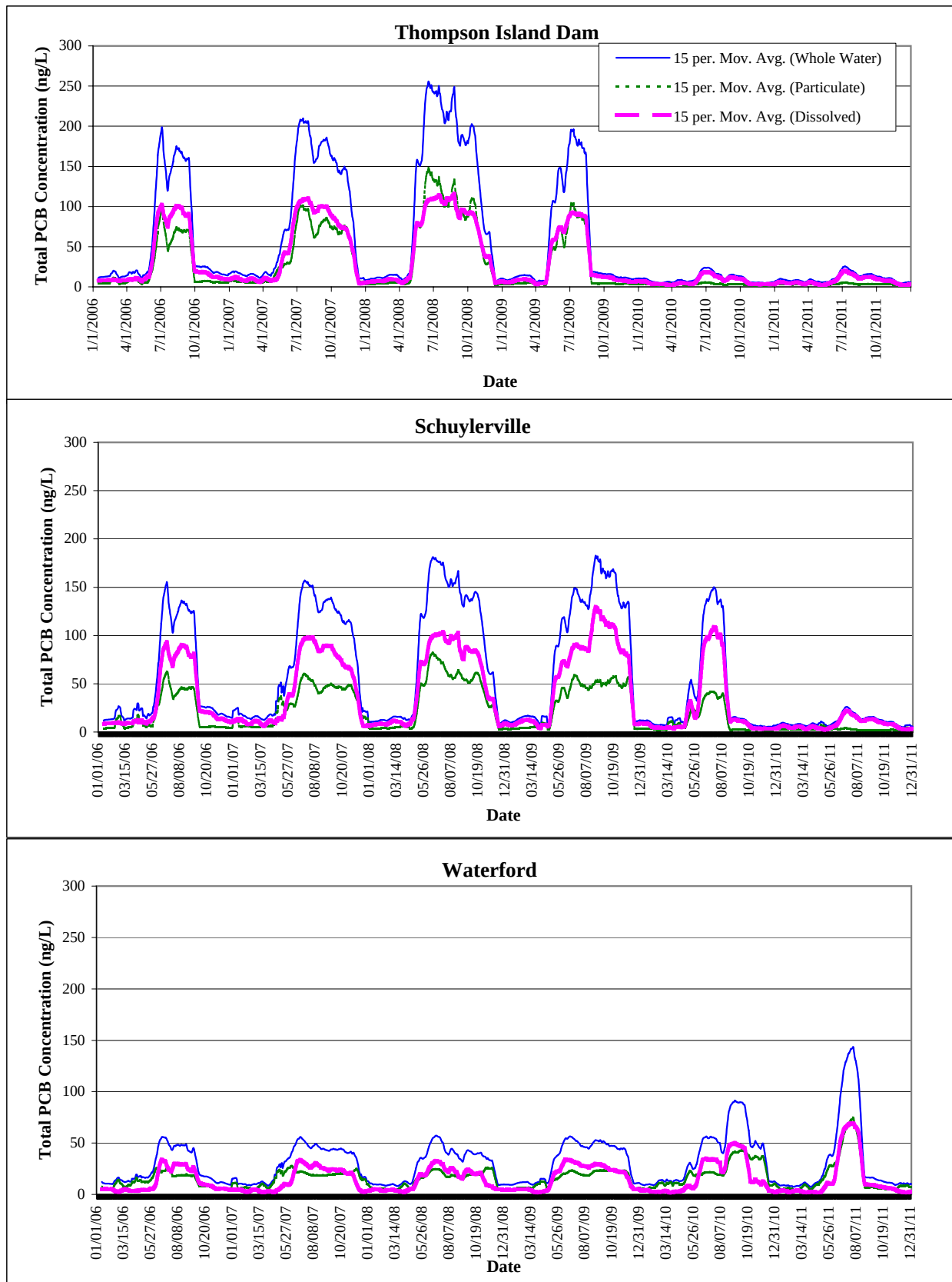
Figure 35 Whole Water, Particulate and Dissolved Total PCB Concentration for Concern Level - 600 g/day Total PCB Flux Dredging Scenario (sr01)
