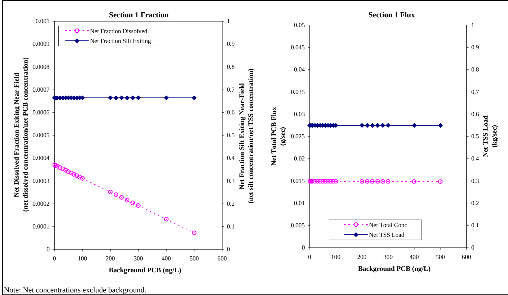
Figure 12 Net Dissolved PCB Fraction, Net Silt Fraction, Net Total PCB Flux and Net TSS Flux Exiting Near-Field as Functions of Background PCB Concentration for CSTR-Chem
