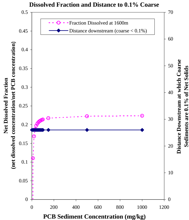
Figure 22 Net Dissolved PCB Fraction, Distance to Coarse < 0.1%, Net Total PCB Flux and Net TSS Flux at 1600 meters as Functions of Sediment PCB Concentration for the TSS-Chem
