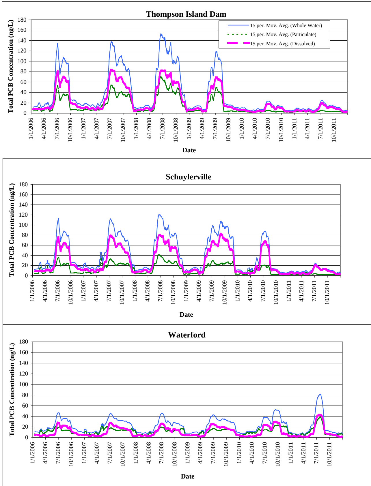
Figure 37 HUDTOX Forecast of Whole Water, Particulate, and Dissolved Total PCB Concentrations for Evaluation Level - 300 g/day Scenario
