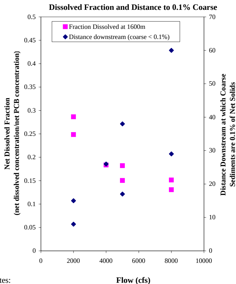
Figure 17 Net Dissolved PCB Fraction, Distance to Coarse < 0.1%, Net Total PCB Flux and Net TSS Flux at 1600 meters as Functions of Riverwide Volumetric Flow (Velocity-Depth Pairs) for the TSS-Chem
