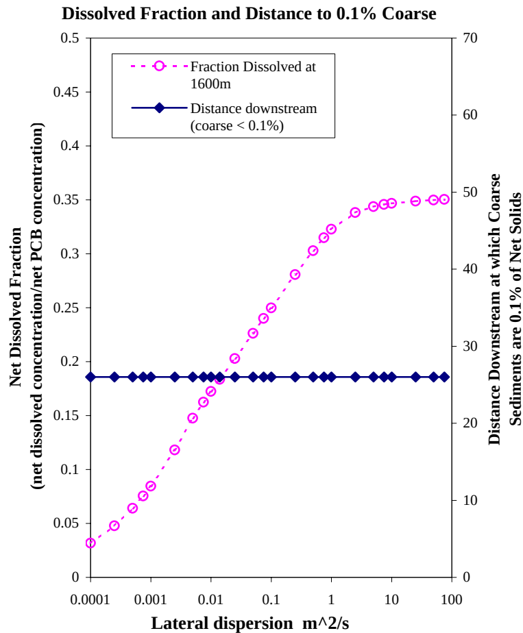
Figure 26 Net Dissolved PCB Fraction, Distance to Coarse < 0.1%, Net Total PCB Flux and Net TSS Flux at 1600 meters as Functions of Lateral Dispersion for the TSS-Chem
