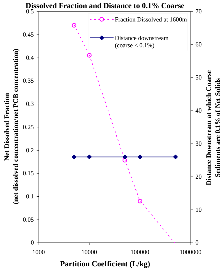
Figure 24 Net Dissolved PCB Fraction, Distance to Coarse < 0.1%, Net Total PCB Flux and Net TSS Flux at 1600 meters as Functions of K_d for the TSS-Chem
