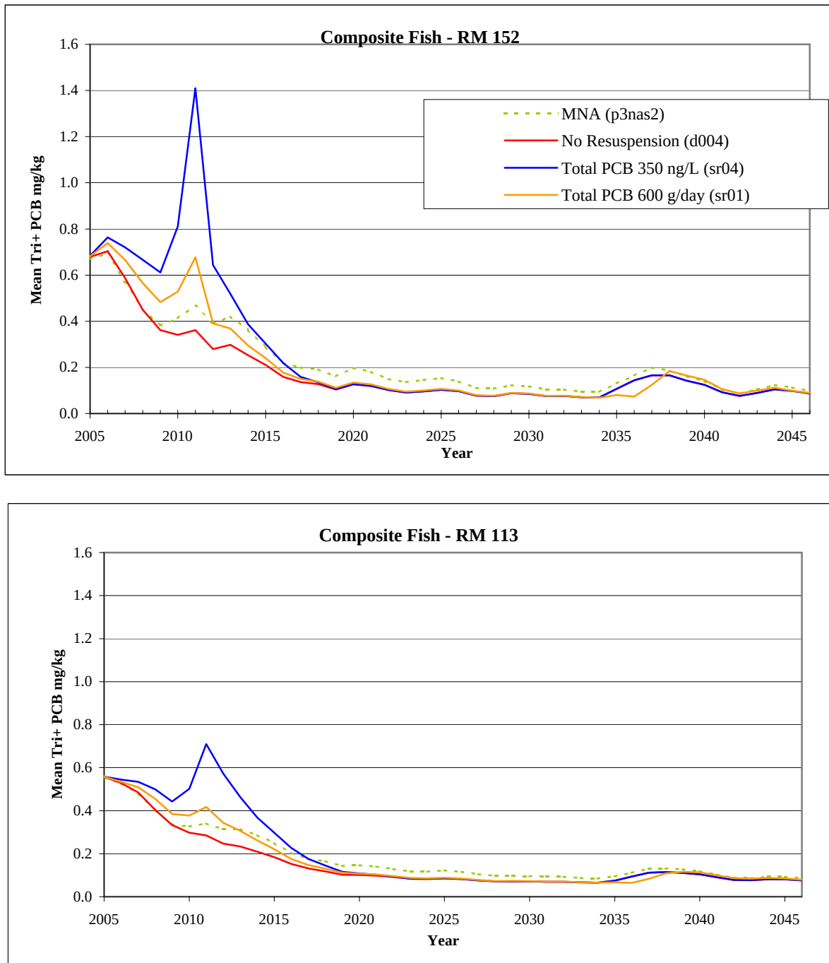
Figure 41 Composite Fish Tissue Concentrations for the Lower Hudson River
