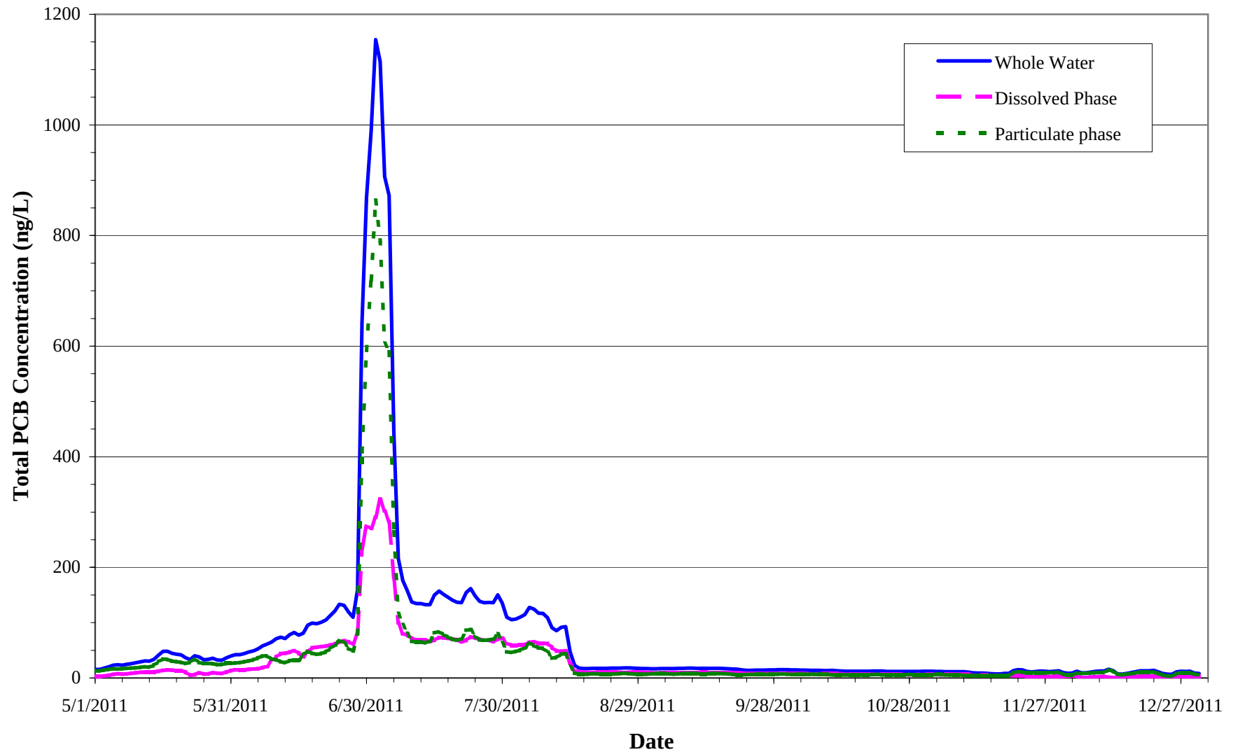
Figure 39 Total PCB Concentrations at Waterford for the Accidental Release Scenario
