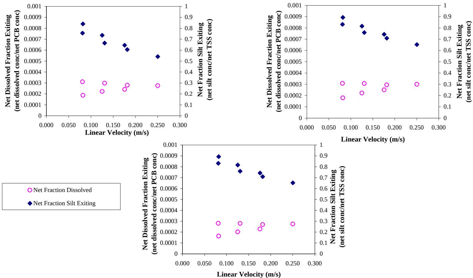
Figure 1 Sensitivity of Net Dissolved and Silt Fractions Exiting Near-Field with Variations in Linear Velocity and Depth for CSTR-Chem
