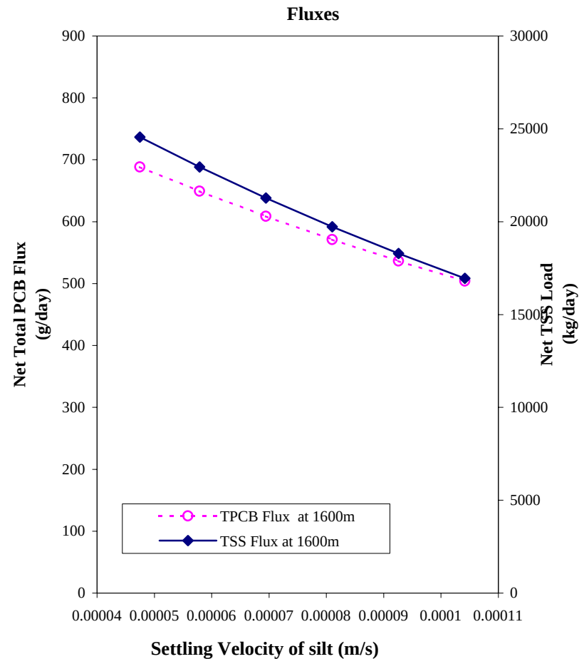
Figure 28 Net Dissolved PCB Fraction, Distance to Coarse < 0.1%, Net Total PCB Flux and Net TSS Flux at 1600 meters as Functions of Silt Settling Velocity for the TSS-Chem
