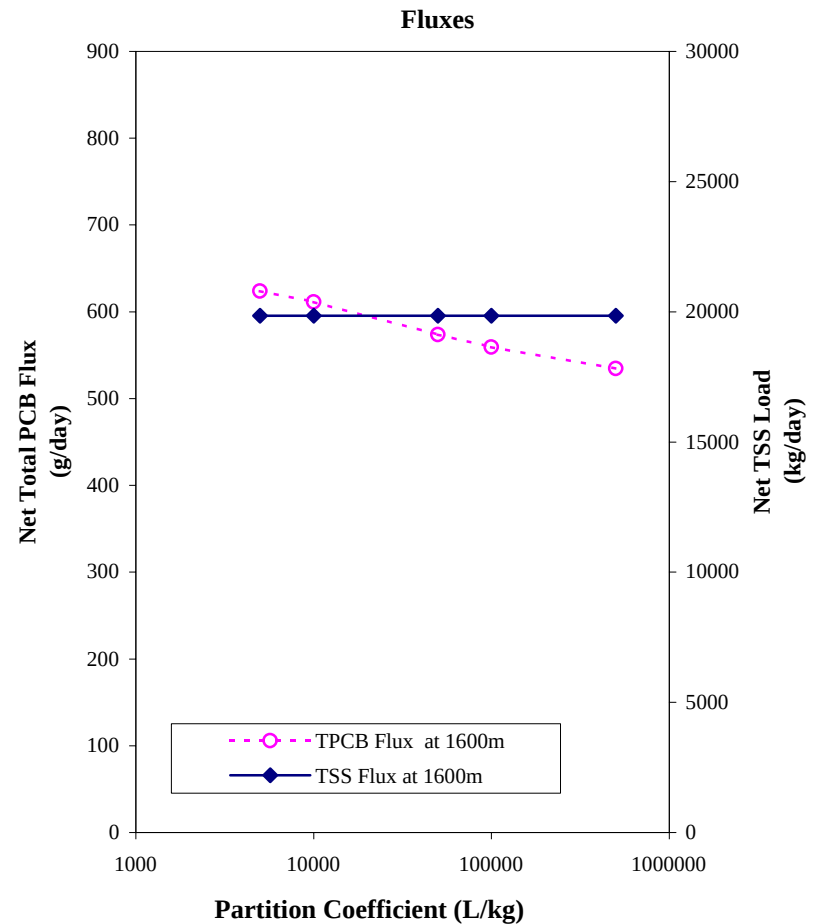
Figure 24 Net Dissolved PCB Fraction, Distance to Coarse < 0.1%, Net Total PCB Flux and Net TSS Flux at 1600 meters as Functions of K_d for the TSS-Chem
