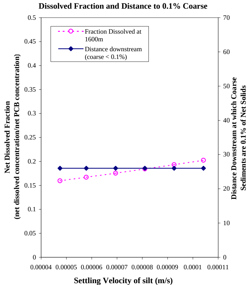
Figure 28 Net Dissolved PCB Fraction, Distance to Coarse < 0.1%, Net Total PCB Flux and Net TSS Flux at 1600 meters as Functions of Silt Settling Velocity for the TSS-Chem
