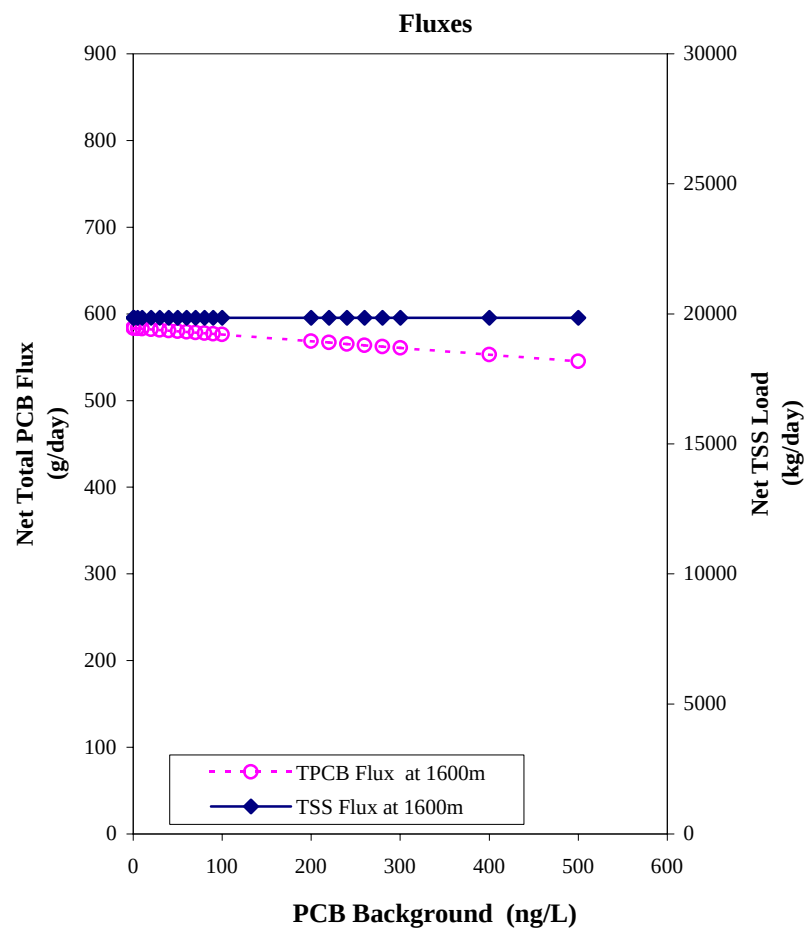
Figure 27 Net Dissolved PCB Fraction, Distance to Coarse < 0.1%, Net Total PCB Flux and Net TSS Flux at 1600 meters as Functions of PCB Background Concentration for the TSS-Chem
