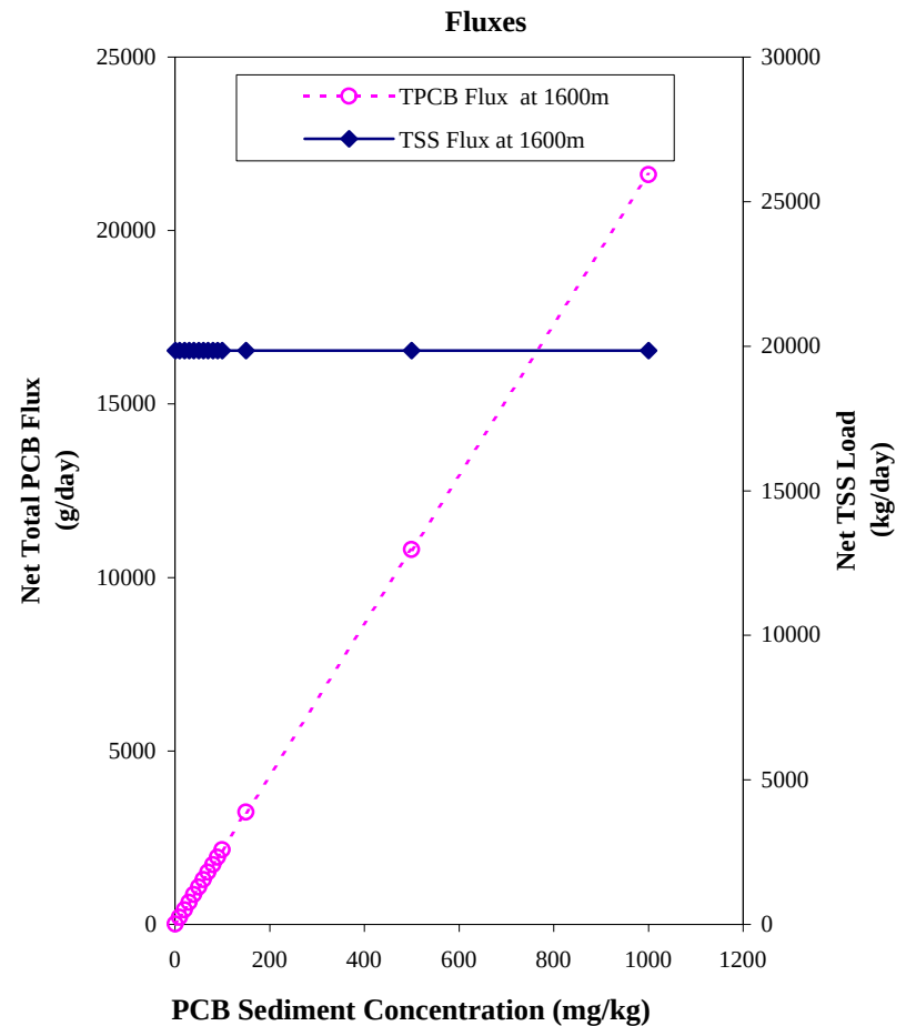
Figure 22 Net Dissolved PCB Fraction, Distance to Coarse < 0.1%, Net Total PCB Flux and Net TSS Flux at 1600 meters as Functions of Sediment PCB Concentration for the TSS-Chem
