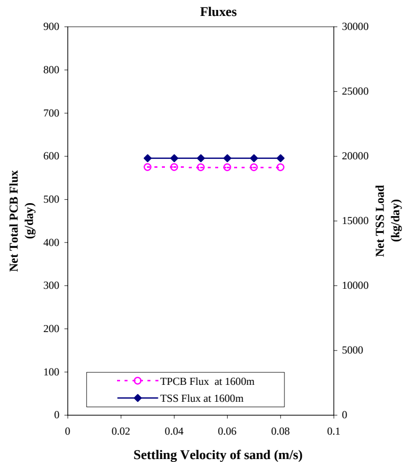
Figure 29 Net Dissolved PCB Fraction, Distance to Coarse < 0.1%, Net Total PCB Flux and Net TSS Flux at 1600 meters as Functions of Sand Settling Velocity for the TSS-Chem
