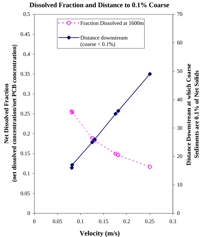
Figure 18 Net Dissolved PCB Fraction, Distance to Coarse < 0.1%, Net Total PCB Flux and Net TSS Flux at 1600 meters as Functions of Velocity for the TSS-Chem
