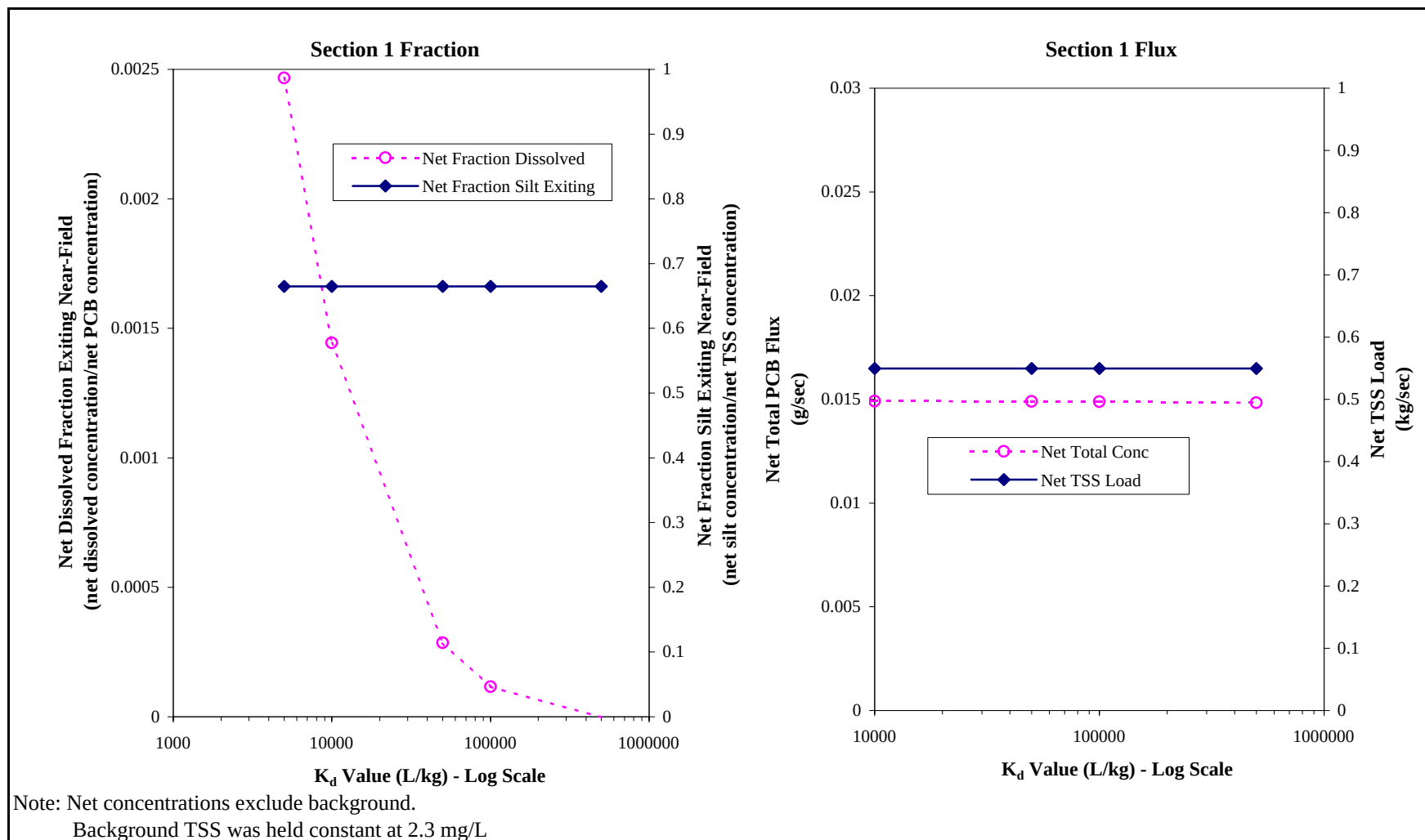
Figure 10 Net Dissolved PCB Fraction, Net Silt Fraction, Net Total PCB Flux and Net TSS Flux Exiting Near-Field as Functions of Dissolved PCB Fraction in the Background and K_d Value for CSTR-Chem
