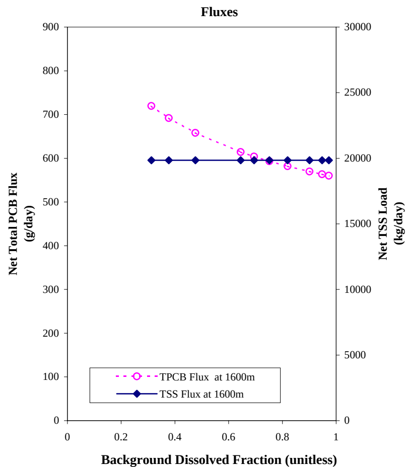
Figure 23 Net Dissolved PCB Fraction, Distance to Coarse < 0.1%, Net Total PCB Flux and Net TSS Flux at 1600 meters as Functions of TSS Background and PCB Dissolved Fraction ( K_d = 55,000 ) for the TSS-Chem
