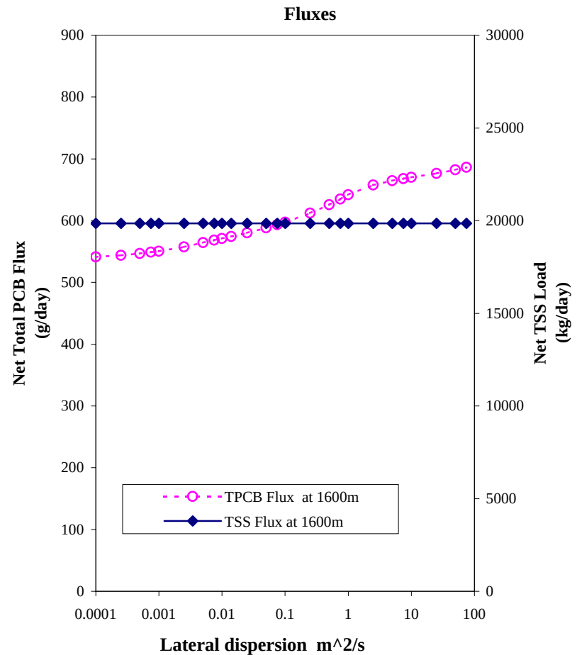
Figure 26 Net Dissolved PCB Fraction, Distance to Coarse < 0.1%, Net Total PCB Flux and Net TSS Flux at 1600 meters as Functions of Lateral Dispersion for the TSS-Chem
