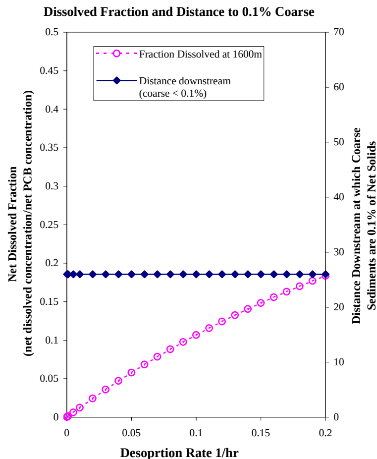
Figure 25 Net Dissolved PCB Fraction, Distance to Coarse < 0.1%, Net Total PCB Flux and Net TSS Flux at 1600 meters as Functions of Desorption Rate for the TSS-Chem
