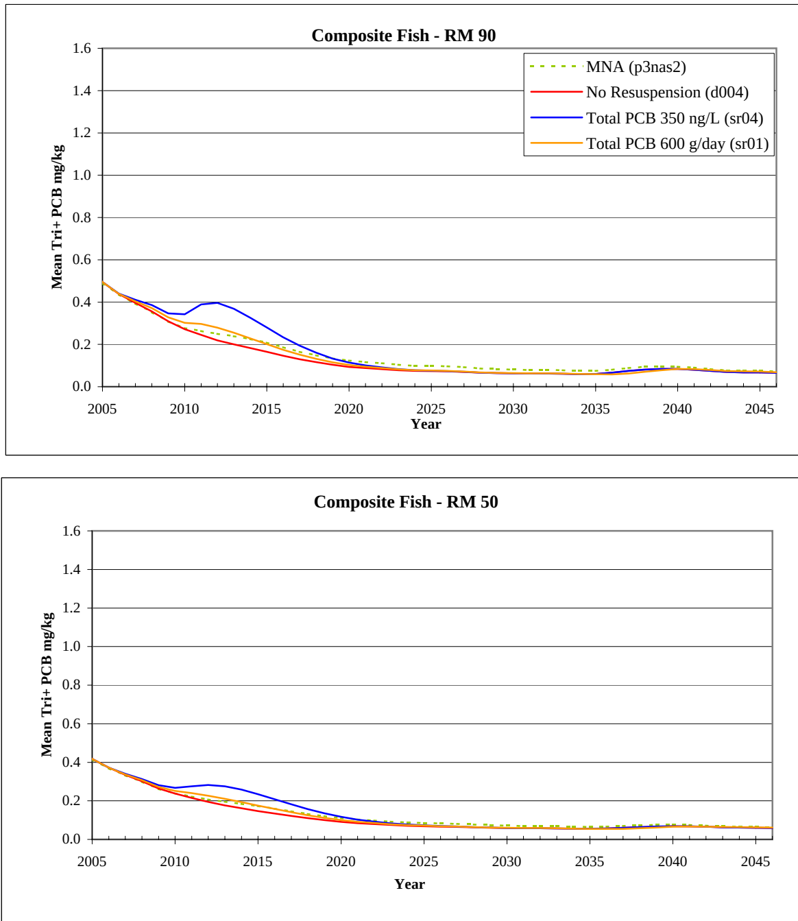
Figure 41 (Cont.) Composite Fish Tissue Concentrations for the Lower Hudson River
