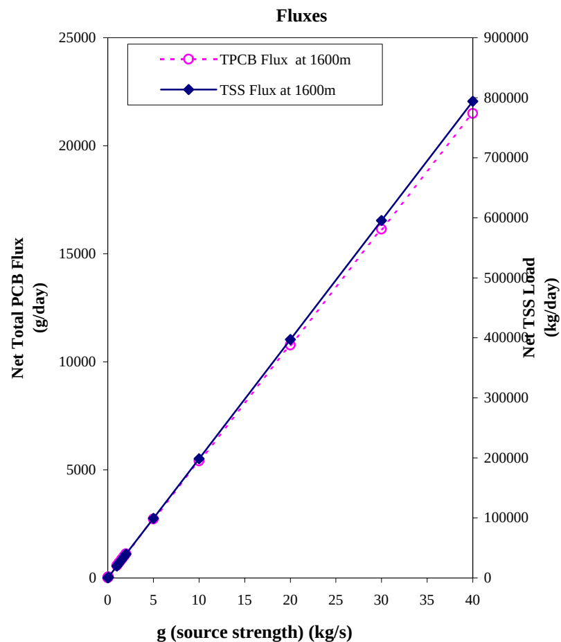
Figure 20 Net Dissolved PCB Fraction, Distance to Coarse < 0.1%, Net Total PCB Flux and Net TSS Flux at 1600 meters as Functions of Source Strength for the TSS-Chem
