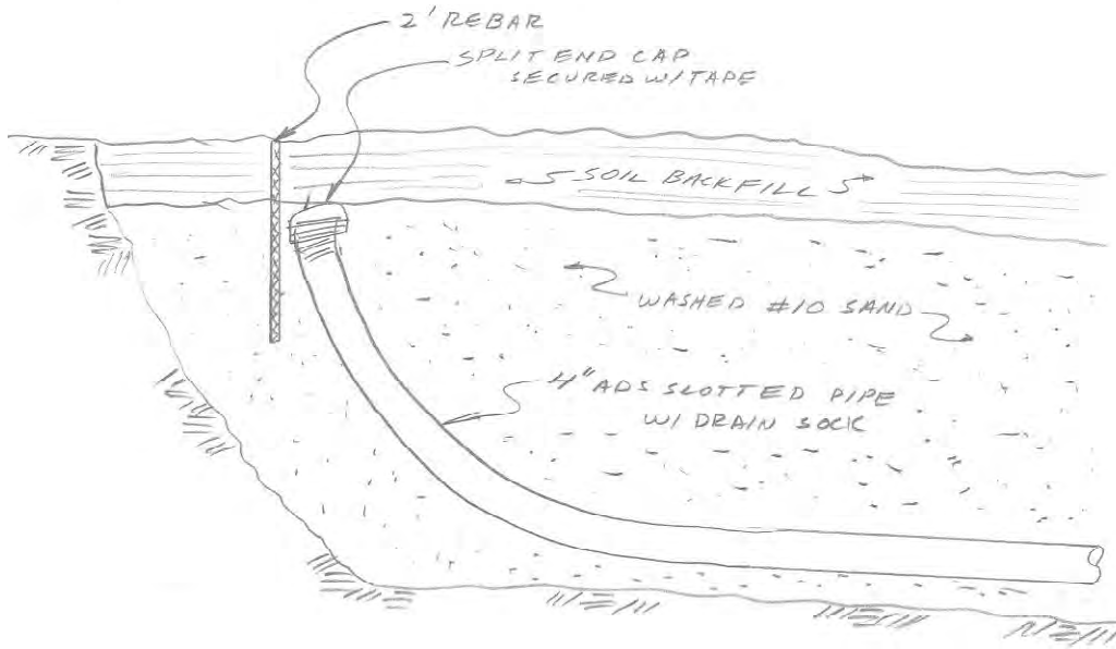
Section C-C Thru end of toe drain
