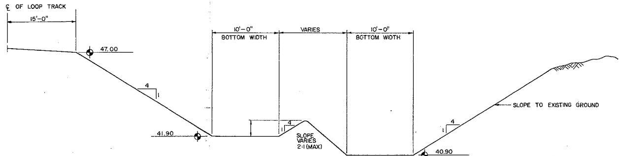
OUTFALL AND DRAINAGE DITCHES SECTION D-C-12
