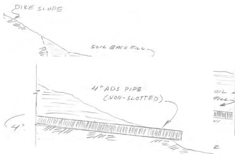
Section B-B Thru Outlet Pipe (NTS)
