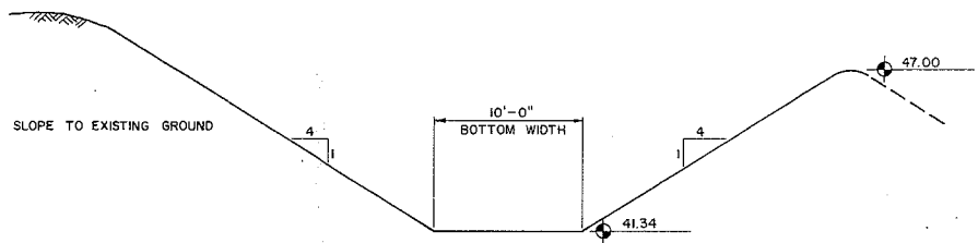
OUTFALL DITCH FROM TREATMENT FACILITY SECTION B-C-12
