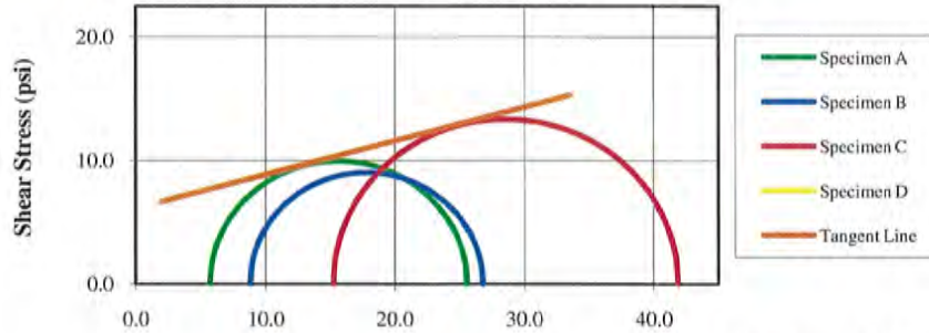
Effective Stress at Maximum Deviator Stress Criterion
