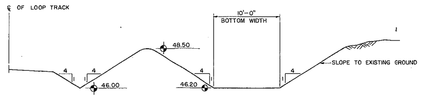
SETTLING BASIN OVERFLOW SECTION E-C-12
