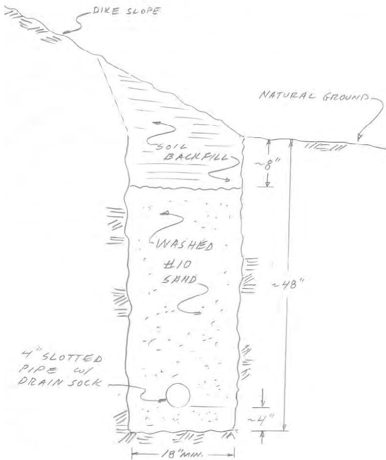
Section A-A Thru Toe Drain (NTS)
