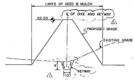
ASH POND DIKE SECTION G-C-12
