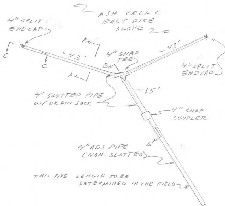
Toe Drain Pipe Layout (NTS)
