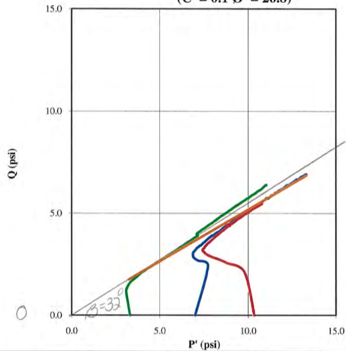
Stress Paths (Effective) ( C' = 0.1 \phi' = 26.8 )
