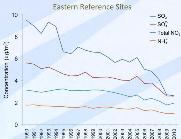
Trend in Annual Mean \text{SO}_2 Concentrations ( \mu\text{g}/\text{m}^3 )
