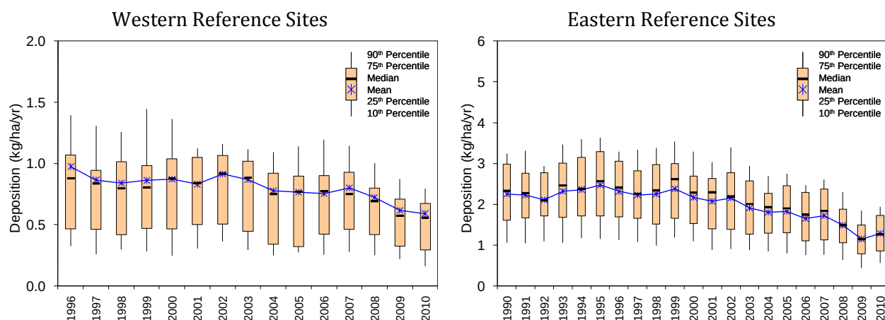
Figure 3-11 Trend in Dry Nitrogen Deposition (kg/ha/yr)
