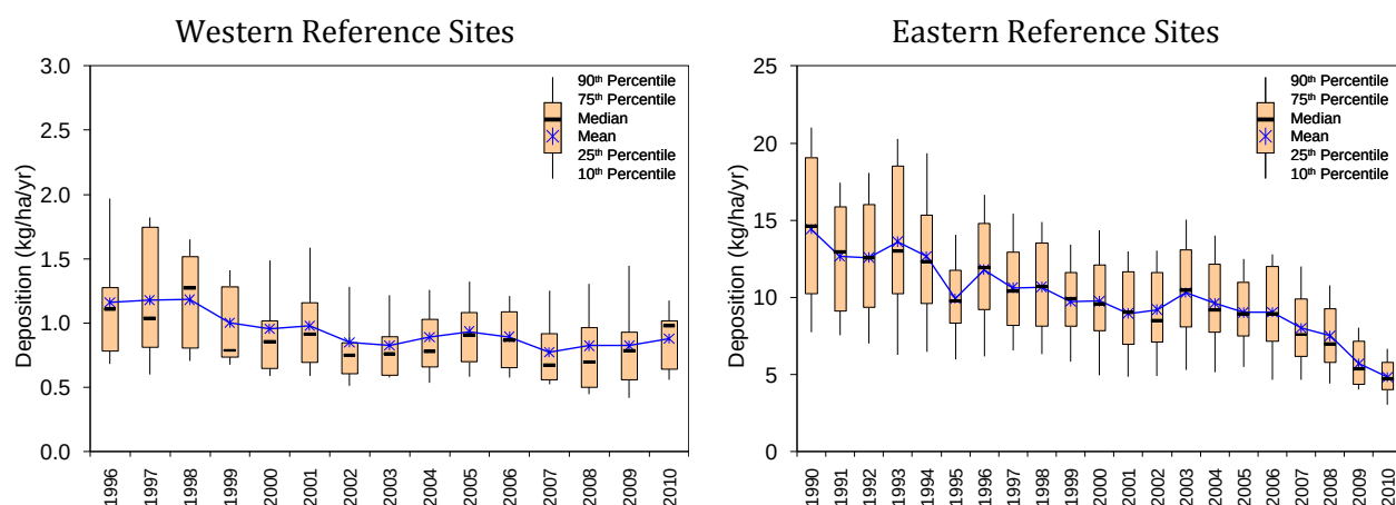
Figure 3-7 Trend in Total Sulfur Deposition (kg/ha/yr)
