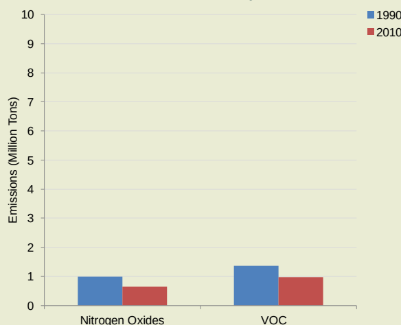
Figure 1d Canadian \text{NO}_x and VOCs PEMA Emissions and Projections
