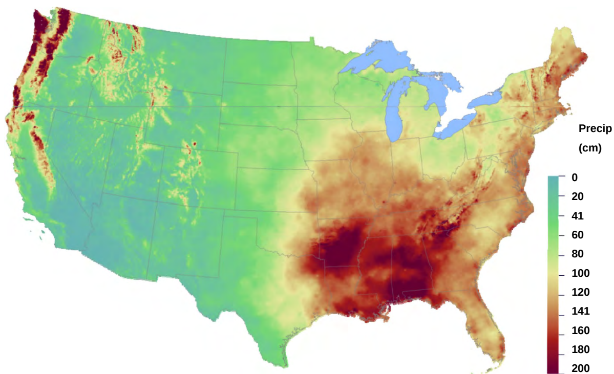
Figure 3-2 Resulting PRISM Precipitation Grid for 2009
