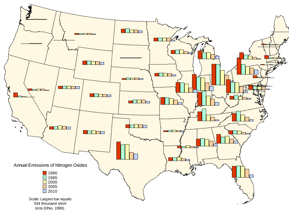
Figure 1-7 Annual NO x Emissions (for CAIR and ARP Sources)
