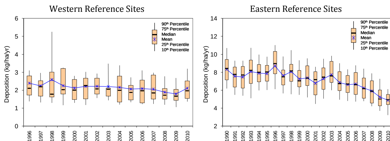
Figure 3-12 Trend in Total Nitrogen Deposition (kg/ha/yr)
