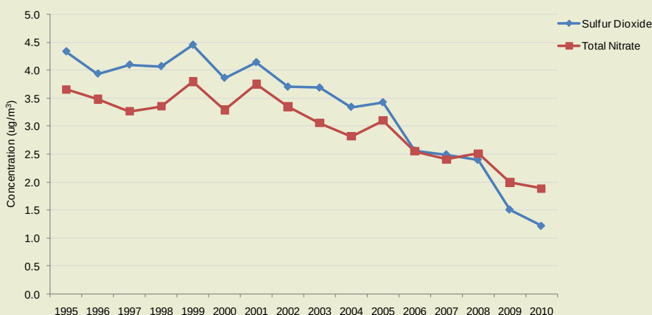
Figure 1f Trends in Annual \text{SO}_2 and Total Nitrate Concentrations for Egbert, ON
