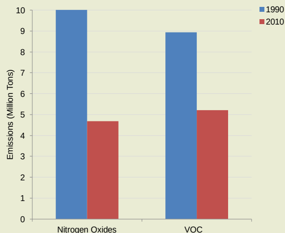
Figure 1e U.S. \text{NO}_x and VOCs PEMA Emissions
