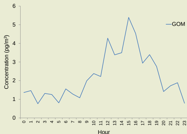
Figure 2b Average Diurnal Cycle of and GOM for 2010
