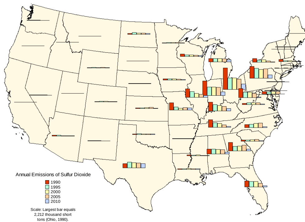
Figure 1-6 Annual SO 2 Emissions (for CAIR and ARP Sources)
