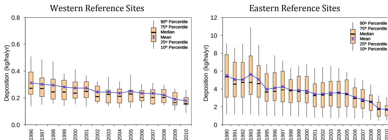
Figure 3-6 Trend in Dry Sulfur Deposition (kg/ha/yr)
