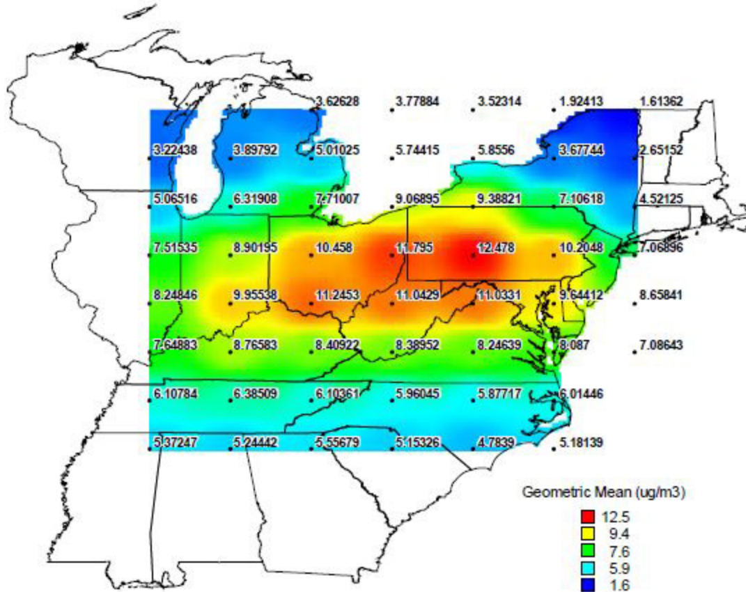
Figure 1: Kriging Estimated SO 2 Concentration (ug/m 3 ), 4th Quarter 2000
