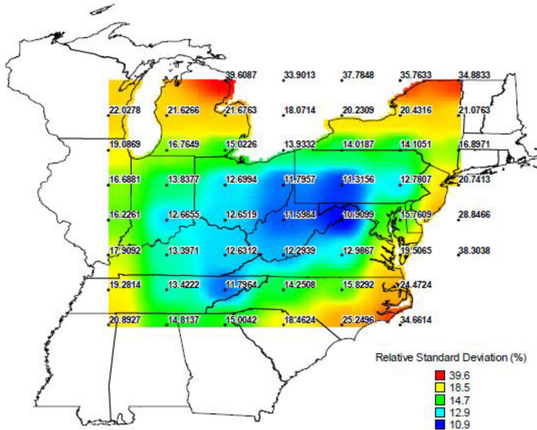
Figure 2: Kriging Relative Standard Deviation (%), SO 2 , 4th Quarter 2000
