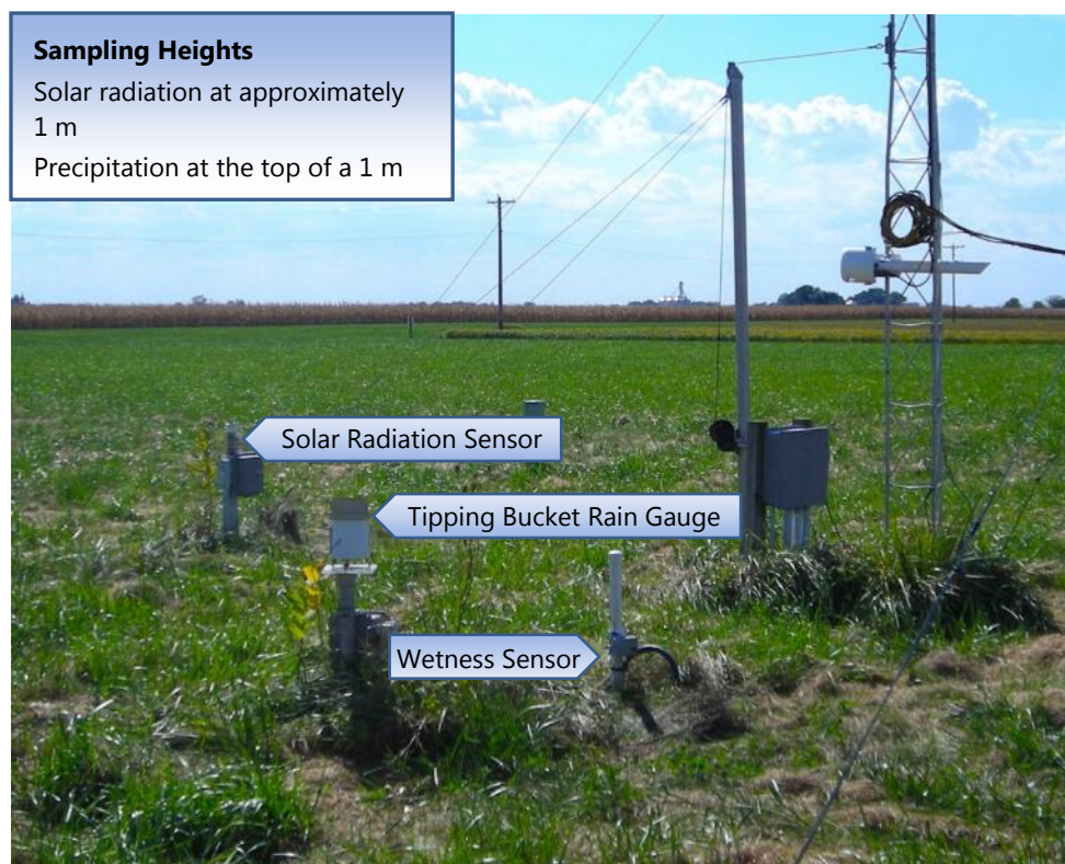
Figure 1-3. Typical CASTNET Ground-Level Sensors
