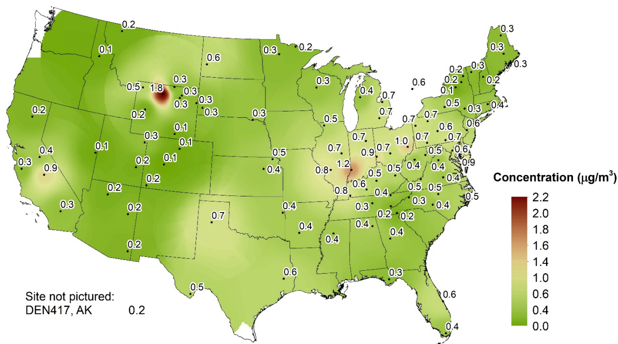
Figure 1-7. Annual Mean SO 2 Concentrations ( \mu\text{g}/\text{m}^3 ) for 2018
