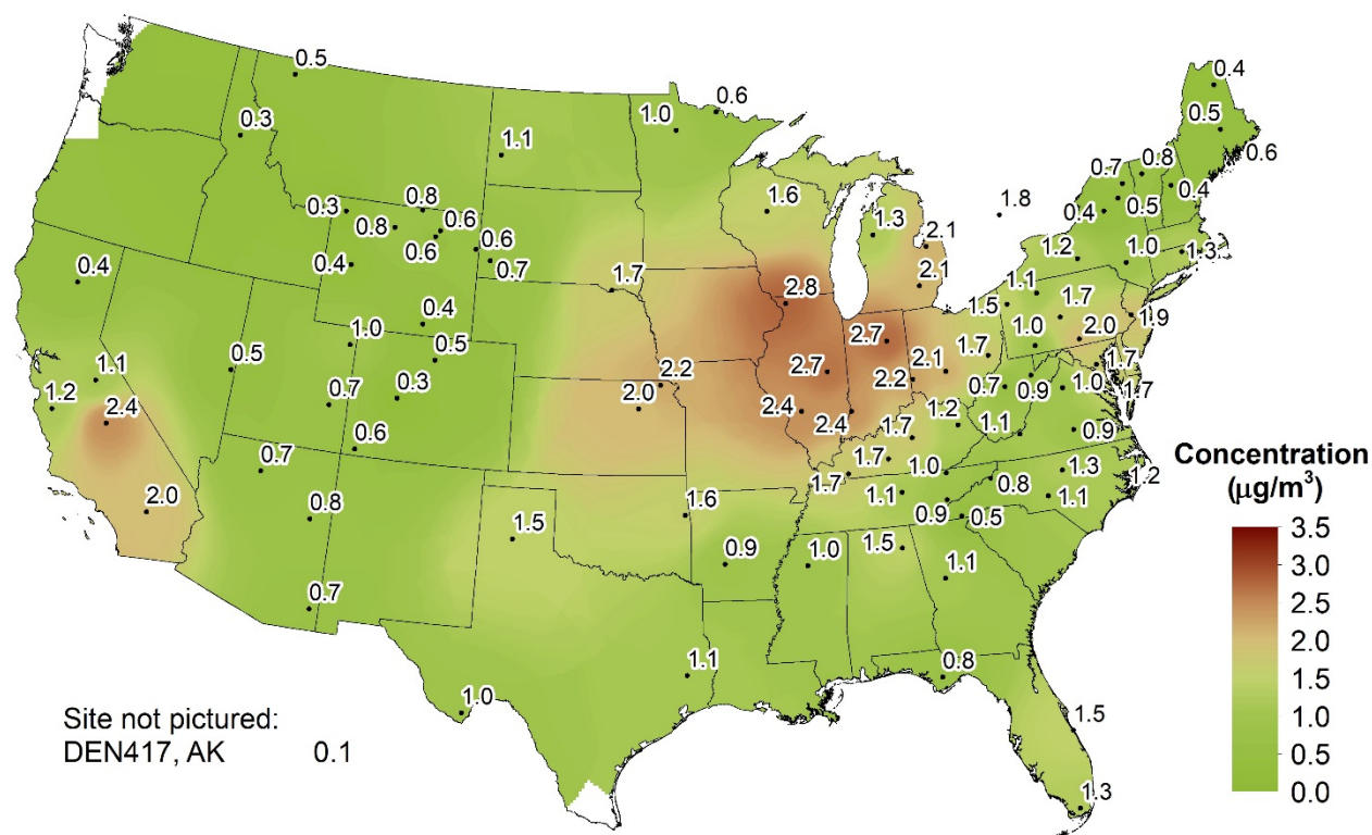
Figure 1-8. Annual Mean Total Nitrate Concentrations ( \mu\text{g}/\text{m}^3 ) for 2018
