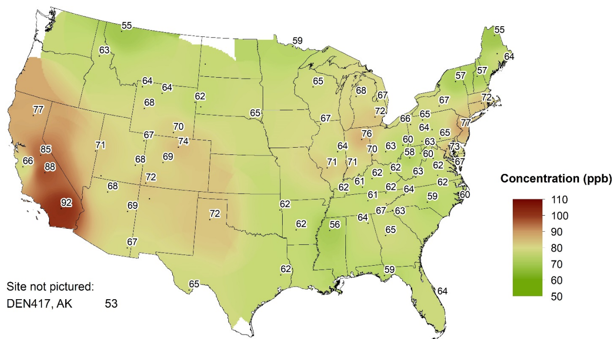
Figure 1-9. Fourth Highest DM8A O 3 Concentrations (ppb) for 2018
