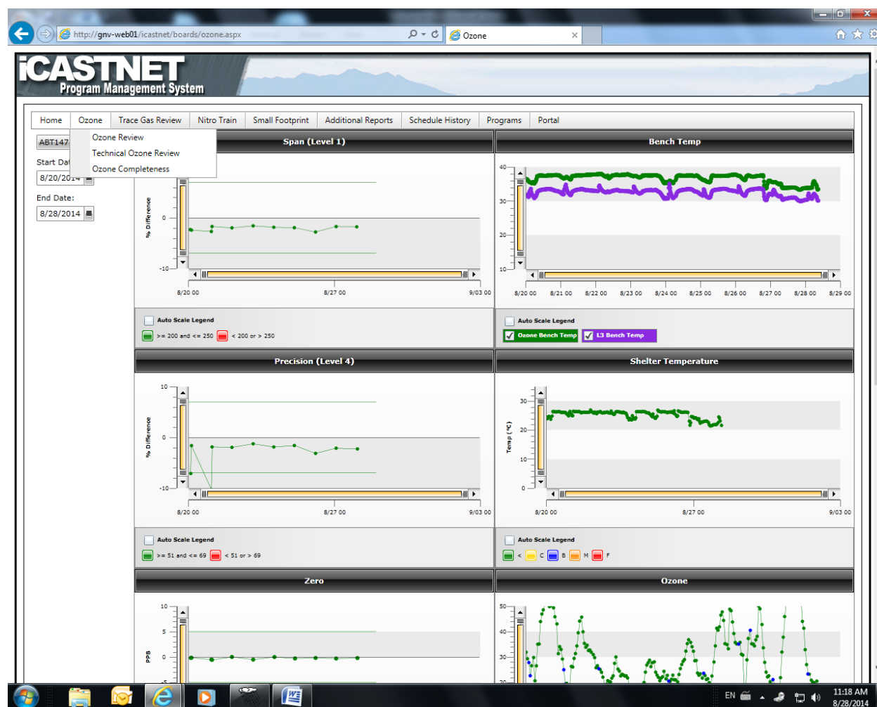
Figure 2-15. Example Daily O 3 Precision and Span Checks
