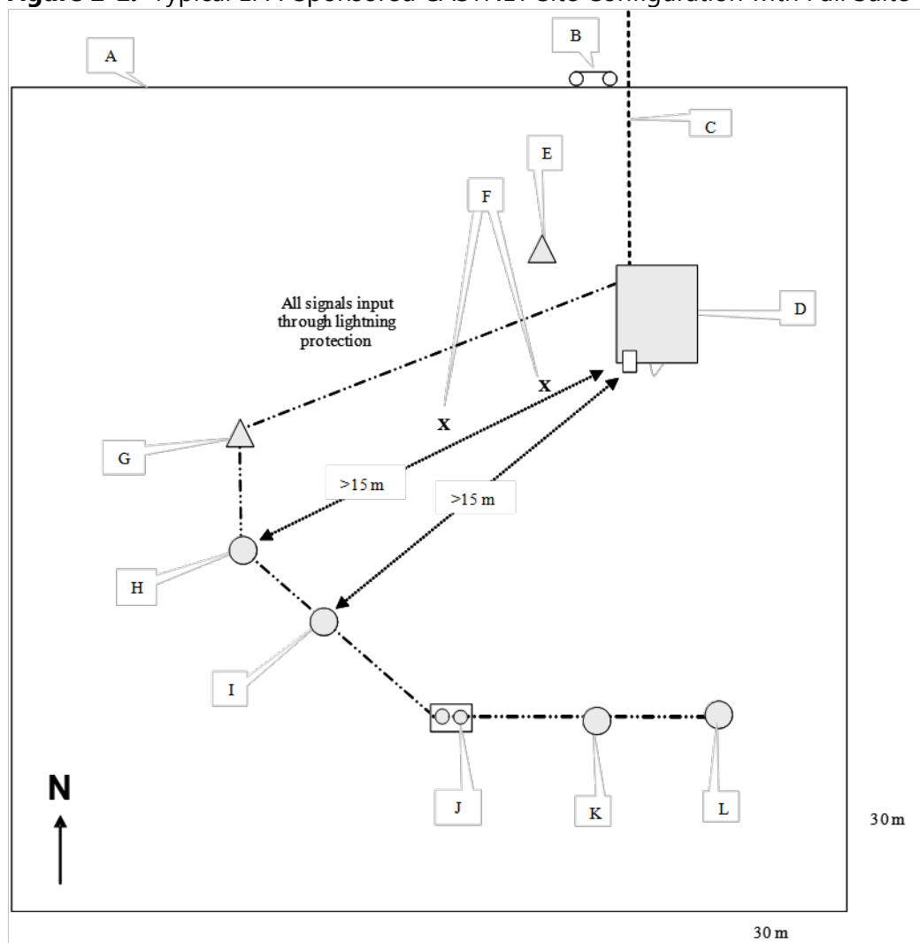
Figure 2-1. Typical EPA-Sponsored CASTNET Site Configuration with Full Suite
