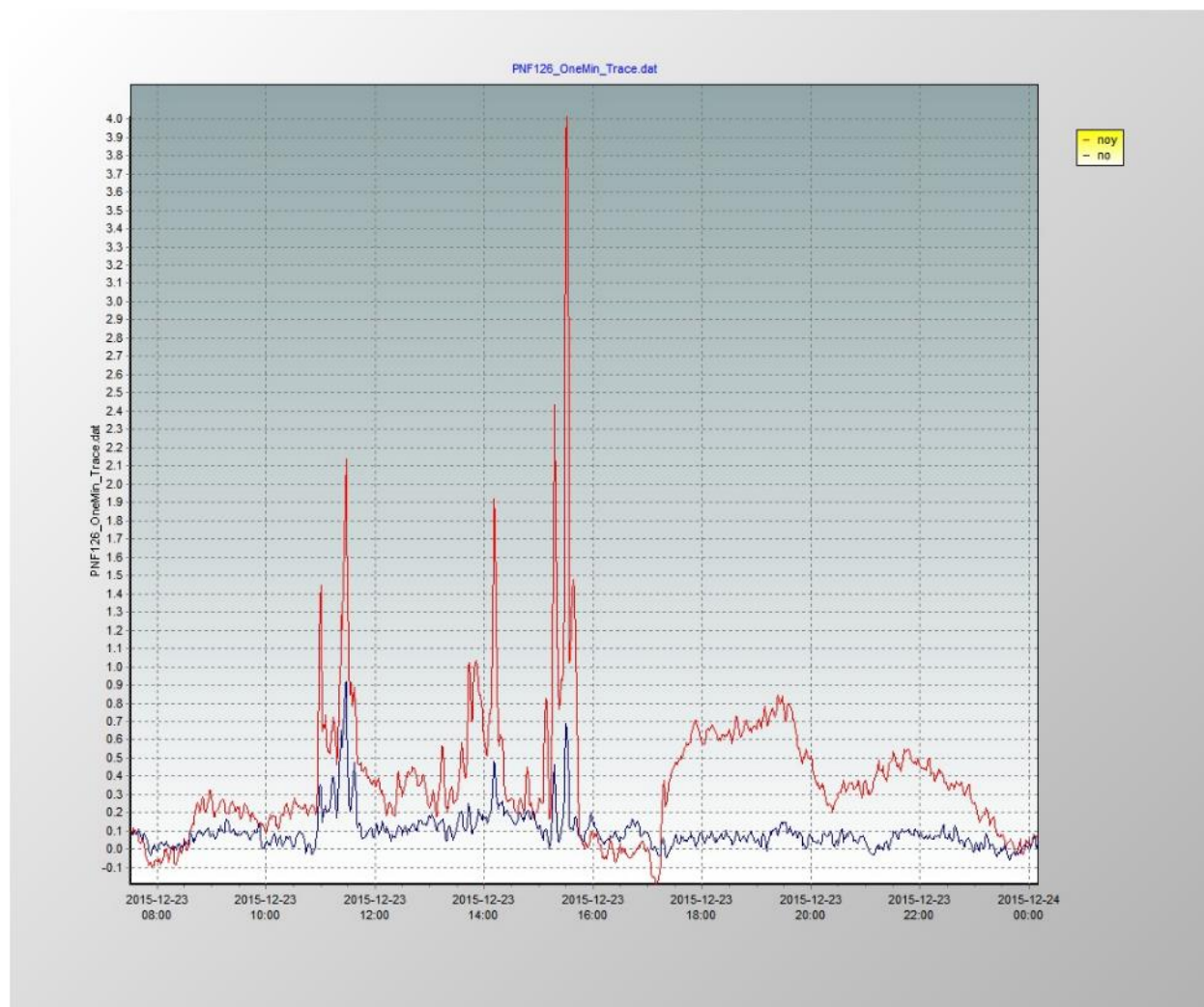
Figure 4-3. Time series of 1-minute \text{NO}_y and NO concentrations for PNF126, NC
