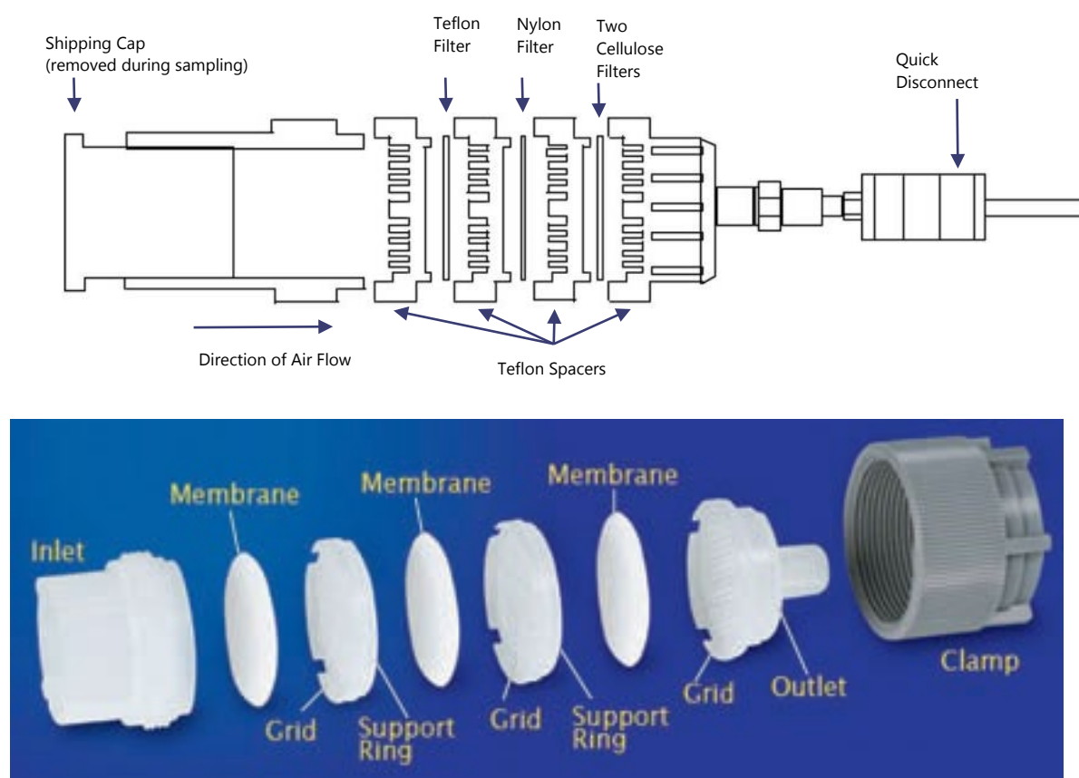
Figure 2-11. Filter Pack Assembly
