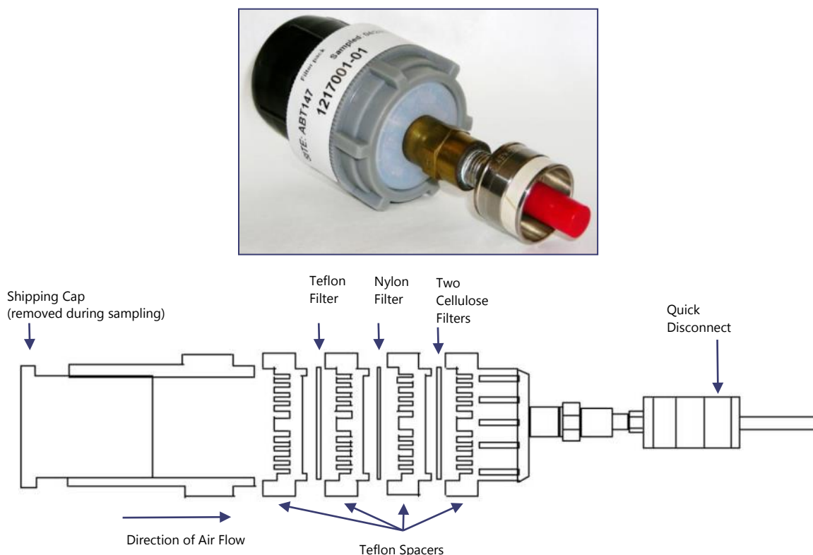
Figure 1-6. Three-Stage Filter Pack
