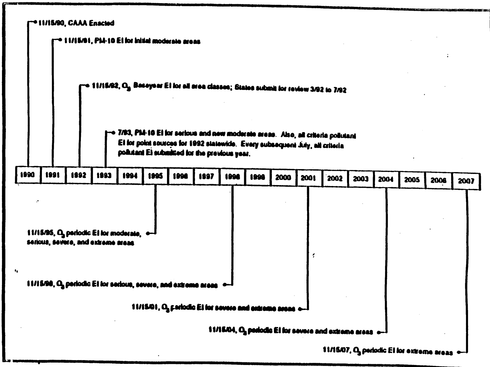
Figure 2-12. Timeline for criteria pollutant emission inventory State submittals.
