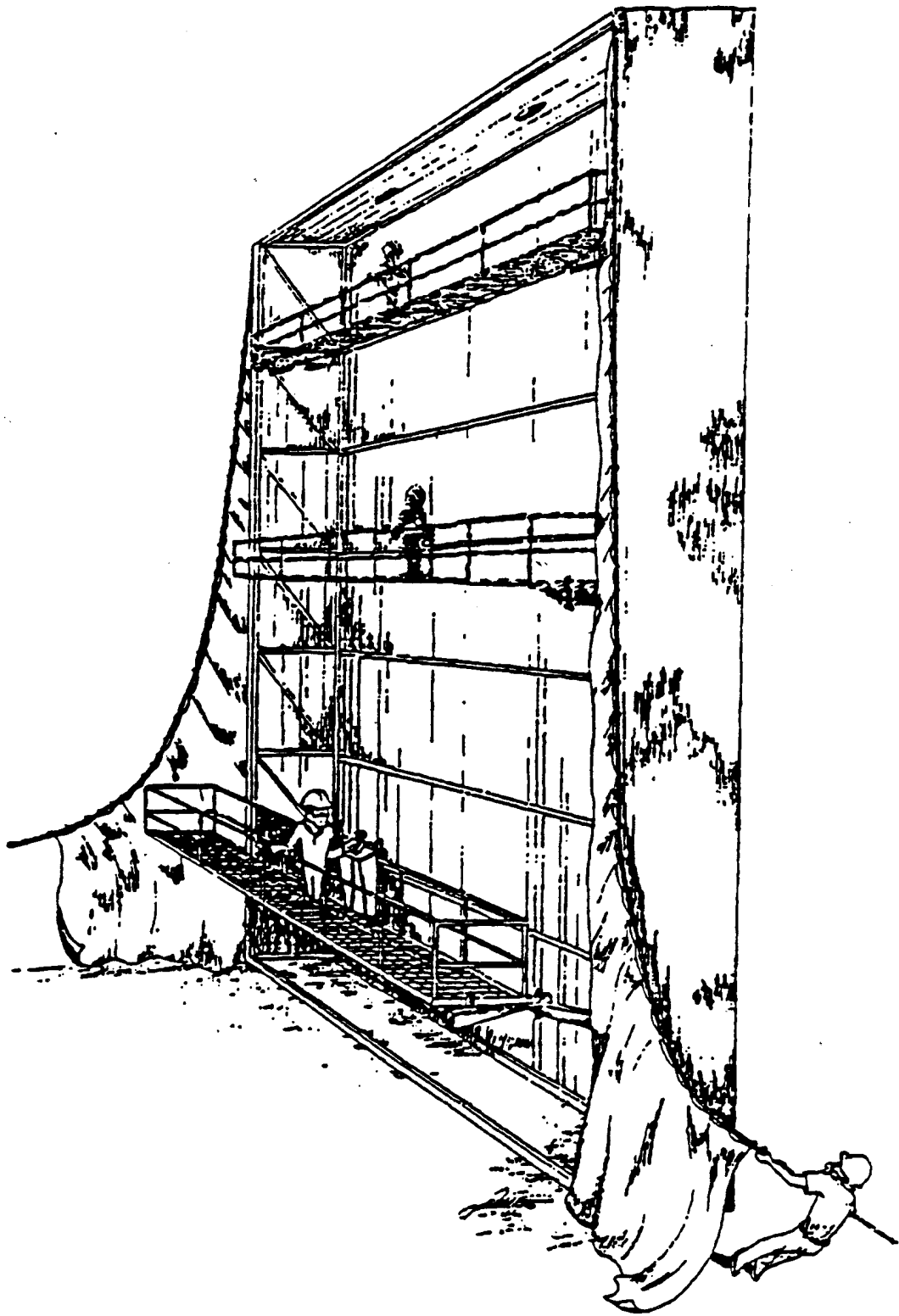
Figure 3-3. Portable enclosure. 5
