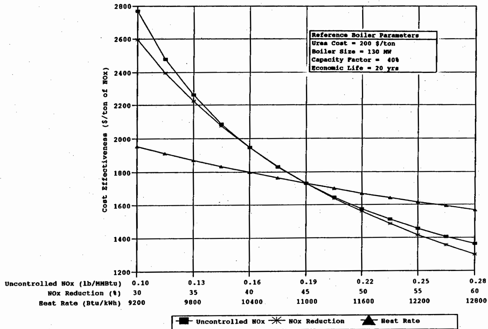
Figure 6-40. Impact of NO x emission characteristics and heat rate on SNCR cost effectiveness for coal-fired FBC boilers.
