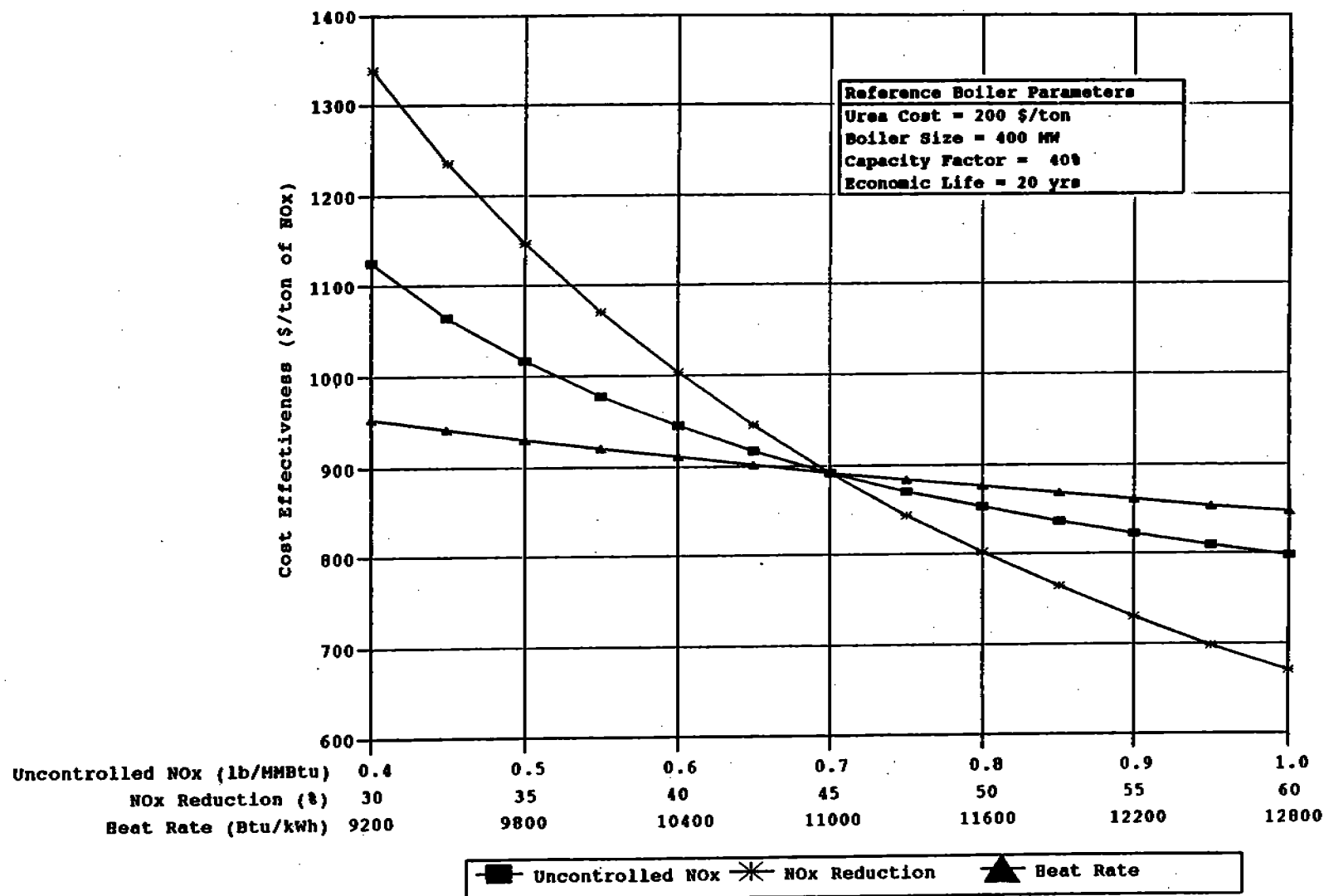
Figure 6-36. Impact of NO x emission characteristics and heat rate on SNCR cost effectiveness for coal-fired tangential boilers.
