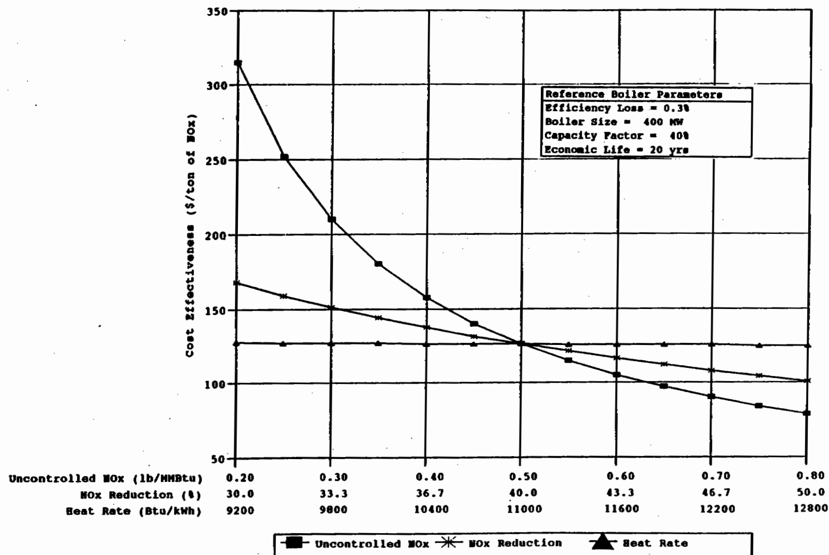
Figure 6-18. Impact of NO x emission characteristics and heat rate on LEA + BOOS cost effectiveness for natural gas- and oil-fired wall boilers.
