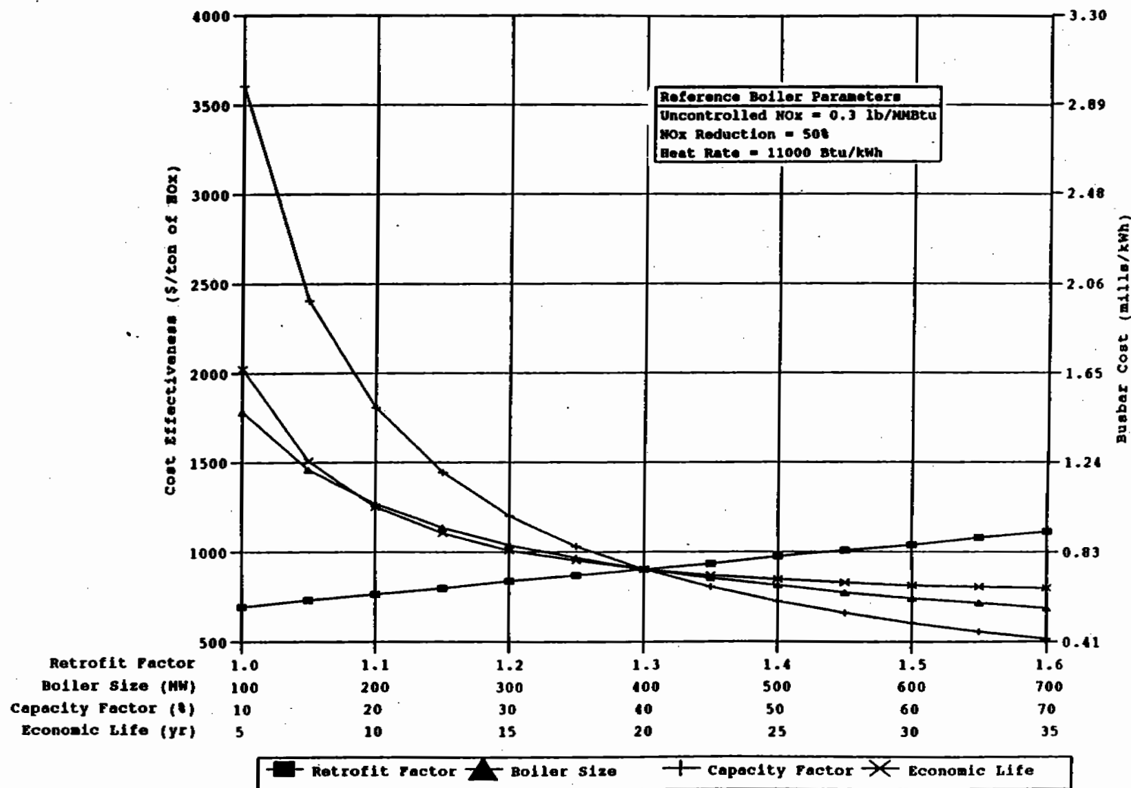
Figure 6-27. Impact of plant characteristics on LNB + AOFA cost effectiveness and busbar cost for natural gas- and oil-fired tangential boilers.
