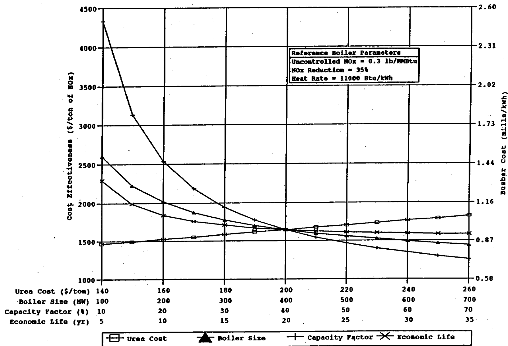
Figure 6-43. Impact of plant characteristics on SNCR cost effectiveness and busbar cost for natural gas- and oil-fired tangential boilers.
