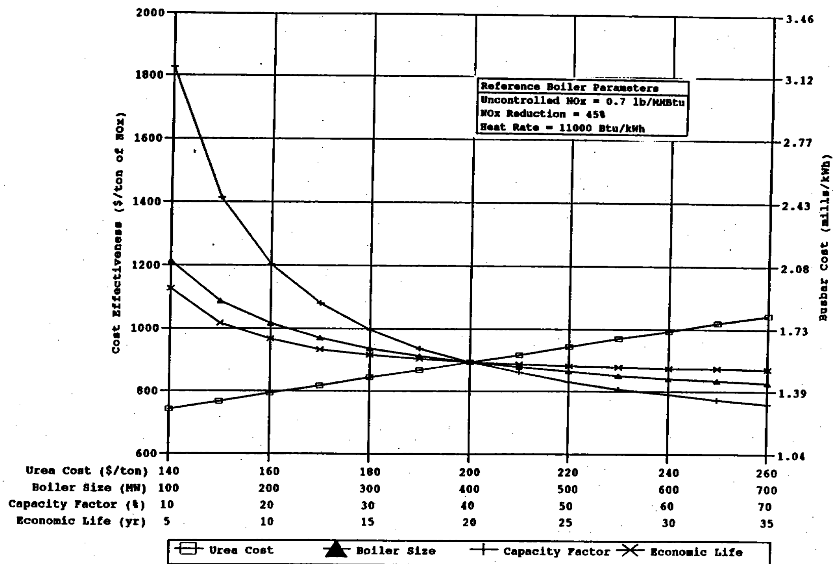
Figure 6-35. Impact of plant characteristics on SNCR cost effectiveness and busbar cost for coal-fired tangential boilers.
