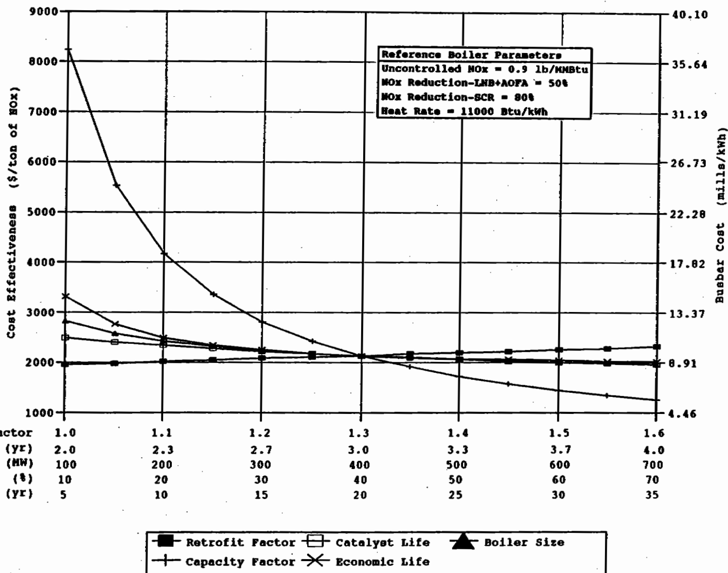
Figure 6-67. Impact of plant characteristics on LNB + AOFA + SCR cost effectiveness and busbar cost for coal-fired wall boilers.
