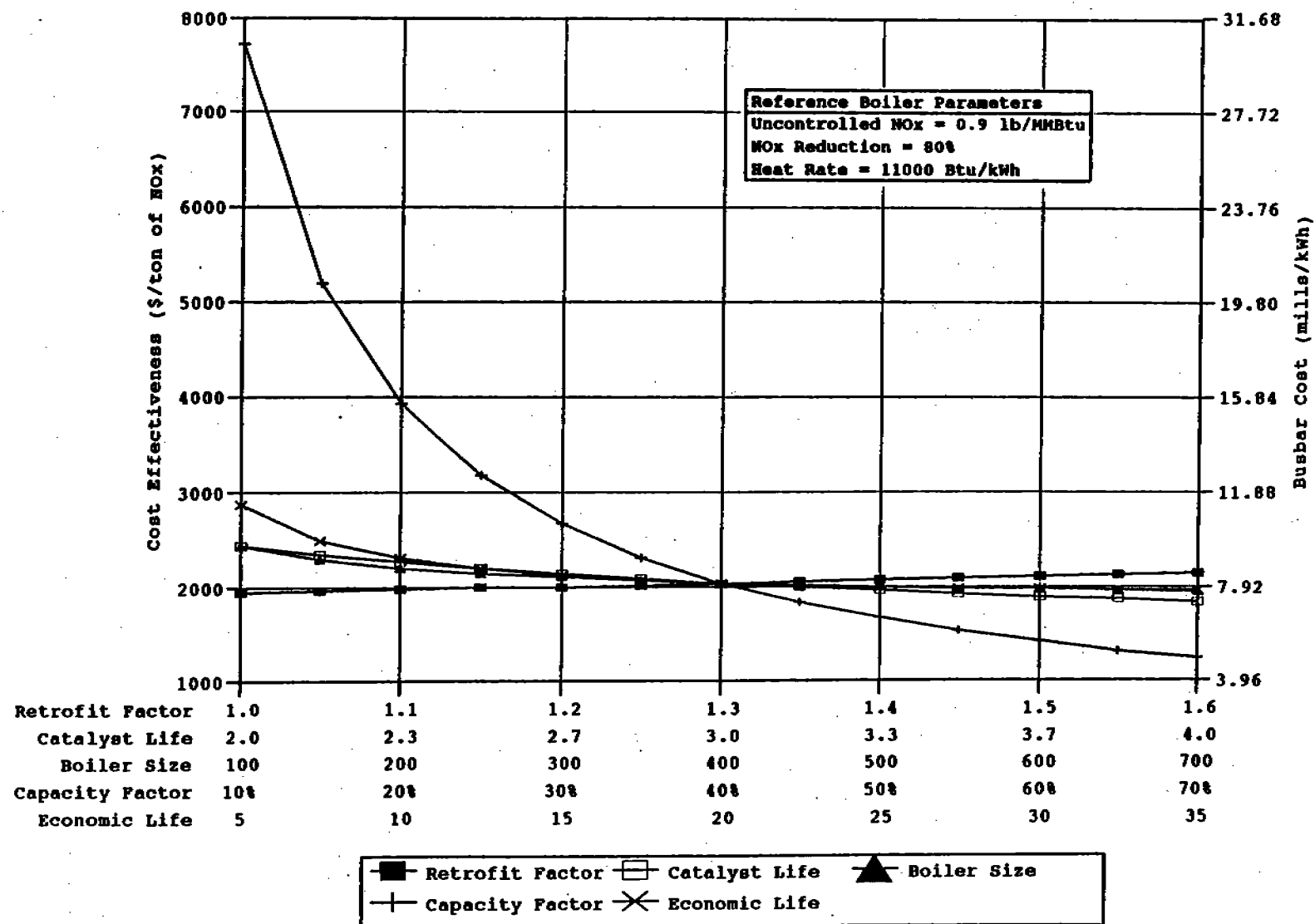
Figure 6-45. Impact of plant characteristics on SCR cost effectiveness and busbar cost for coal-fired wall boilers.
