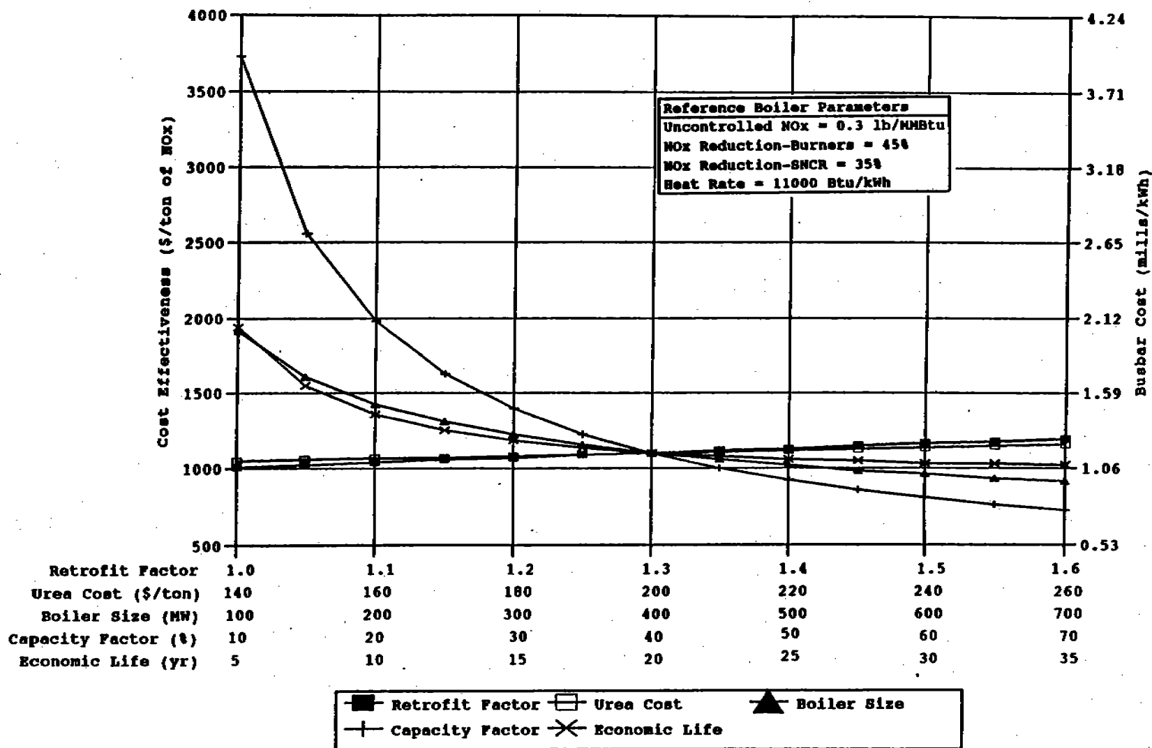
Figure 6-65. Impact of plant characteristics on LNB + SNCR cost effectiveness and busbar cost for natural gas- and oil-fired tangential boilers.
