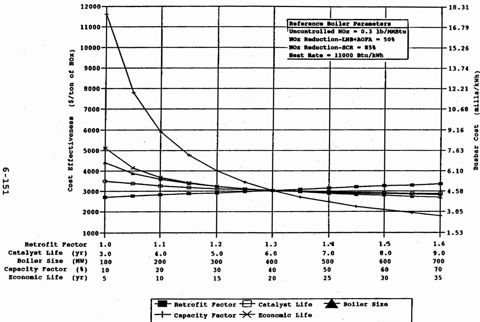
Figure 6-76. Impact of plant characteristics on LNB + AOFA + SCR cost effectiveness and busbar cost for oil-fired tangential boilers.
