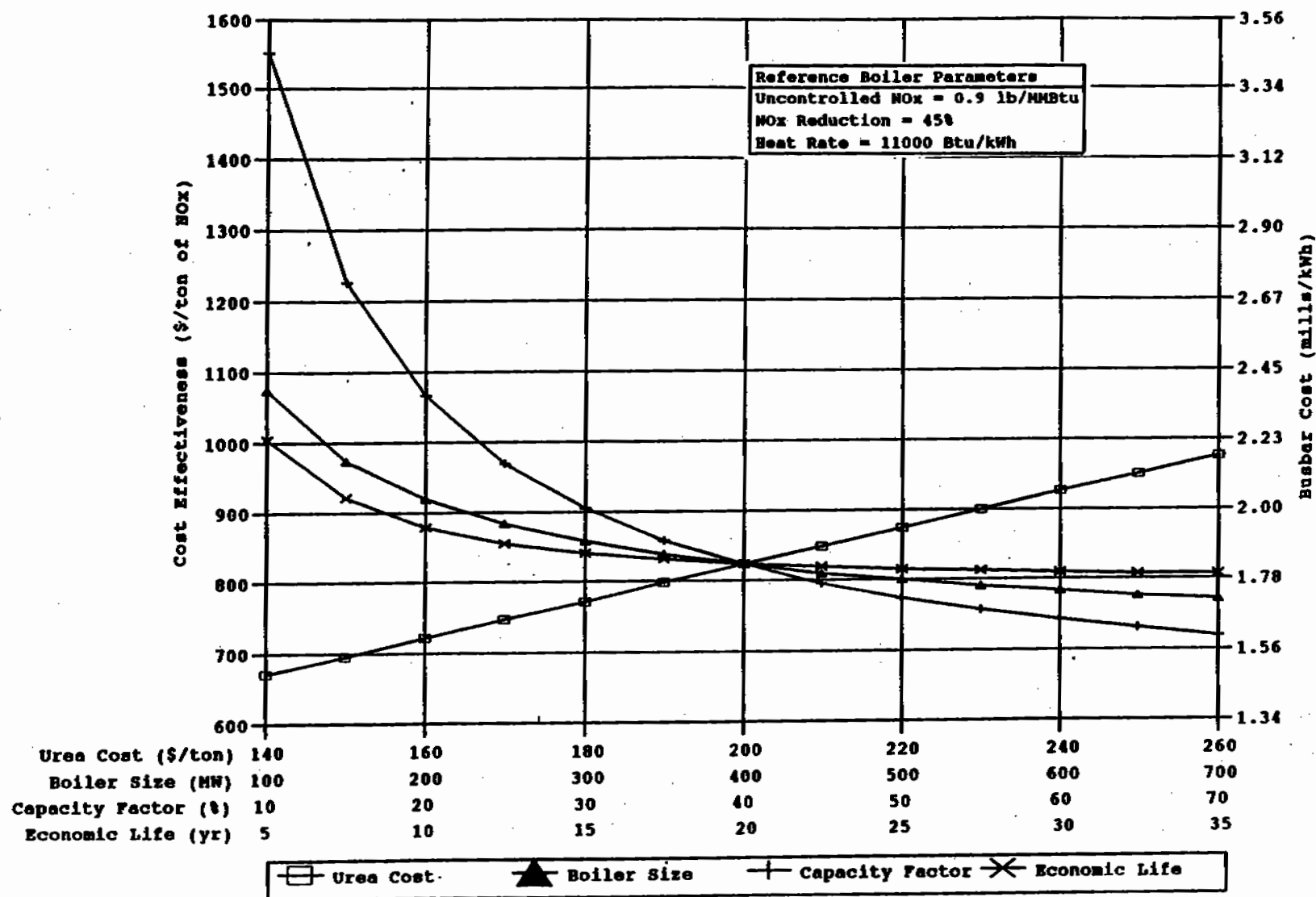
Figure 6-33. Impact of plant characteristics on SNCR cost effectiveness and busbar cost for coal-fired wall boilers.
