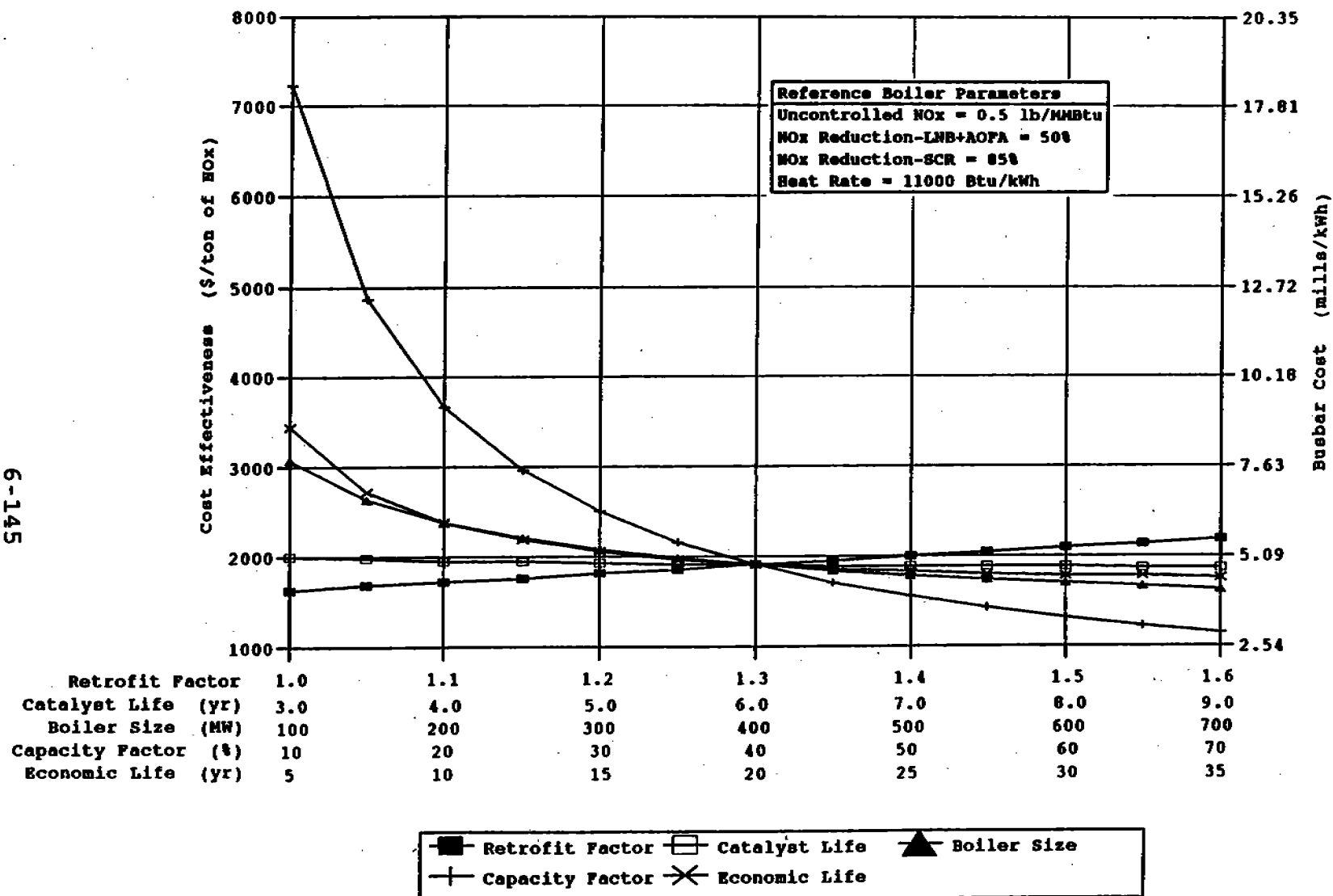
Figure 6-71. Impact of plant characteristics on LNB + AOFA + SCR cost effectiveness and busbar cost for natural gas-fired wall boilers.
