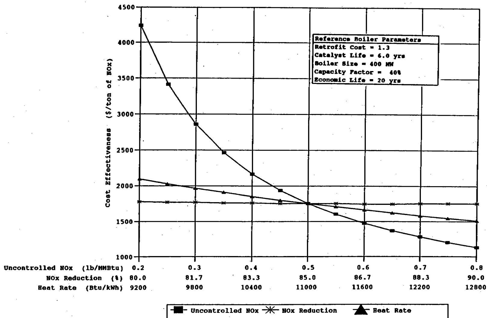
Figure 6-54. Impact of NO x emission characteristics and heat rate on SCR cost effectiveness for oil-fired wall boilers.
