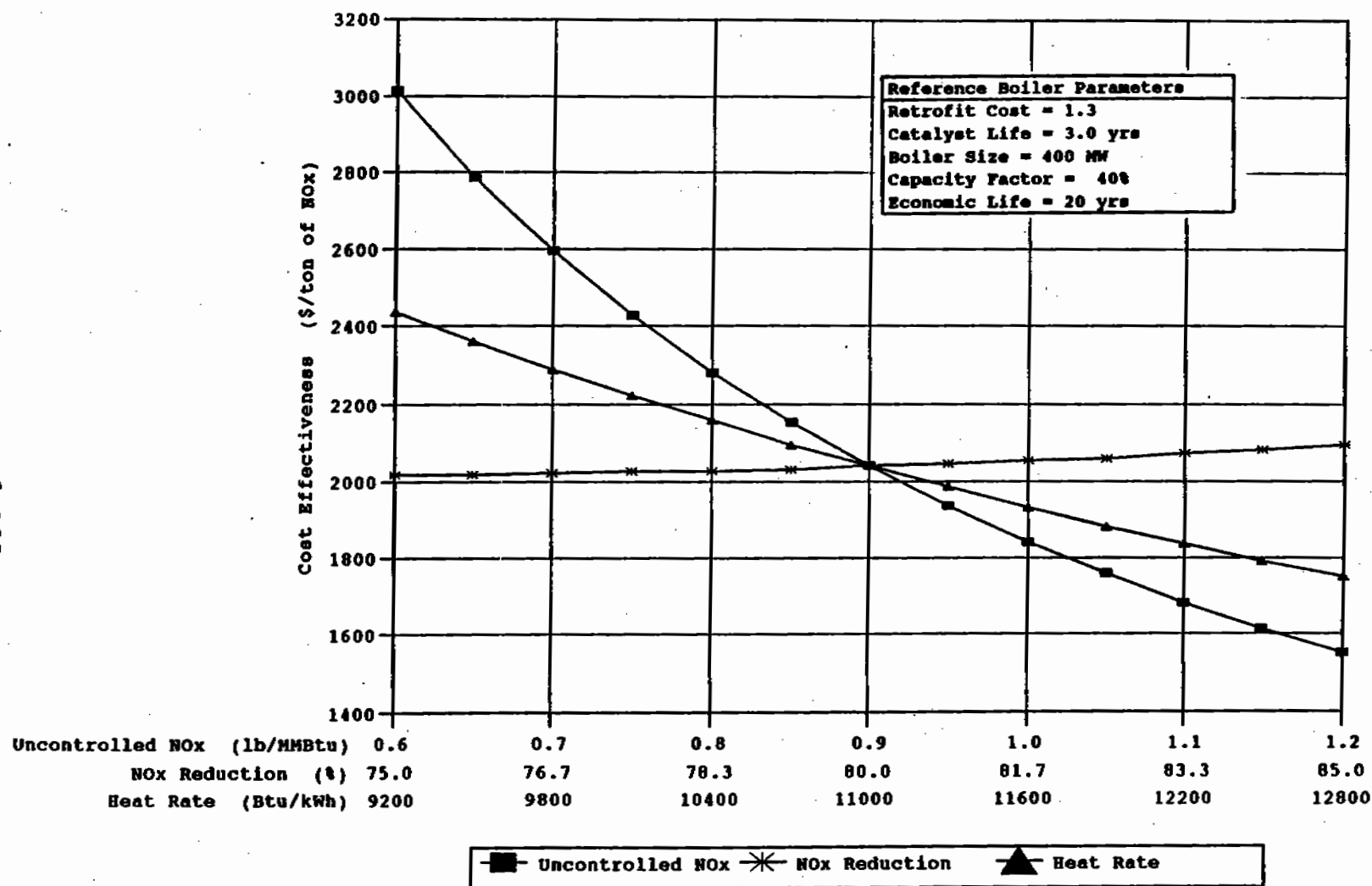
Figure 6-46. Impact of NO x emission characteristics and heat rate on SCR cost effectiveness for coal-fired wall boilers.
