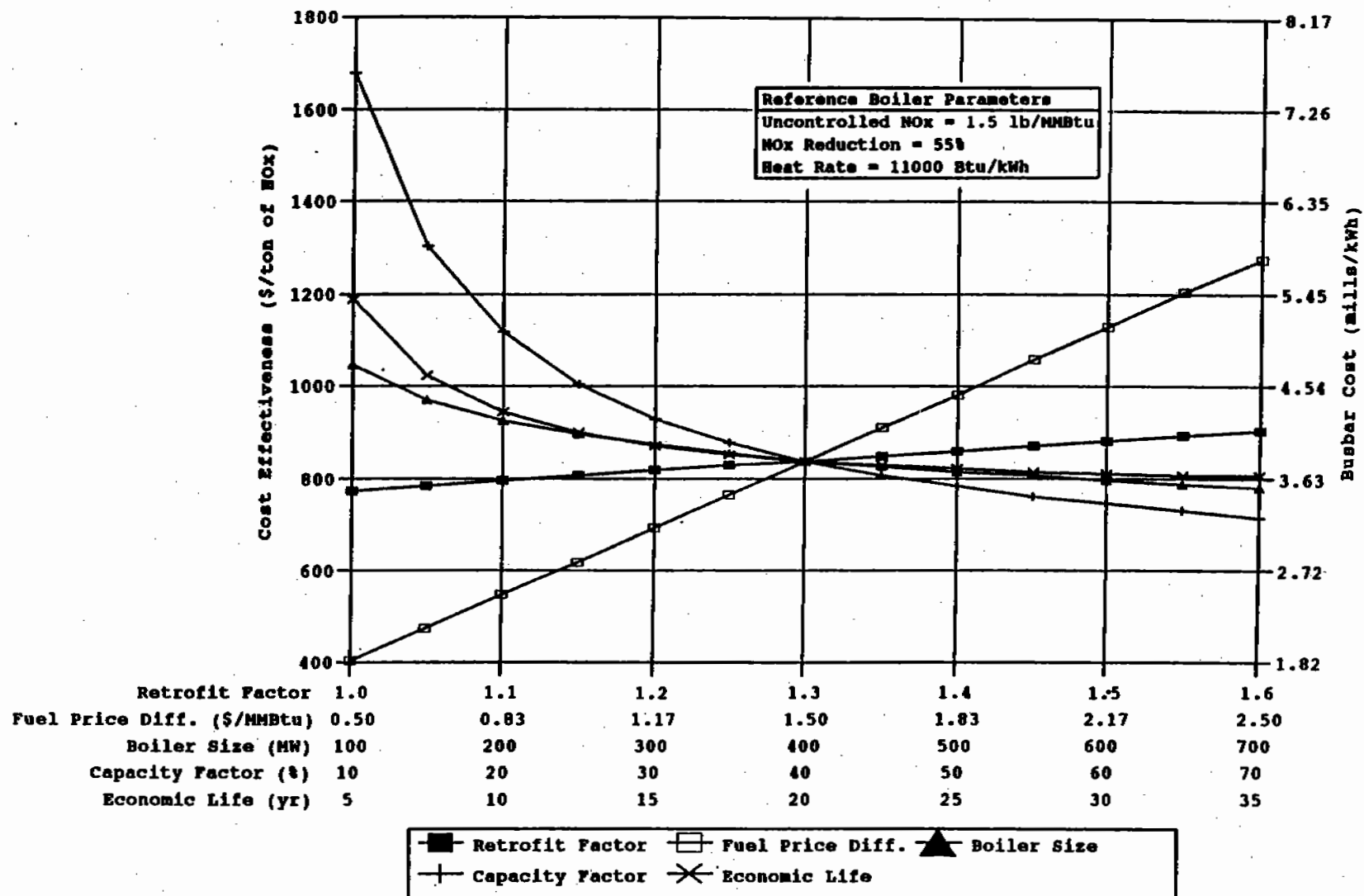
Figure 6-15. Impact of plant characteristics on NGR cost effectiveness and busbar cost for coal-fired cyclone boilers.
