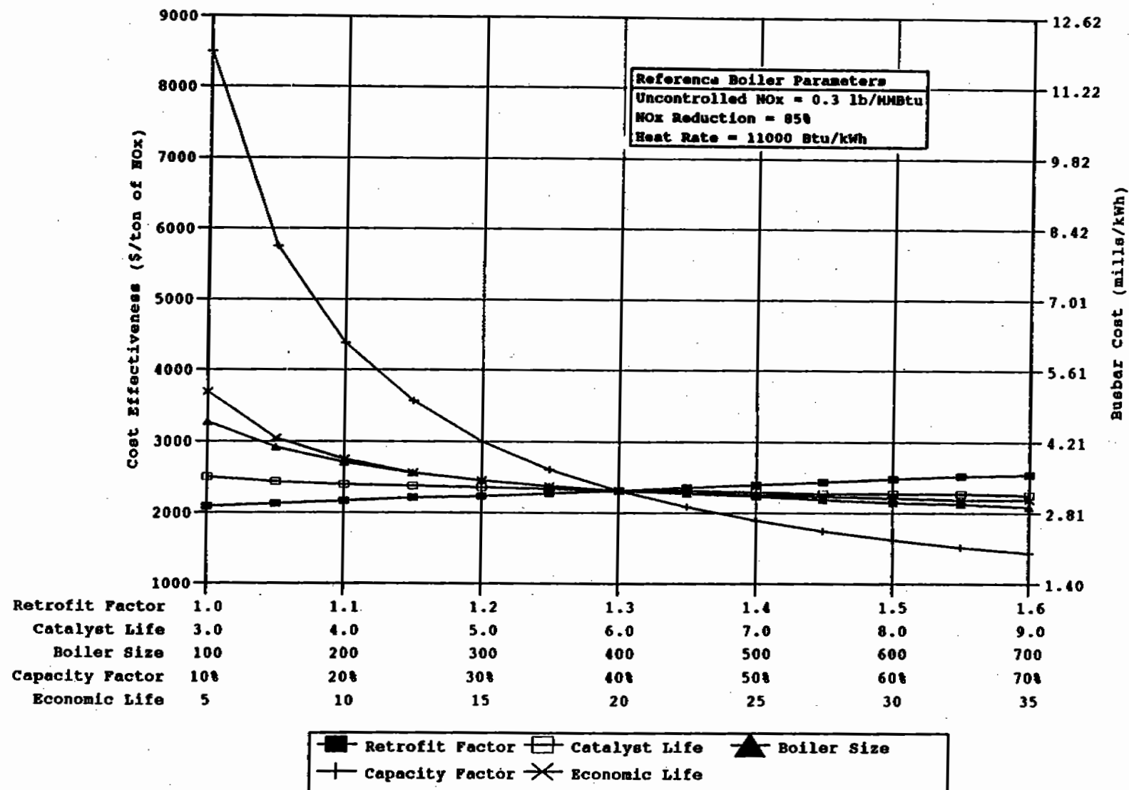
Figure 6-55. Impact of plant characteristics on SCR cost effectiveness and busbar cost for natural gas-fired tangential boilers.
