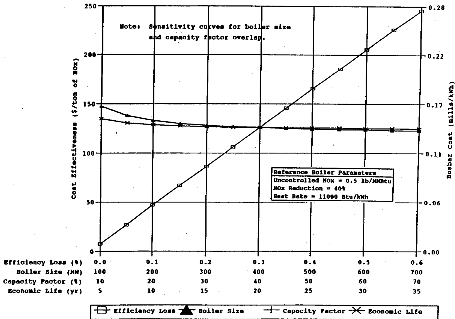
Figure 6-17. Impact of plant characteristics on LEA + BOOS cost effectiveness and busbar cost for natural gas- and oil-fired wall boilers.
