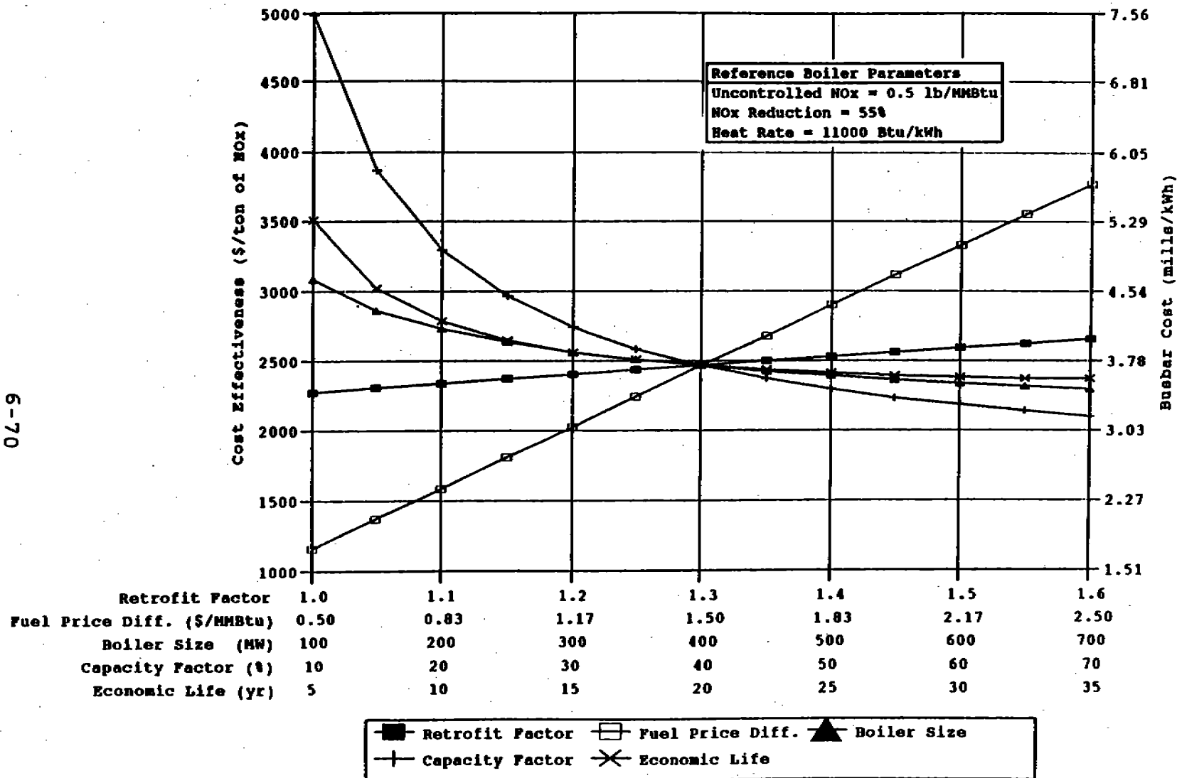
Figure 6-29. Impact of plant characteristics on NGR cost effectiveness and busbar cost for oil-fired wall boilers.
