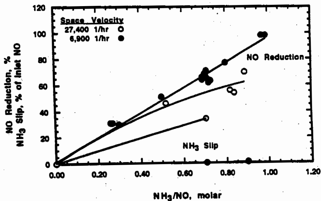
Figure 5-49b. Vanadium titanium extruded catalyst \text{NO}_x conversion and residual \text{NH}_3 versus \text{NH}_3 -to- \text{NO}_x ratio. 133
