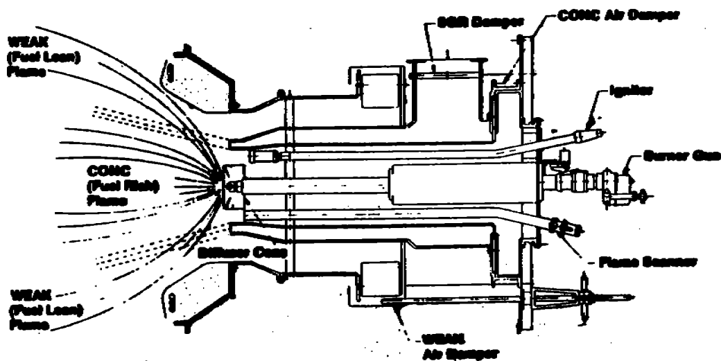
Figure 5-25. ROPM™ burner for natural gas- and oil-fired boilers. 83
