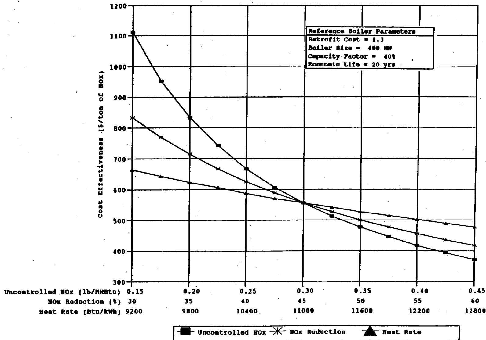
Figure 6-24. Impact of NO x emission characteristics and heat rate on LNB cost effectiveness for natural gas- and oil-fired tangential boilers.
