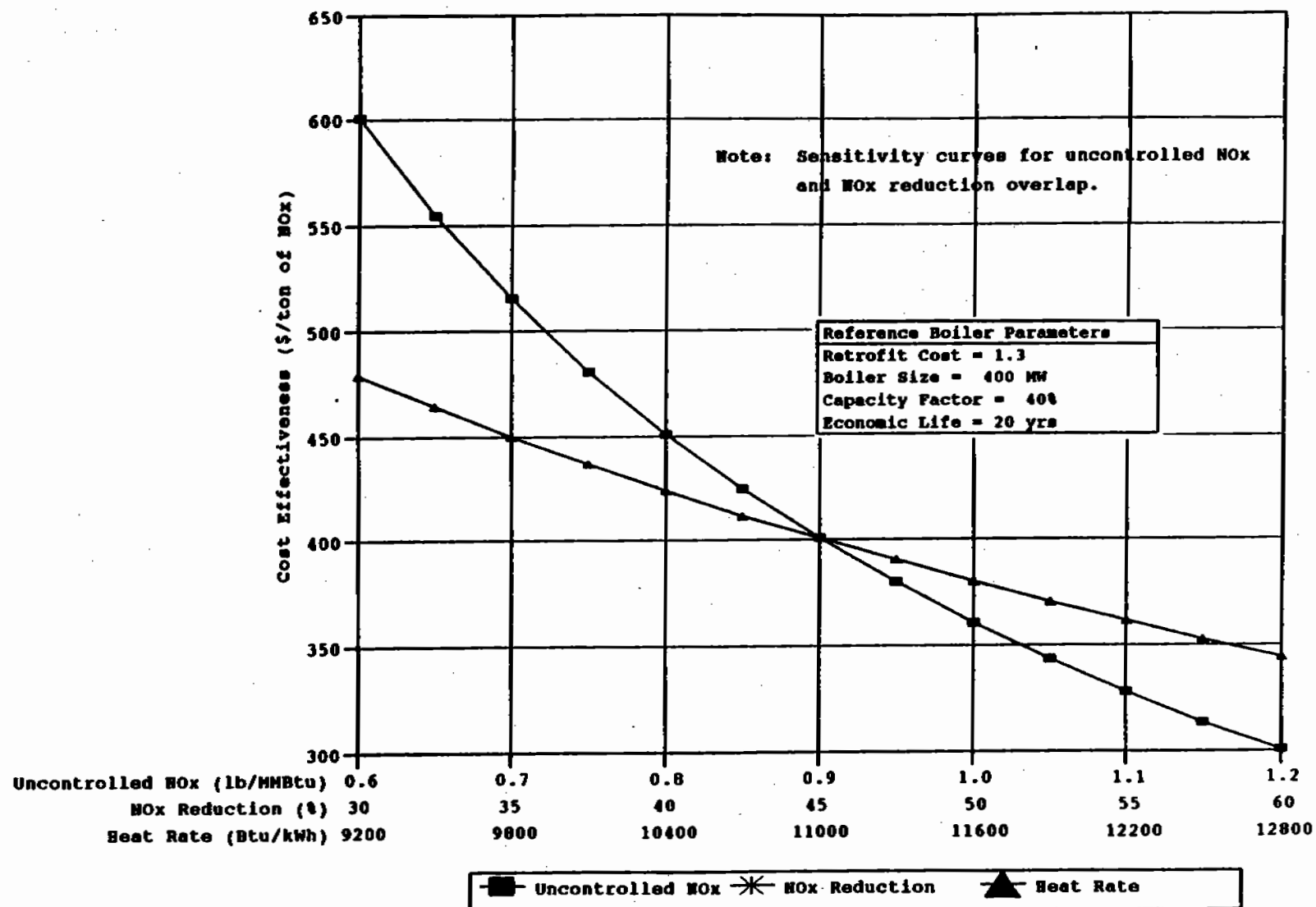
Figure 6-4. Impact of NO x emission characteristics and heat rate on LNB cost effectiveness for coal-fired wall boilers.
