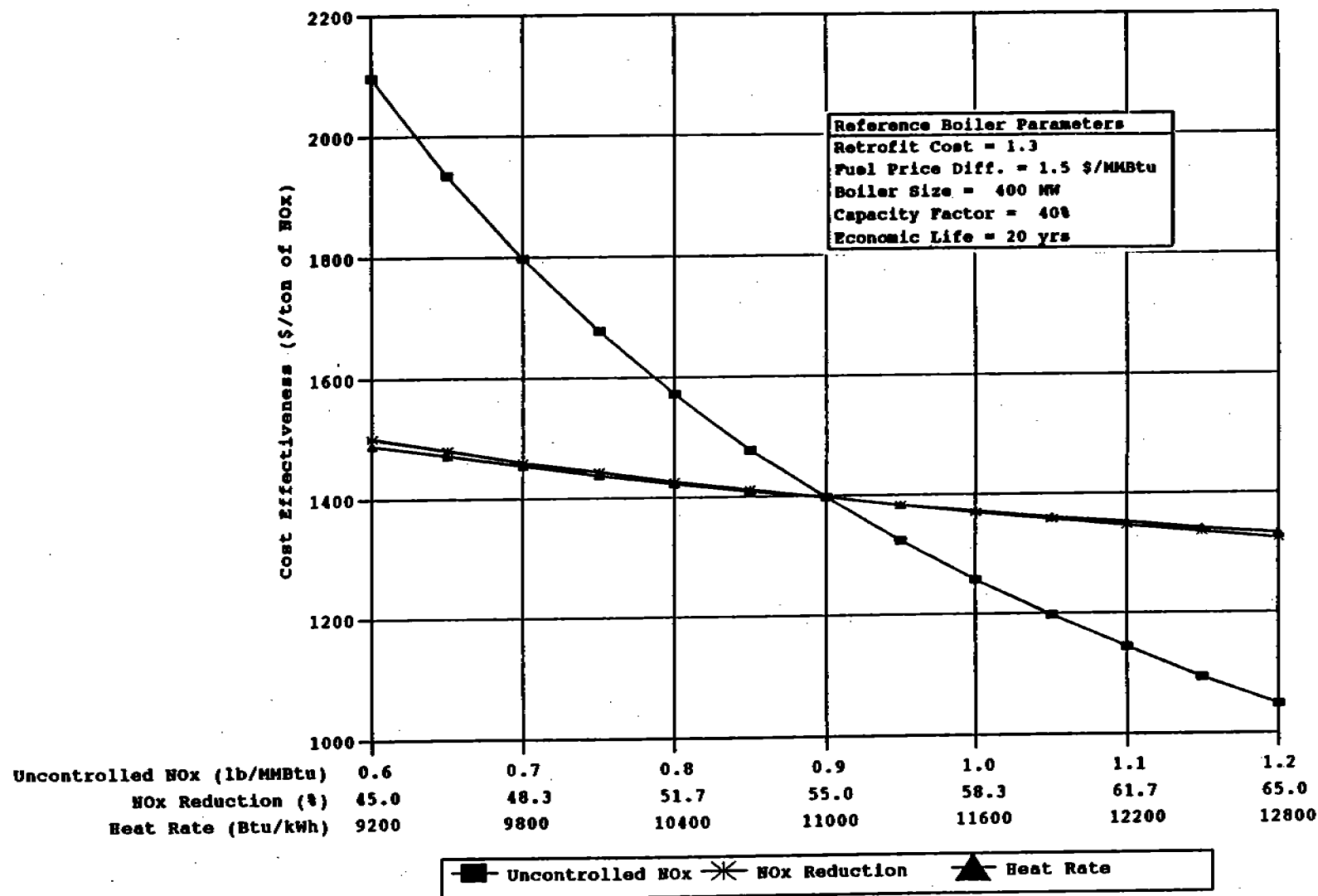
Figure 6-12. Impact of NO x emission characteristics and heat rate on NGR cost effectiveness for coal-fired wall boilers.
