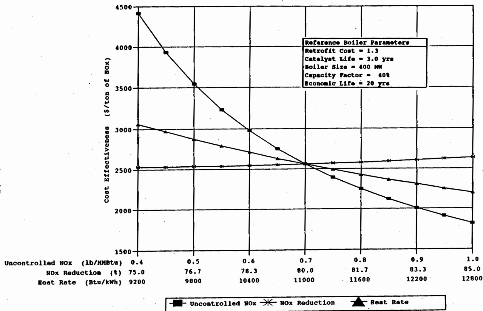
Figure 6-48. Impact of NO x emission characteristics and heat rate on SCR cost effectiveness for coal-fired tangential boilers.
