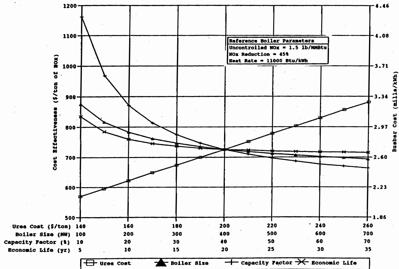
Figure 6-37. Impact of plant characteristics on SNCR cost effectiveness and busbar cost for coal-fired cyclone boilers.
