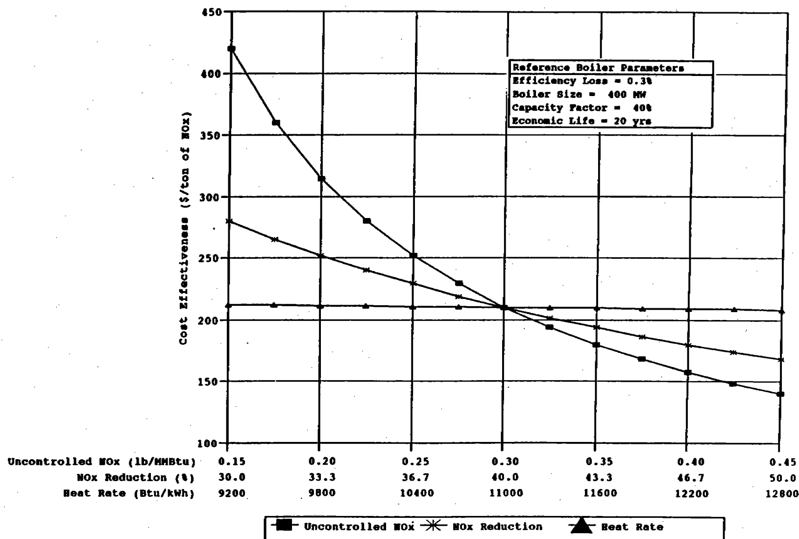
Figure 6-20. Impact of NO x emission characteristics and heat rate on LEA + BOOS cost effectiveness for natural gas- and oil-fired boilers.
