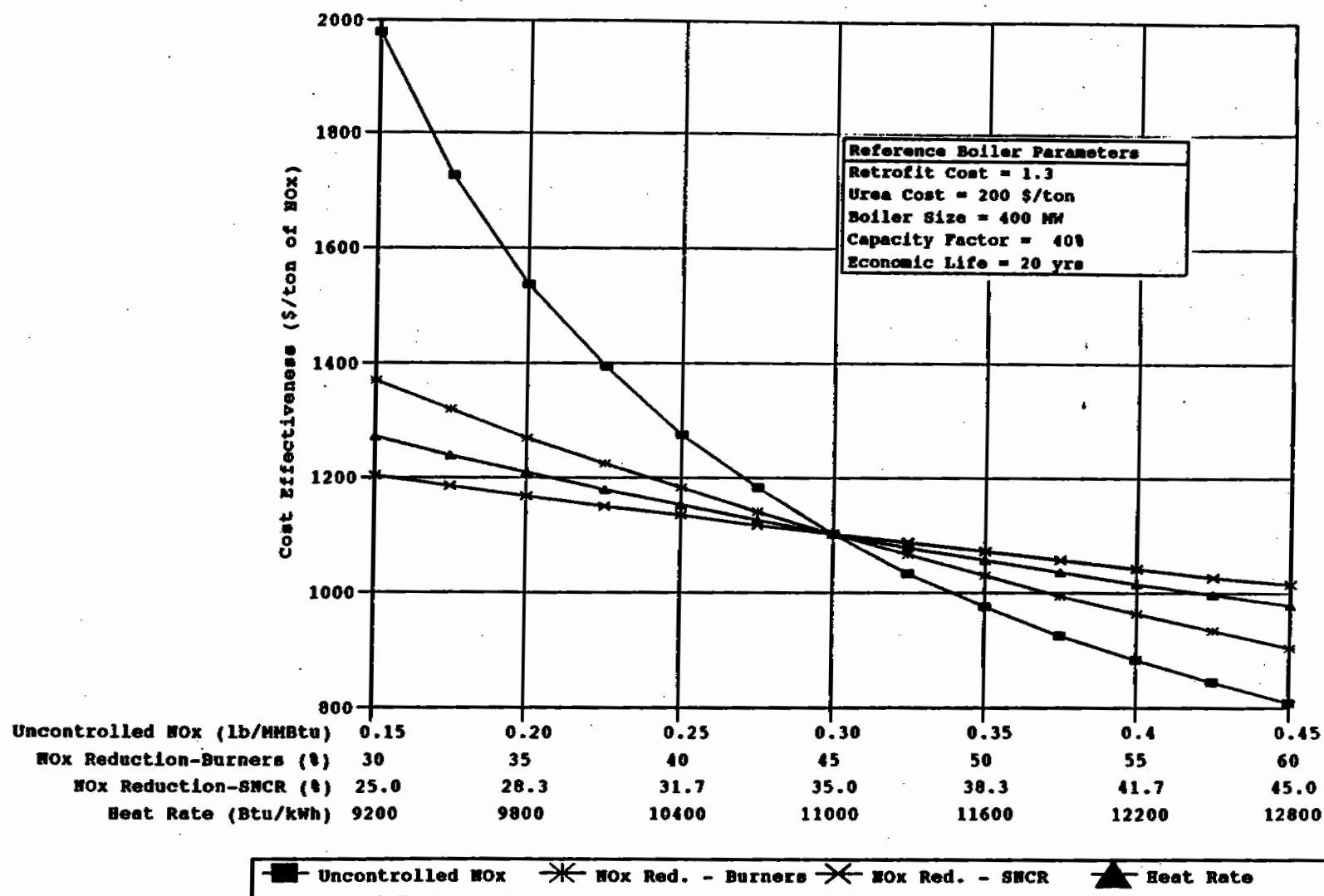
Figure 6-66. Impact of NO x emission characteristics and heat rate on LNB + SNCR cost effectiveness for natural gas- and oil-fired tangential boilers.
