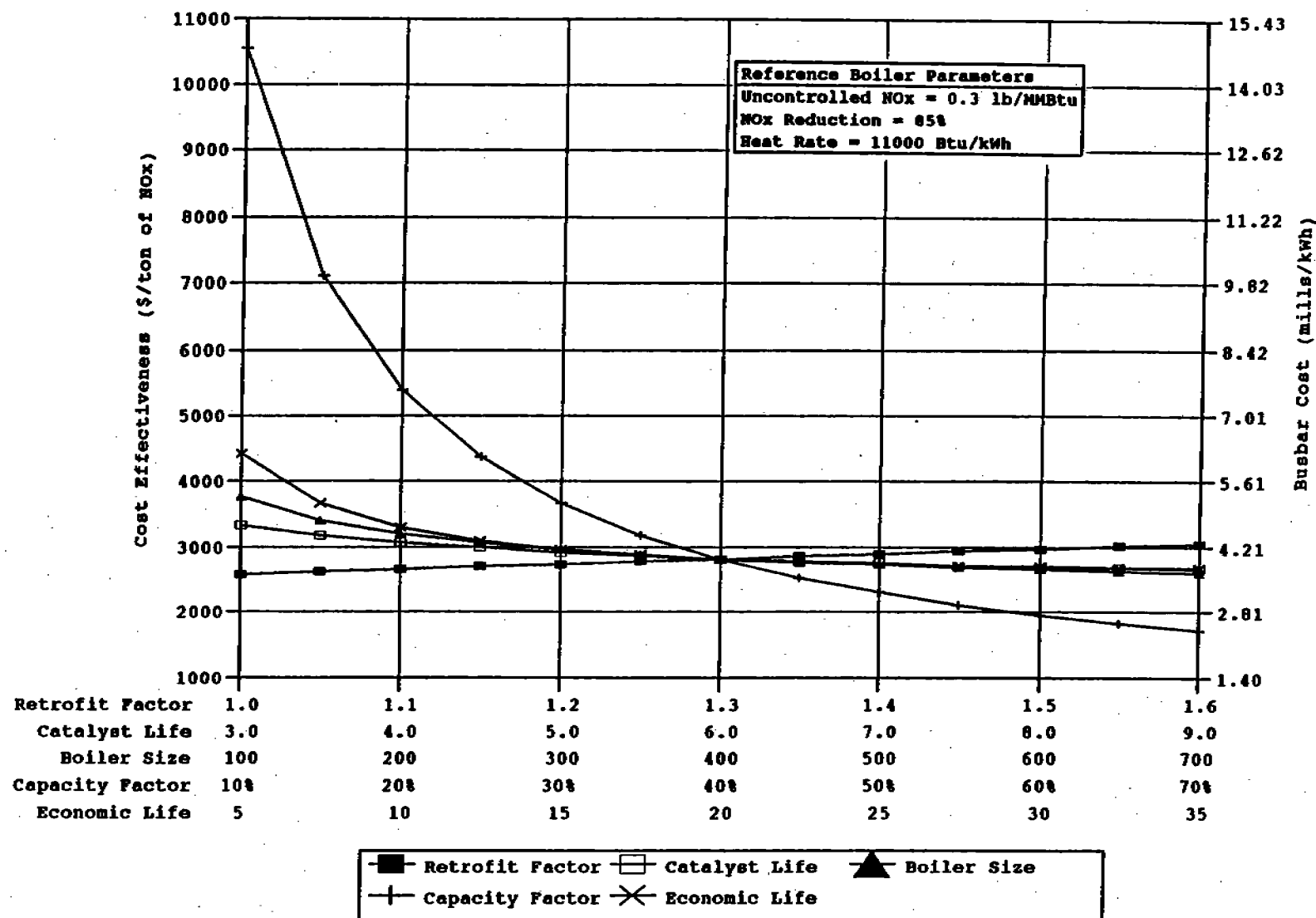
Figure 6-56. Impact of plant characteristics on SCR cost effectiveness and busbar cost for oil-fired tangential boilers.
