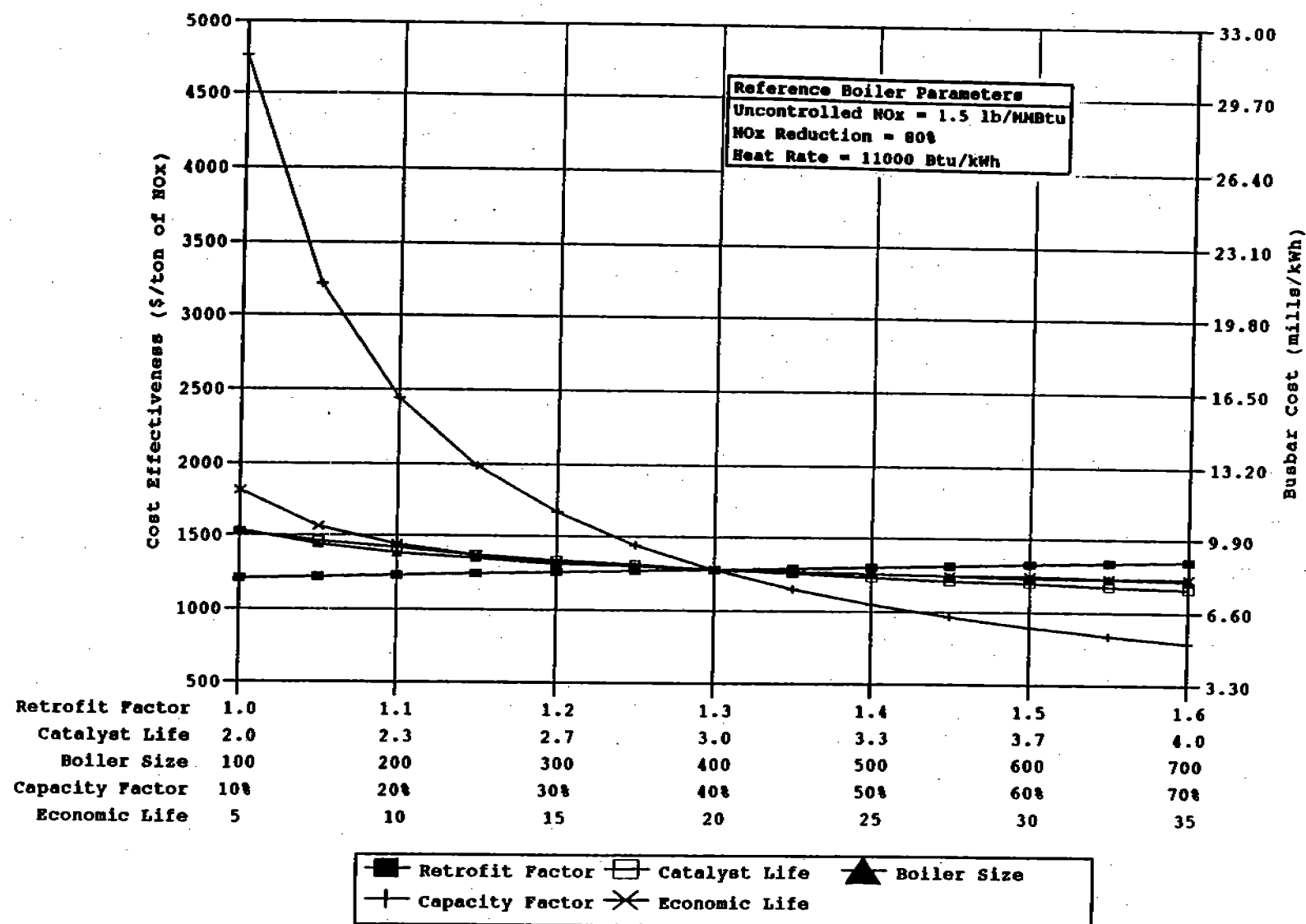
Figure 6-49. Impact of plant characteristics on SCR cost effectiveness and busbar cost for coal-fired cyclone boilers.
