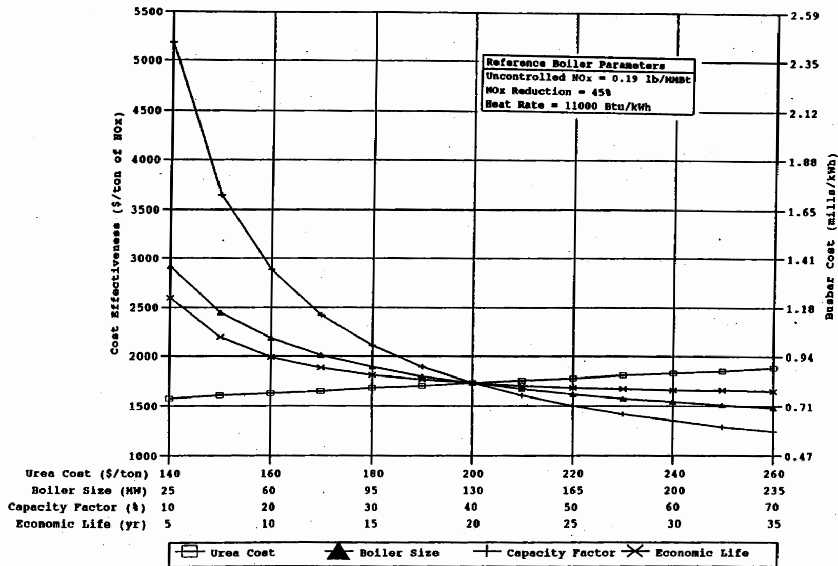
Figure 6-39. Impact of plant characteristics on SNCR cost effectiveness and busbar cost for coal-fired FBC boilers.
