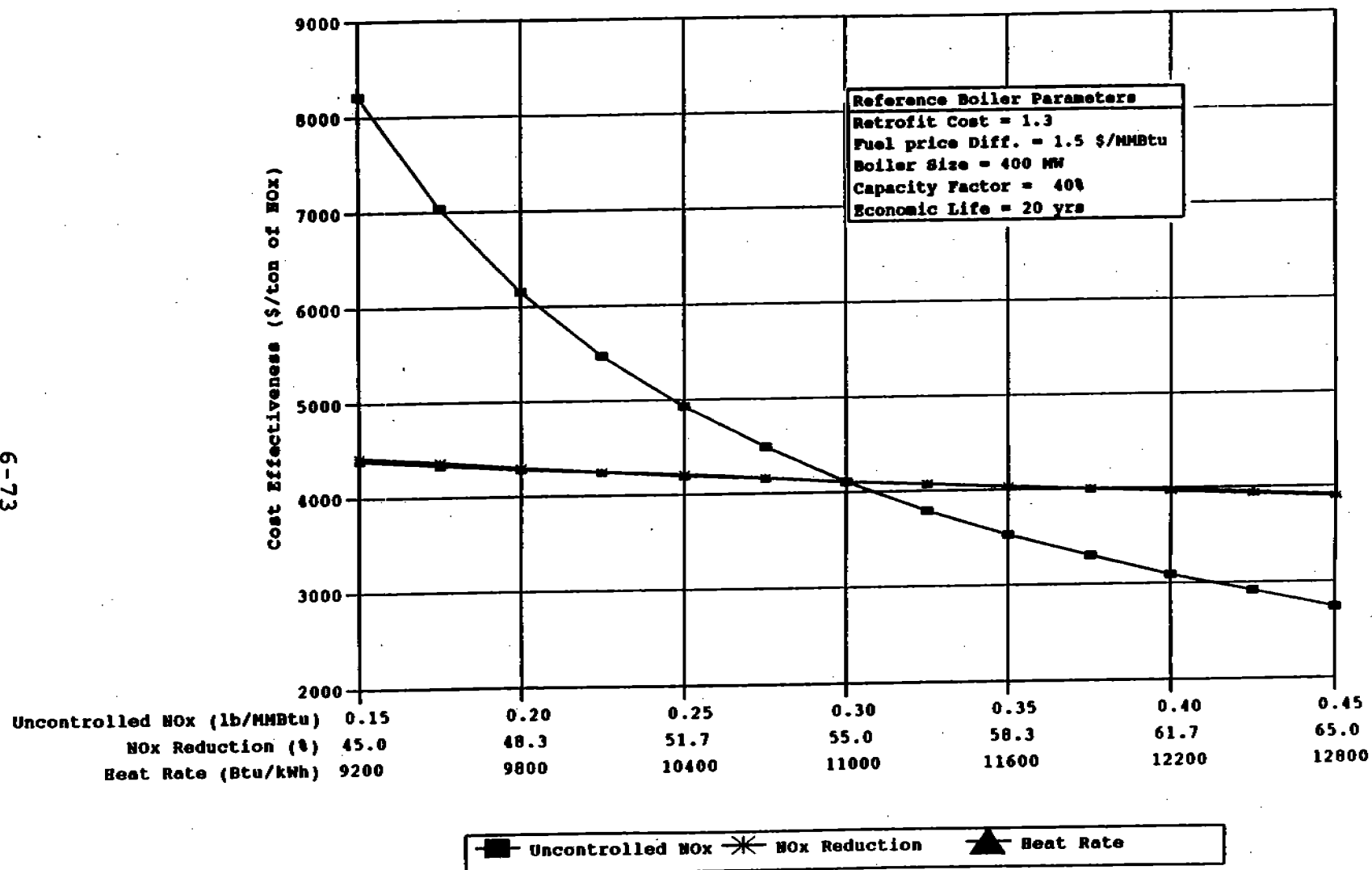
Figure 6-32. Impact of NO x emission characteristics and heat rate on NGR cost effectiveness for oil-fired tangential boilers.
