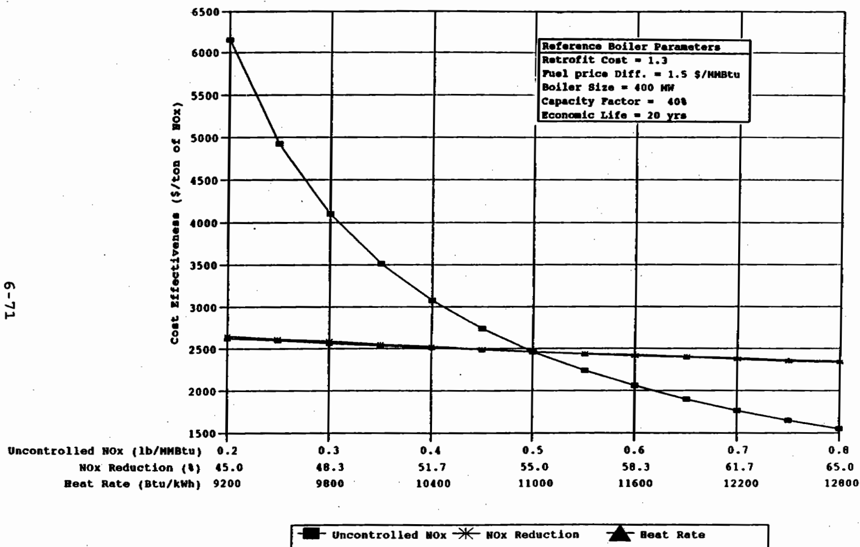
Figure 6-30. Impact of NO x emission characteristics and heat rate on NGR cost effectiveness for oil-fired wall boilers.
