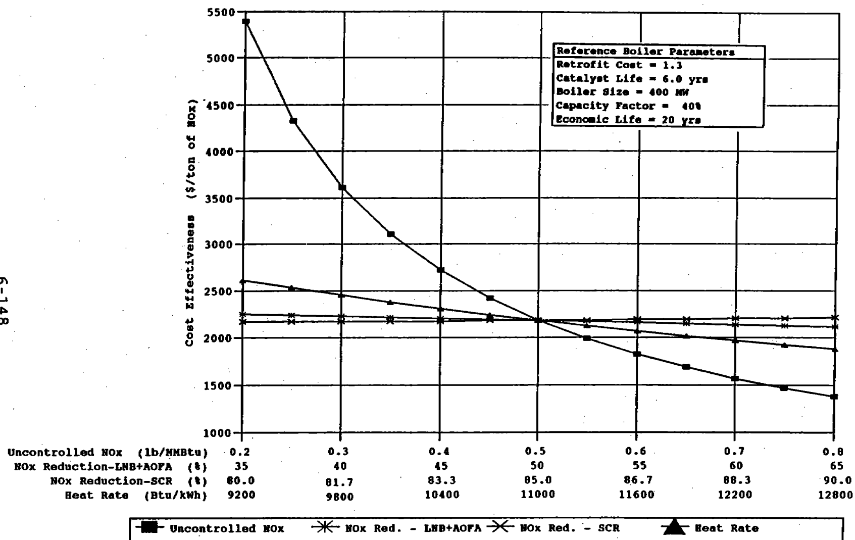
Figure 6-74. Impact of NO x emission characteristics and heat rate on LNB + AOFA + SCR cost effectiveness for oil-fired wall boilers.
