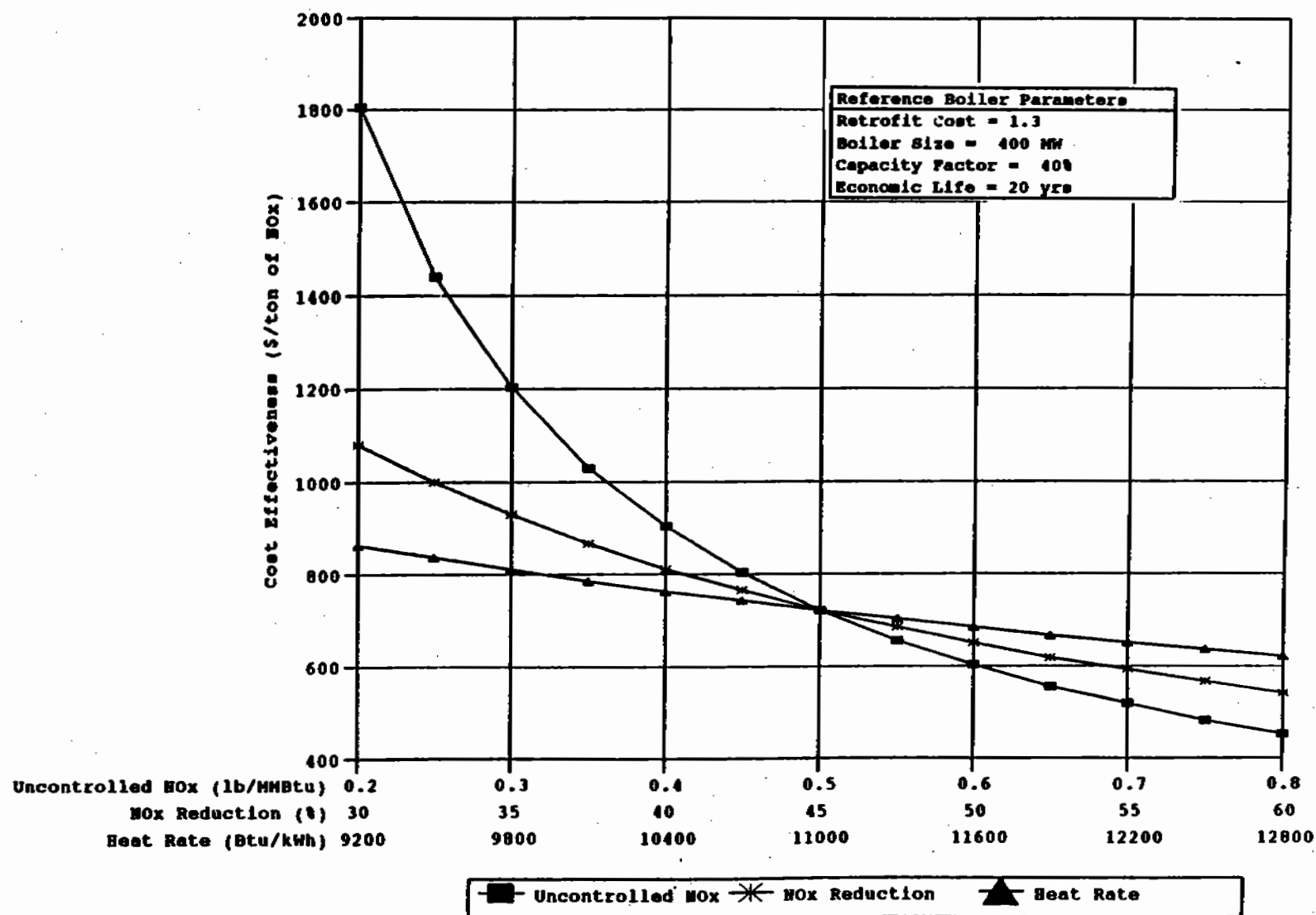
Figure 6-22. Impact of NO x emission characteristics and heat rate on LNB cost effectiveness for natural gas- and oil-fired wall boilers.
