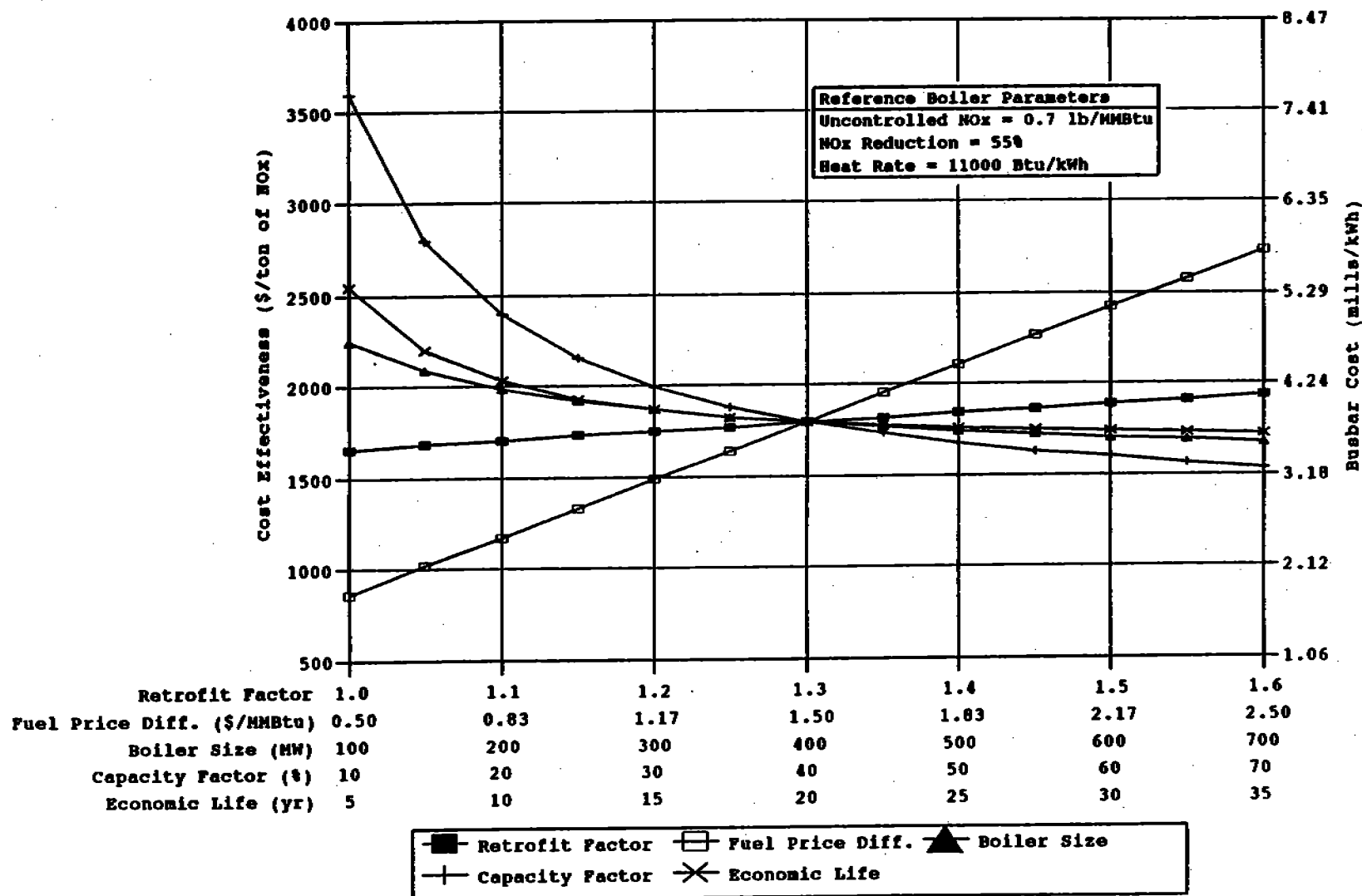
Figure 6-13. Impact of plant characteristics on NGR cost effectiveness and busbar cost for coal-fired tangential boilers.
