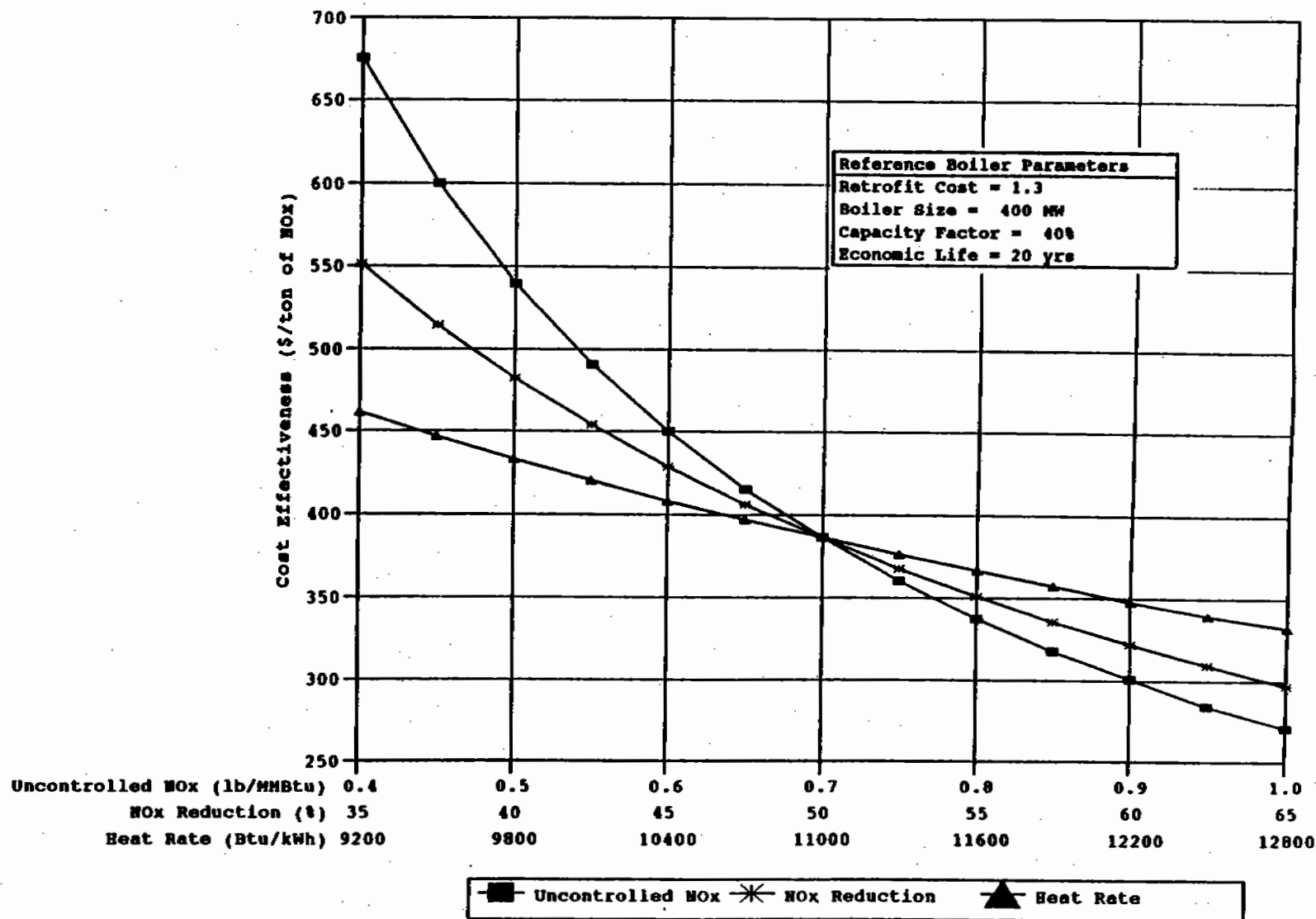
Figure 6-10. Impact of NO x emission characteristics and heat rate on LNB + AOFA cost effectiveness for coal-fired tangential boilers.
