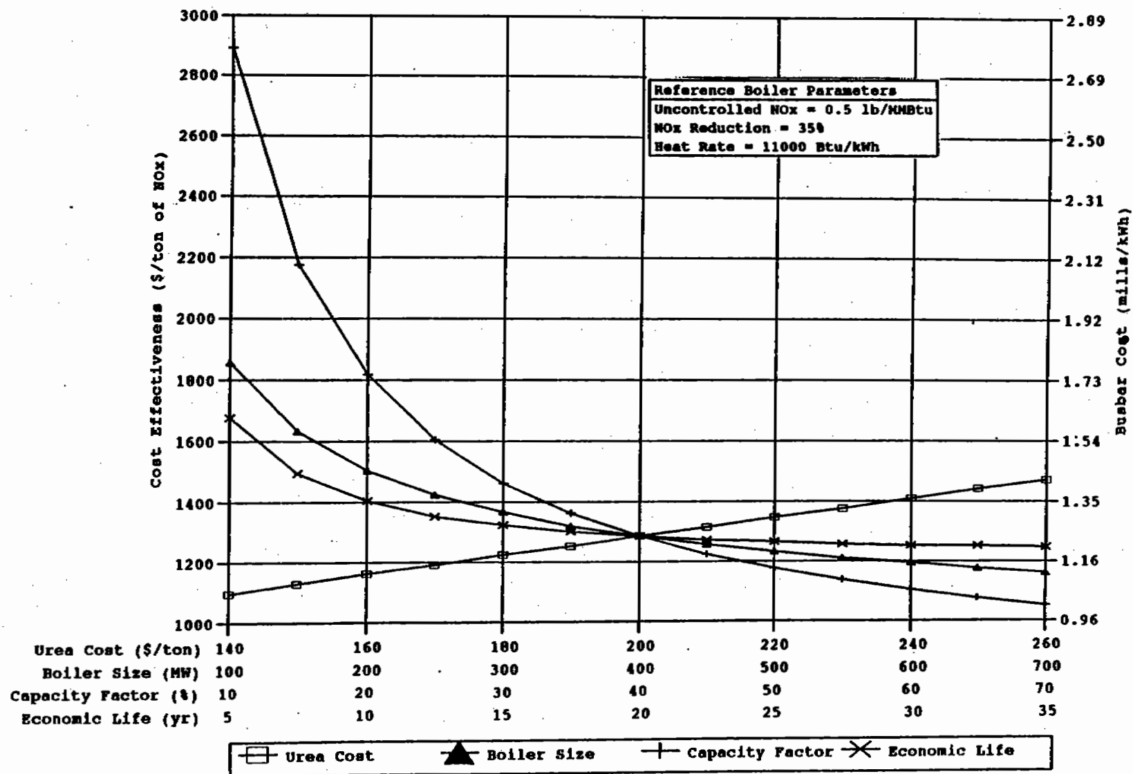
Figure 6-41. Impact of plant characteristics on SNCR cost effectiveness and busbar cost for natural gas- and oil-fired wall boilers.
