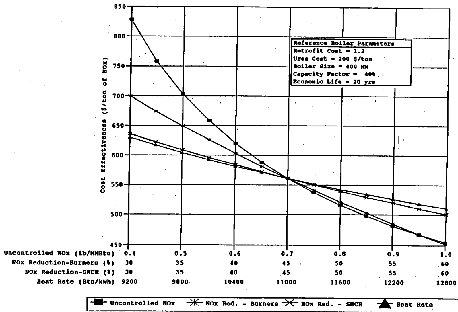
Figure 6-62. Impact of NO x emission characteristics and heat rate on LNB + SNCR cost effectiveness for coal-fired tangential boilers.
