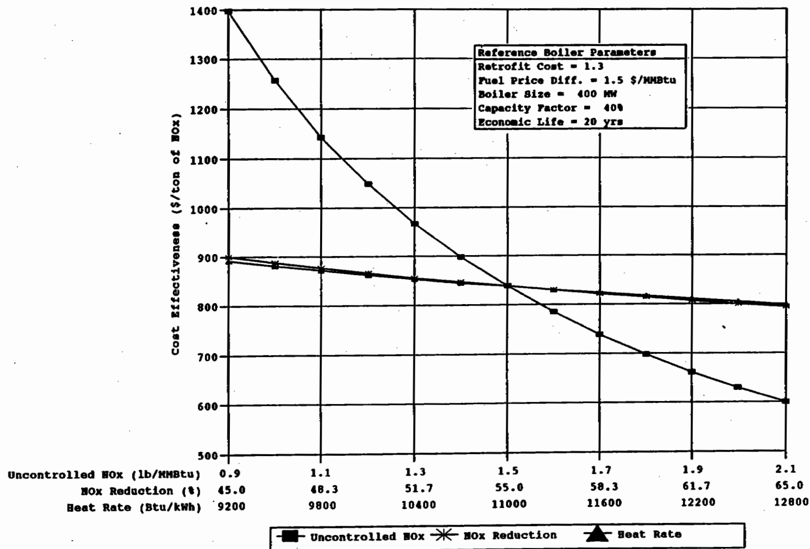
Figure 6-16. Impact of NO x emission characteristics and heat rate on NGR cost effectiveness for coal-fired cyclone boilers.
