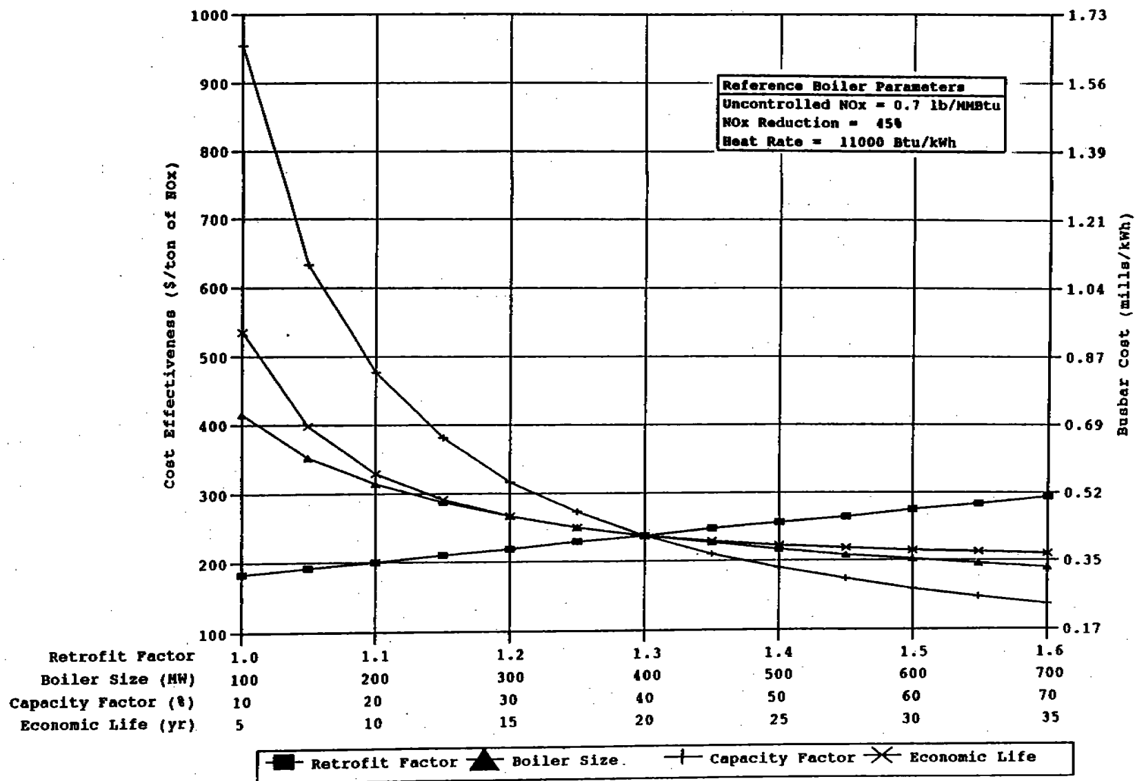
Figure 6-1. Impact of plant characteristics on LNB cost effectiveness and busbar cost for coal-fired tangential boilers.
