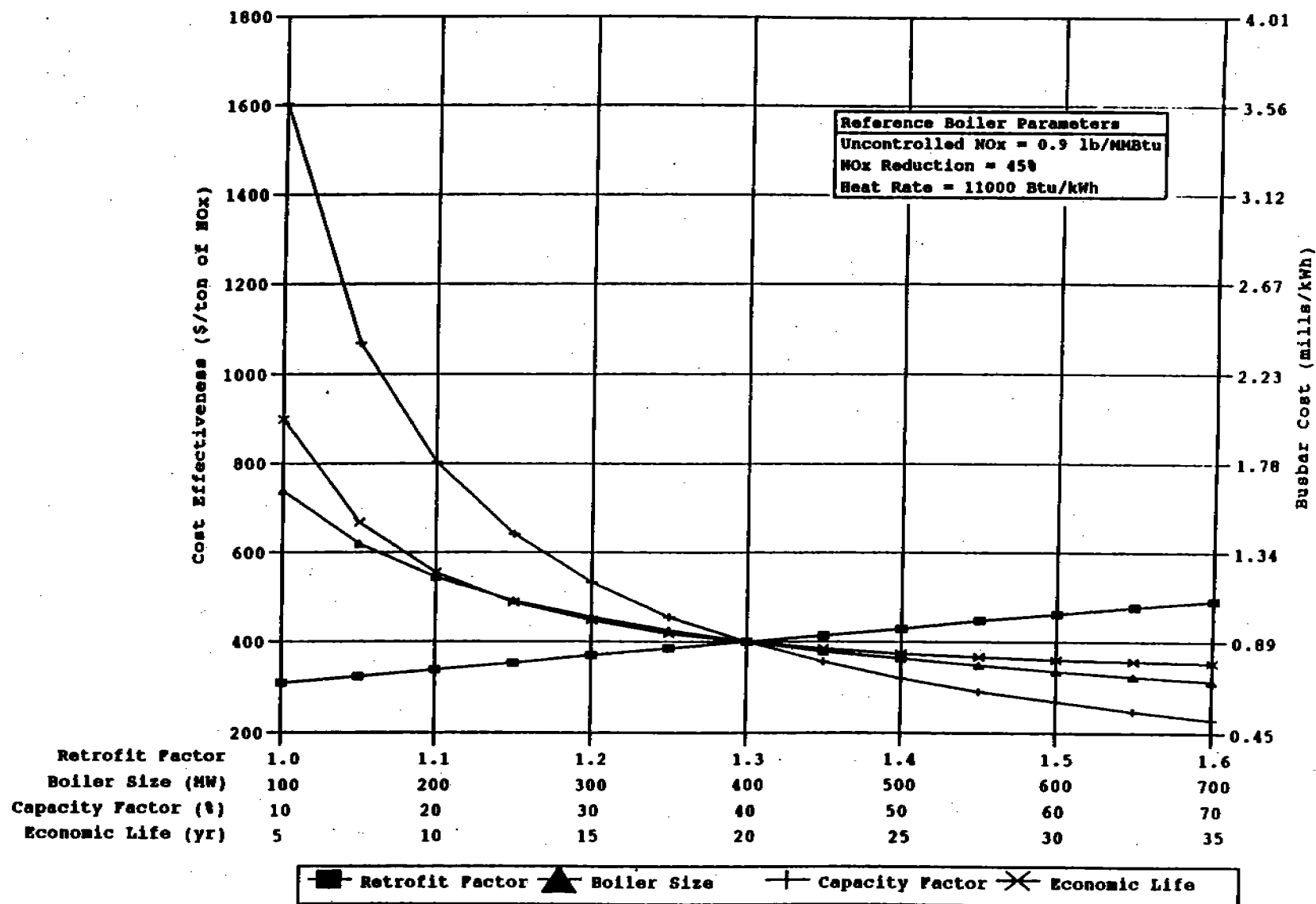
Figure 6-3. Impact of plant characteristics on LNB cost effectiveness and busbar cost for coal-fired wall boilers.
