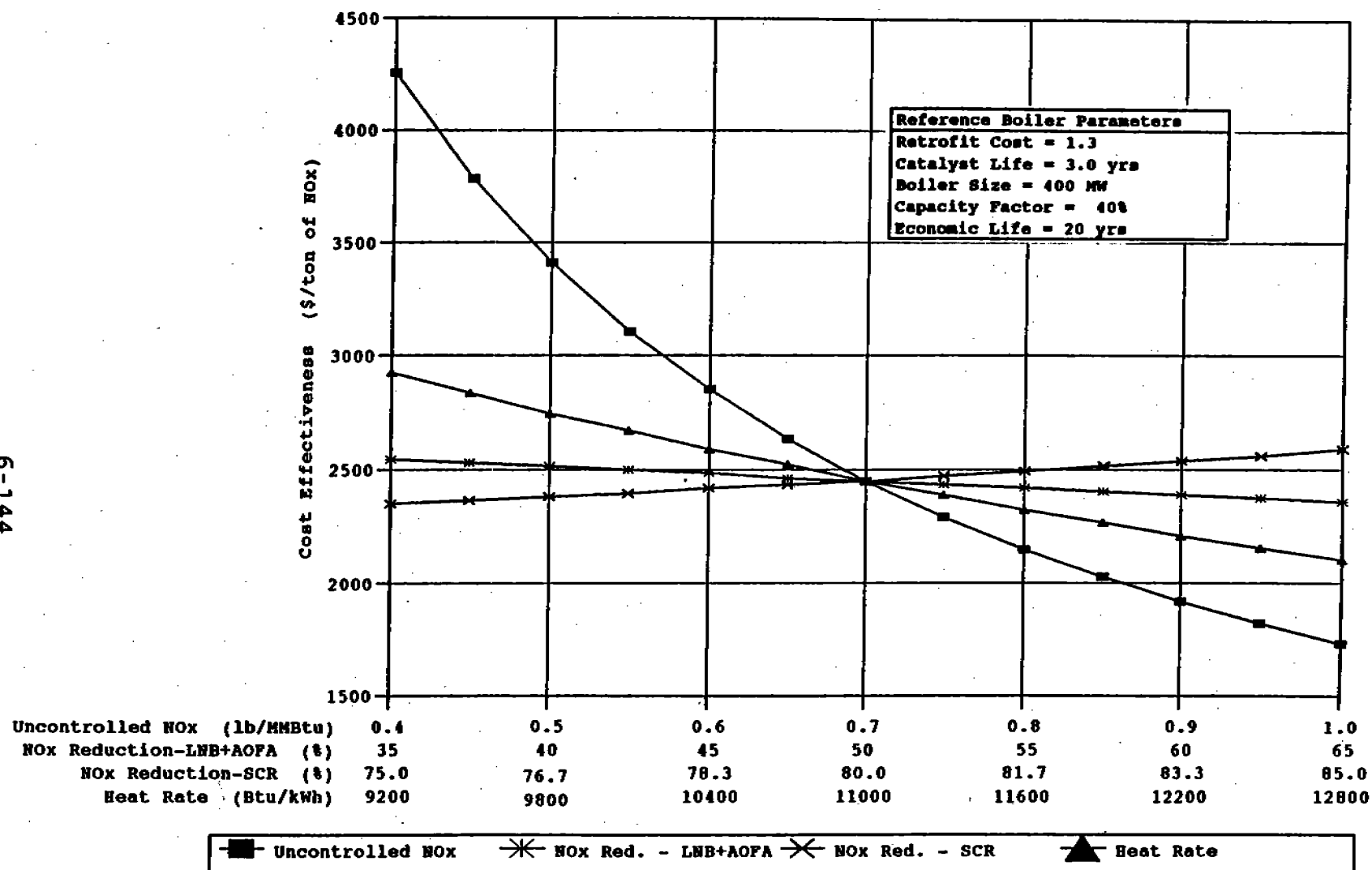
Figure 6-70. Impact of NO x emission characteristics and heat rate on LNB + AOFA + SCR cost effectiveness for coal-fired tangential boilers.
