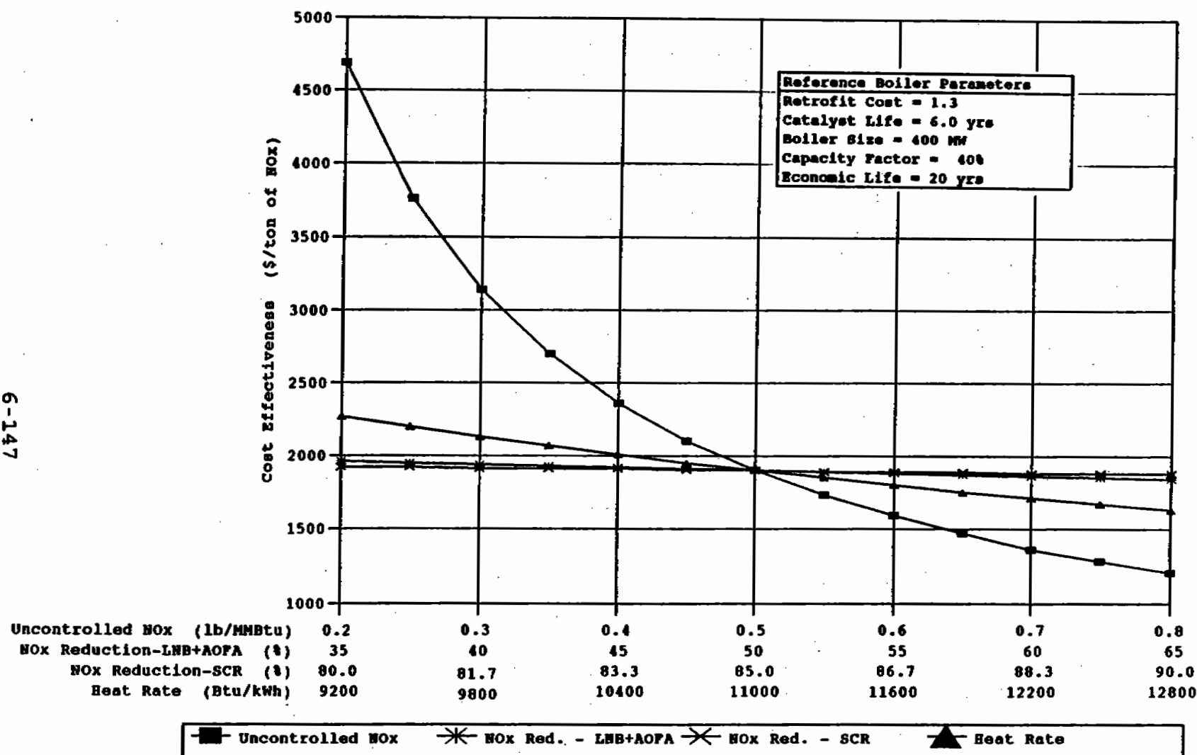
Figure 6-73. Impact of NO x emission characteristics and heat rate on LNB + AOFA + SCR cost effectiveness for natural gas-fired wall boilers.
