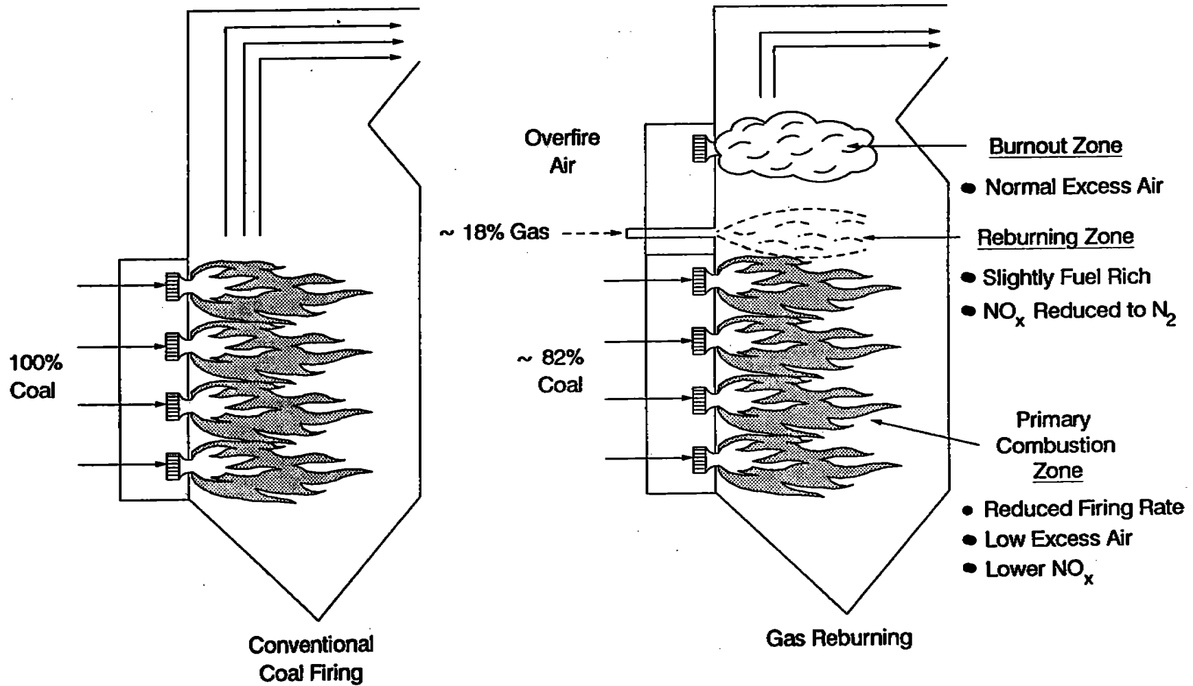
Figure 5-20. Application of natural gas reburn on a wall-fired boiler. 67
