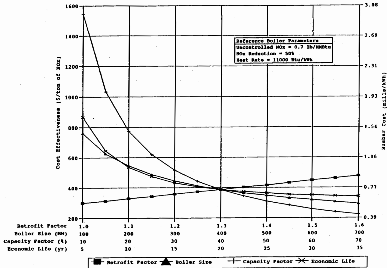
Figure 6-9. Impact of plant characteristics on LNB + AOFA cost effectiveness and busbar cost for coal-fired tangential boilers.
