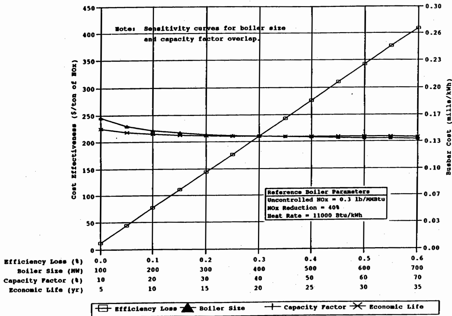
Figure 6-19. Impact of plant characteristics on LEA + BOOS cost effectiveness and busbar cost for natural gas- and oil-fired tangential boilers.
