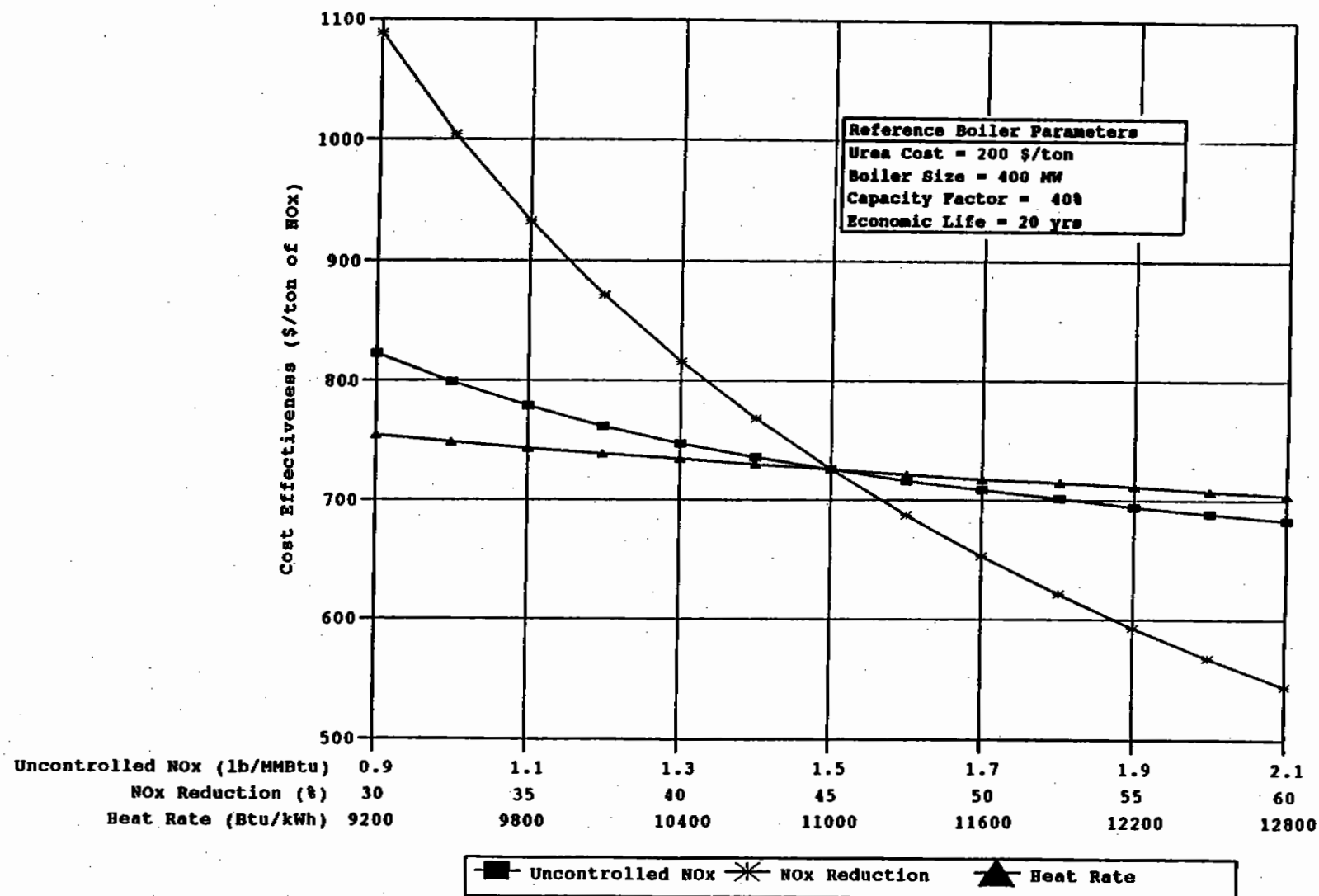
Figure 6-38. Impact of NO x emission characteristics and heat rate on SNCR cost effectiveness for coal-fired cyclone boilers.
