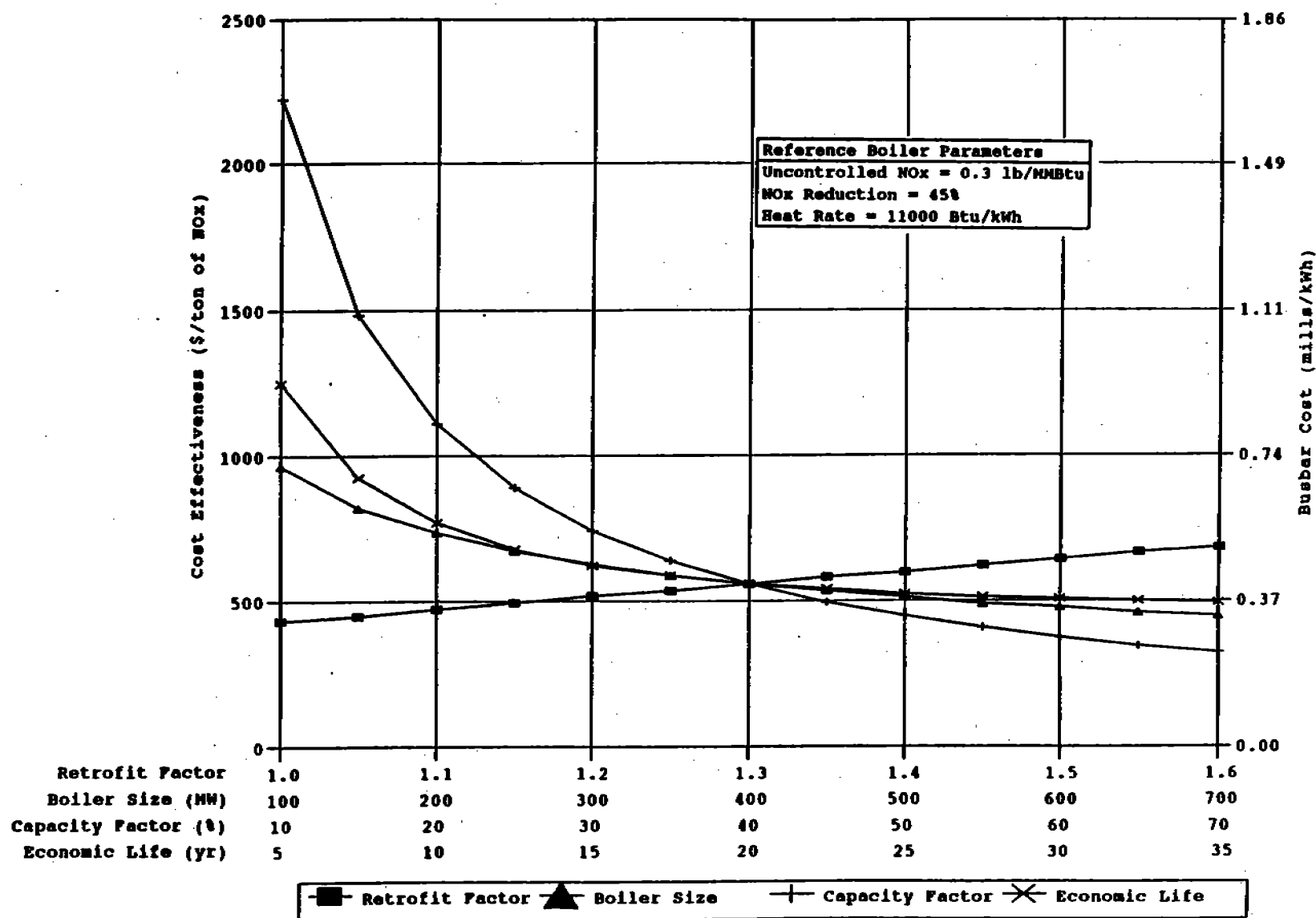
Figure 6-23. Impact of plant characteristics on LNB cost effectiveness and busbar cost for natural gas- and oil-fired tangential boilers.
