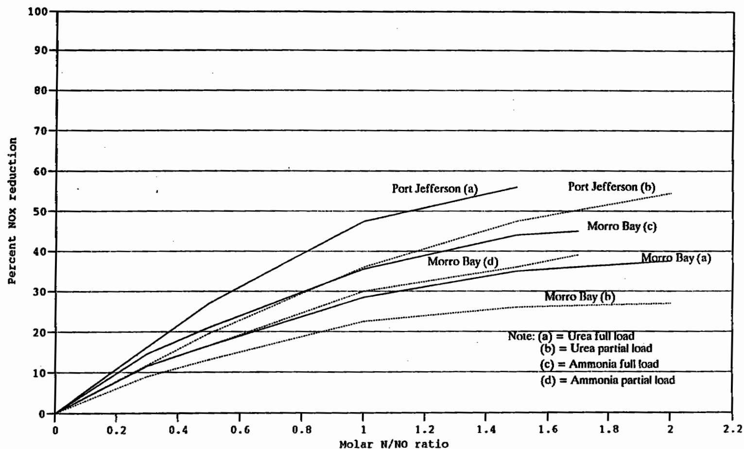
Figure 5-39. NO x reduction vs. Molar N/NO ratio for conventional U. S. natural gas- and oil-fired boilers with SNCR.
