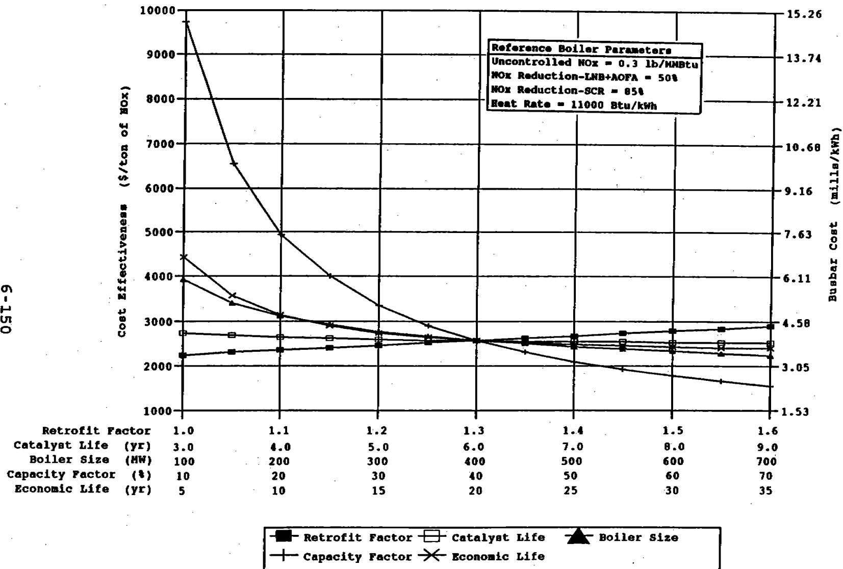
Figure 6-75. Impact of plant characteristics on LNB + AOFA + SCR cost effectiveness and busbar cost for natural gas-fired tangential boilers.
