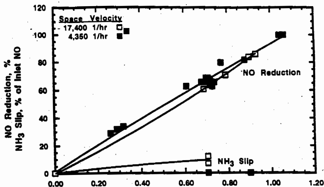
Figure 5-49a. \text{T}_1\text{O}_2 corrugated plate catalyst \text{NO}_x conversion and residual \text{NH}_3 versus \text{NH}_3 -to- \text{NO}_x ratio. 133
