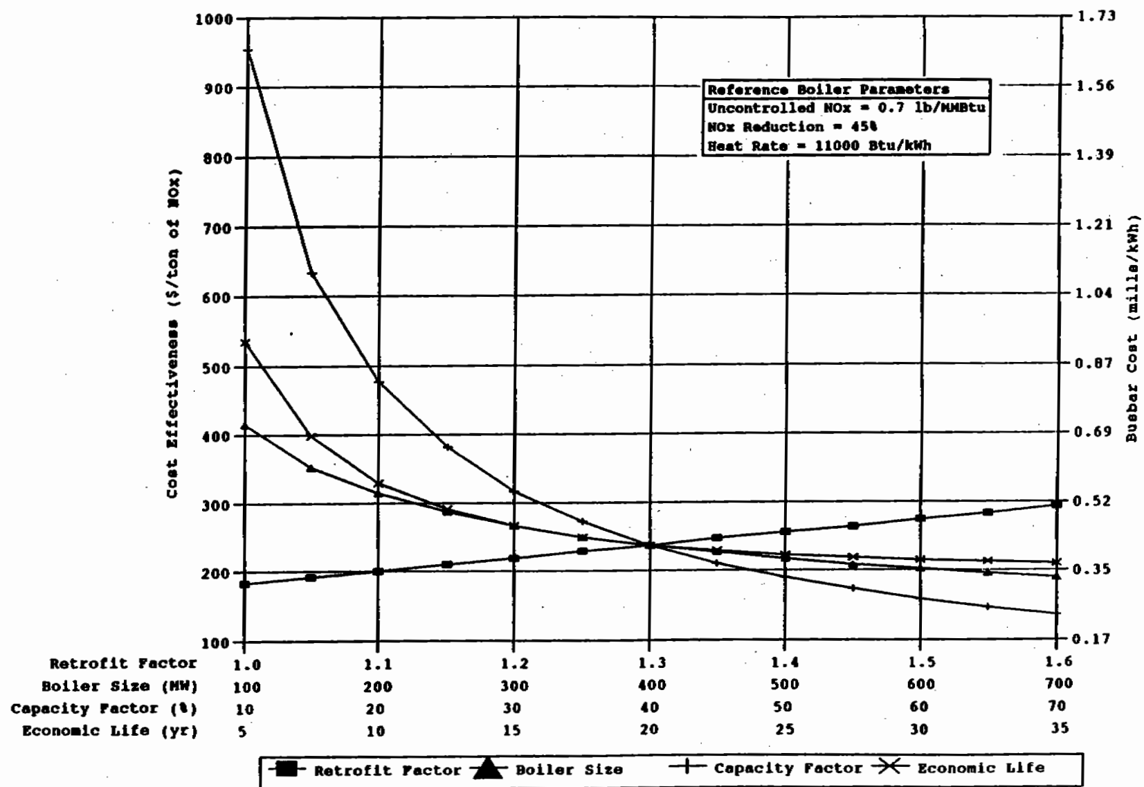
Figure 6-5. Impact of plant characteristics on LNB cost effectiveness and busbar cost for coal-fired tangential boilers.
