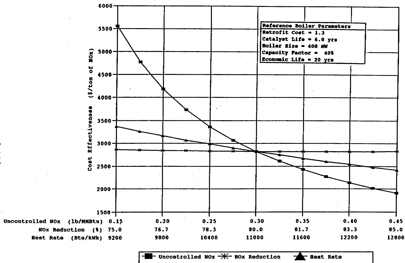
Figure 6-58. Impact of NO x emission characteristics and heat rate on SCR cost effectiveness for oil-fired tangential boilers.
