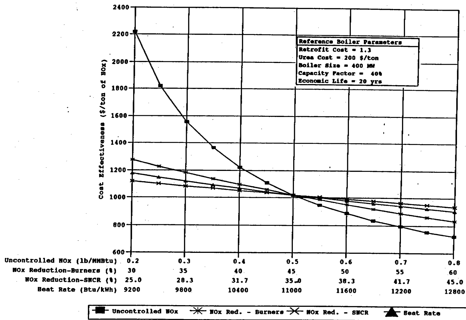
Figure 6-64. Impact of NO x emission characteristics and heat rate on LNB + SNCR cost effectiveness for natural gas- and oil-fired wall boilers.
