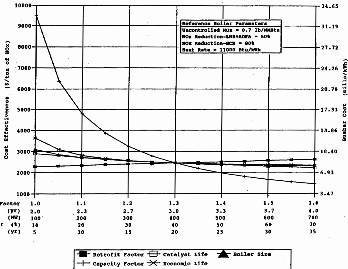
Figure 6-69. Impact of plant characteristics on LNB + AOFA + SCR cost effectiveness and busbar cost for coal-fired tangential boilers.
