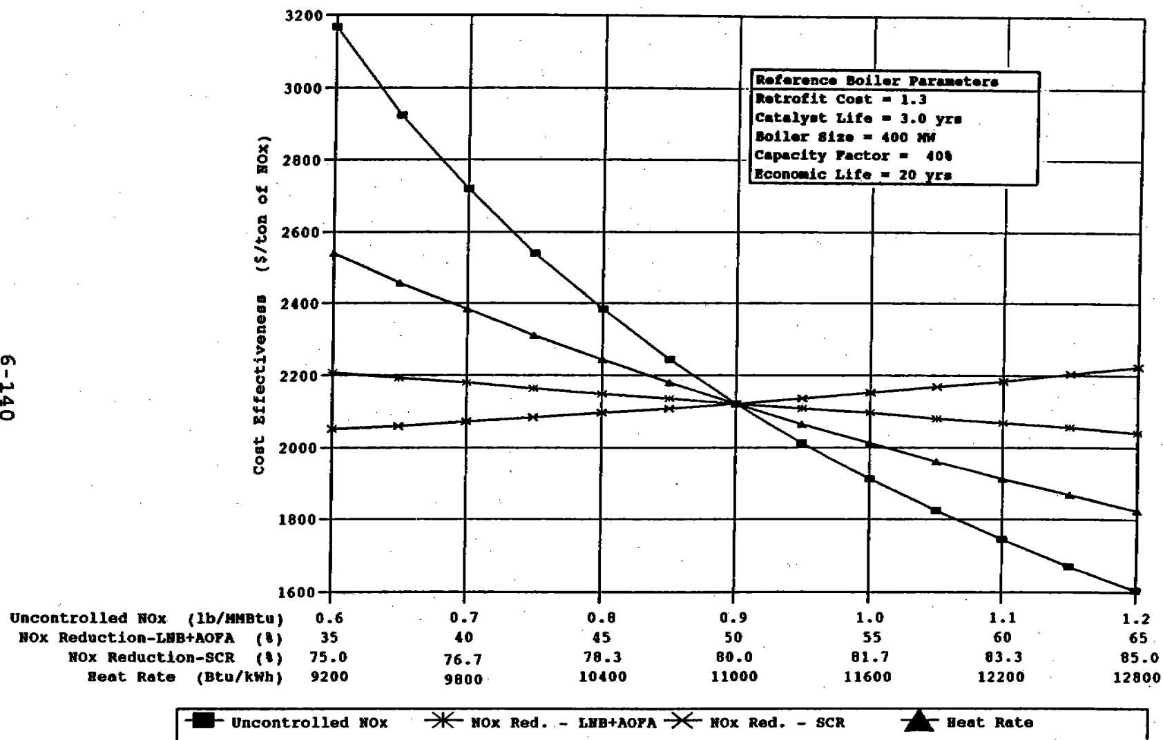
Figure 6-68. Impact of NO x emission characteristics and heat rate on LNB + AOFA + SCR cost effectiveness for coal-fired wall boilers.
