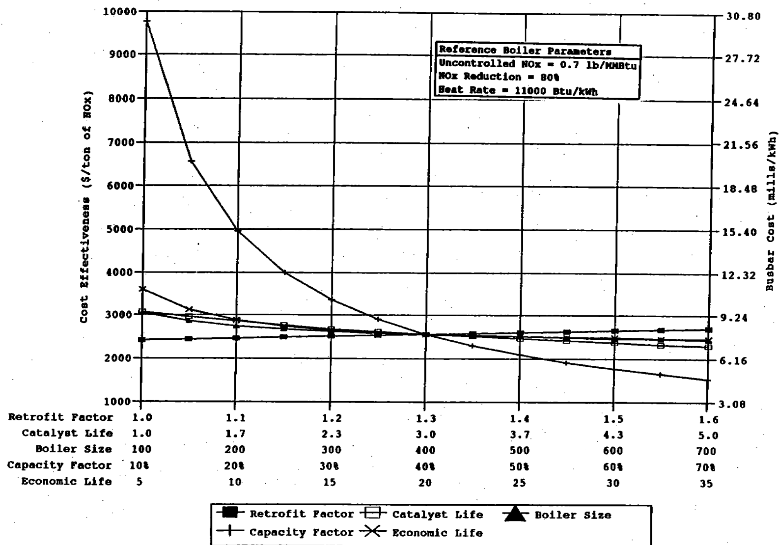
Figure 6-47. Impact of plant characteristics on SCR cost effectiveness and busbar cost for coal-fired tangential boilers.
