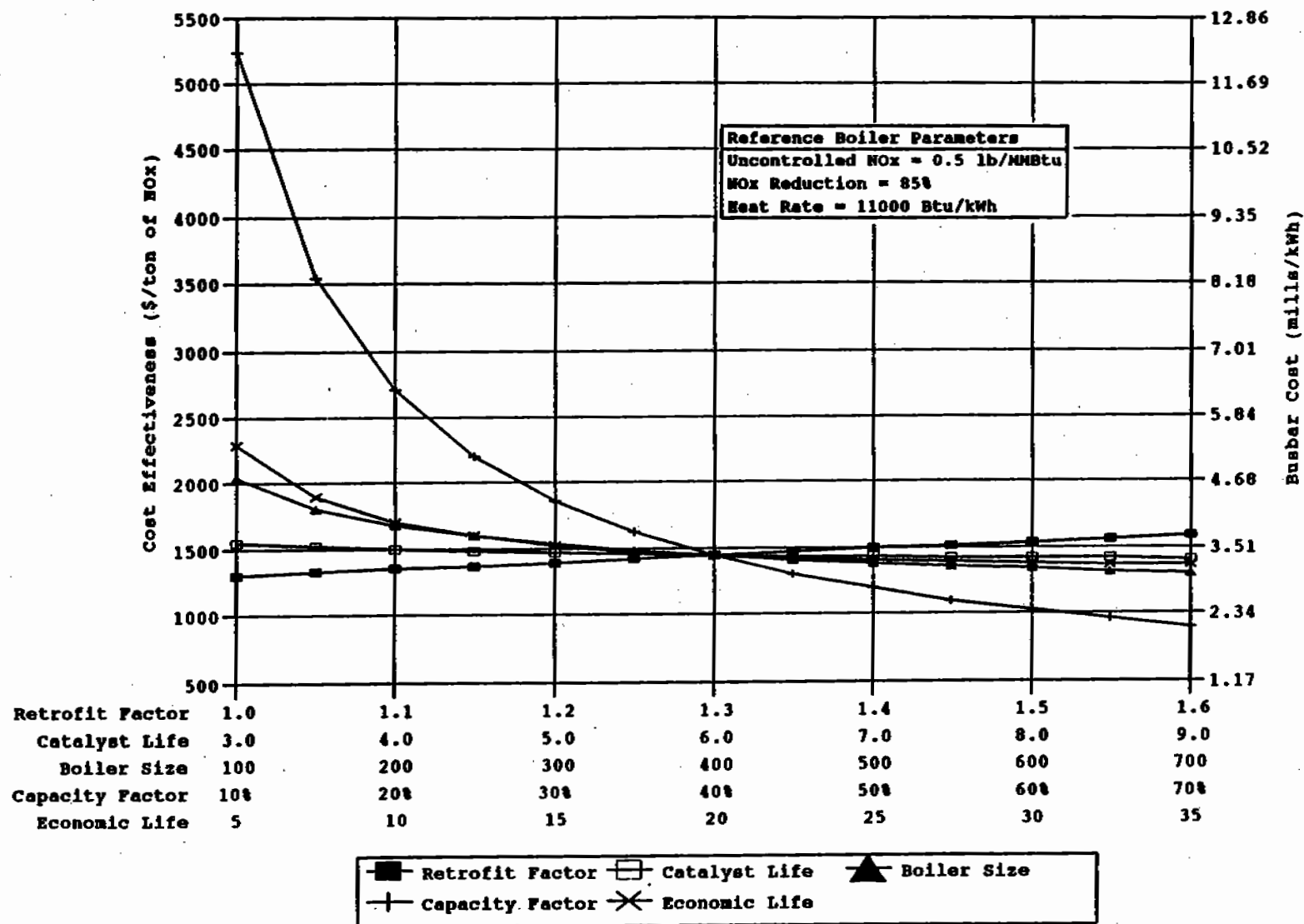
Figure 6-51. Impact of plant characteristics on SCR cost effectiveness and busbar cost for natural gas-fired wall boilers.
