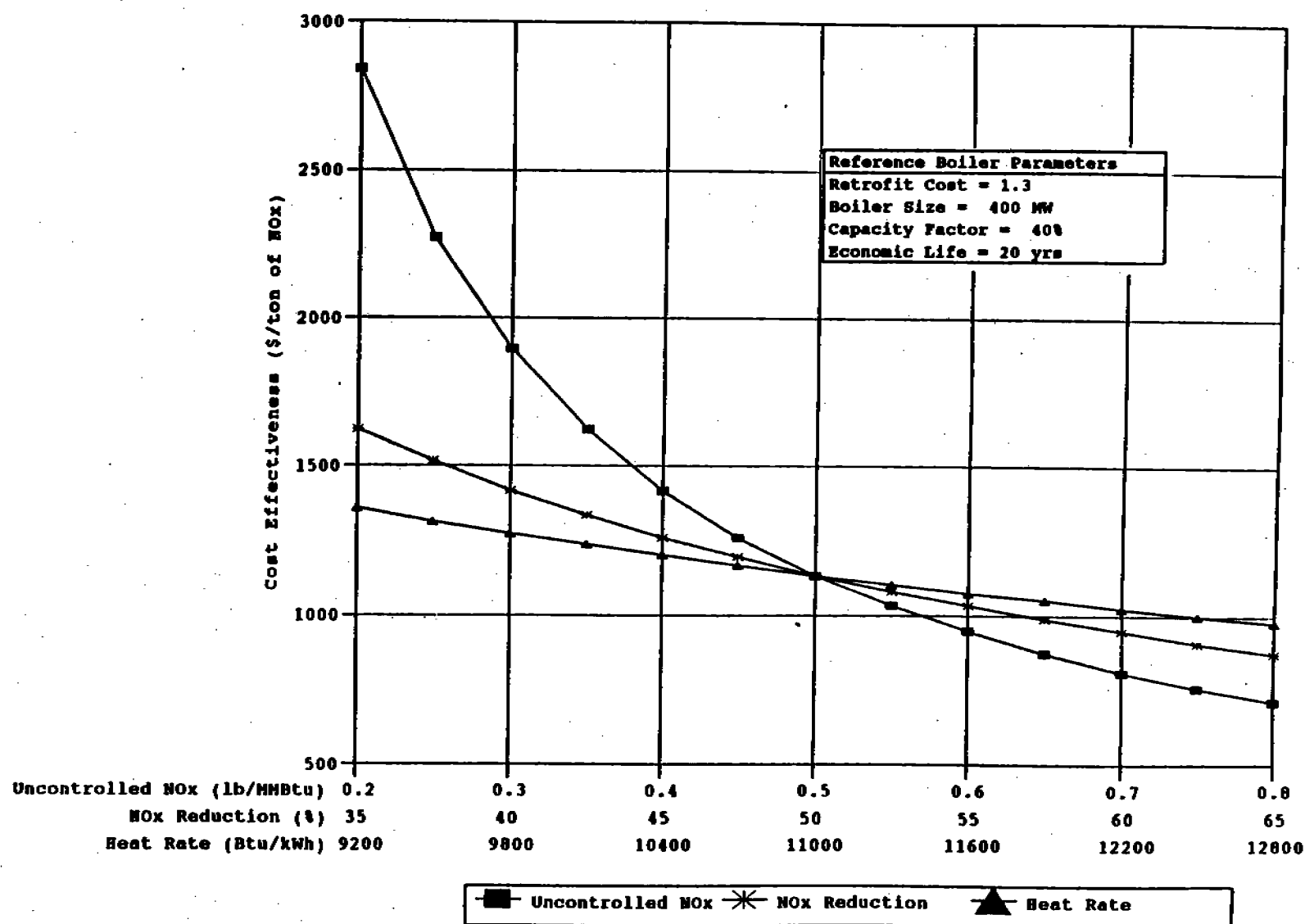
Figure 6-26. Impact of NO x emission characteristics and heat rate on LNB + AOFA cost effectiveness for natural gas- and oil-fired wall boilers.
