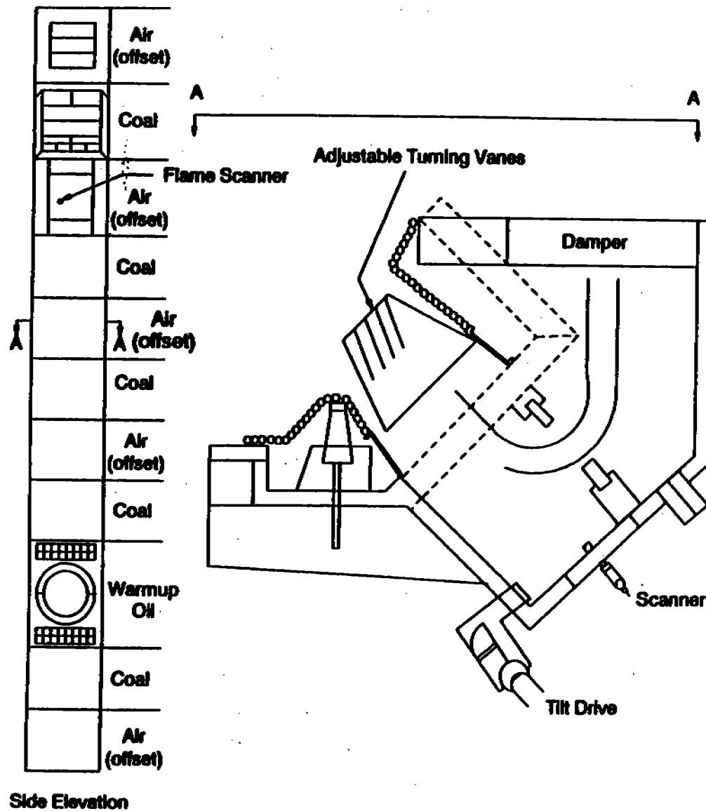
Figure 5-12a. Low NO x Concentric Firing System fuel and air compartment arrangement. 18
