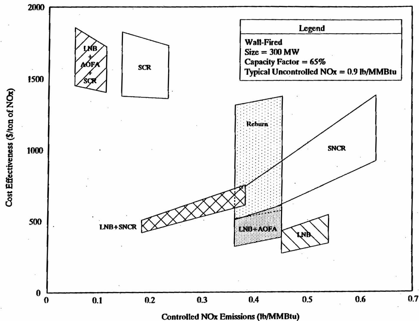
Figure 2-2. NO x control cost effectiveness for coal-fired wall boilers
