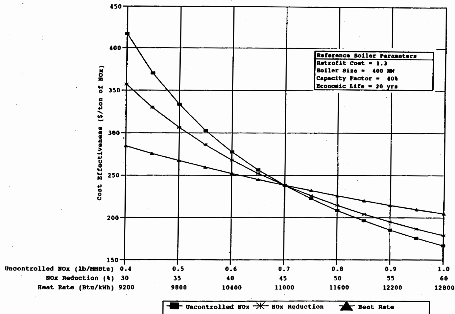
Figure 6-2. Impact of NO x emission characteristics and heat rate on LNB cost effectiveness for coal-fired tangential boilers.
