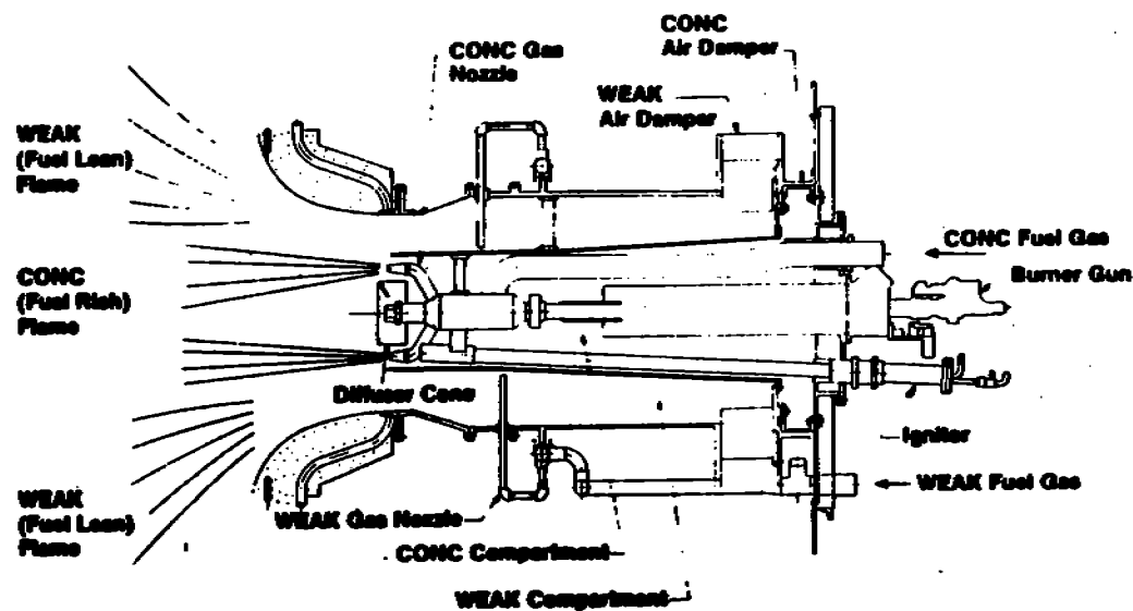
Schematic of Gas Firing ROPM Burner
