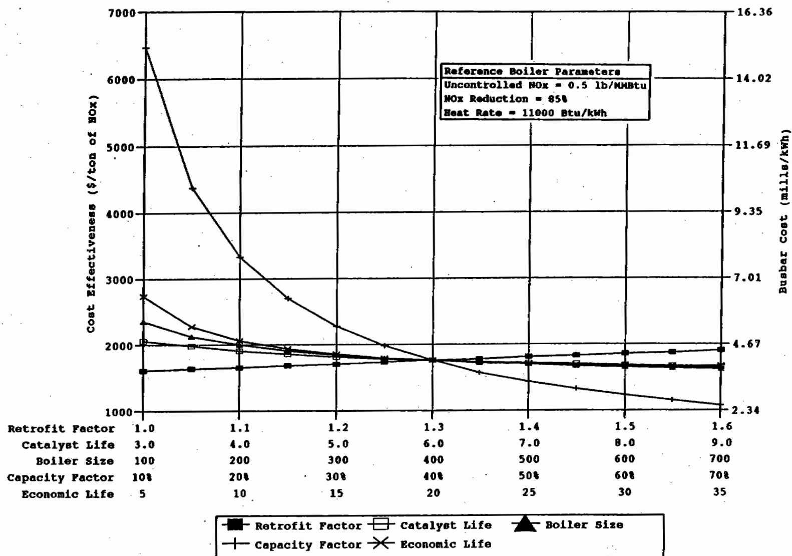
Figure 6-52. Impact of plant characteristics on SCR cost effectiveness and busbar cost for oil-fired wall boilers.
