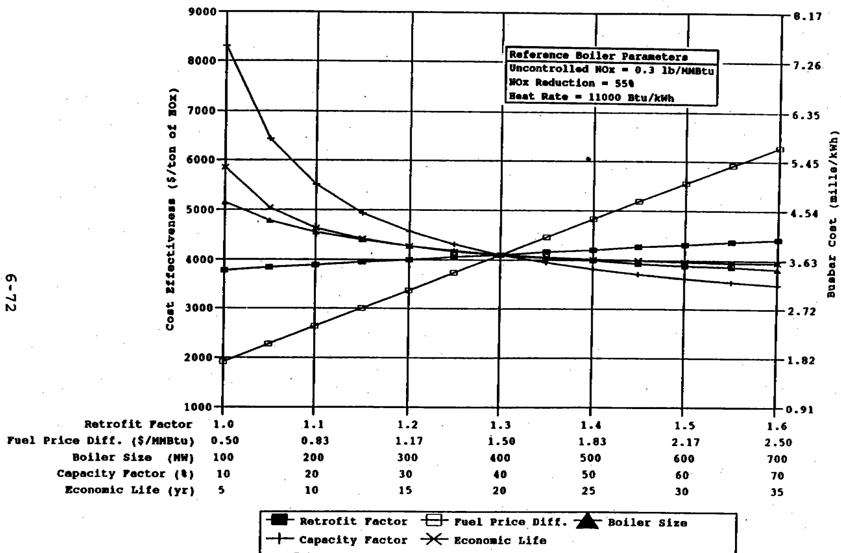
Figure 6-31. Impact of plant characteristics on NGR cost effectiveness and busbar cost for oil-fired tangential boilers.
