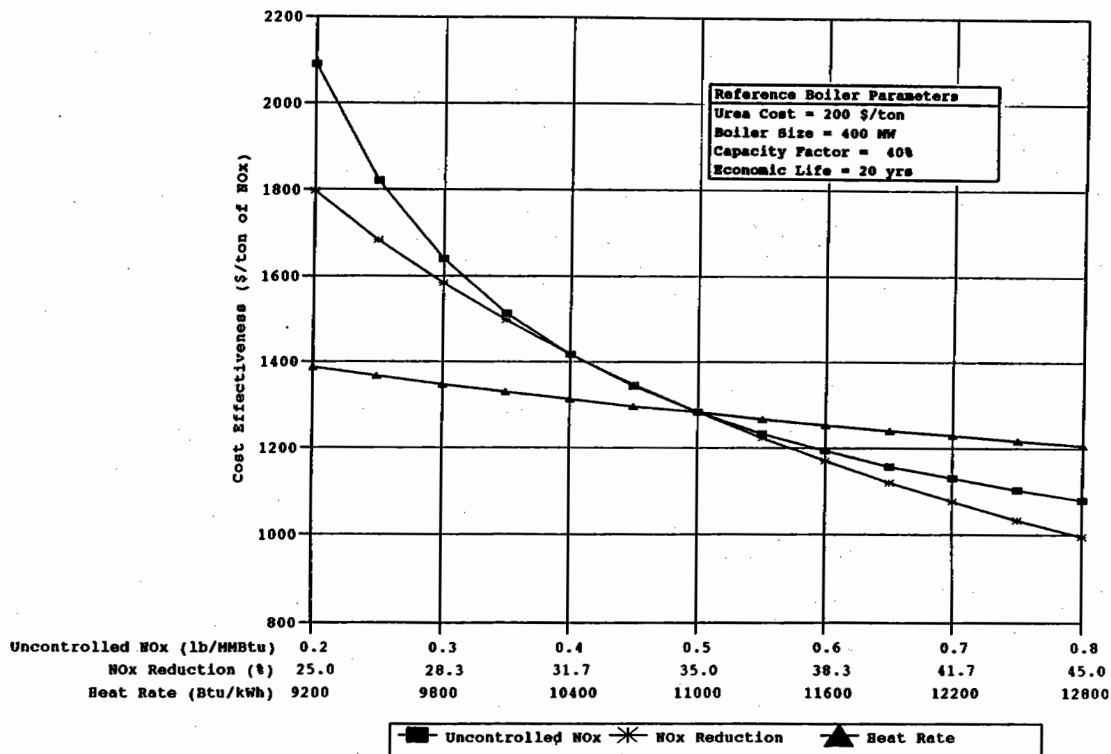
Figure 6-42. Impact of NO x emission characteristics and heat rate on SNCR cost effectiveness for natural gas- and oil-fired wall boilers.
