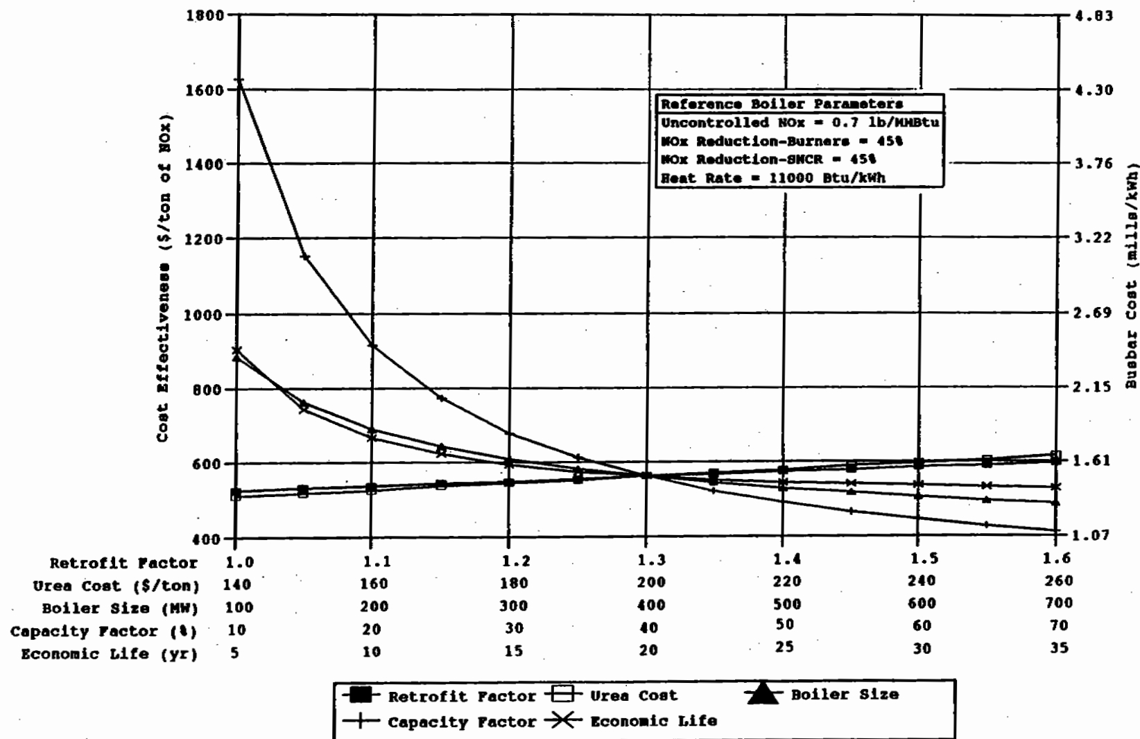
Figure 6-61. Impact of plant characteristics on LNB + SNCR cost effectiveness and busbar cost for coal-fired tangential boilers.
