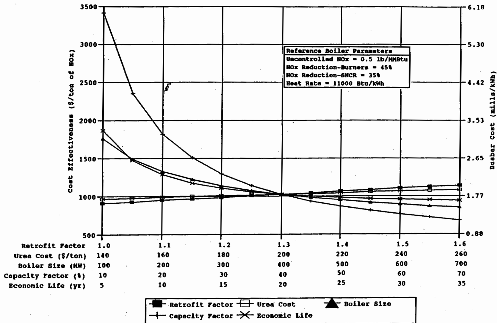
Figure 6-63. Impact of plant characteristics on LNB + SNCR cost effectiveness and busbar cost for natural gas- and oil-fired wall boilers.
