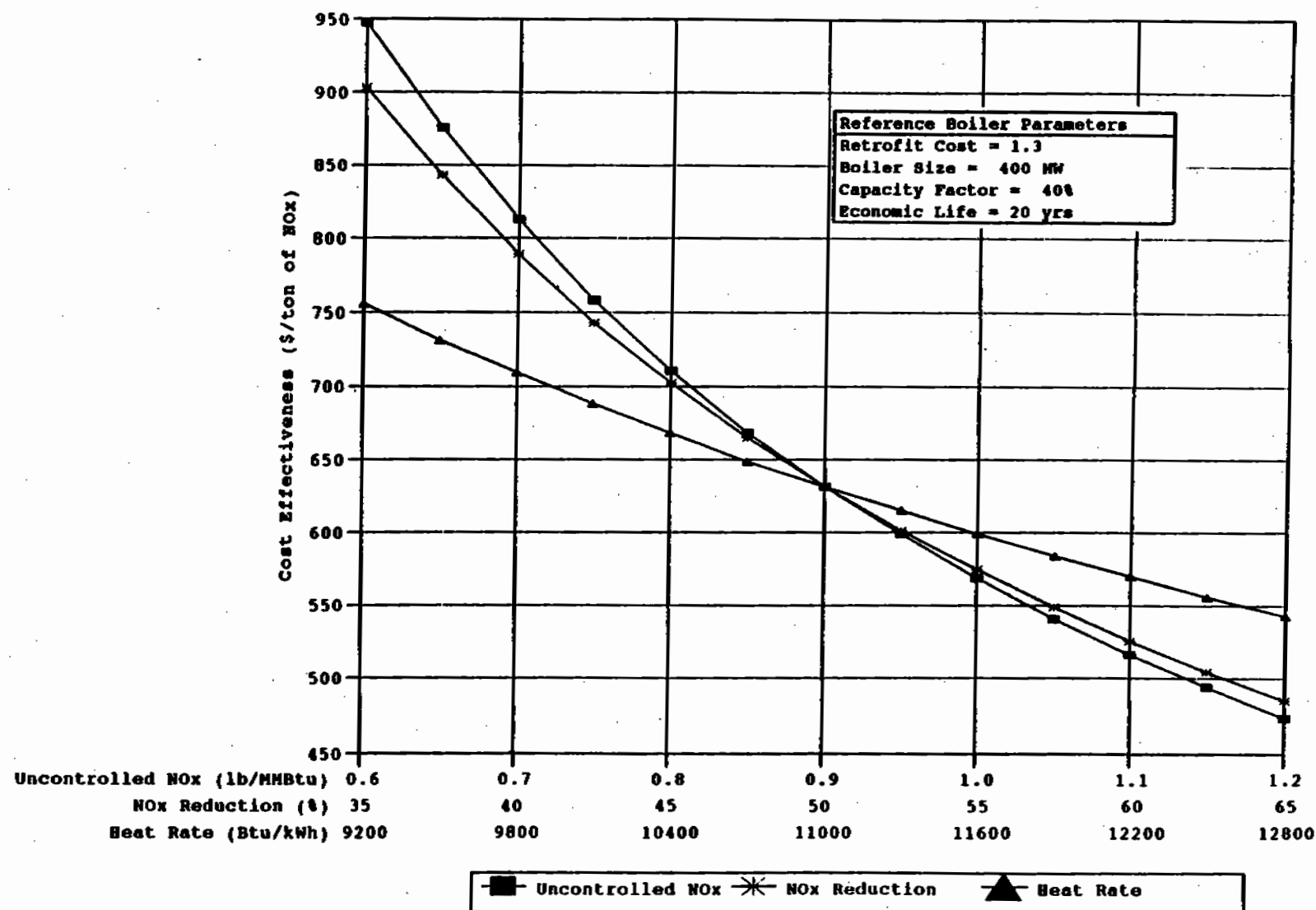
Figure 6-8. Impact of NO x emission characteristics and heat rate on LNB + AOFA cost effectiveness for coal-fired wall boilers.
