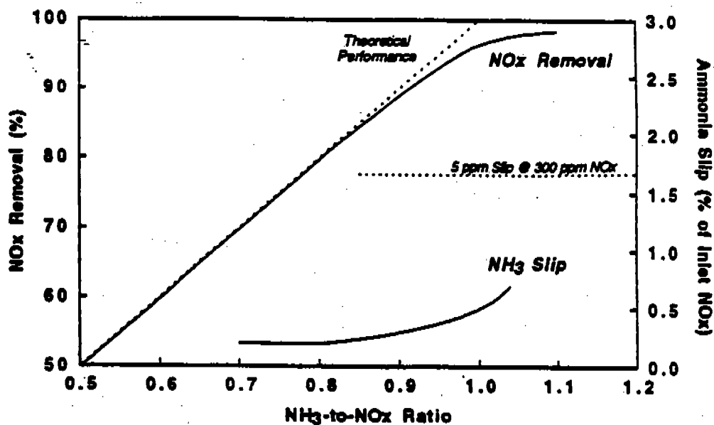
Figure 5-47a. Extruded catalyst \text{NO}_x conversion and residual \text{NH}_3 versus \text{NH}_3 -to- \text{NO}_x Ratio. 131
