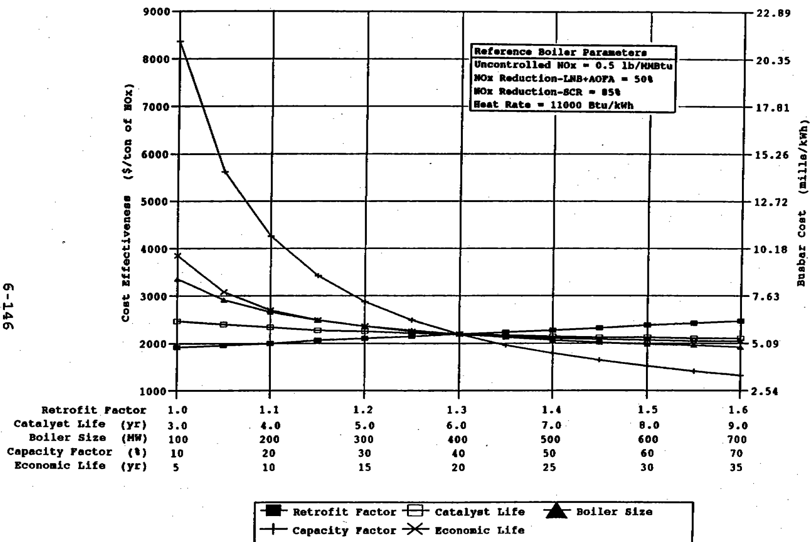
Figure 6-72. Impact of plant characteristics on LNB + AOFA + SCR cost effectiveness and busbar cost for oil-fired wall boilers.
