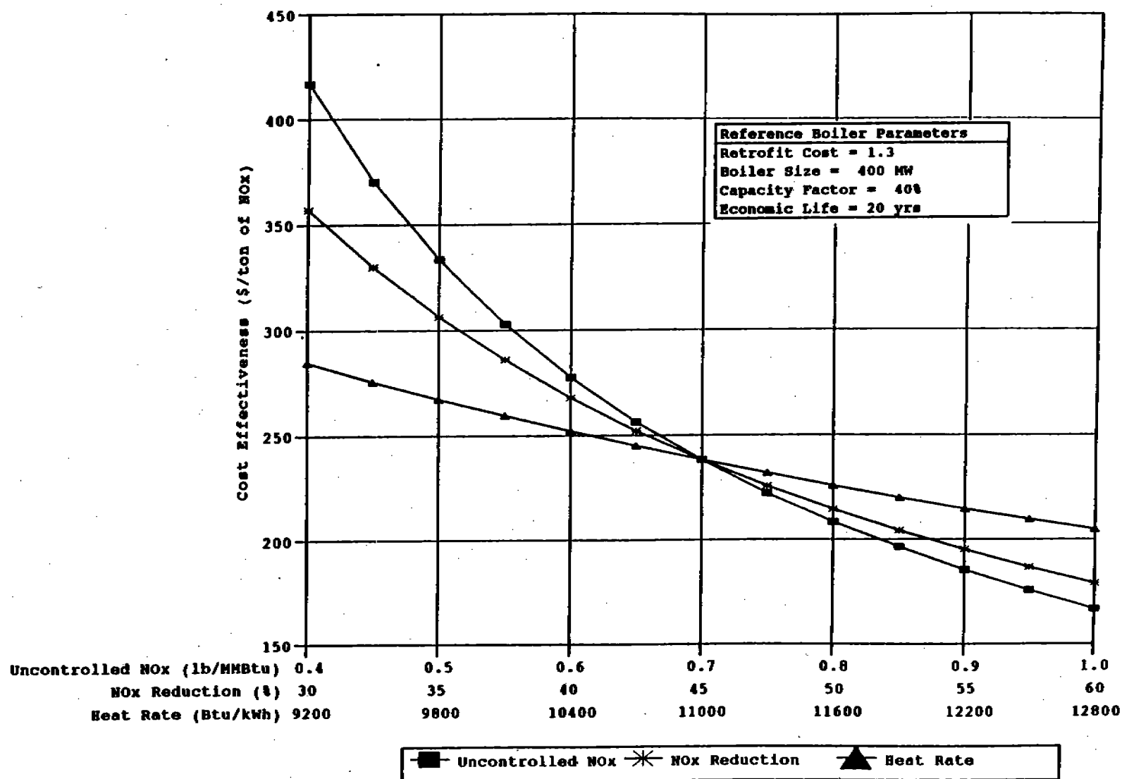
Figure 6-6. Impact of NO x emission characteristics and heat rate on LNB cost effectiveness for coal-fired tangential boilers.
