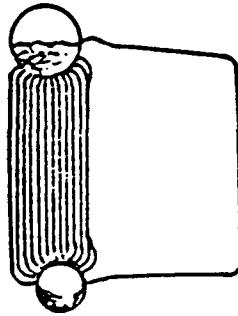
Figure 3-19. Watertube design configurations. 44
