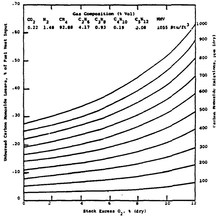
Figure 7-4. Unburned carbon monoxide loss as a function of excess O 2 and carbon monoxide emissions for natural gas fuel. 28
