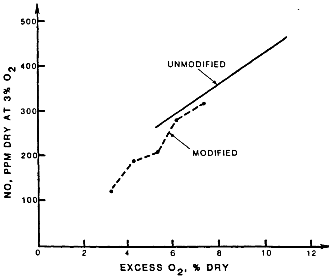
Figure 5-10. NO emission versus excess O 2 , stoker boiler with FGR. 27
