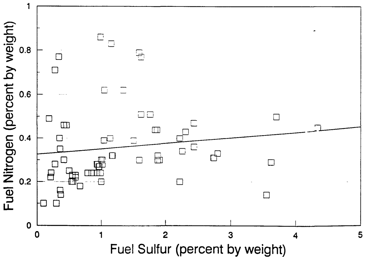
Figure 4-2. Fuel oil nitrogen versus sulfur for residual oil. (Data from several EPA- and EPRI-sponsored tests; see Table 4-1.)
