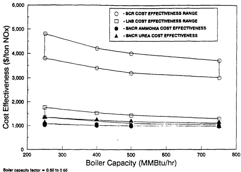
Figure 2-1. Cost effectiveness versus boiler capacity, PC wall-fired boilers.
