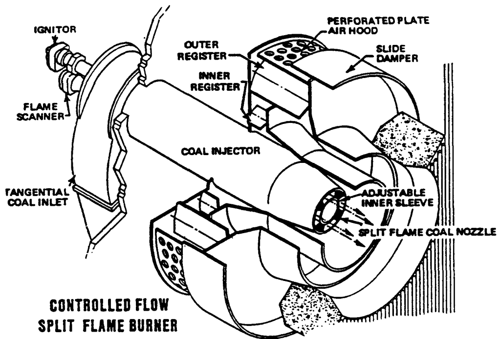
Figure 5-4. Foster Wheeler CF/SF LNB. 9
