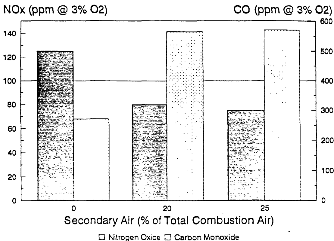
Figure 5-12. Effect of SCA on NO x and CO emissions, Chalmers University. 34
