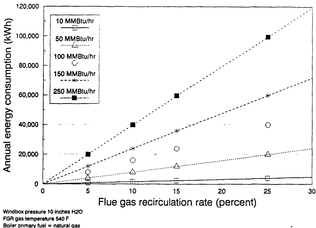
Figure 7-6. Estimated energy consumption in FGR use.
