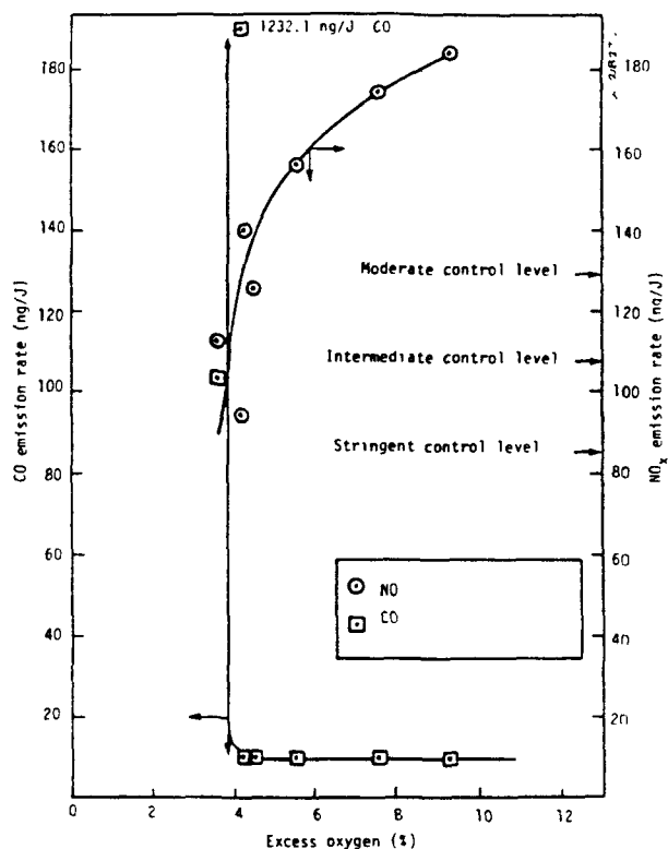
Figure 5-2. Changes in CO and NO x emissions with reduced excess oxygen for a residual oil-fired watertube industrial boiler. 5
