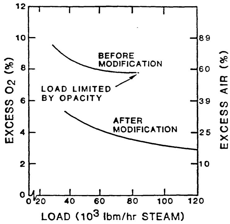
Figure 5-9. FGR effects on excess O 2 . 27
