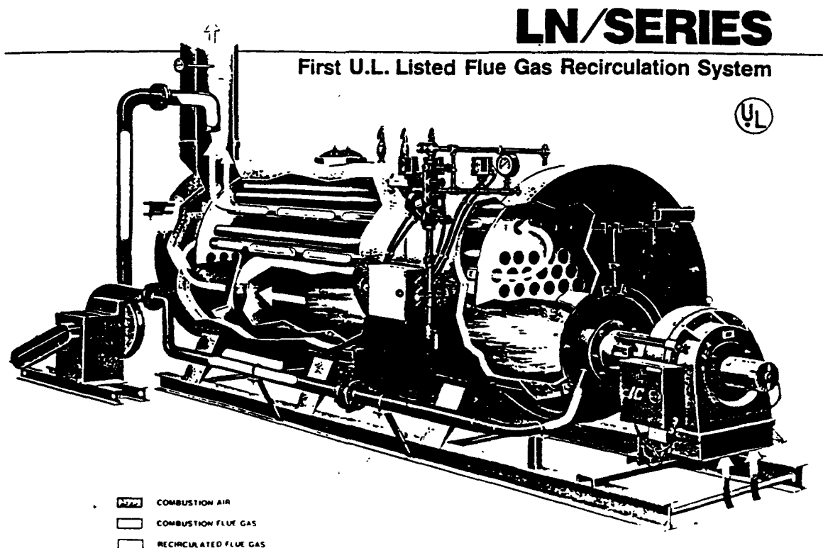
Figure 5-22. FGR system for gas- or oil-fired boiler. 71
