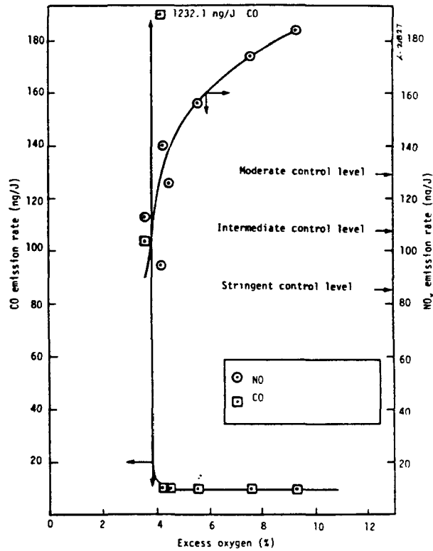
Figure 7-1. Changes in CO and NO x emissions with reduced excess oxygen for a residual-oil-fired watertube industrial boiler. 17
