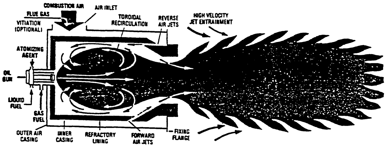
Figure 5-25. Process Combustion Corporation toroidal combustor. 90
