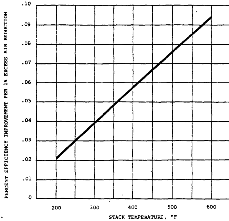
Figure 7-3. Curve showing percent efficiency improvement per every 1 percent reduction in excess air. Valid for estimating efficiency improvements on typical natural gas, No. 2 through No. 6 oils, and coal fuels. 25
