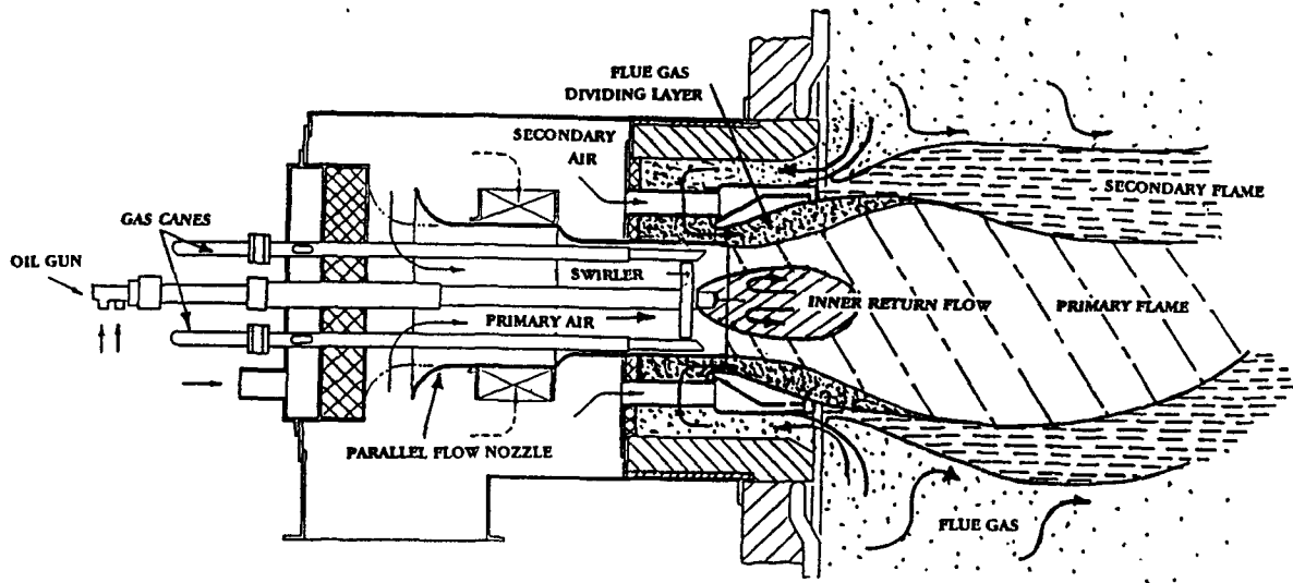
Figure 5-18. Low-NO x ASR burner. 59
