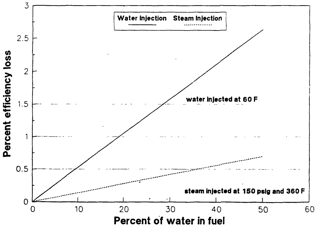
Figure 7-5. Energy penalty associated with the use of WI or SI for NO x control in ICI boilers.
