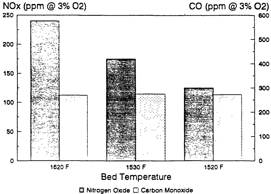
Figure 5-14. Effect of bed temperature on NO x and CO, Chalmers University. 34
