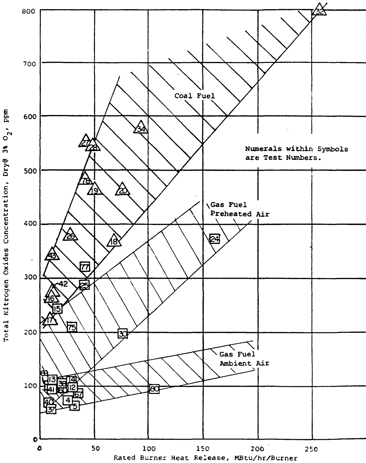
Figure 4-5. Effect of burner heat release rate on NO x emissions for coal and natural gas fuels. 16
