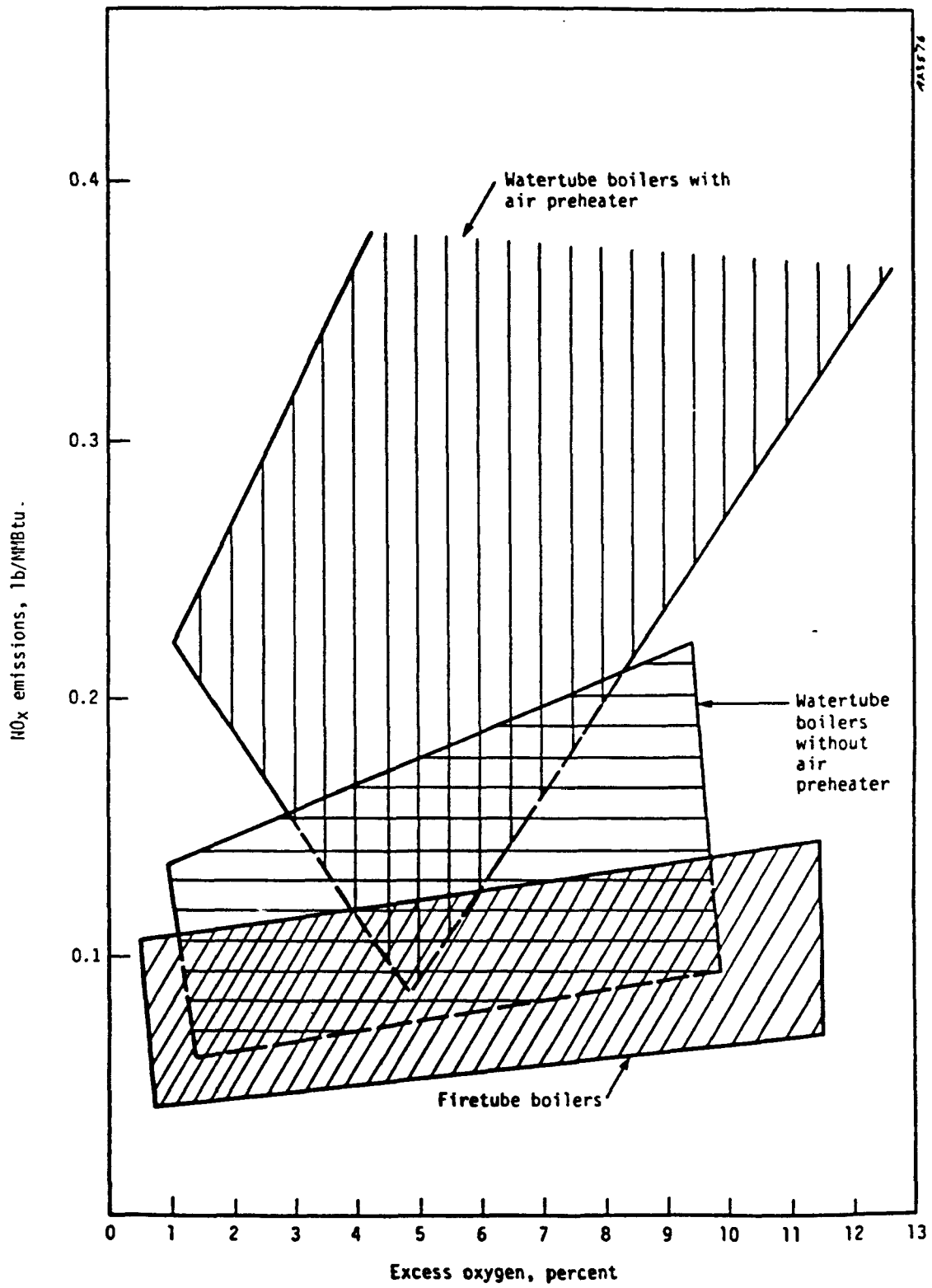
Figure 4-7. Effect of excess oxygen and preheat on NO x emissions, natural-gas-fired boilers. 39
