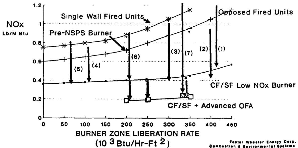
Figure 5-5. Performance of CF/SF LNB. 10
