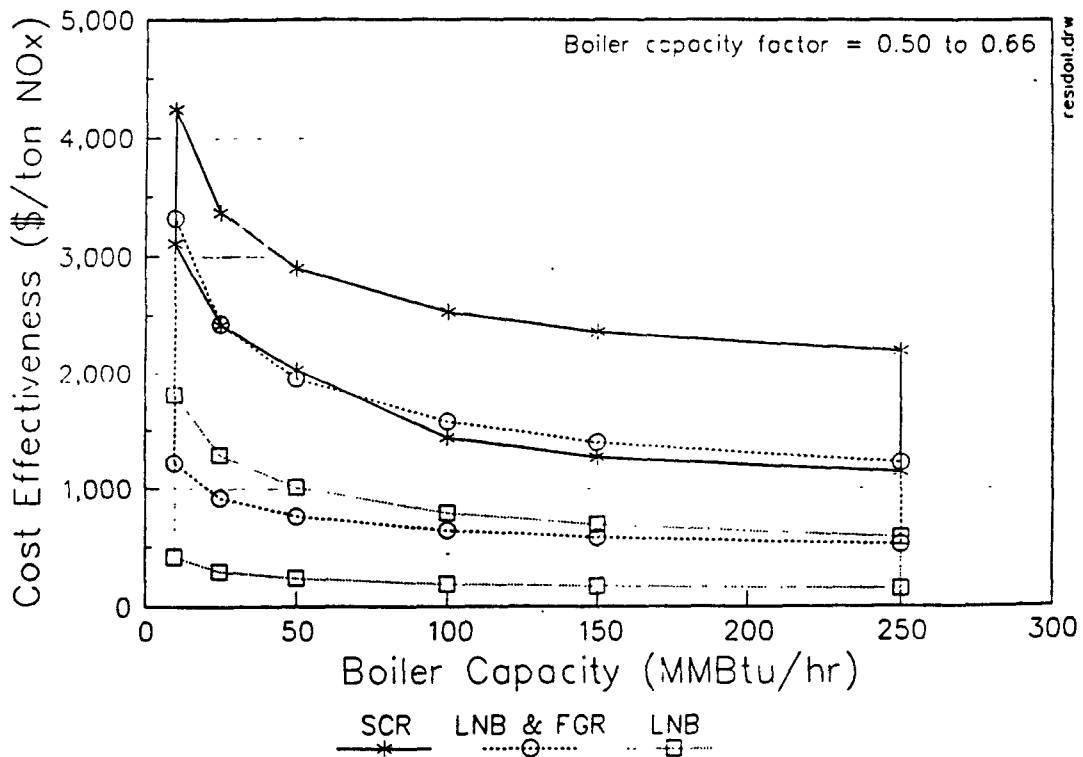
Figure 2-4. Cost effectiveness versus boiler capacity, residual-oil-fired boilers.
