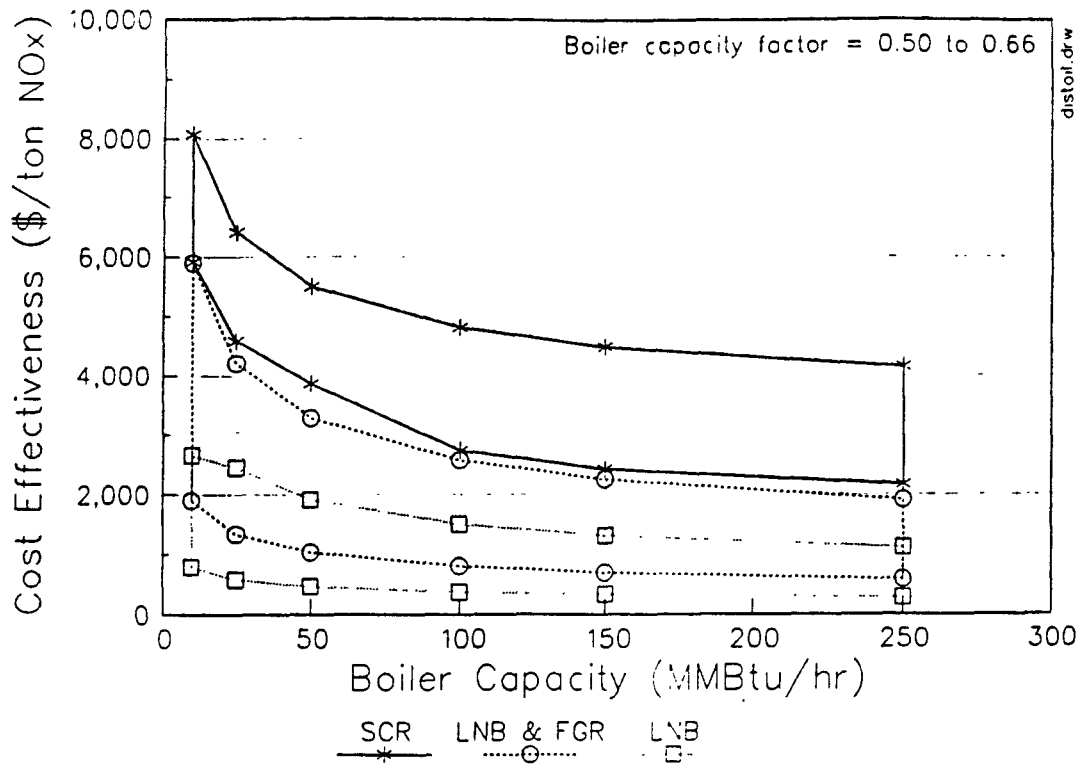
Figure 2-3. Cost effectiveness versus boiler capacity, distillate-oil-fired boilers.
