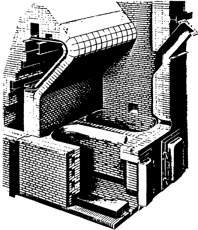
Figure 3-24. Ward fuel cell furnace. 56
