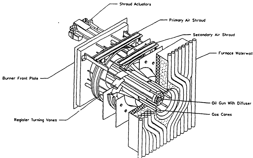
Figure 5-20. Riley Stoker STS burner. 59
