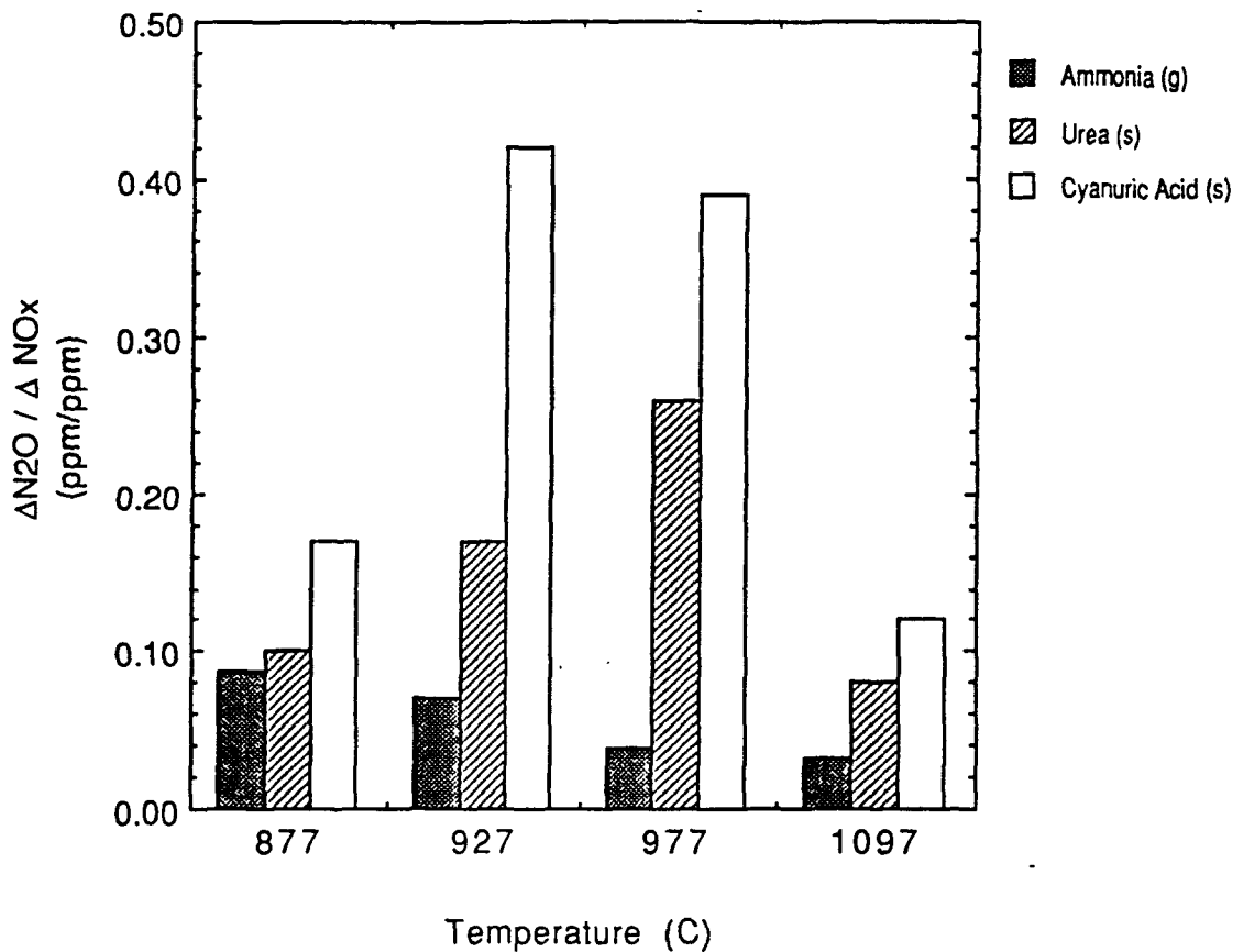
Figure 7-2. Pilot-scale test results, conversion of NO x to N 2 O (NO i = 300 ppm, N/NO = 2.0). 20
