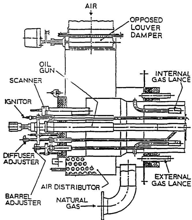
Figure 5-19. AFS air- and fuel-staged burner. 59
