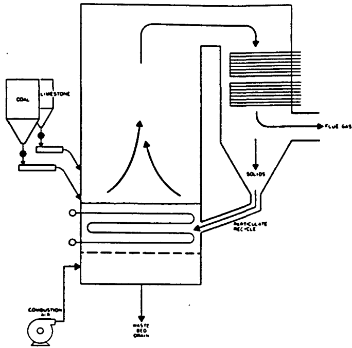
Figure 3-13. Bubbling FBC schematic. 32
