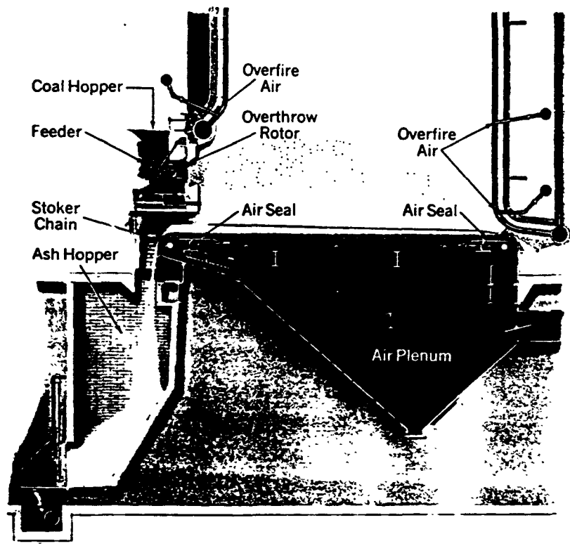
Figure 3-10. Spreader stoker. 21
