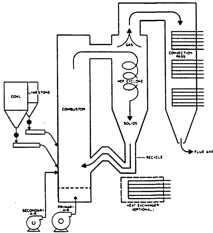
Figure 3-14. Circulating FBC schematic. 32
