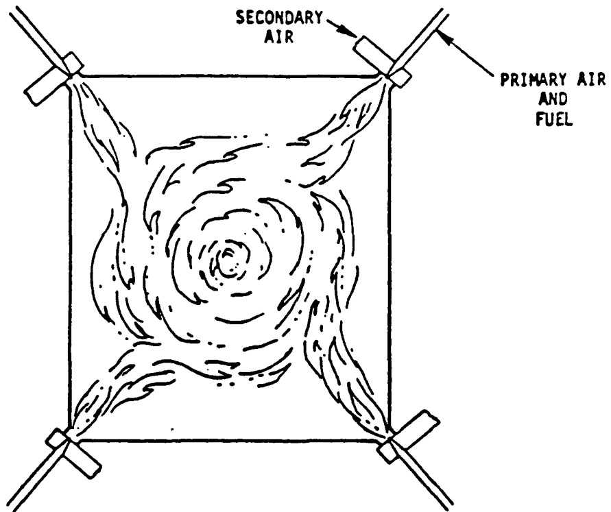
Figure 3-12. Tangential firing. 26
