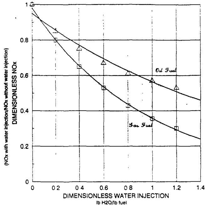
Figure 5-15. As the rate of water injection increases, NO x decreases. 48
