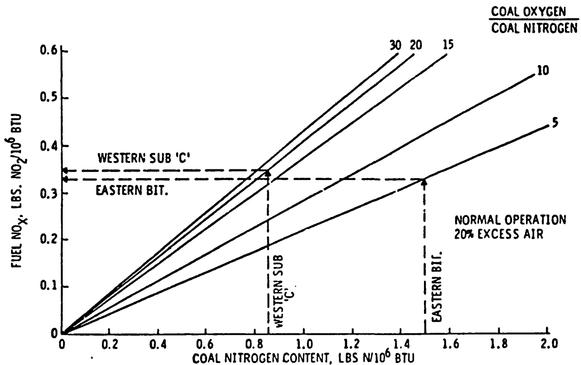
Figure 4-4. Fuel NO x formation as a function of coal oxygen/nitrogen ratio and coal nitrogen content. 21
