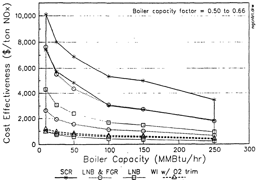
Figure 2-2. Cost effectiveness versus boiler capacity, natural-gas-fired packaged watertube boilers.
