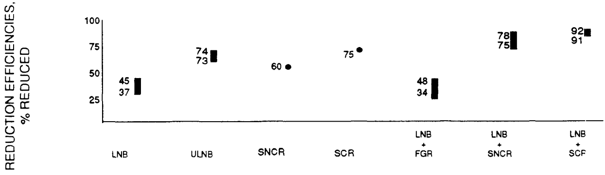
Figure 2-4. Model heaters: NO x emission reductions, capital costs, and cost effectiveness at a capacity factor of 0.9 for MD, oil-fired, low- and medium-temperature heaters.
