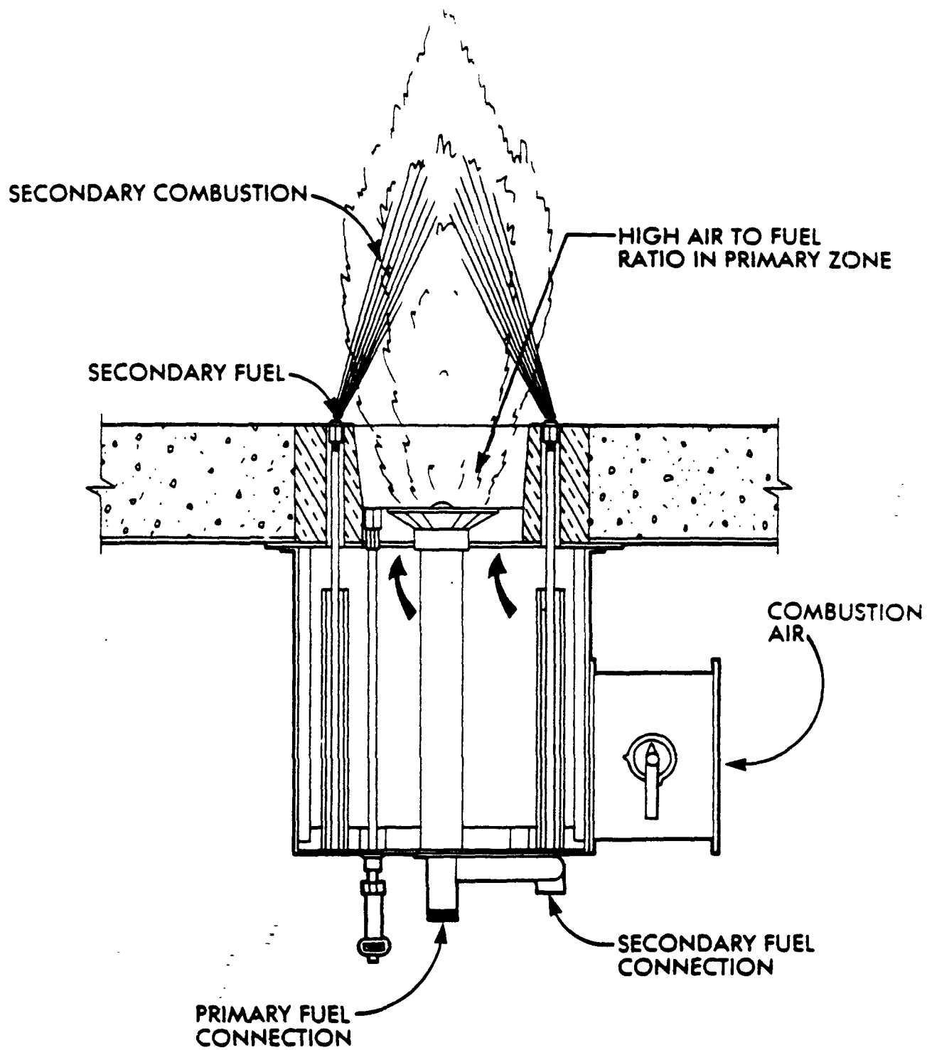
Figure 5-4. Schematic of a staged-fuel low- \text{NO}_x burner. 1
