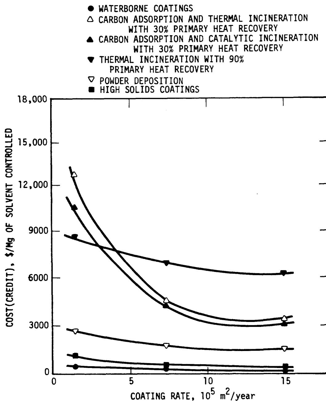
FIGURE 3-3. Cost-Effectiveness Comparison of Solvent Emission Control Options
