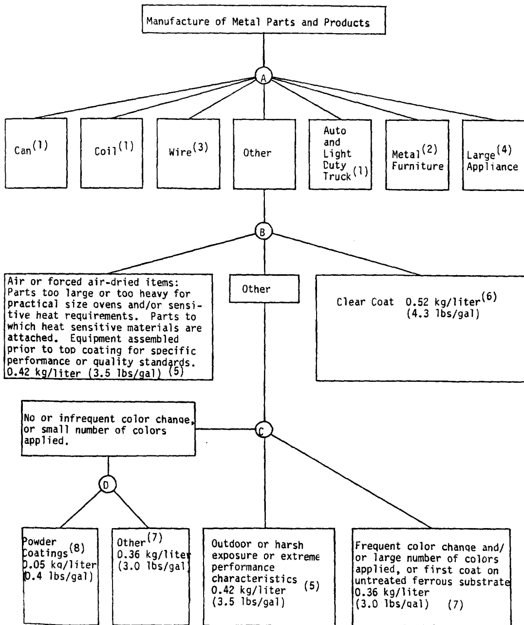
Figure 4.1 Logic diagram for derivation of emission limits for coating of miscellaneous metal parts and products.
