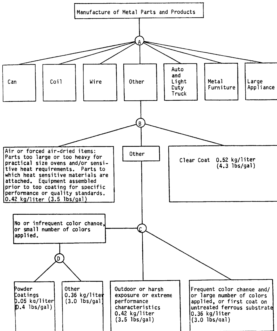
Logic diagram for derivation of emission limits for coating of miscellaneous metal parts and products.
