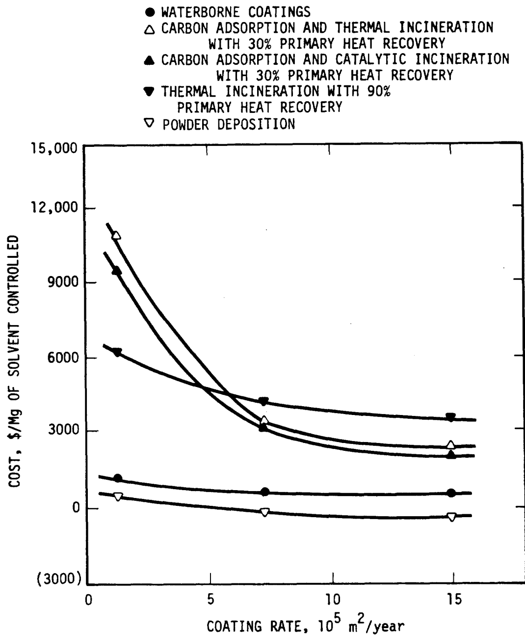
FIGURE 3-4. Cost-Effectiveness Comparison of Solvent Emission Control Options
