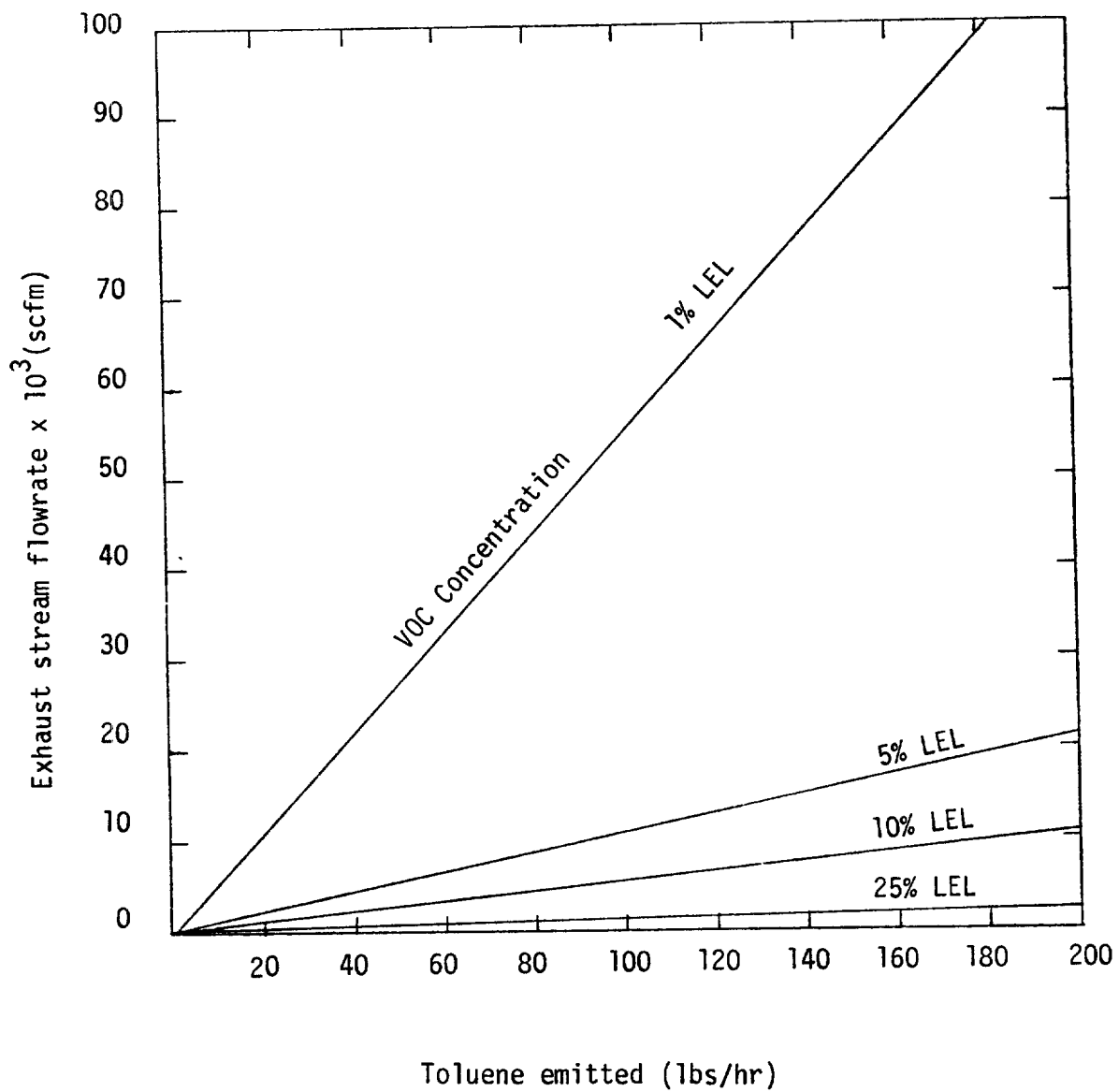
Figure 1-2. Data for toluene, LEL = 1.2% ( V/V_v ), showing the relationship between VOC emission, exhaust flowrate and VOC concentration.
