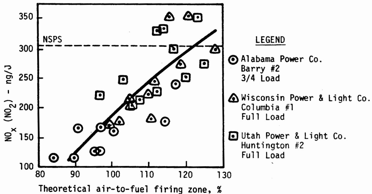
Figure 3-8. \text{NO}_x vs. theoretical air, overfire air study (Reference 3-31).
