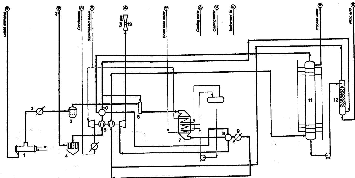
Figure 6-2. Dual pressure nitric acid plant flow diagram (Reference 6-2).
