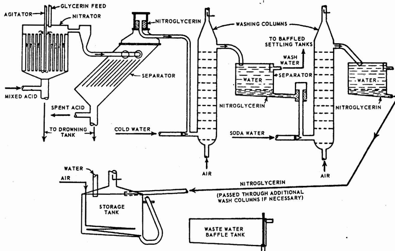
Figure 6-13. Schmid-Meissner continuous-nitration plant (Reference 6-39).
