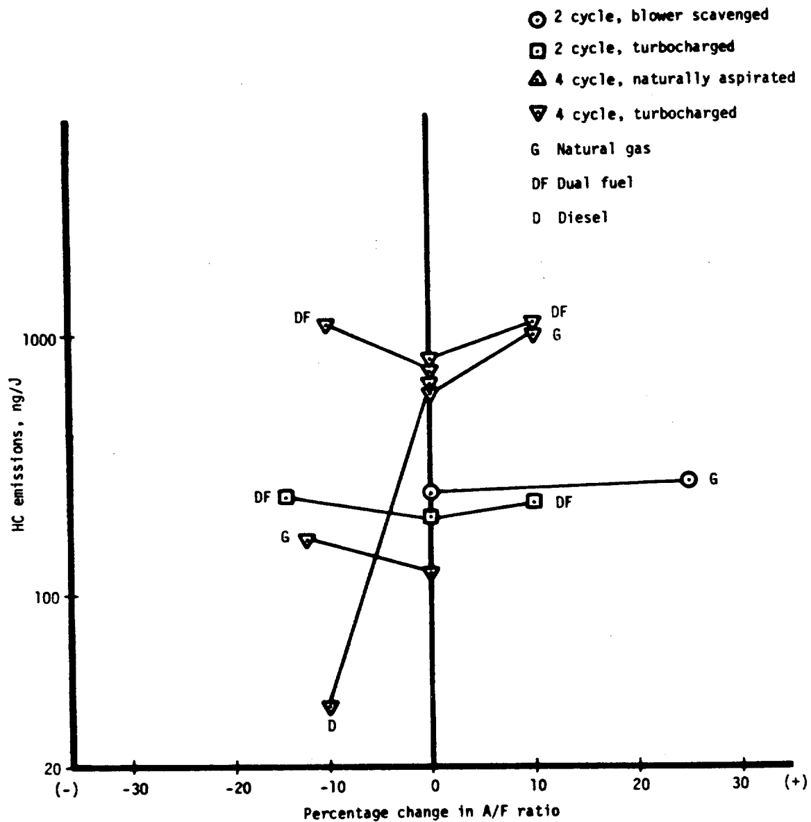
Figure 4-17. Effect of air-to-fuel ratio on IC engine HC emissions (Reference 4-56).
