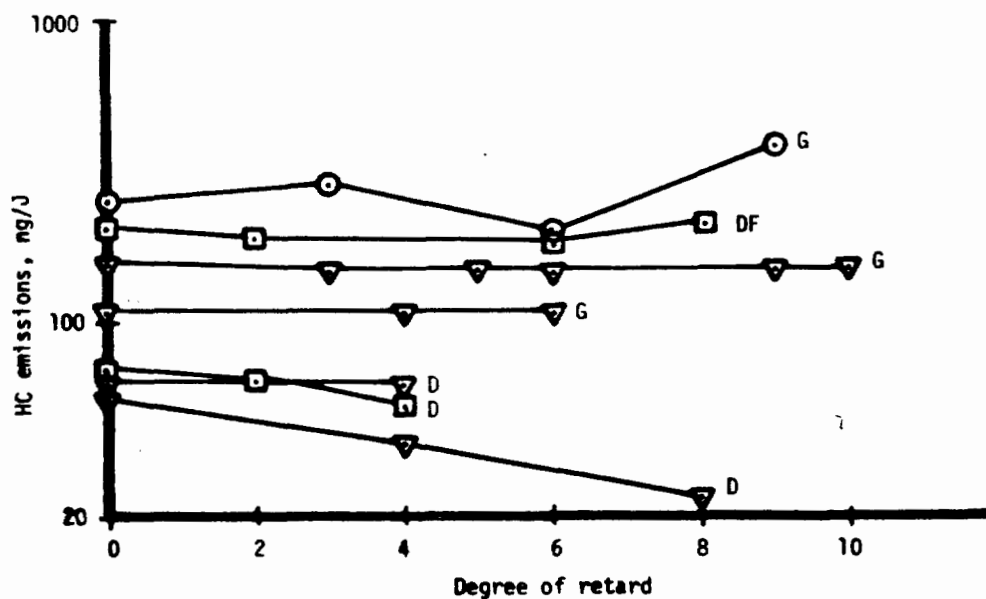
Figure 4-16. Effect of retarding ignition on IC engine HC emissions (Reference 4-56).
