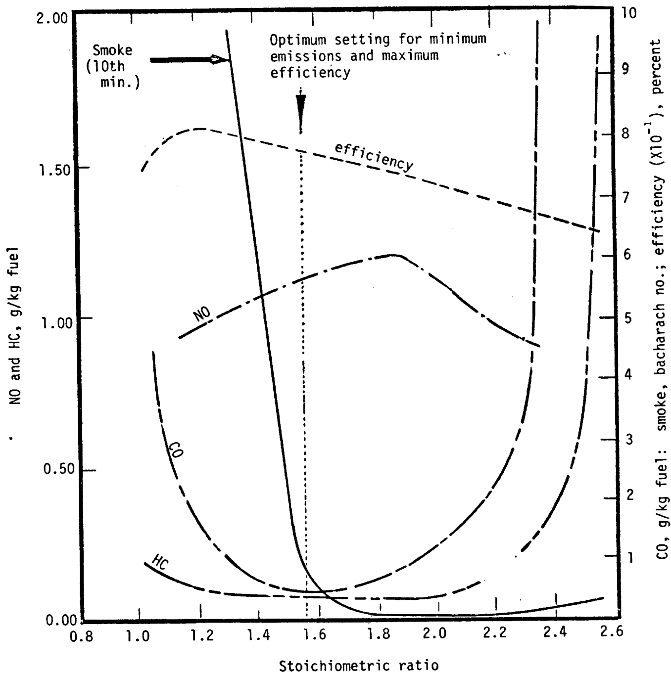
Figure 5-1. General trend of smoke, gaseous emissions, and efficiency versus stoichiometric ratio for residential heaters (Reference 5-4).
