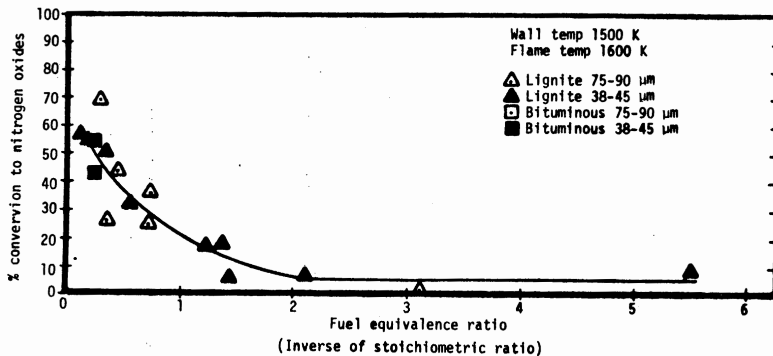
Figure 3-5. Conversion of nitrogen in coal to \text{NO}_x (Reference 3-22).
