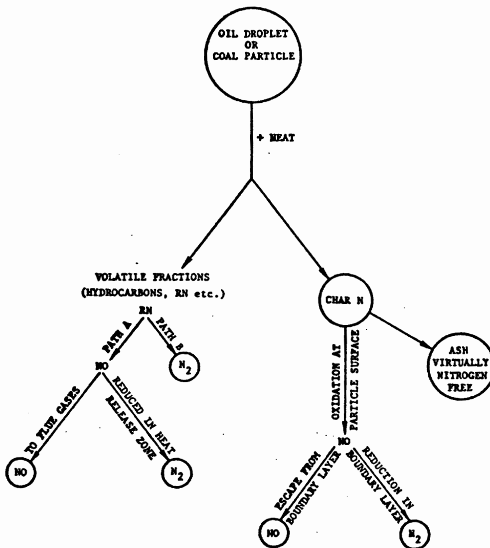
Figure 3-4. Possible fate of fuel nitrogen contained in coal particles or oil droplets during combustion (Reference 3-15).
