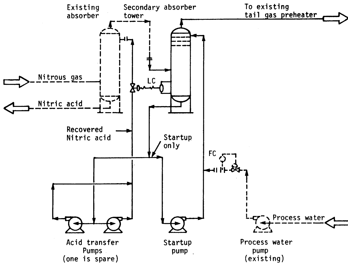
Figure 6-7. Grande Paroisse extended absorption process for \text{NO}_x Abatement.
