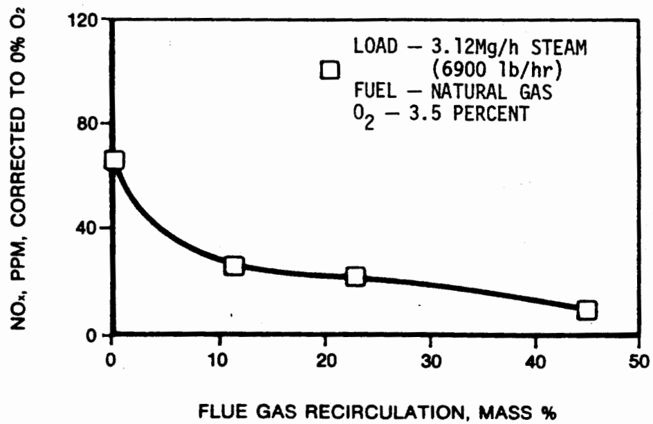
Figure 4-11. The influence of flue gas recirculation on NO x emissions from a watertube boiler (Reference 4-52).
