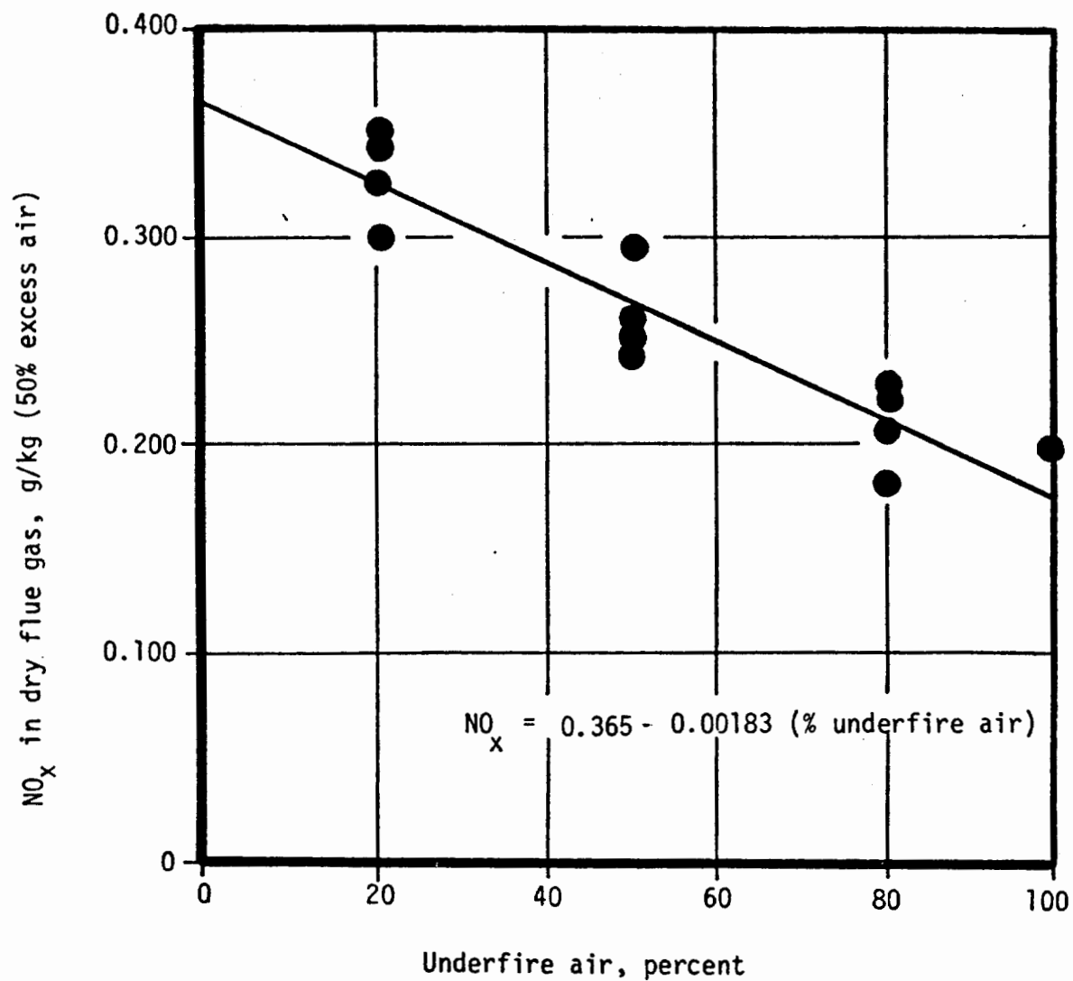
Figure 5-3. Effect of underfire air on NO x emissions from a 227 Mg (250 ton) per day continuous-feed incinerator (Reference 5-17).
