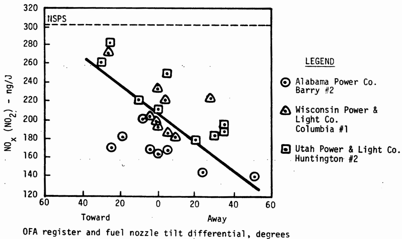
Figure 3-9. \text{NO}_x vs. tilt differential, overfire, air study (Reference 3-31).
