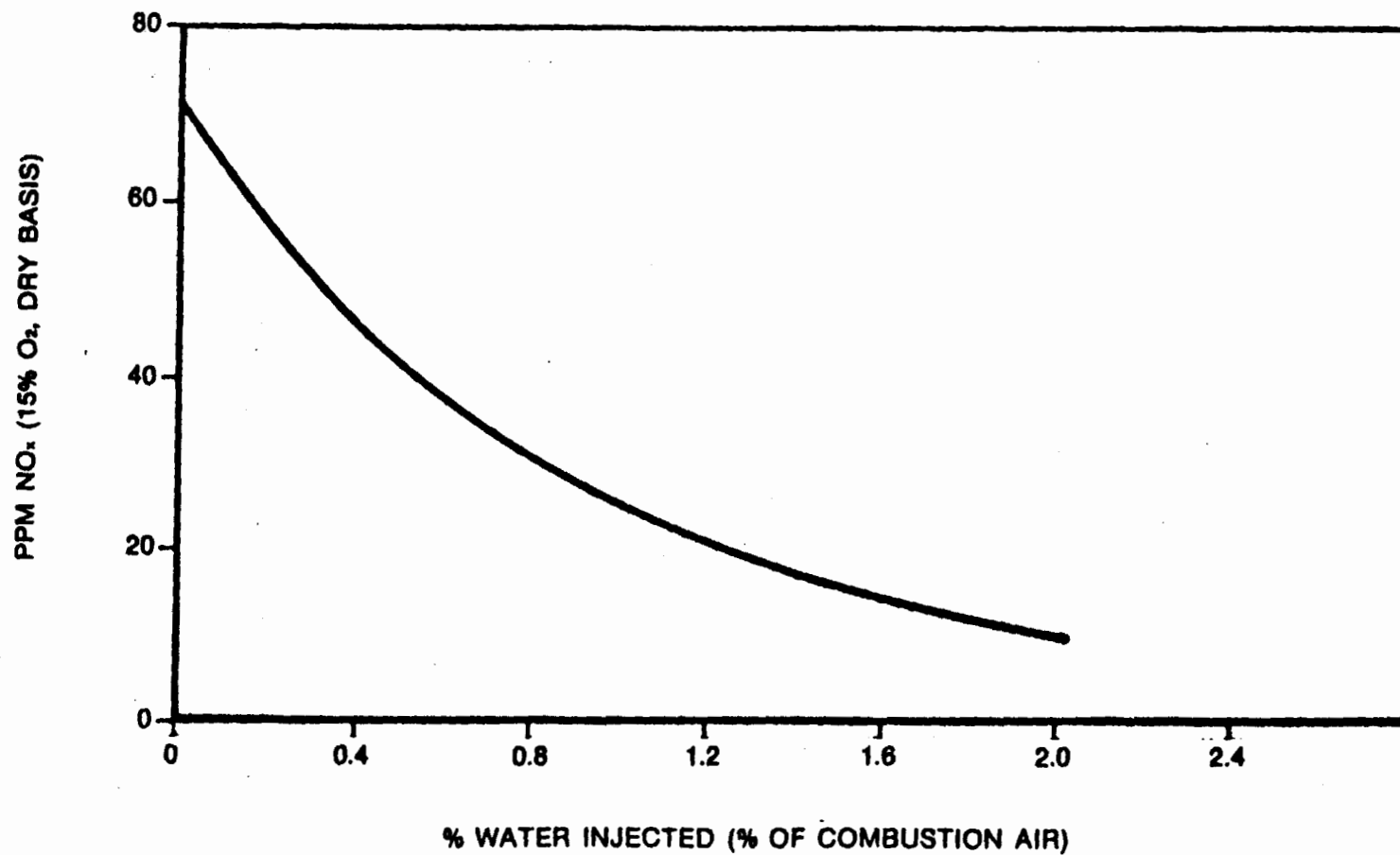
Figure 3-13. Correlation of NO x emissions with water injection rate for natural gas fired gas turbine (Houston L&P Wharton No. 43 unit) (Reference 3-35).
