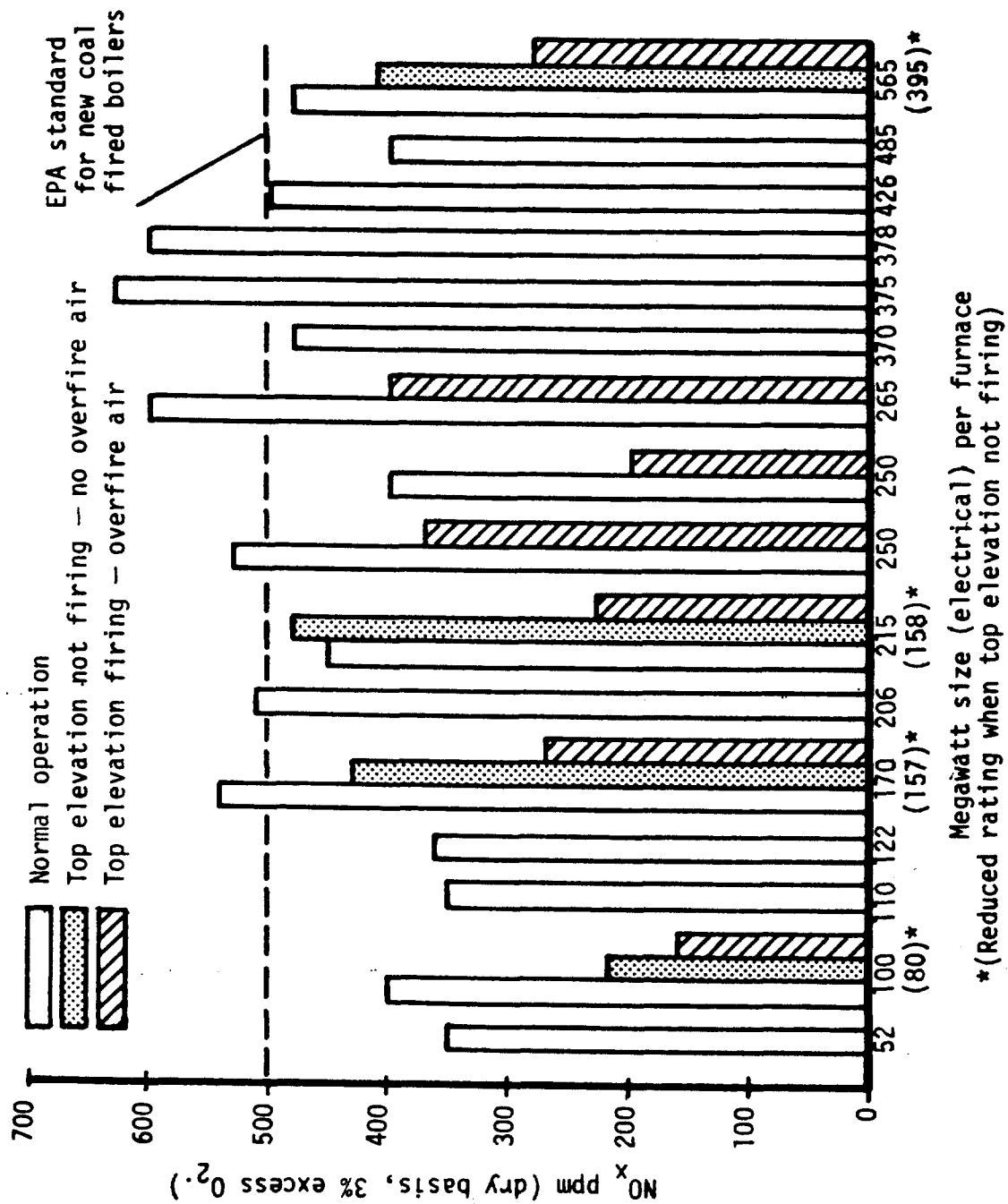
Figure 4-5. NO x emissions from tangential, coal-fired utility boilers (Reference 4-6).
