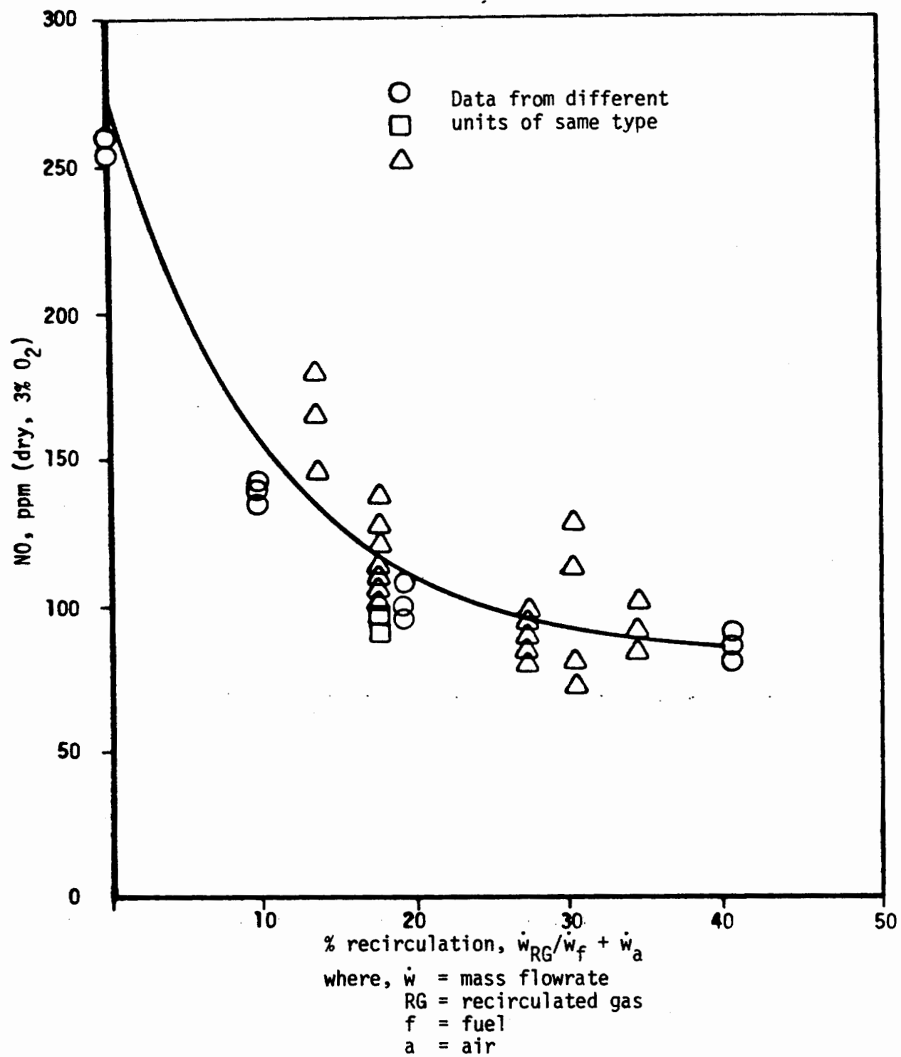
Figure 3-11. Effect of FGR on NO emissions (Reference 3-32).
