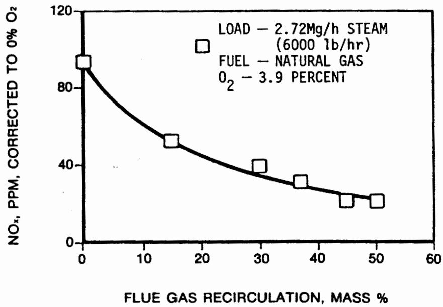
Figure 4-10. The influence of flue gas recirculation on NO x emissions from a firetube boiler (Reference 4-52).
