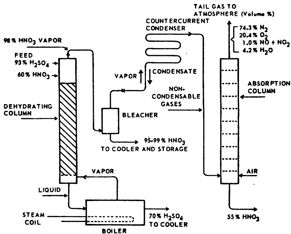
Figure 6-3. Nitric acid concentrating unit.
