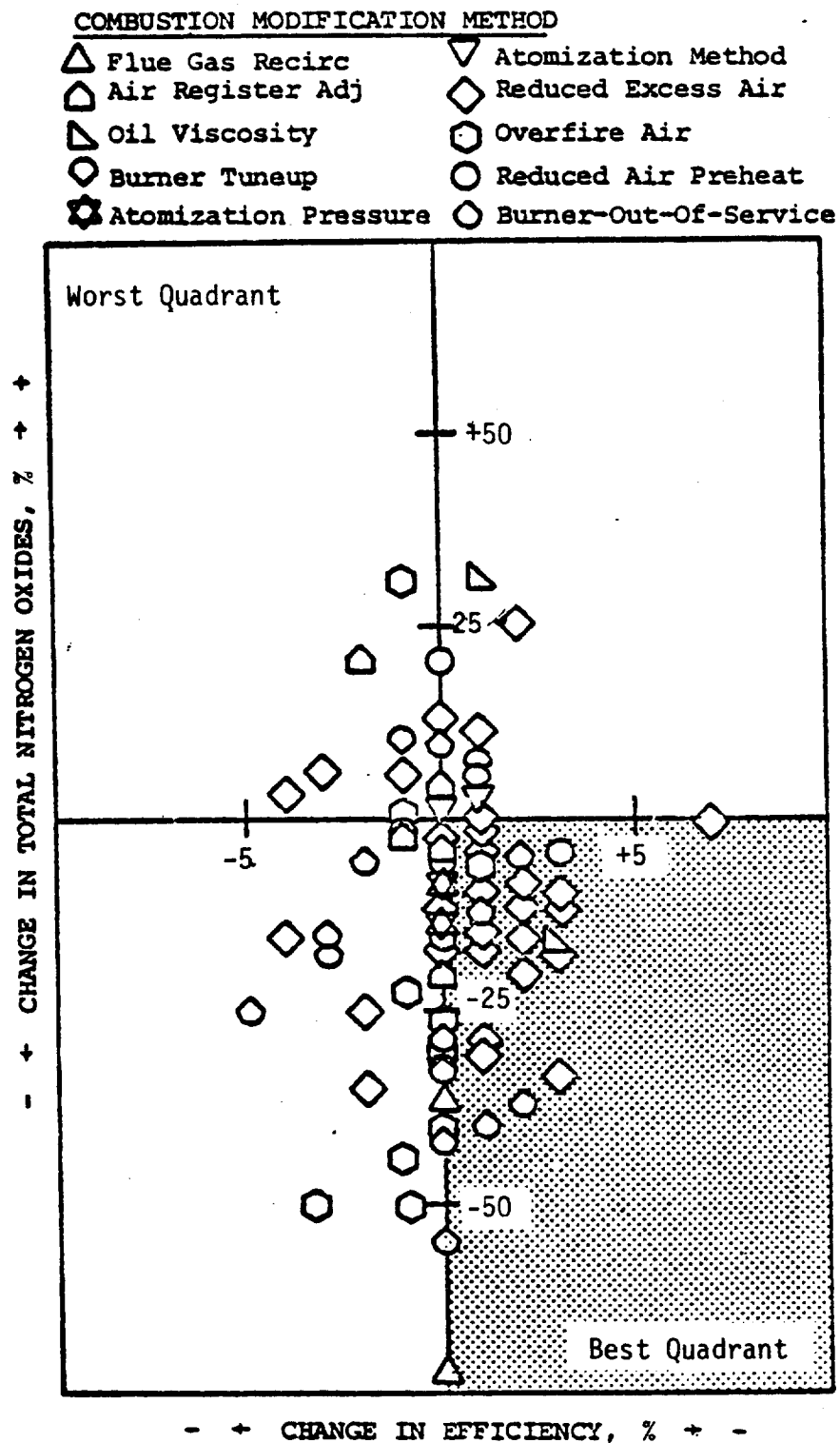
Figure 4-9. Effect of combustion modification methods on total nitrogen oxides emissions and boiler efficiency (Reference 4-50).
