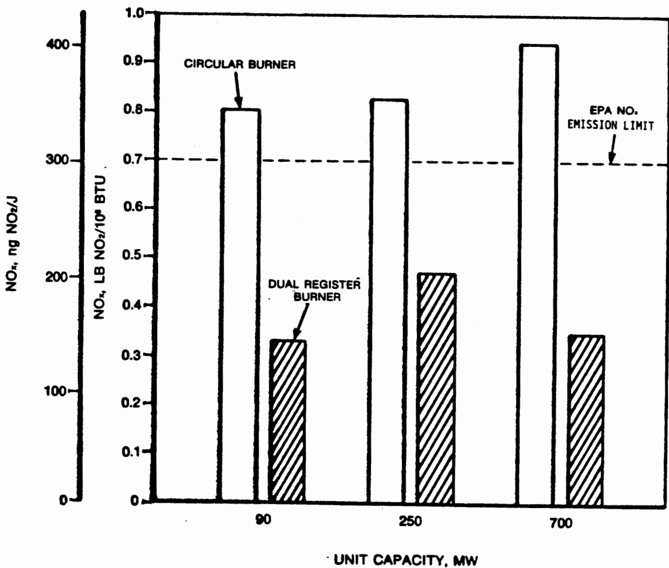
Figure 3-14. Comparison of NO x emissions with pulverized coal firing, circular burner vs. dual register burner (Reference 3-47).
