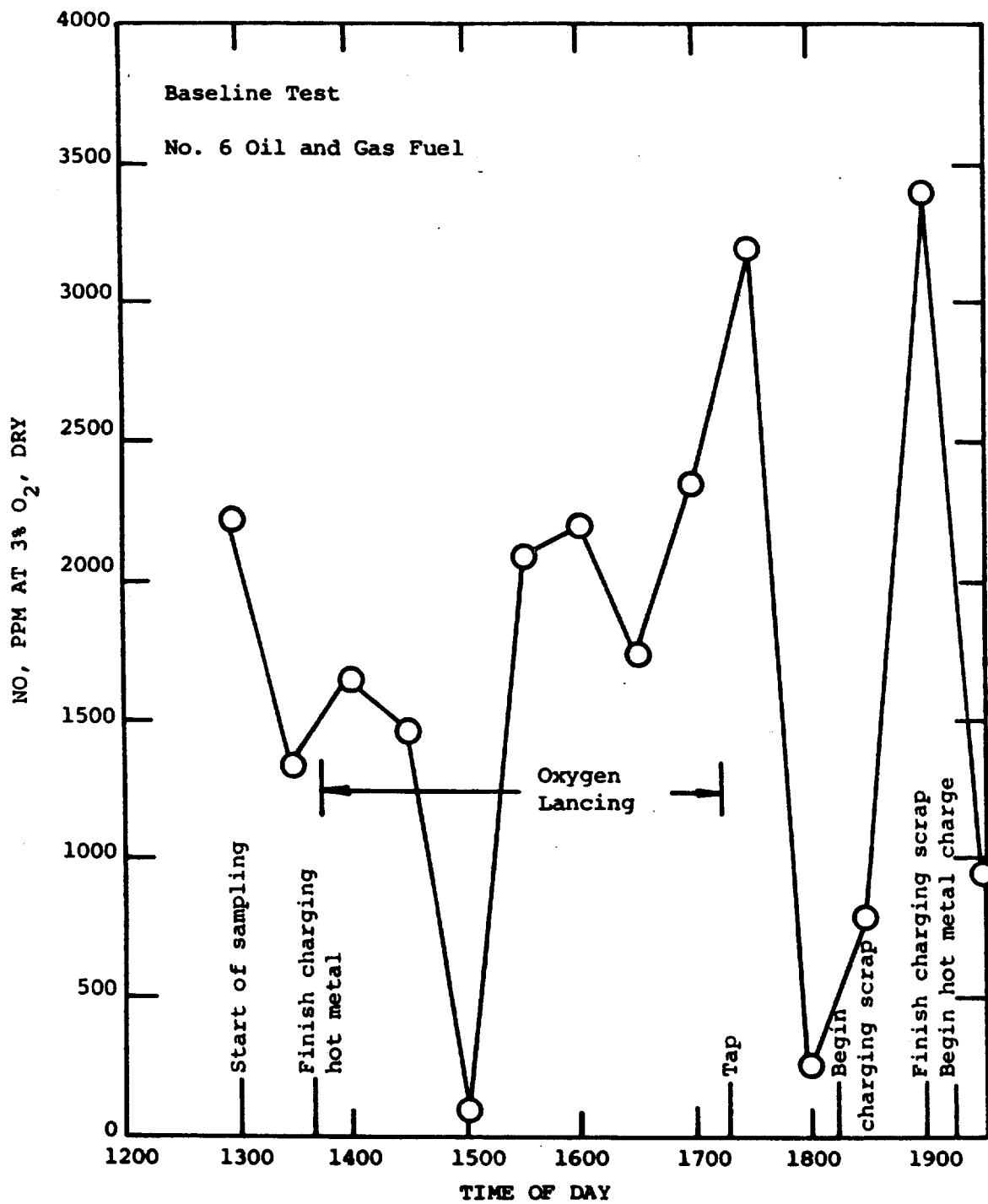
Figure 5-5. NO emissions as a function of time for an open hearth furnace (Reference 5-26).
