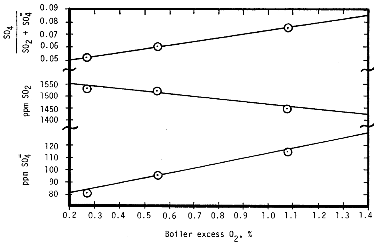
Figure 4-8. SO_2 conversion vs. excess oxygen in coal-fired utility boilers (Reference 4-40).
