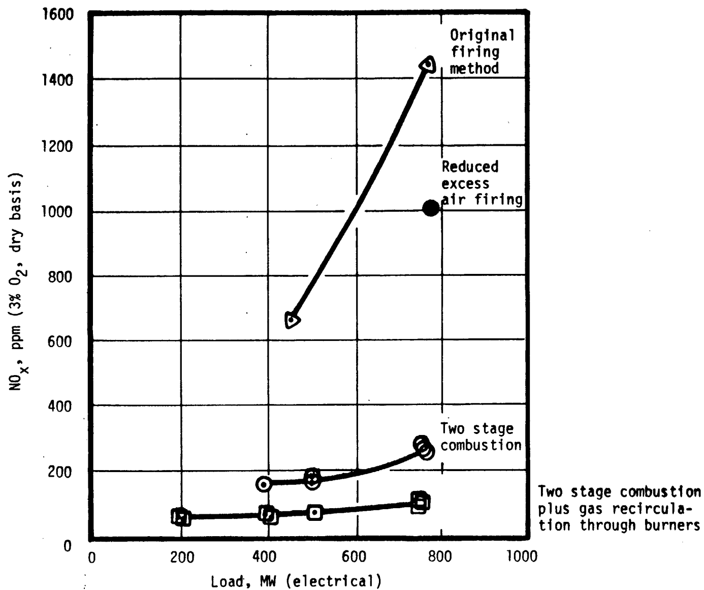
Figure 4-2. Effects on NO x control methods on a gas, wall-fired utility boiler (Reference 4-4).
