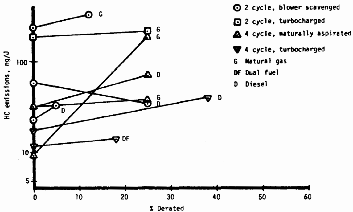
Figure 4-15. Effect of derating on IC engine HC emissions (Reference 4-56).
