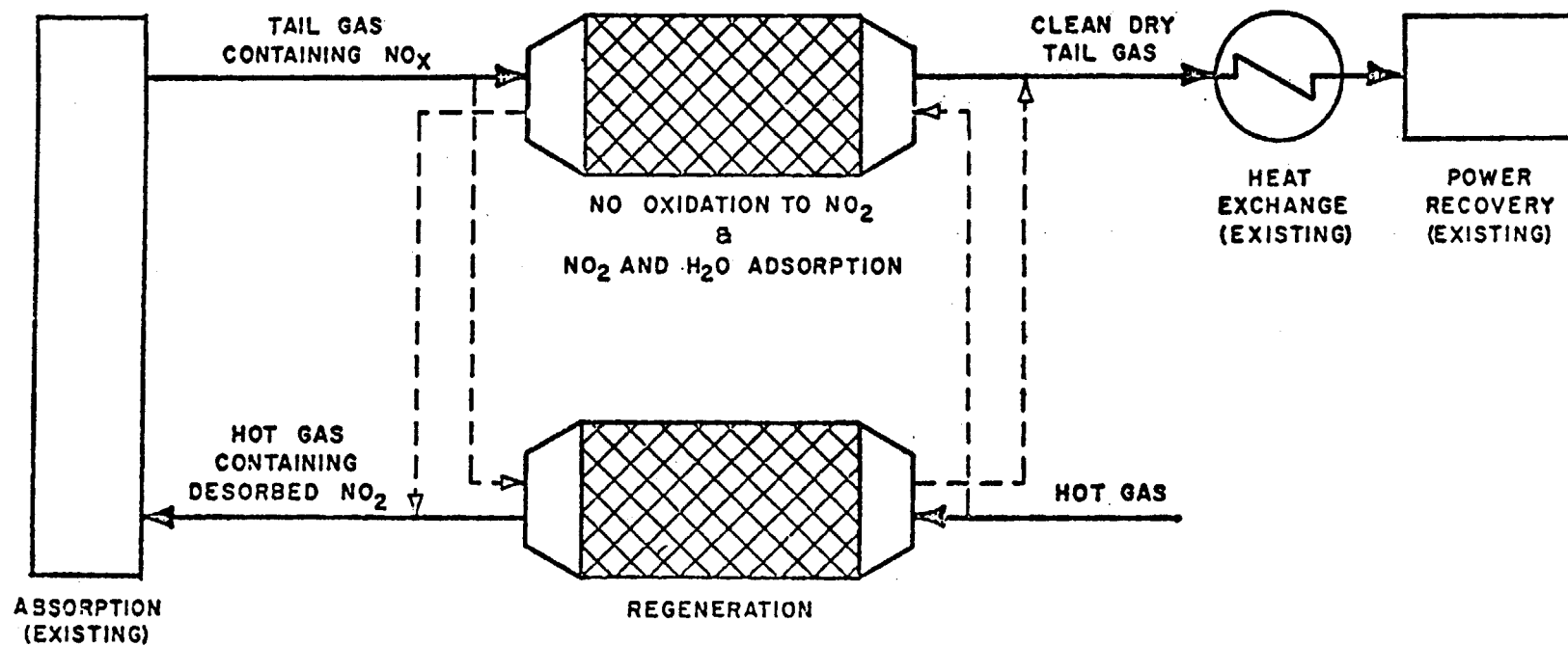
Figure 6-11. Molecular sieve system (Reference 6-22).
