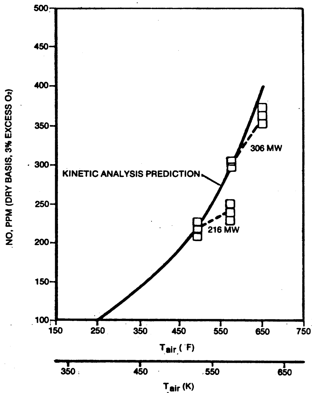
Figure 3-12. Reduced air preheat with natural gas firing, 320 MW corner-fired unit (Reference 3-32).
