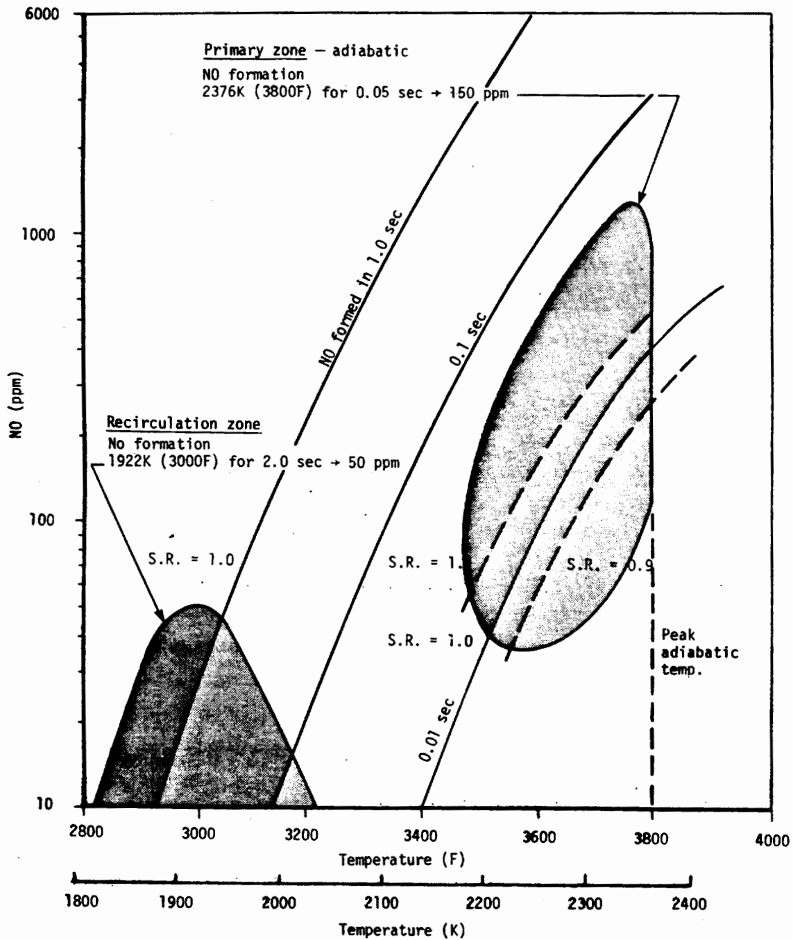
Figure 3-1. Kinetic formation of nitric oxide for combustion of natural gas atmospheric pressure (References 3-3 and 3-4).
