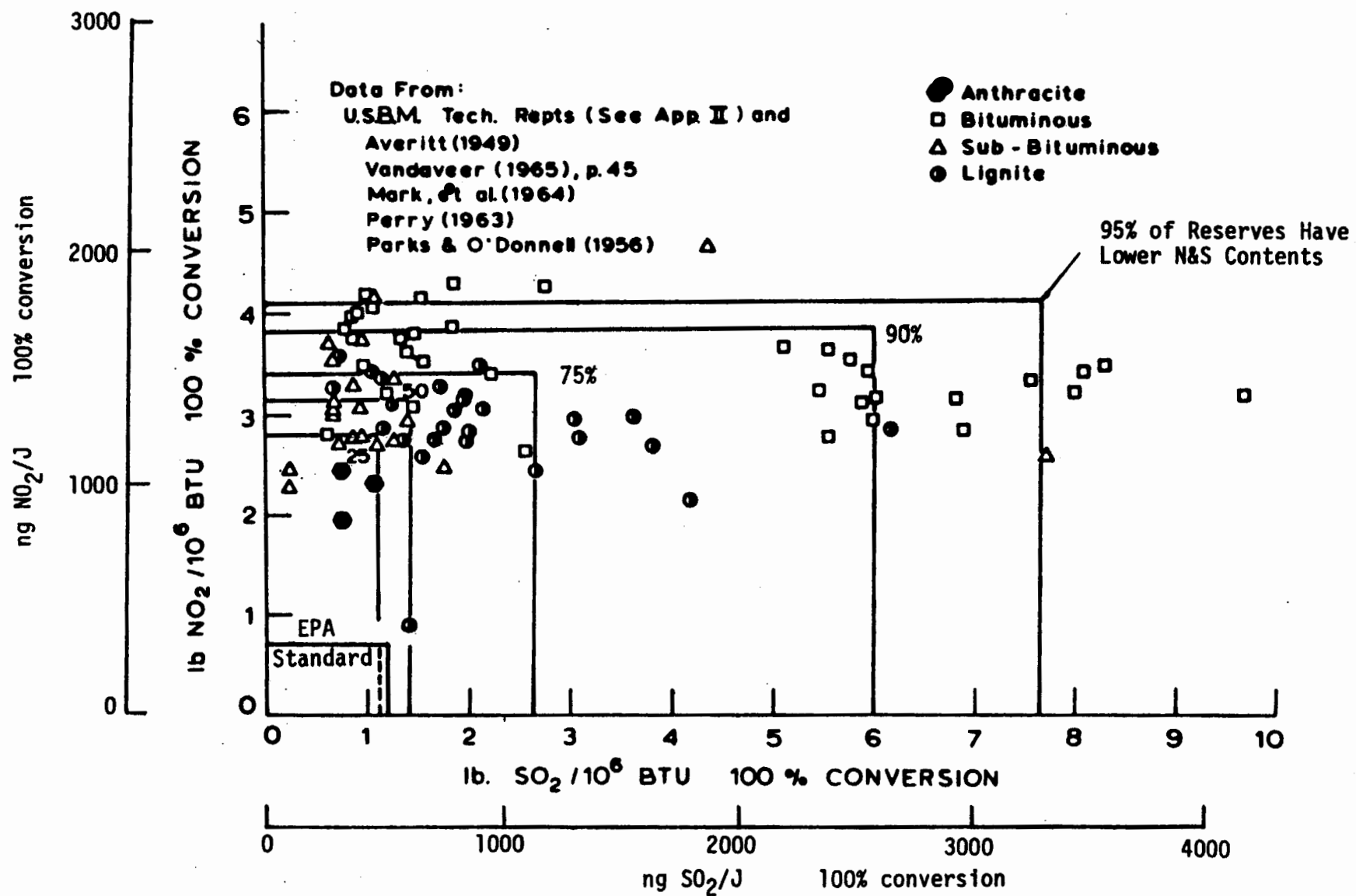
Figure 3-2. Nitrogen and sulfur content of U.S. coal reserves (Reference 3-13).
