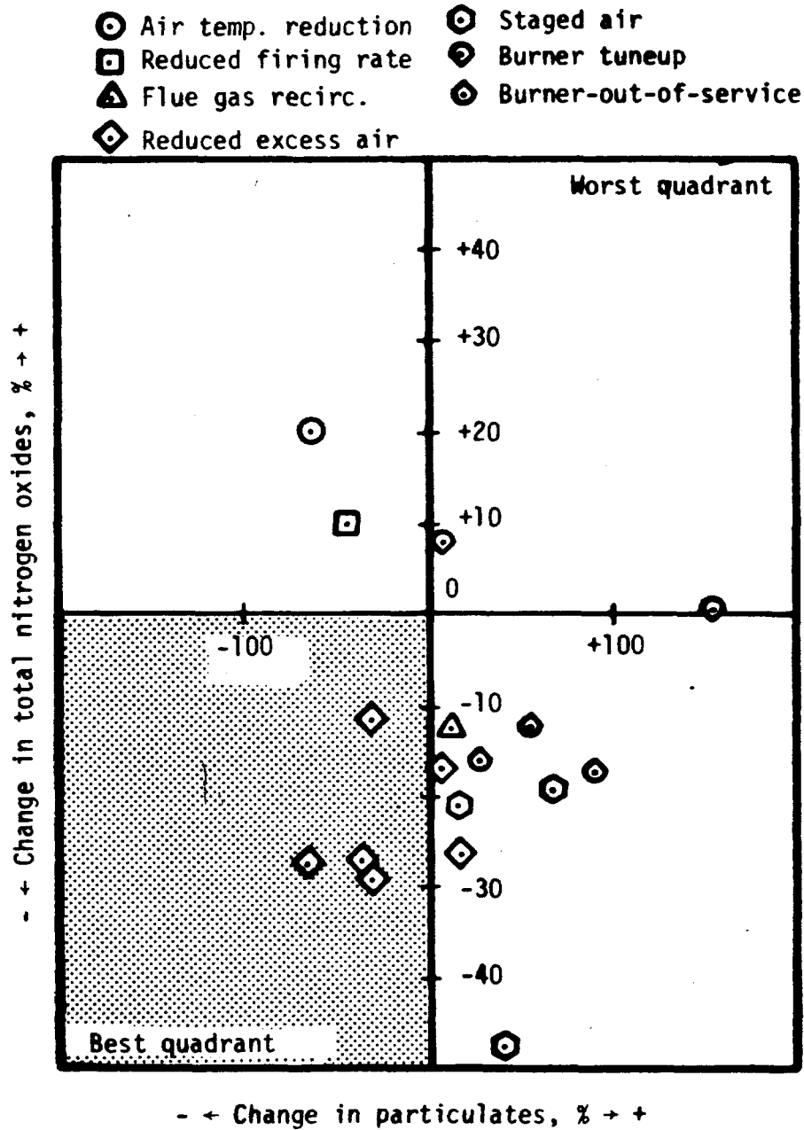
Figure 4-12. Effect of NO x Controls on solid particulate emissions from industrial boilers (Reference 4-50).
