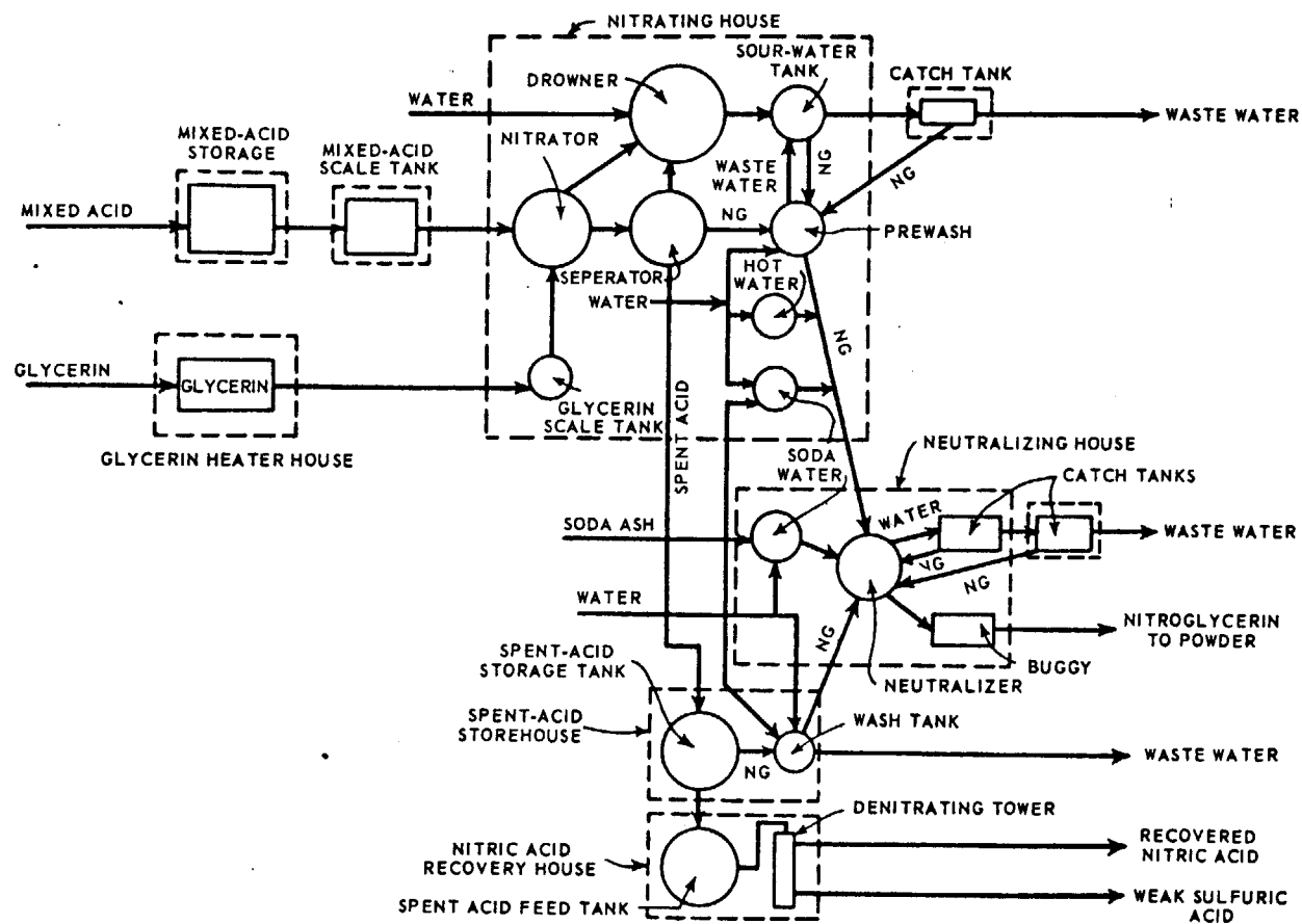
Figure 6-12. Batch process for the manufacture of nitroglycerin (NG) (Reference 6-39).
