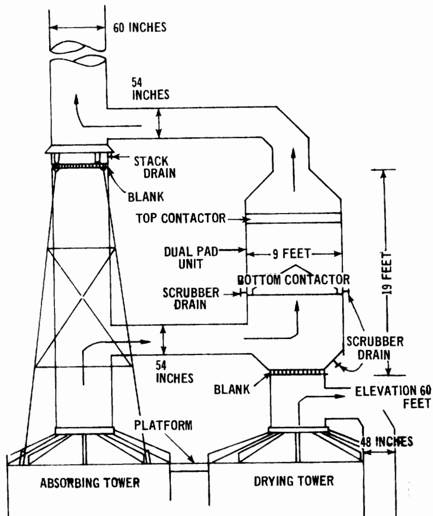
Figure 6.6. Retrofit horizontal dual pad mist eliminator installation.
