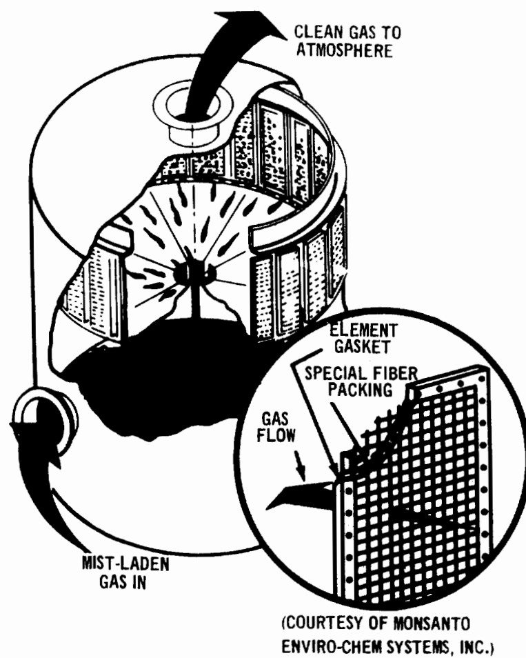
Figure 6.2. Vertical panel mist eliminator.
