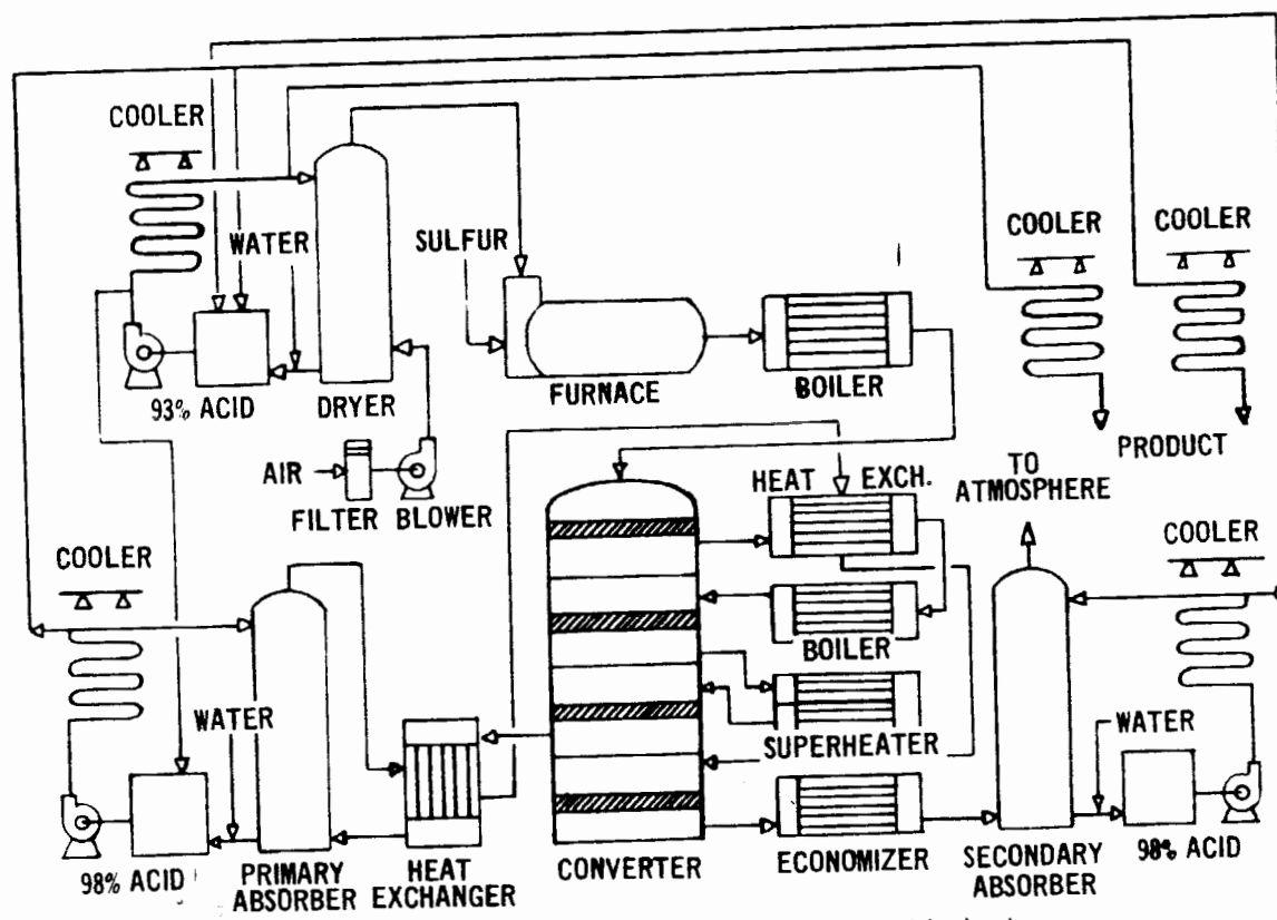
Figure 3.3. Dual absorption sulfuric acid plant.
