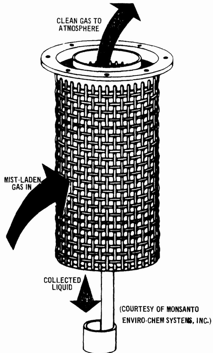
Figure 6.1. Vertical tube mist eliminator element.
