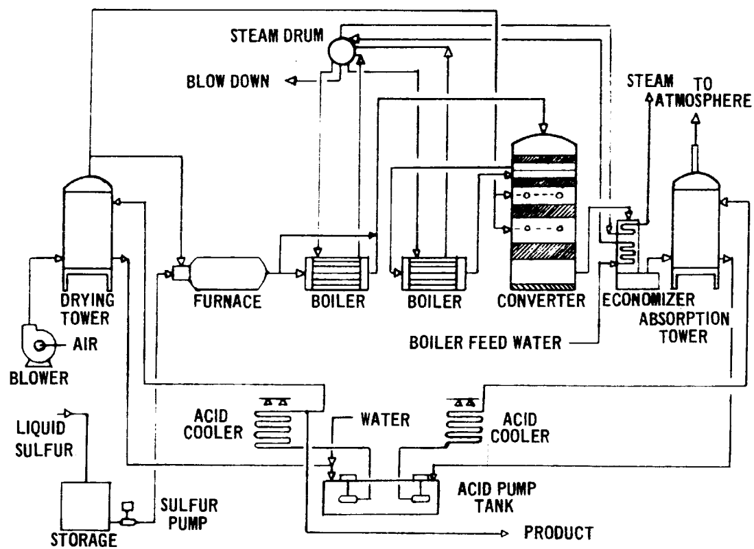
Figure 3.1. Contact-process sulfuric acid plant burning elemental sulfur.
