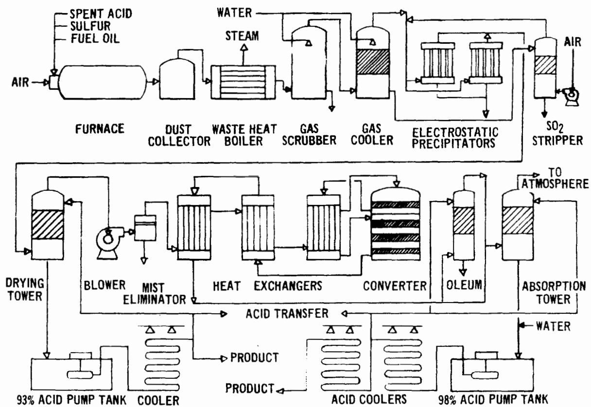
Figure 3.2. Contact-process sulfuric acid plant burning spent acid.
