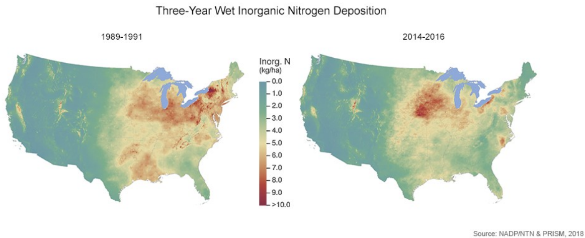
Figure 2. Three-Year Wet Inorganic Nitrogen Deposition
