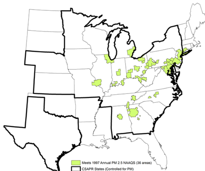
Figure 2. Changes in PM 2.5 NAAQS Nonattainment Areas in CSAPR Region, 2001–2003 (Original Designations) versus 2014–2016
