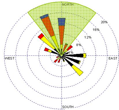
Temple Elementary School Composite Hourly Windrose on Sample Days (Oct. 28, 2009-Mar. 8, 2010)
