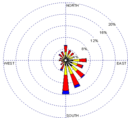
Angelina County Airport NWS Station Composite Hourly Windrose, 2002-2007 1
