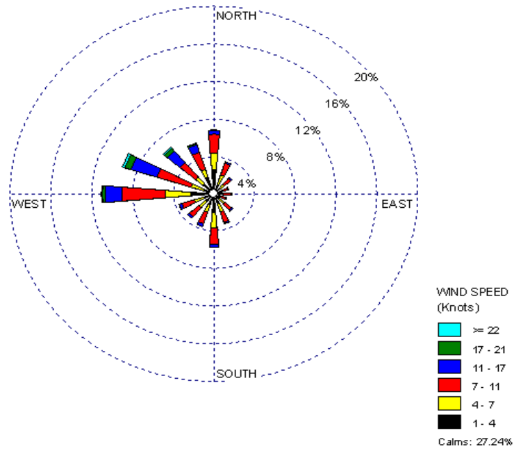
Reading Regional/C A Spaatz Field Airport NWS Station 2002-2007
