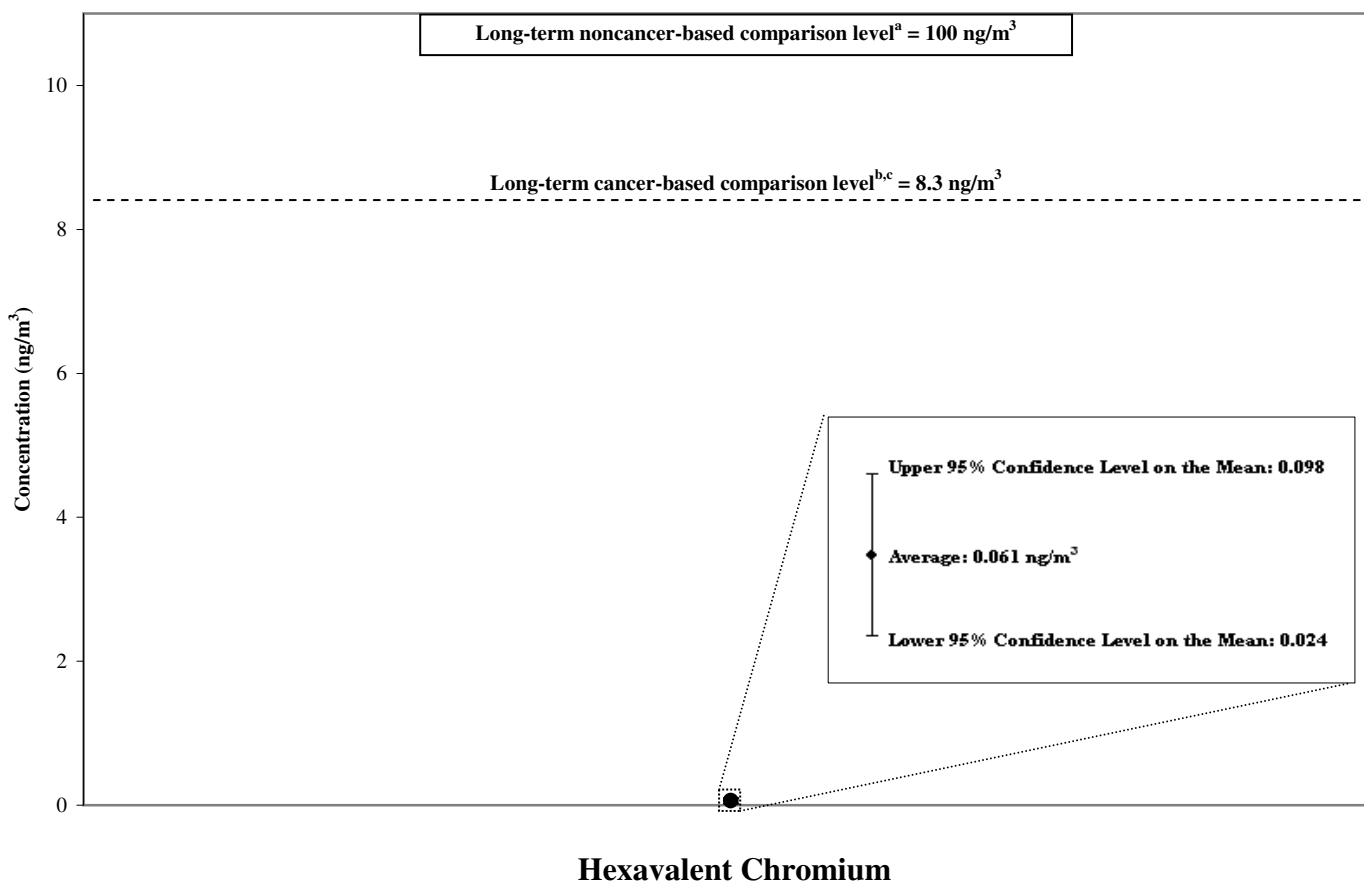
Figure 1. Riverside Elementary School - Key Pollutant (Hexavalent Chromium) Analysis.
