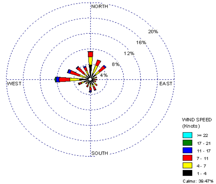
Reading Regional/C A Spaatz Field Airport NWS Station Across Sampling Period (July 30-Oct. 28, 2009) 1
