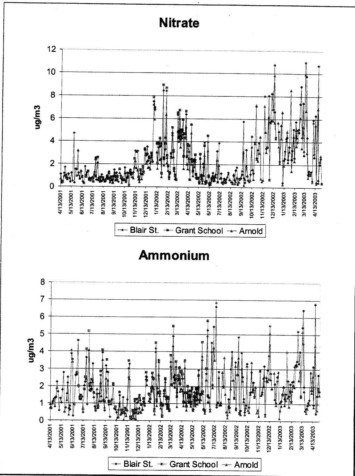
Figure 2.2-2. St. Louis area \text{PM}_{2.5} speciation results, nitrate and ammonium.
