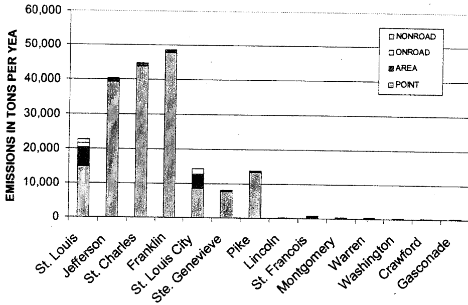
Figure 2.3-3. SO 2 EMISSIONS IN THE ST. LOUIS AREA
