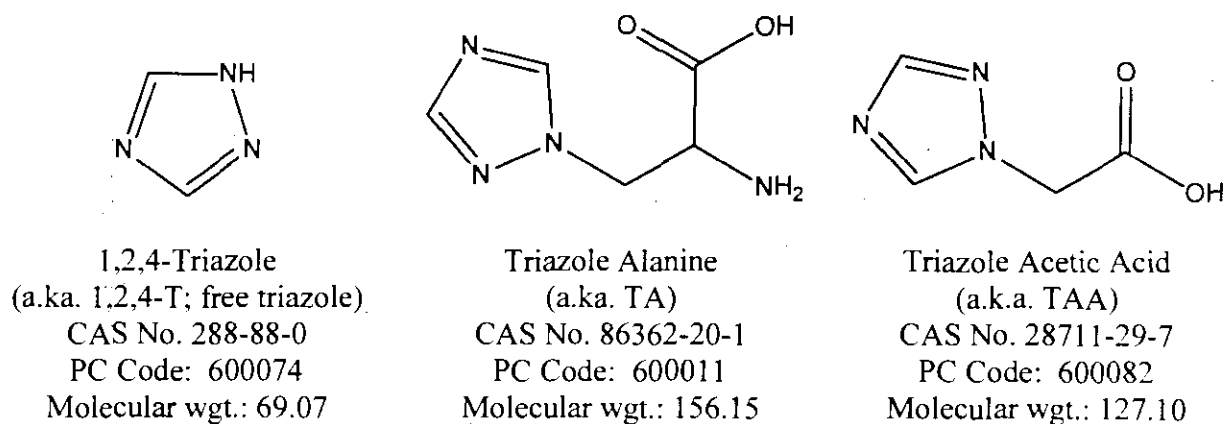
Figure 1.1. Chemical structures for 1,2,4-triazole, triazole alanine, and triazole acetic acid
