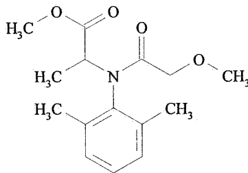
Figure 1. Metalaxyl/Mefenoxam
