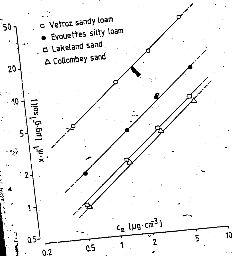
Fig. 1 Freundlich Adsorption Isotherms, Metolachlor for various Soil Types.
