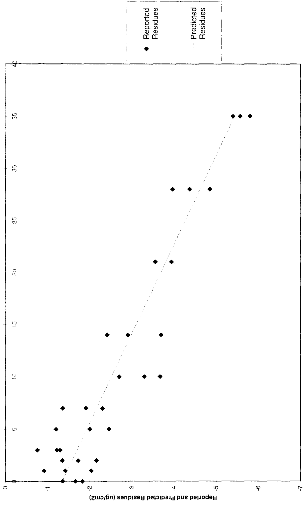
Regression Analysis: A Plot of Natural Log of Combined Residues (Acephate and Methamidophos) vs Time
