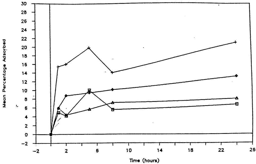
Figure 1. Mean percentage of adsorption with time of ^{14}\text{C} -Prometryn from a 10.2\text{-}\mu\text{g/mL} solution (10 mL) of ^{14}\text{C} -Prometryn in aqueous 0.01\text{M Ca(NO}_3)_2 to duplicate soil samples of Mississippi silt loam (□), Kewaunee clay loam (+), California sandy loam (◇), and Plainfield sand (Δ).
