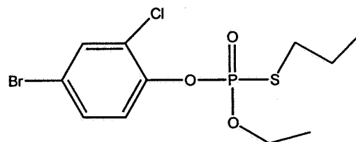
Profenophos
