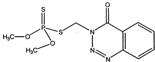
Azinphos-methyl
