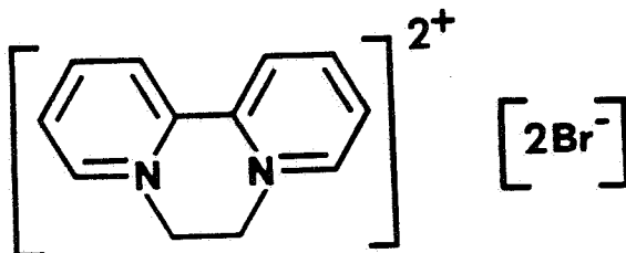
6,7-Dihydrodipyrido(1,2-a:2',1'-c)pyrazinedium dibromide
