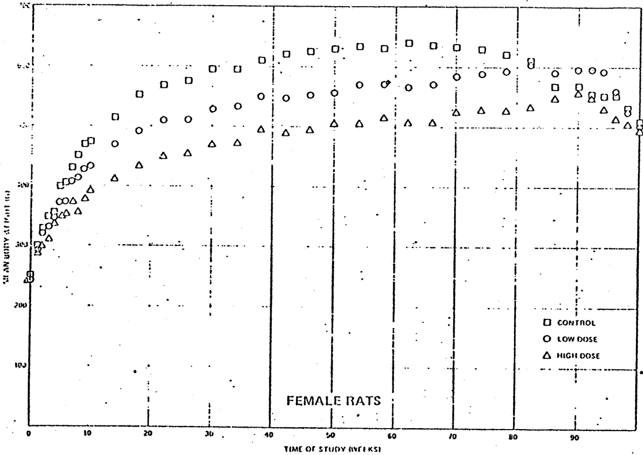
Figure 2. Growth Curves for Rats - Chloroform
